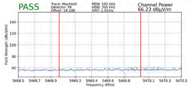
Plot 7-294. Radiated Lower Band Edge Plot SISO ANT1 (Peak - UNII Band 2C)
