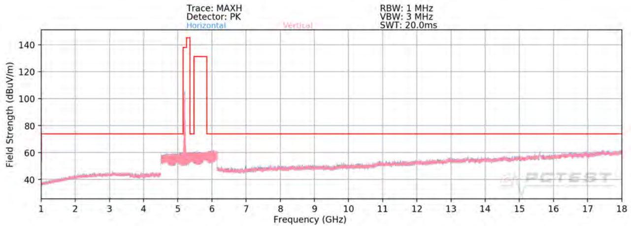
Plot 7-265. Radiated Spurious Plot above 1GHz SISO ANT2 (802.11a – U1 Ch. 40)
