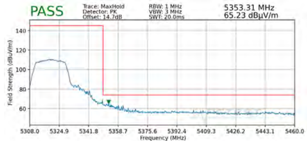
Plot 7-327. Radiated Upper Band Edge Plot MIMO (Peak – UNII Band 2A)
