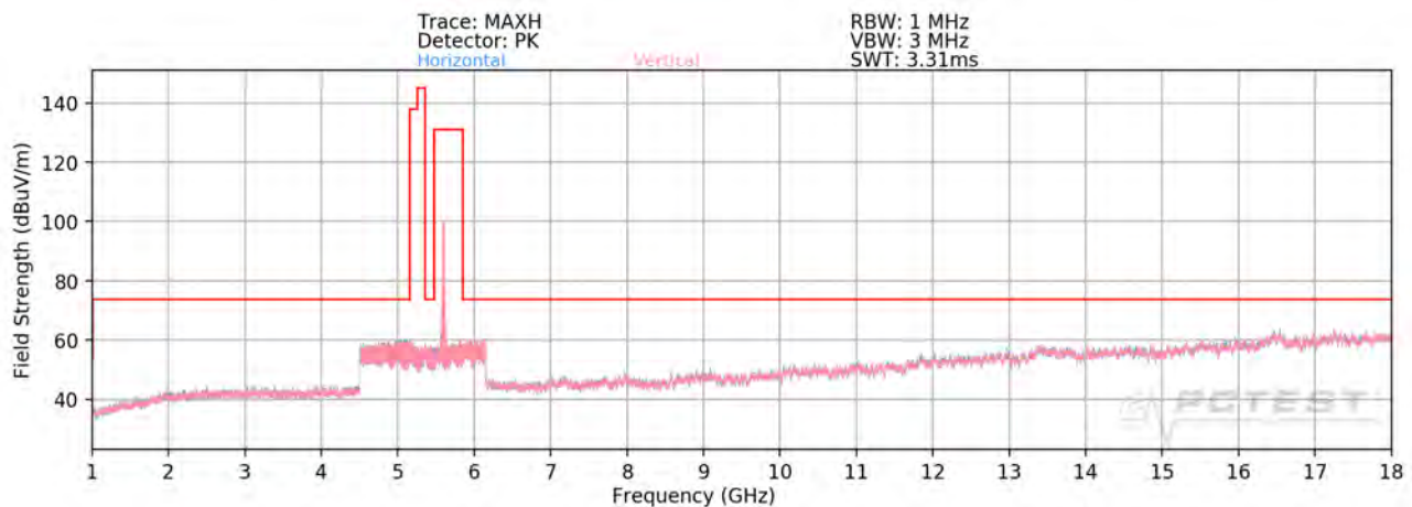
Plot 7-261. Radiated Spurious Plot above 1GHz SISO ANT1 (802.11a – U2C Ch. 116)
