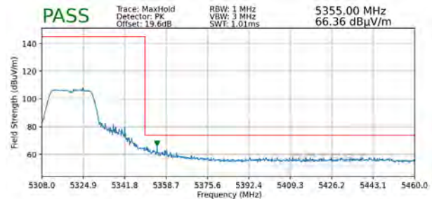
Plot 7-285. Radiated Upper Band Edge Plot SISO ANT1 (Peak – UNII Band 2A)
