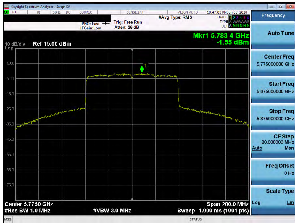
Plot 7-258. Power Spectral Density Plot SISO ANT2 (80MHz BW 802.11ax (UNII Band 3) – Ch. 155)
