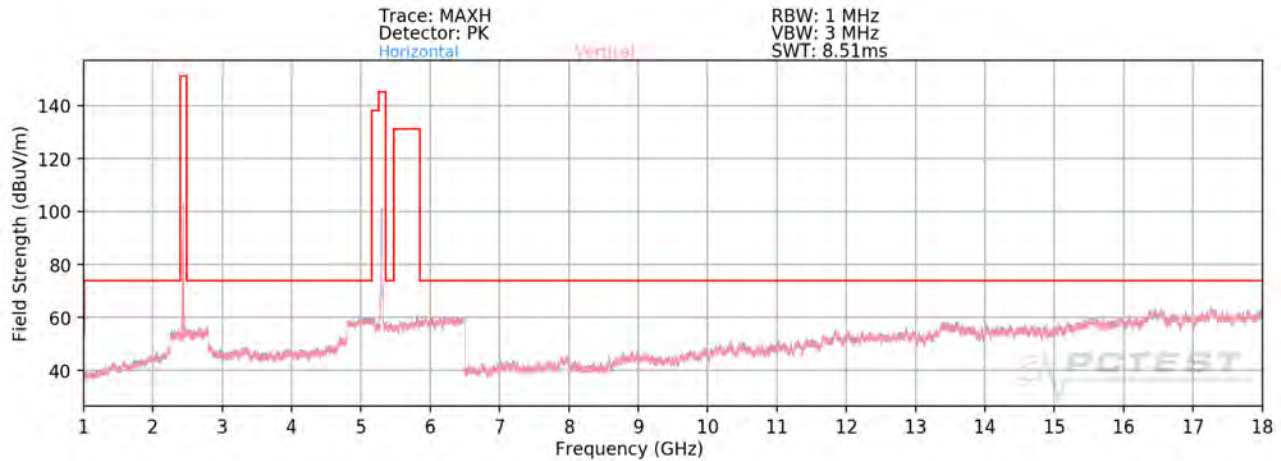
Plot 7-279. Radiated Spurious Plot above 1GHz (Dual Band Simult. Tx)
