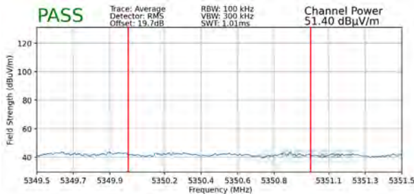
Plot 7-305. Radiated Upper Band Edge Plot SISO ANT2 (Average – UNII Band 2A)
