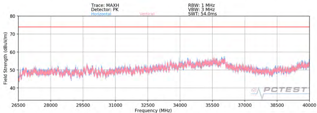
Plot 7-270. Radiated Spurious Plot 26.5GHz - 40GHz SISO ANT2 (802.11a)
