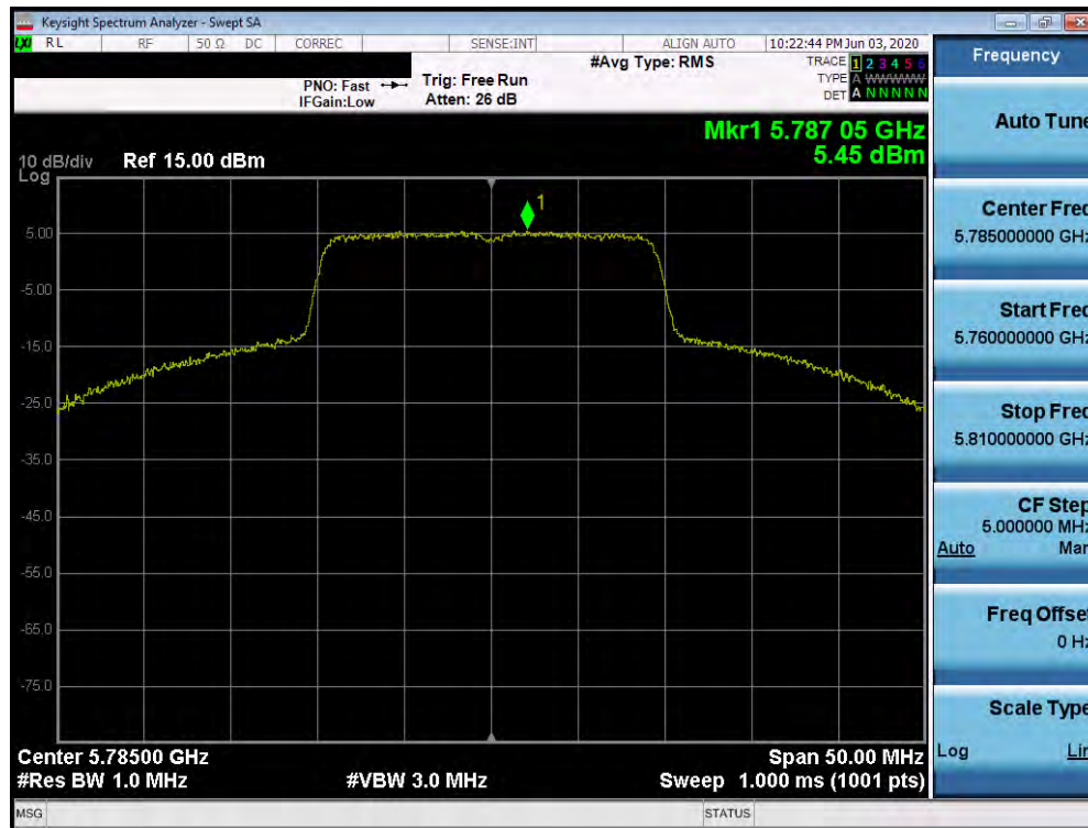
Plot 7-251. Power Spectral Density Plot SISO ANT2 (20MHz BW 802.11ax (UNII Band 3) – Ch. 157)
