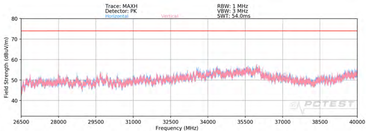
Plot 7-264. Radiated Spurious Plot 26.5GHz - 40GHz SISO ANT1 (802.11a)
