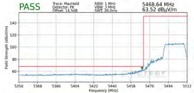
Plot 7-308. Radiated Lower Band Edge Plot SISO ANT2 (Peak - UNII Band 2C)
