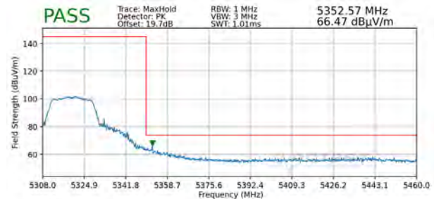
Plot 7-306. Radiated Upper Band Edge Plot SISO ANT2 (Peak – UNII Band 2A)
