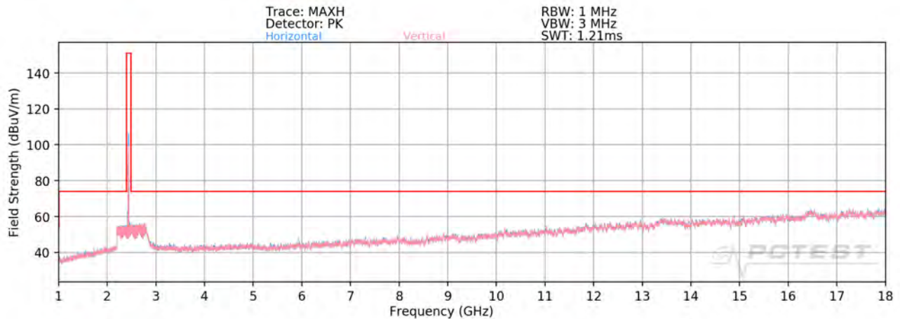
Plot 7-90. Radiated Spurious Plot above 1GHz SISO ANT2 (802.11b – Ch. 6)
