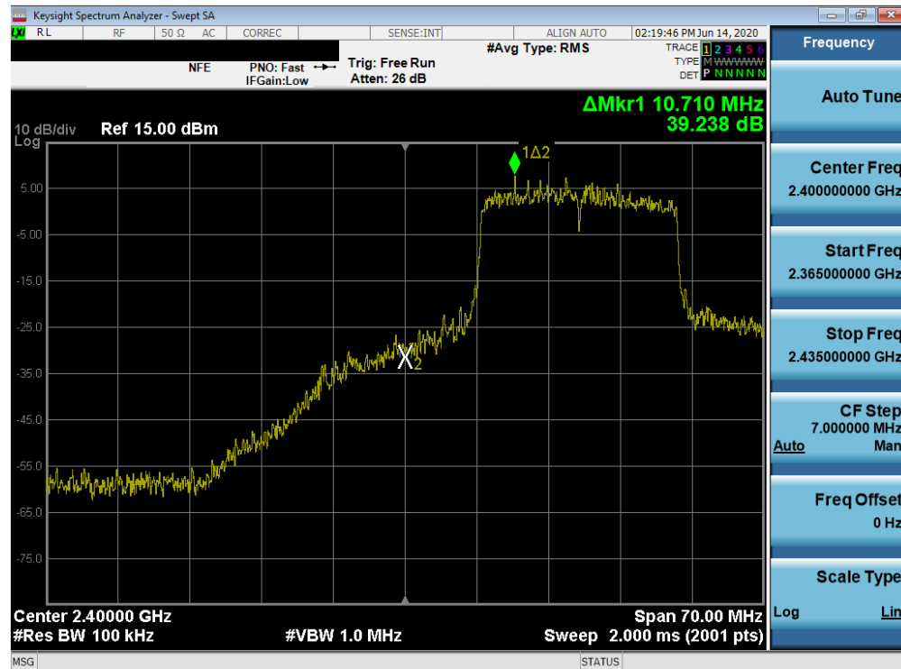
Plot 7-70. Band Edge Plot SISO ANT2 (802.11ax (2.4GHz) – Ch. 2)
