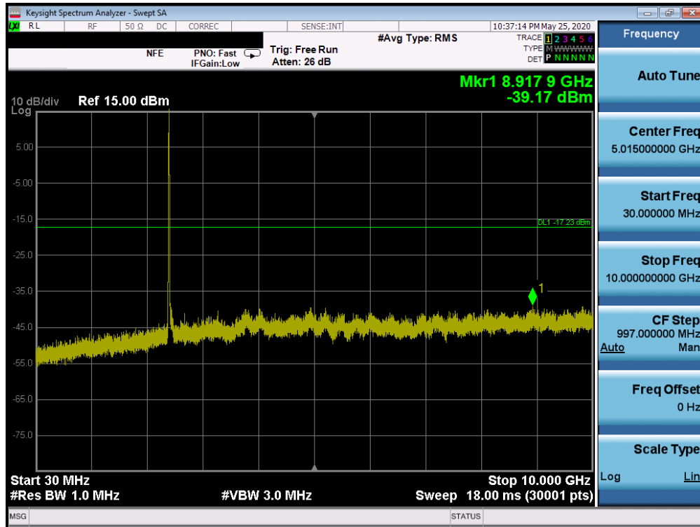
Plot 7-73. Conducted Spurious Plot SISO ANT1 (802.11b – Ch. 1)
