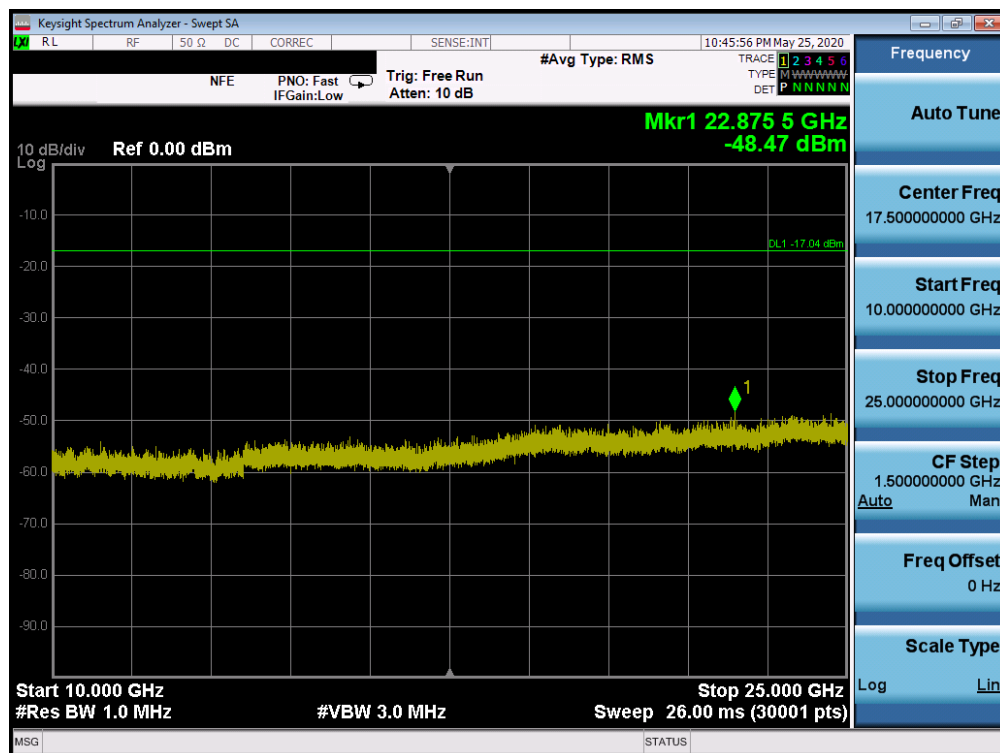
Plot 7-84. Conducted Spurious Plot SISO ANT2 (802.11b – Ch. 11)
