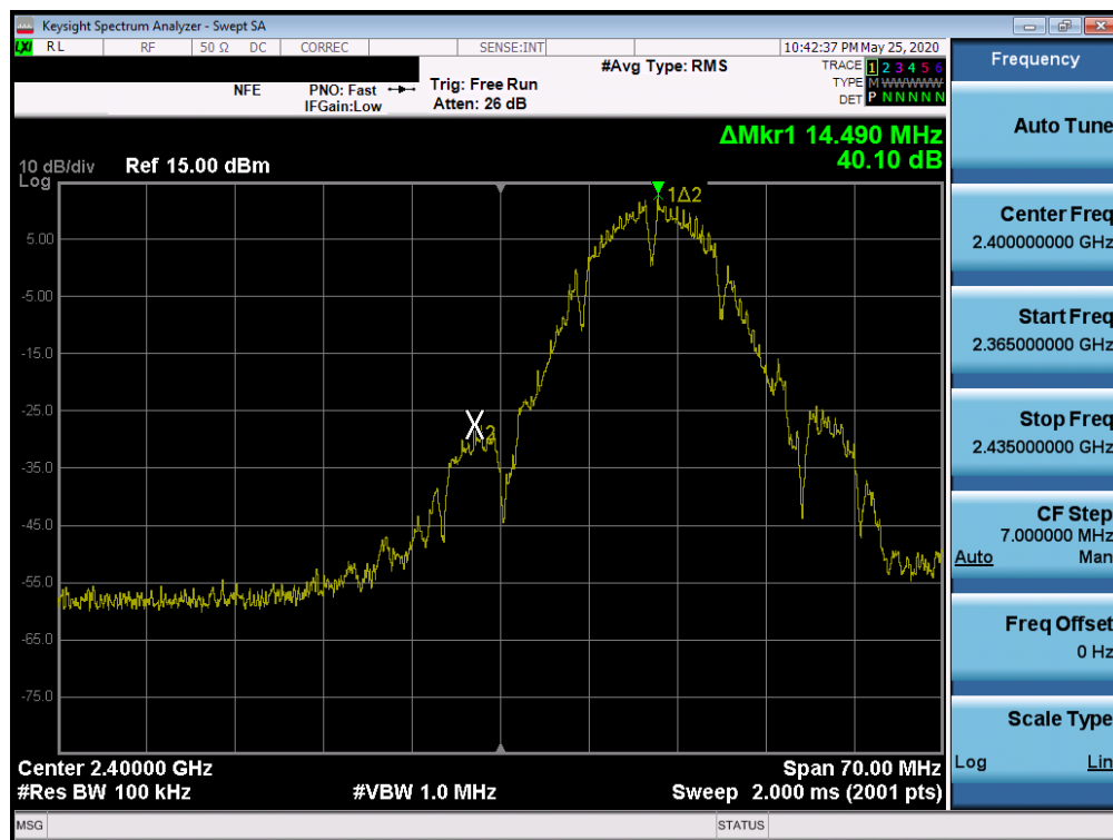
Plot 7-61. Band Edge Plot SISO ANT2 (802.11b - Ch. 1)
