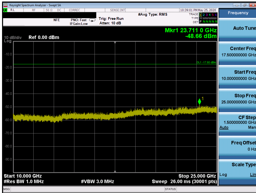
Plot 7-76. Conducted Spurious Plot SISO ANT1 (802.11b – Ch. 6)
