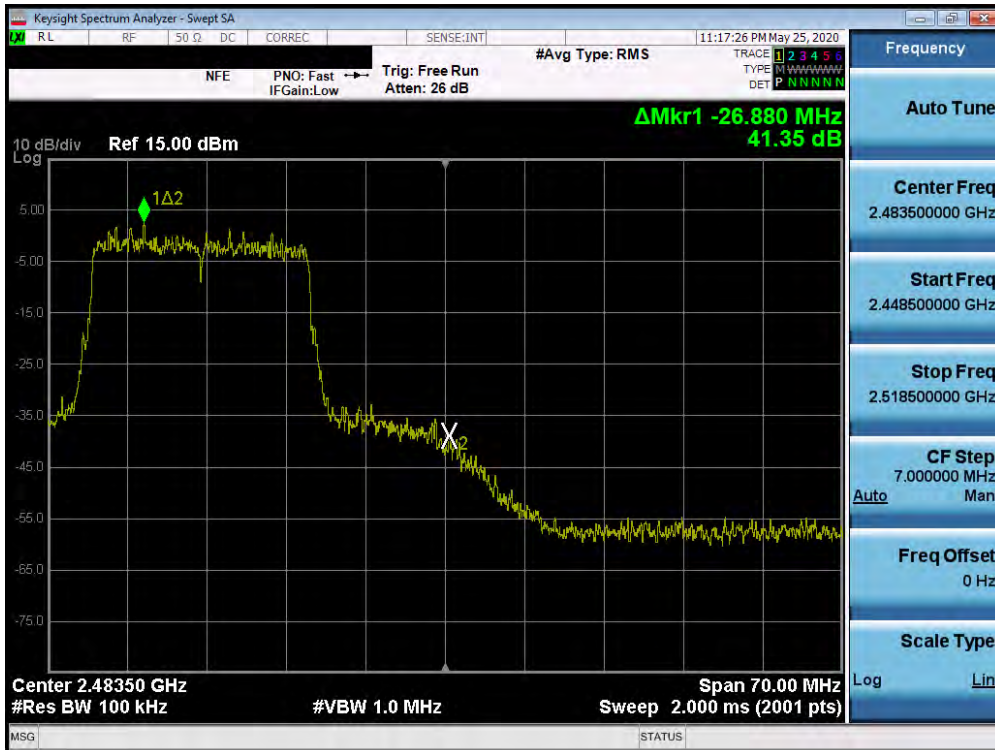
Plot 7-72. Band Edge Plot SISO ANT2 (802.11ax (2.4GHz) – Ch. 11)
