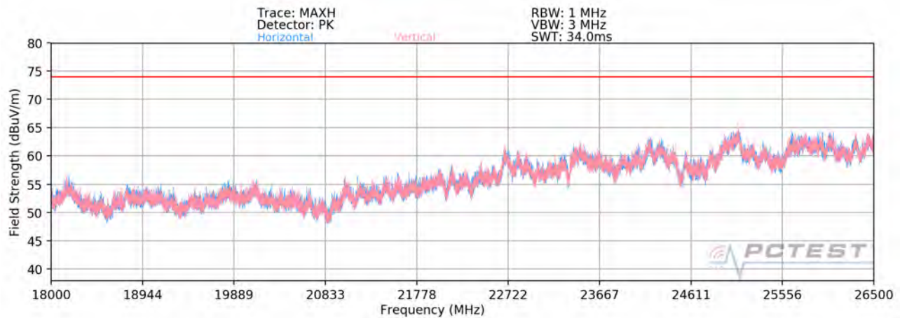
Plot 7-92. Radiated Spurious Plot above 18GHz SISO ANT2
