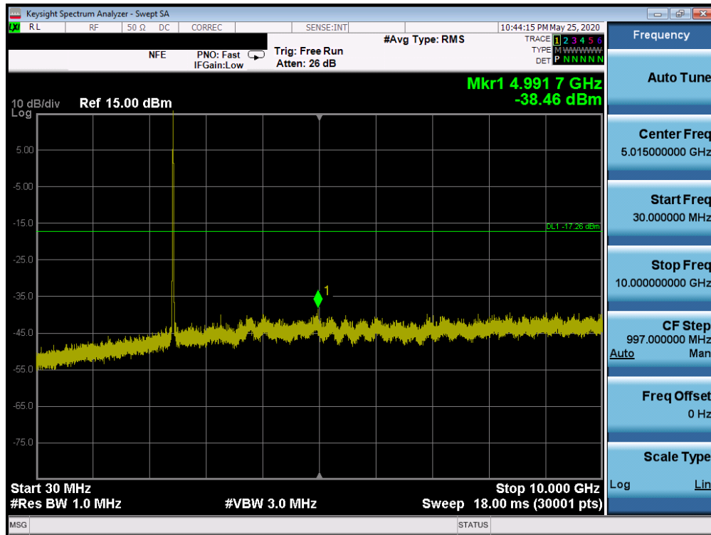
Plot 7-81. Conducted Spurious Plot SISO ANT2 (802.11b – Ch. 6)
