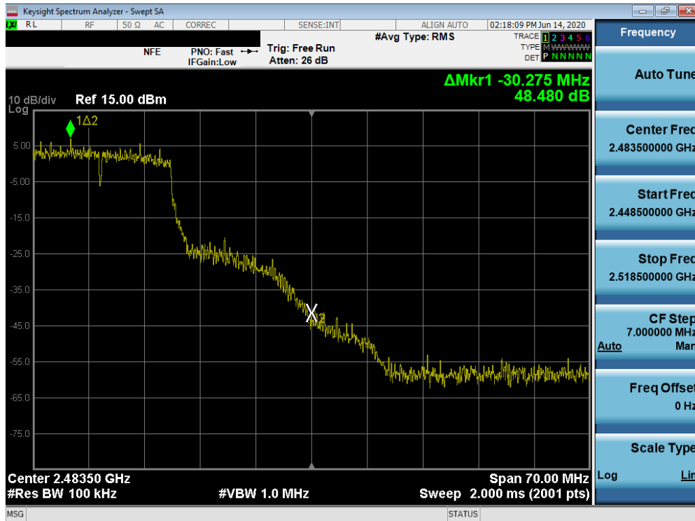
Plot 7-67. Band Edge Plot SISO ANT2 (802.11n (2.4GHz) - Ch. 10)
