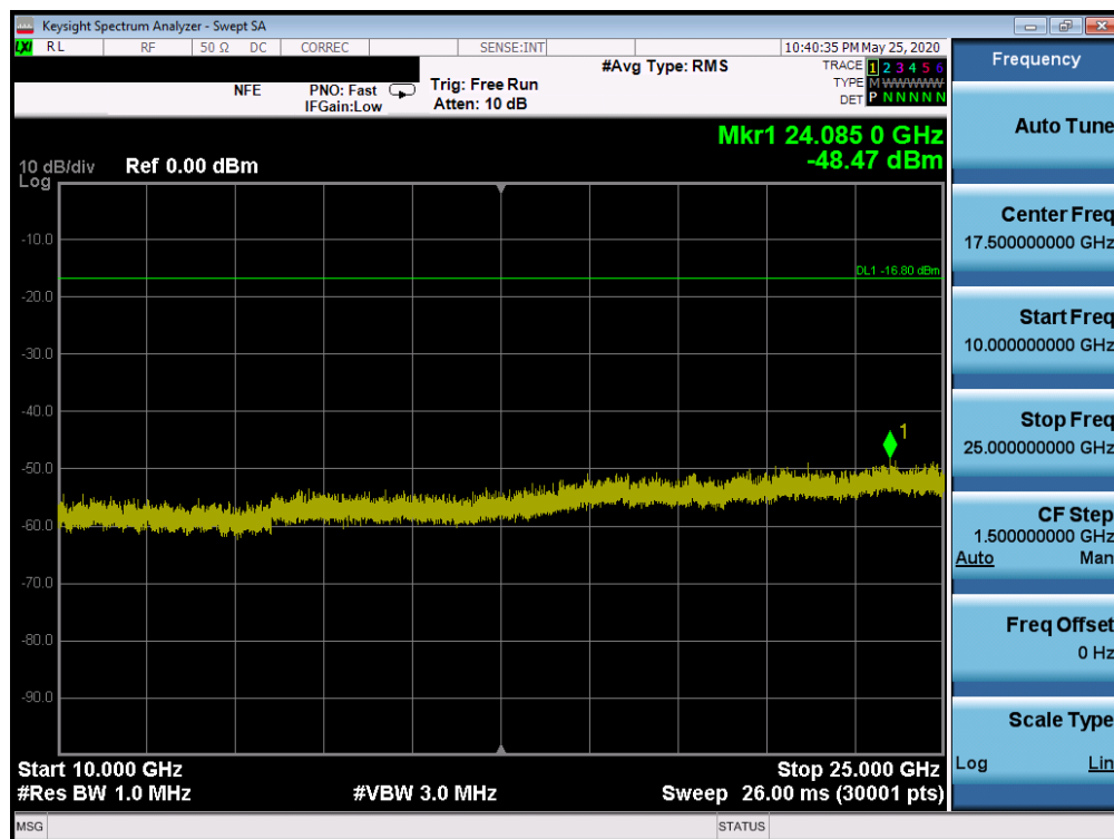
Plot 7-78. Conducted Spurious Plot SISO ANT1 (802.11b – Ch. 11)
