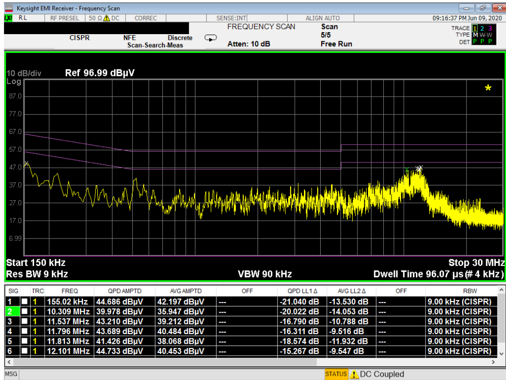
Plot 7-126. Line Conducted Plot with 802.11b (L1) with WCP
