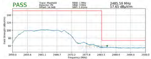
Plot 7-122. Radiated Restricted Band Edge Measurement MIMO with WCP (Peak)
