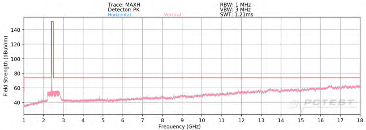
Plot 7-85. Radiated Spurious Plot above 1GHz SISO ANT1 (802.11b – Ch. 1)
