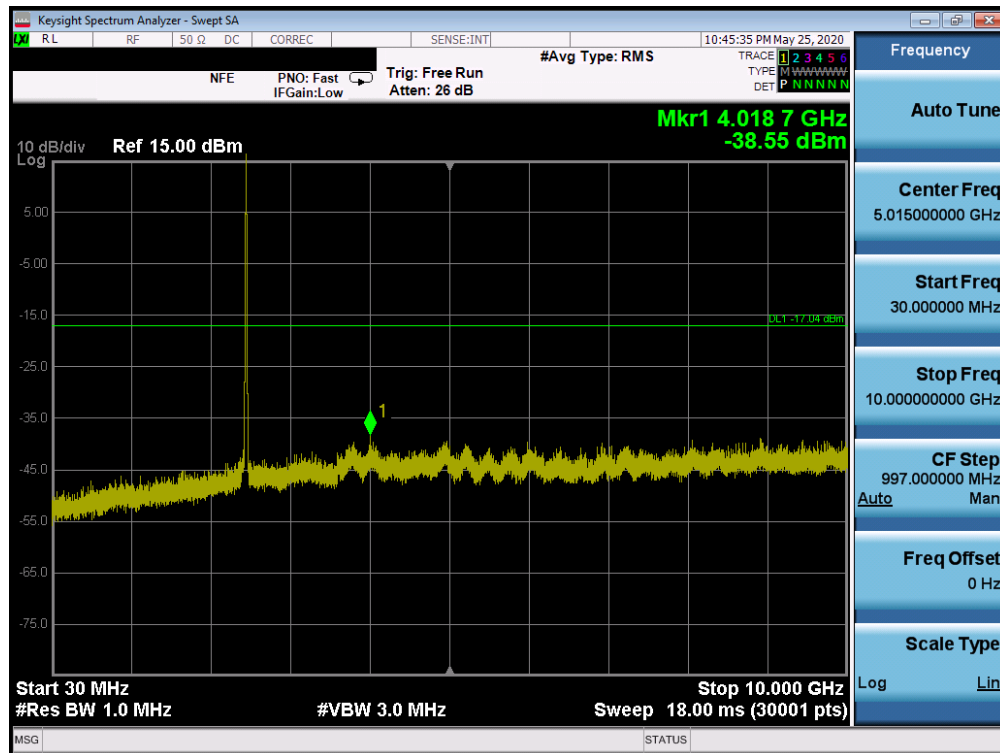
Plot 7-83. Conducted Spurious Plot SISO ANT2 (802.11b – Ch. 11)
