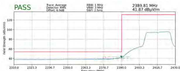
Plot 7-107. Radiated Restricted Lower Band Edge Measurement SISO ANT2 (Average)
