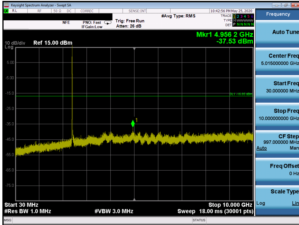
Plot 7-79. Conducted Spurious Plot SISO ANT2 (802.11b – Ch. 1)
