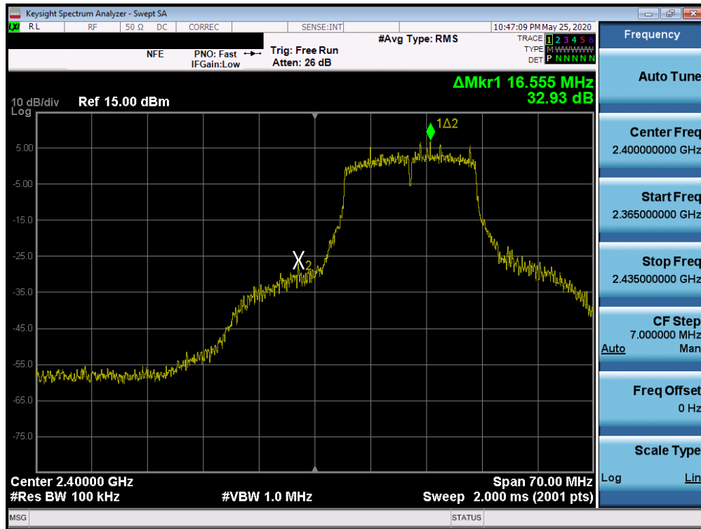
Plot 7-63. Band Edge Plot SISO ANT2 (802.11g- Ch. 1)
