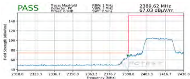
Plot 7-106. Radiated Restricted Lower Band Edge Measurement SISO ANT2 (Peak)
