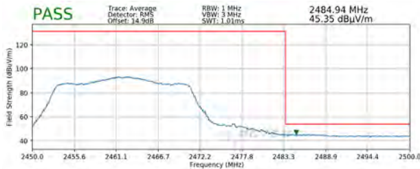
Plot 7-121. Radiated Restricted Band Edge Measurement MIMO with WCP (Average)
