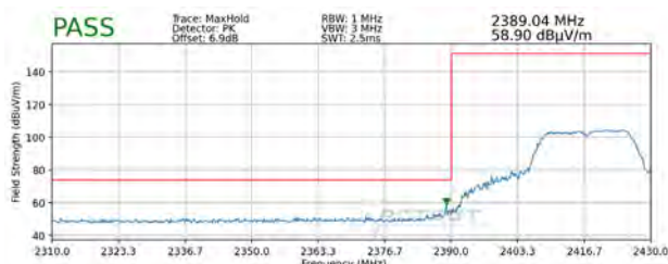
Plot 7-108. Radiated Restricted Lower Band Edge Measurement SISO ANT2 (Peak)
