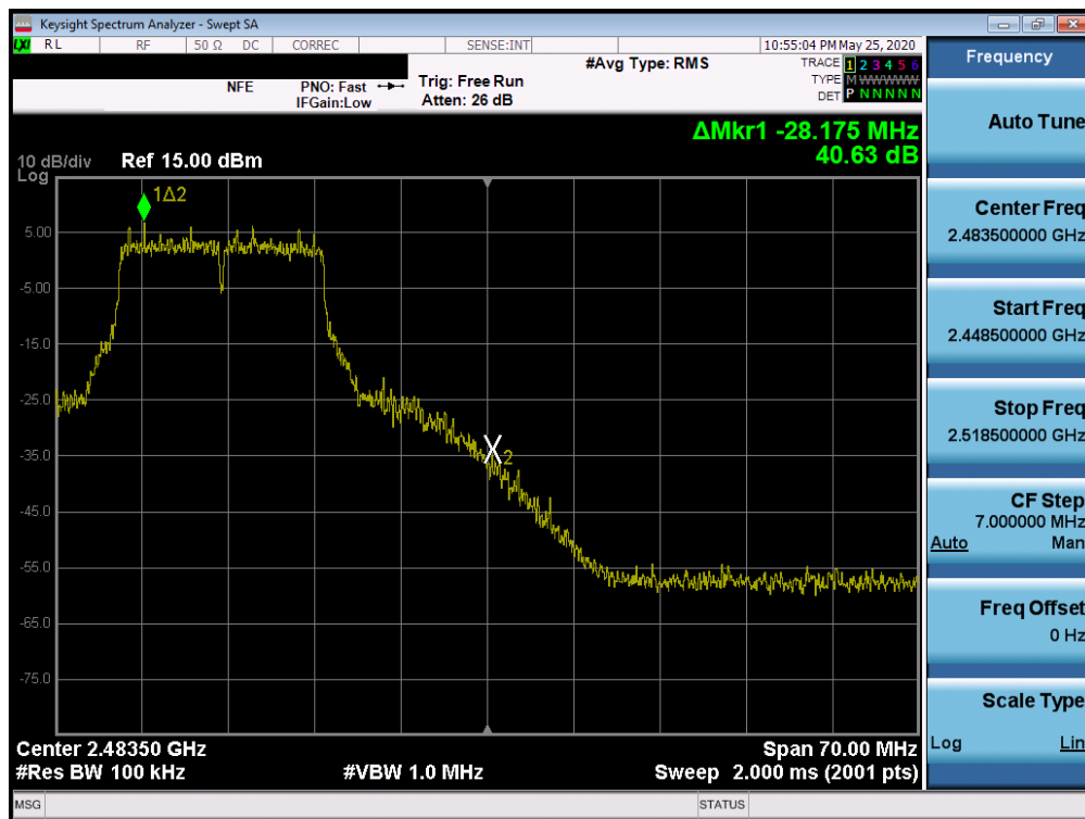
Plot 7-52. Band Edge Plot SISO ANT1 (802.11g - Ch. 11)
