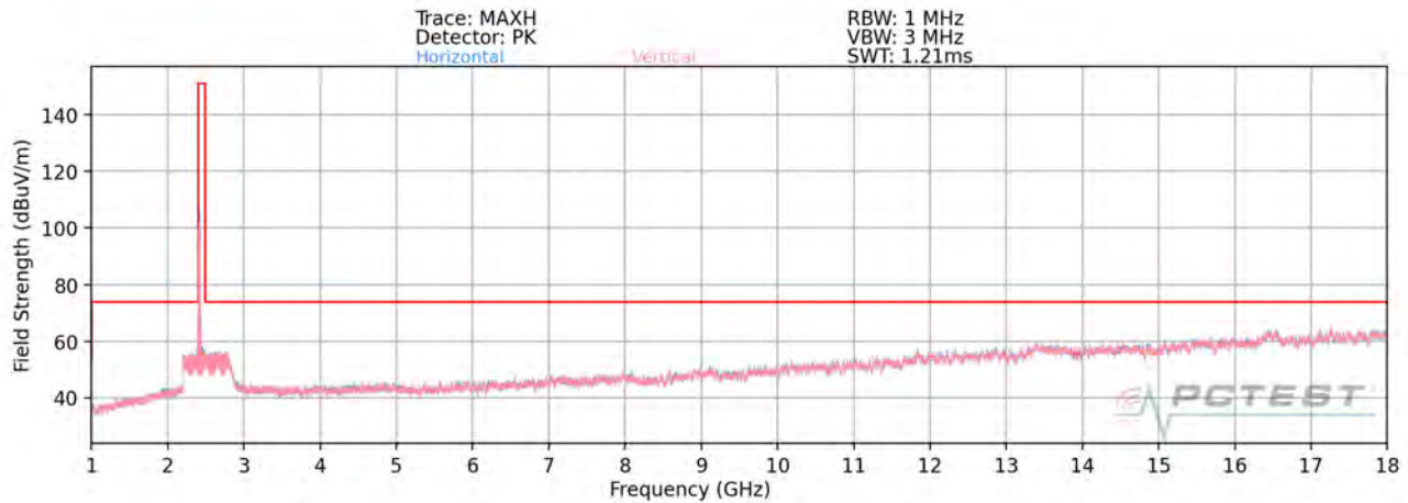
Plot 7-93. Radiated Spurious Plot above 1GHz MIMO/CDD (802.11g – Ch. 1)
