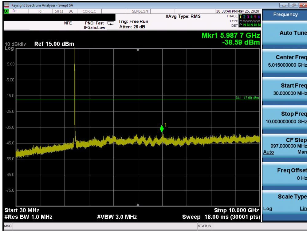
Plot 7-75. Conducted Spurious Plot SISO ANT1 (802.11b – Ch. 6)
