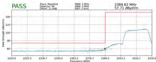
Plot 7-116. Radiated Restricted Lower Band Edge Measurement MIMO (Peak)
