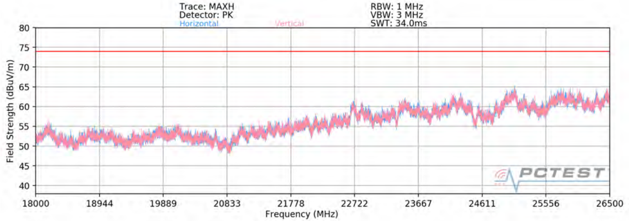
Plot 7-88. Radiated Spurious Plot above 18GHz SISO ANT1
