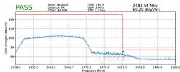
Plot 7-112. Radiated Restricted Upper Band Edge Measurement SISO ANT2 (Peak)
