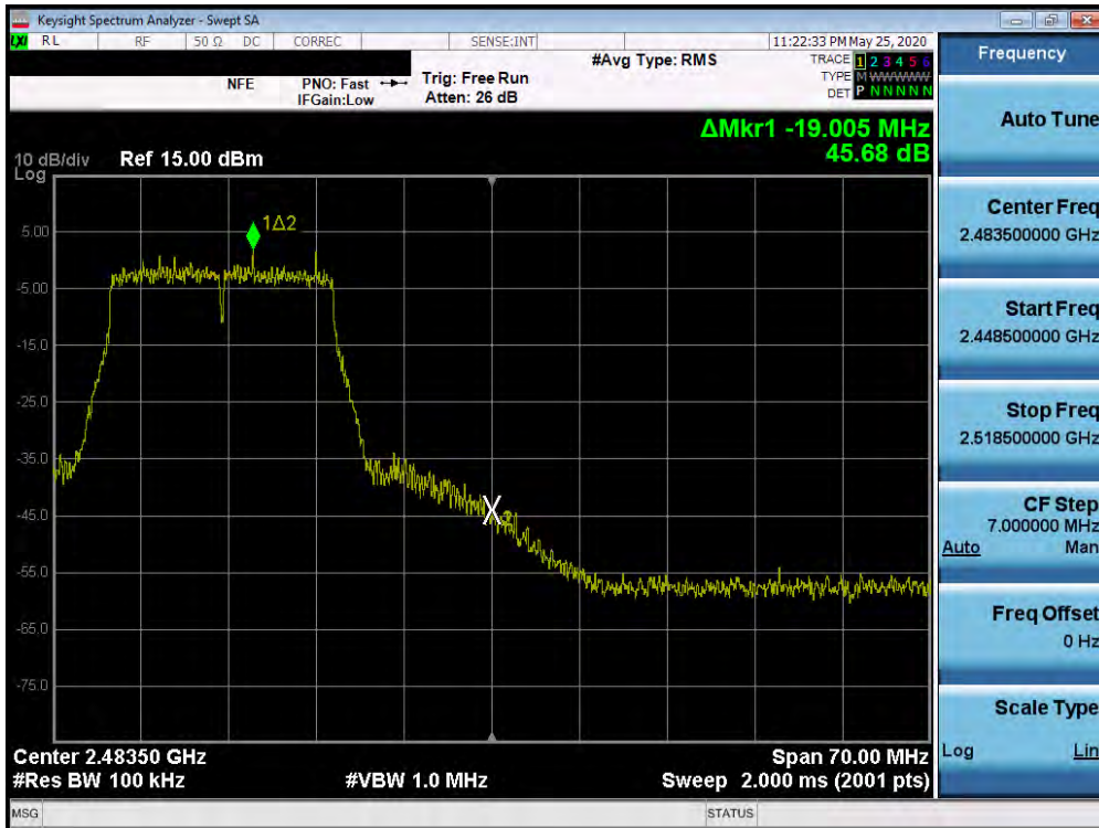
Plot 7-60. Band Edge Plot SISO ANT1 (802.11ax (2.4GHz) - Ch. 11)
