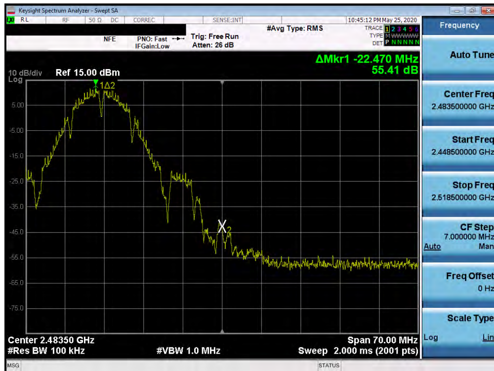
Plot 7-62. Band Edge Plot SISO ANT2 (802.11b - Ch. 11)
