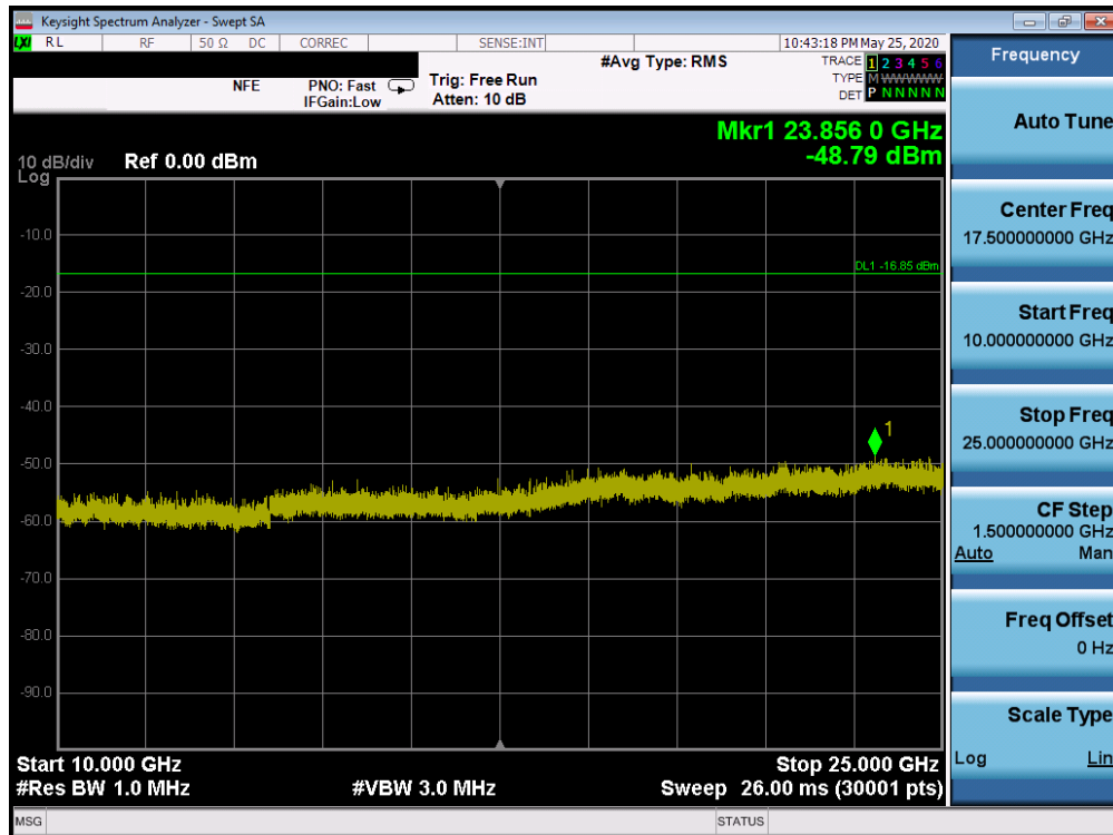
Plot 7-80. Conducted Spurious Plot SISO ANT2 (802.11b – Ch. 1)
