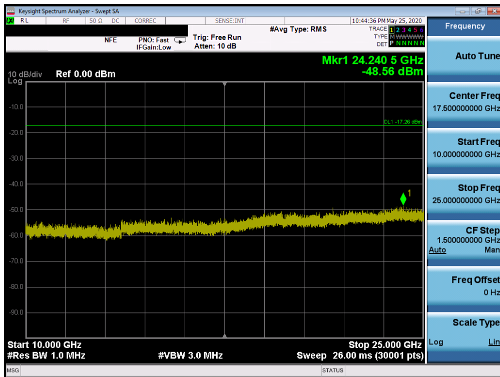
Plot 7-82. Conducted Spurious Plot SISO ANT2 (802.11b – Ch. 6)
