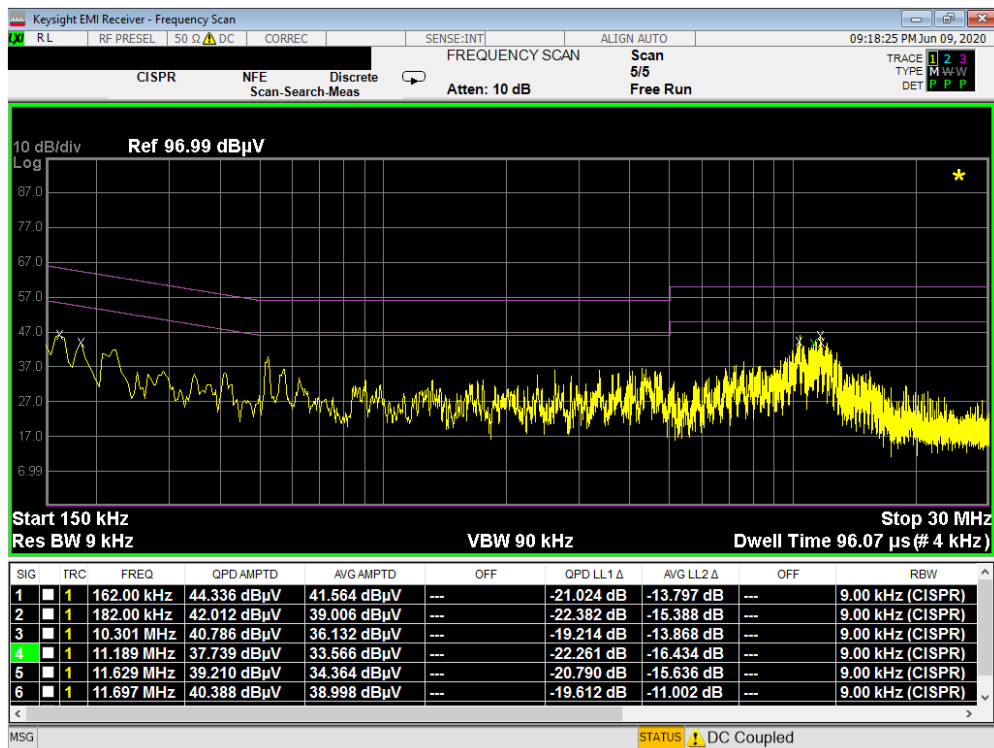
Plot 7-127. Line Conducted Plot with 802.11b (N) with WCP
