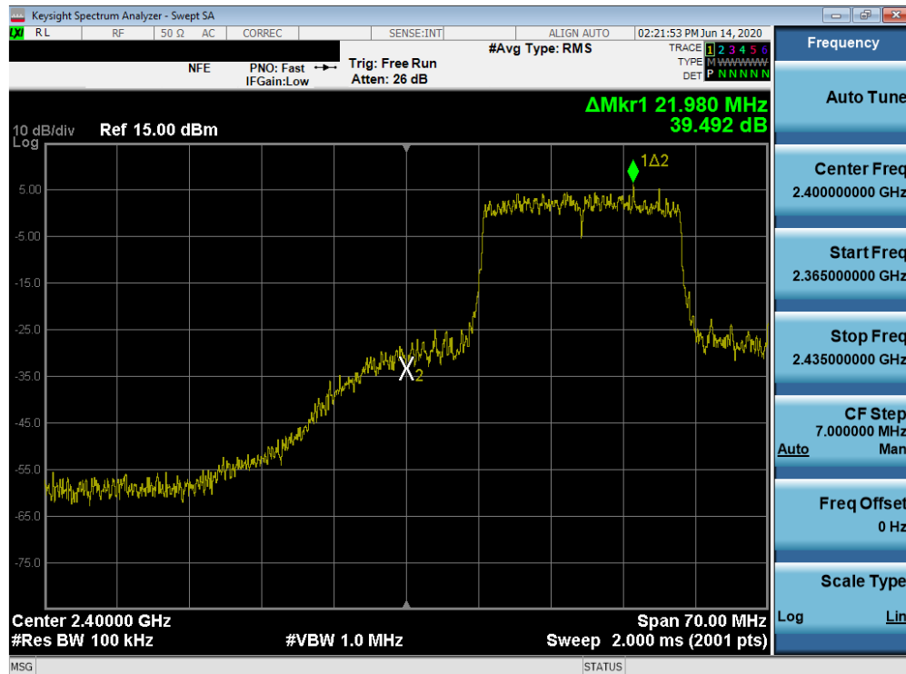
Plot 7-58. Band Edge Plot SISO ANT1 (802.11ax (2.4GHz) – Ch. 2)
