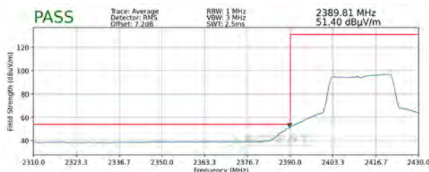
Plot 7-97. Radiated Restricted Lower Band Edge Measurement SISO ANT1 (Average)
