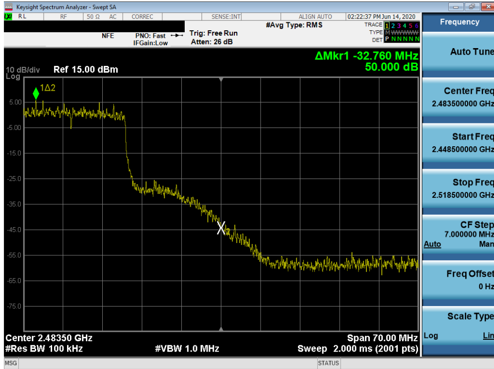
Plot 7-59. Band Edge Plot SISO ANT1 (802.11ax (2.4GHz) - Ch. 10)
