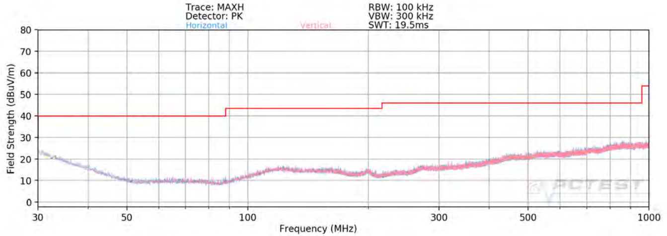
Plot 7-123. Radiated Spurious Plot below 1GHz
