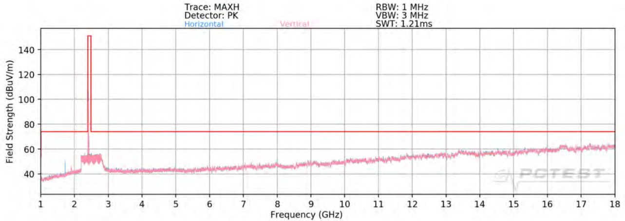
Plot 7-89. Radiated Spurious Plot above 1GHz SISO ANT2 (802.11b – Ch. 1)
