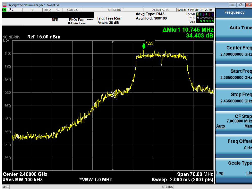
Plot 7-54. Band Edge Plot SISO ANT1 (802.11n (2.4GHz) – Ch. 2)
