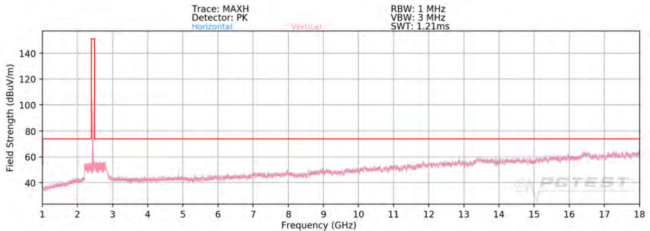
Plot 7-86. Radiated Spurious Plot above 1GHz SISO ANT1 (802.11b – Ch. 6)
