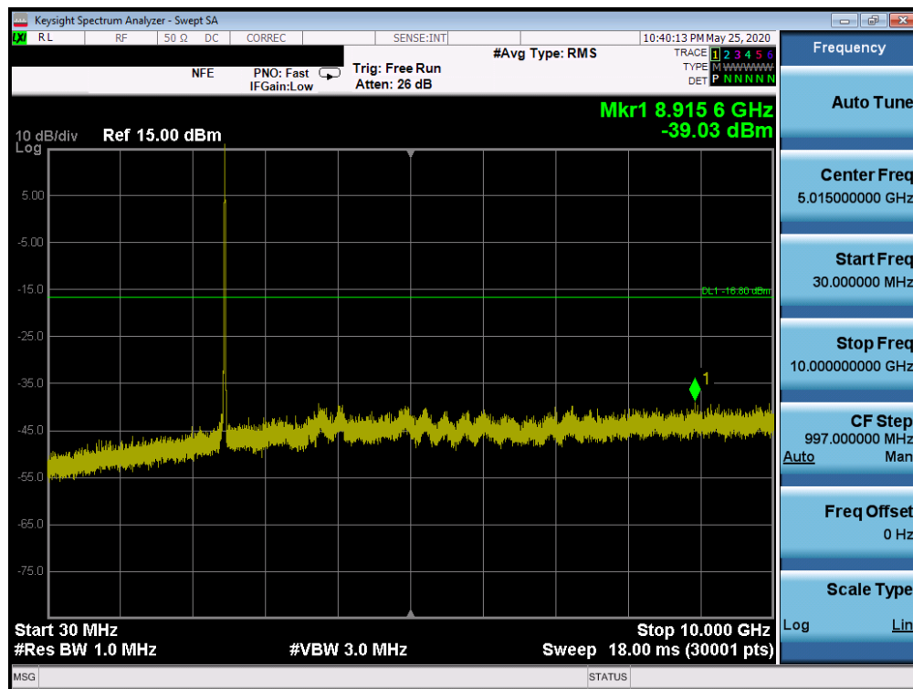
Plot 7-77. Conducted Spurious Plot SISO ANT1 (802.11b – Ch. 11)
