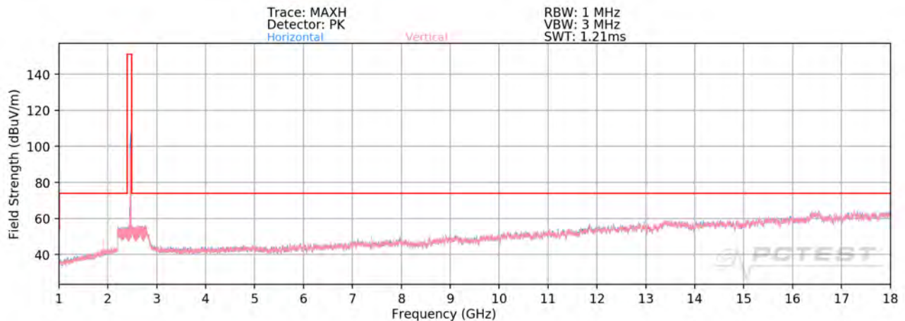
Plot 7-91. Radiated Spurious Plot above 1GHz SISO ANT2 (802.11b – Ch. 11)
