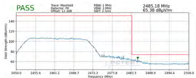
Plot 7-120. Radiated Restricted Upper Band Edge Measurement MIMO (Peak)
