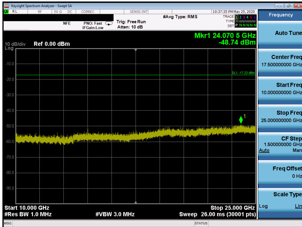
Plot 7-74. Conducted Spurious Plot SISO ANT1 (802.11b – Ch. 1)
