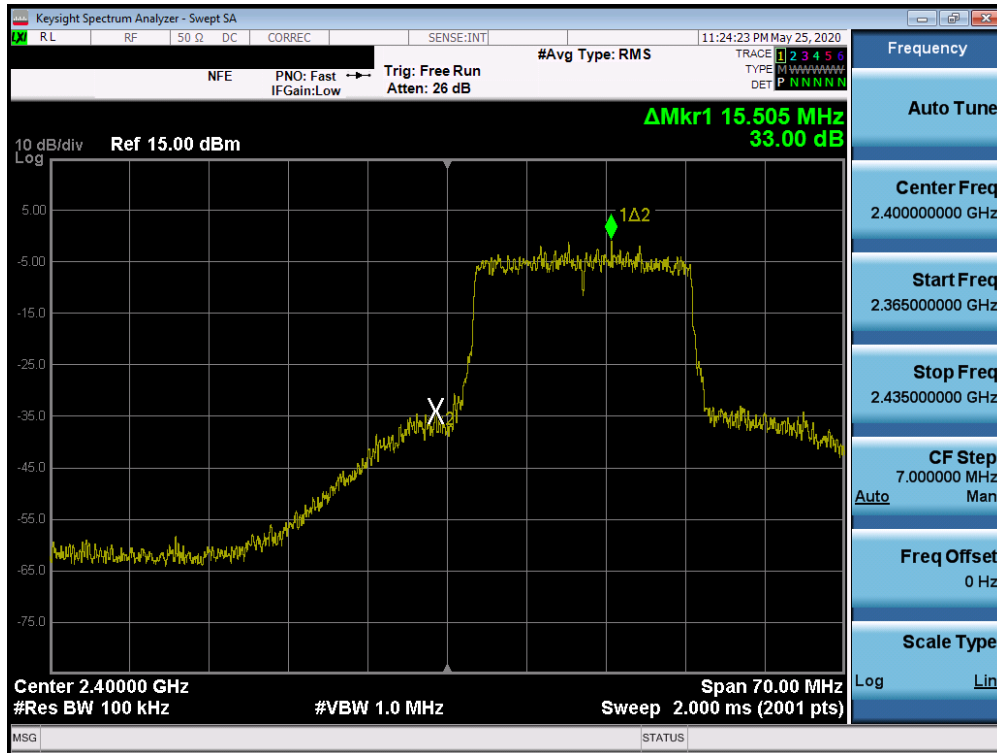
Plot 7-57. Band Edge Plot SISO ANT1 (802.11ax (2.4GHz) – Ch. 1)
