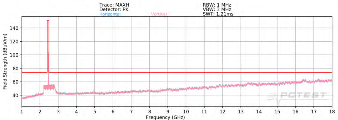
Plot 7-87. Radiated Spurious Plot above 1GHz SISO ANT1 (802.11b – Ch. 11)
