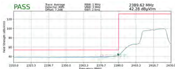
Plot 7-99. Radiated Restricted Lower Band Edge Measurement SISO ANT1 (Average)
