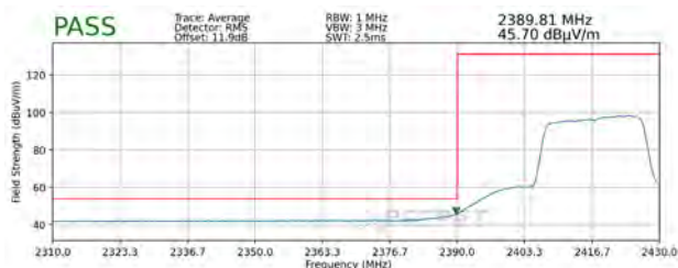
Plot 7-115. Radiated Restricted Lower Band Edge Measurement MIMO (Average)
