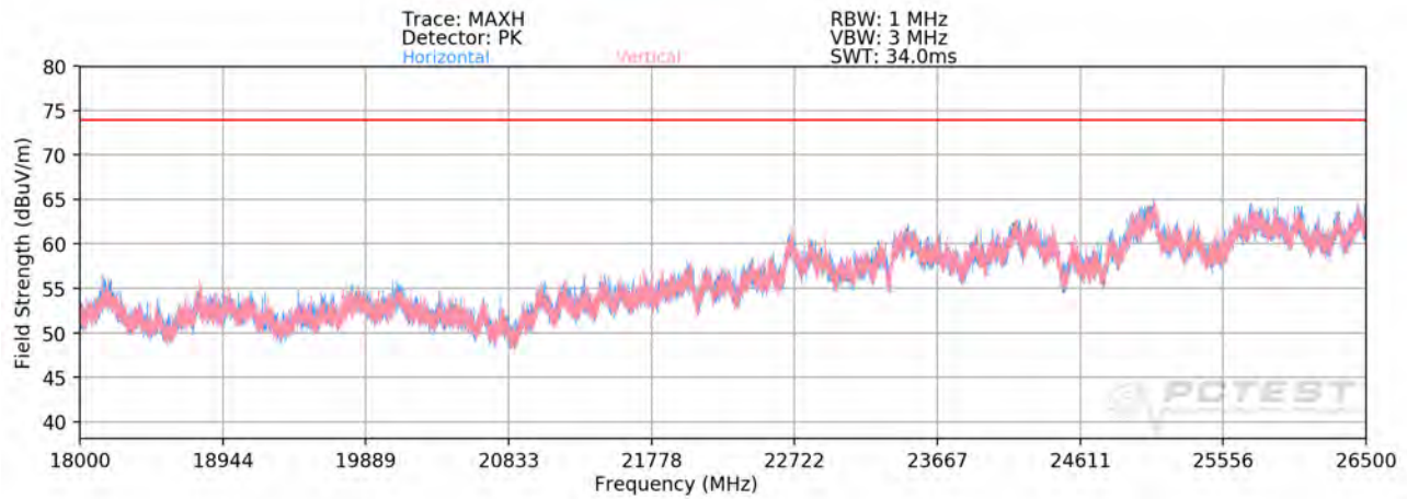
Plot 7-96. Radiated Spurious Plot above 18GHz MIMO/CDD
