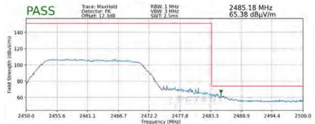
Plot 7-120. Radiated Restricted Upper Band Edge Measurement MIMO (Peak)
