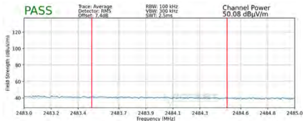
Plot 7-103. Radiated Restricted Upper Band Edge Measurement SISO ANT1 (Average)
