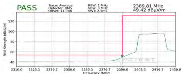
Plot 7-113. Radiated Restricted Lower Band Edge Measurement MIMO (Average)
