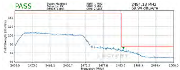
Plot 7-104. Radiated Restricted Upper Band Edge Measurement SISO ANT1 (Peak)
