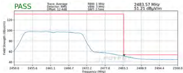
Plot 7-119. Radiated Restricted Upper Band Edge Measurement MIMO (Average)
