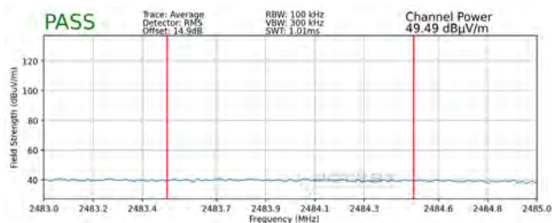
Plot 7-111. Radiated Restricted Upper Band Edge Measurement SISO ANT2 (Average)
