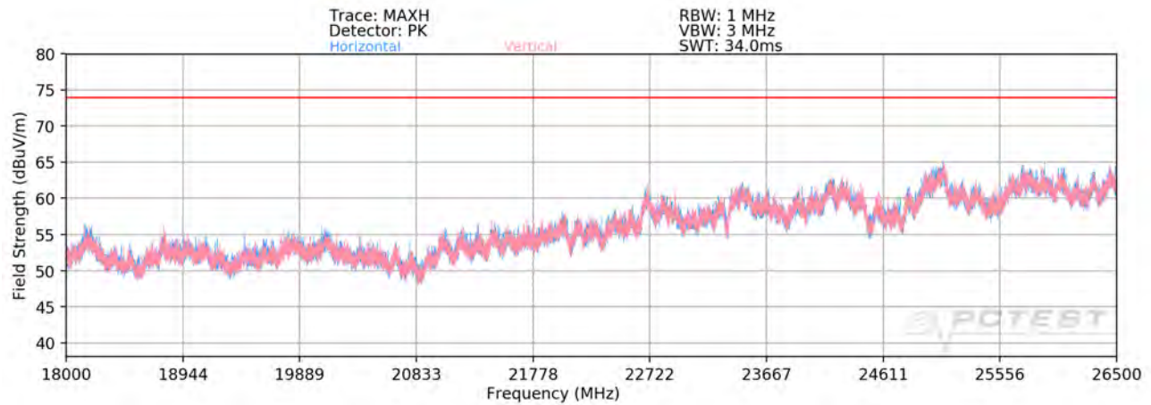
Plot 7-96. Radiated Spurious Plot above 18GHz MIMO/CDD
