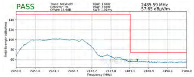
Plot 7-122. Radiated Restricted Band Edge Measurement MIMO with WCP (Peak)
