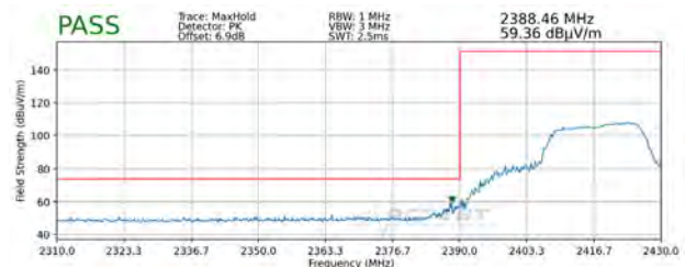
Plot 7-100. Radiated Restricted Lower Band Edge Measurement SISO ANT1 (Peak)
