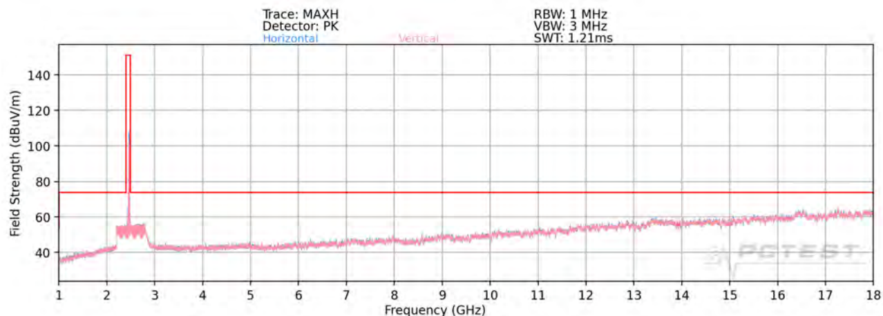
Plot 7-95. Radiated Spurious Plot above 1GHz MIMO/CDD (802.11g – Ch. 11)
