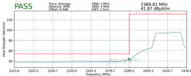
Plot 7-107. Radiated Restricted Lower Band Edge Measurement SISO ANT2 (Average)
