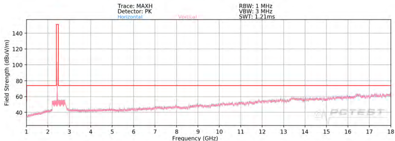
Plot 7-94. Radiated Spurious Plot above 1GHz MIMO/CDD (802.11g – Ch. 6)
