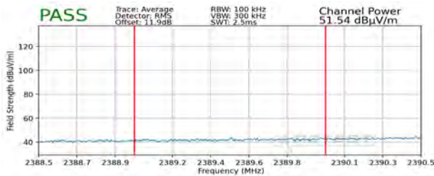
Plot 7-105. Radiated Restricted Lower Band Edge Measurement SISO ANT2 (Average)
