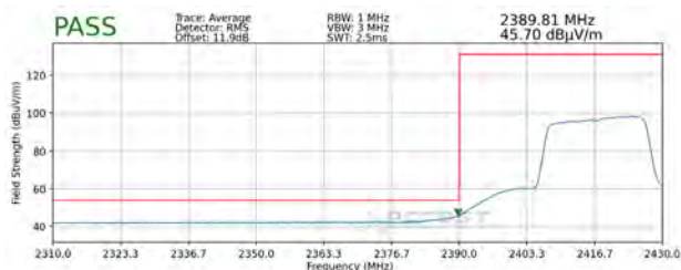
Plot 7-115. Radiated Restricted Lower Band Edge Measurement MIMO (Average)
