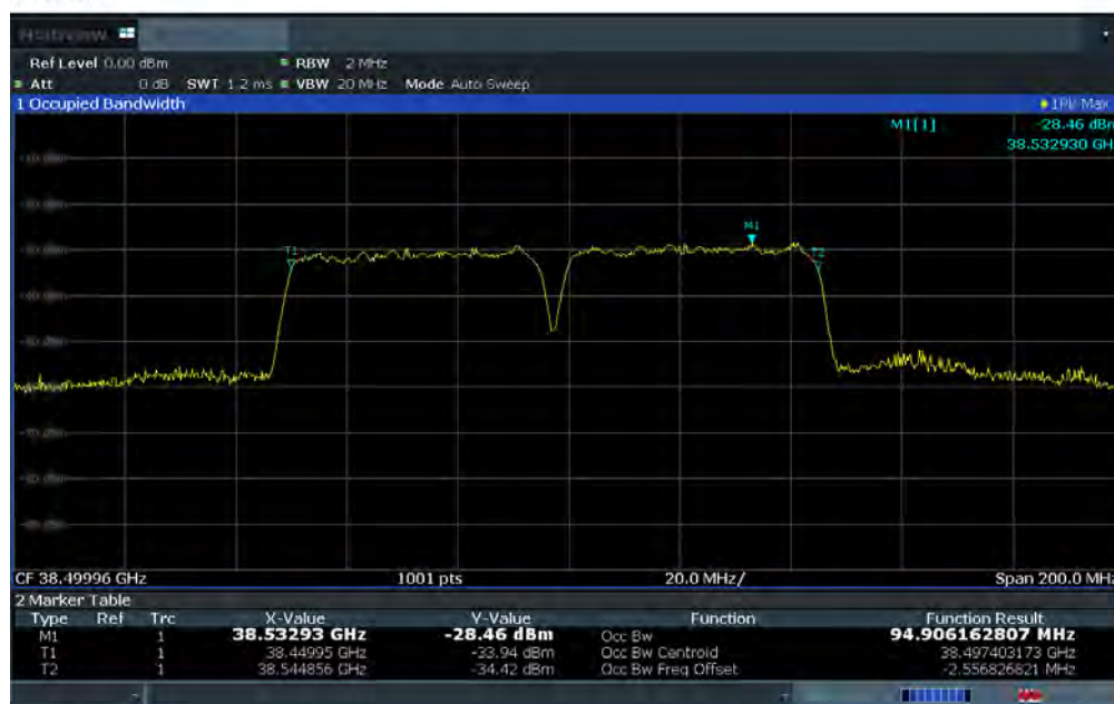
Plot 7-21. Ant 2 Occupied Bandwidth Plot (50MHz-2CC – QPSK – Mid Channel)
