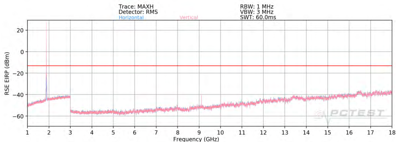
Plot 7-48. Ant 1-n260 Radiated Spurious Plot (1CC QPSK Mid Channel MIMO – ENDC Anchor Band 2)
