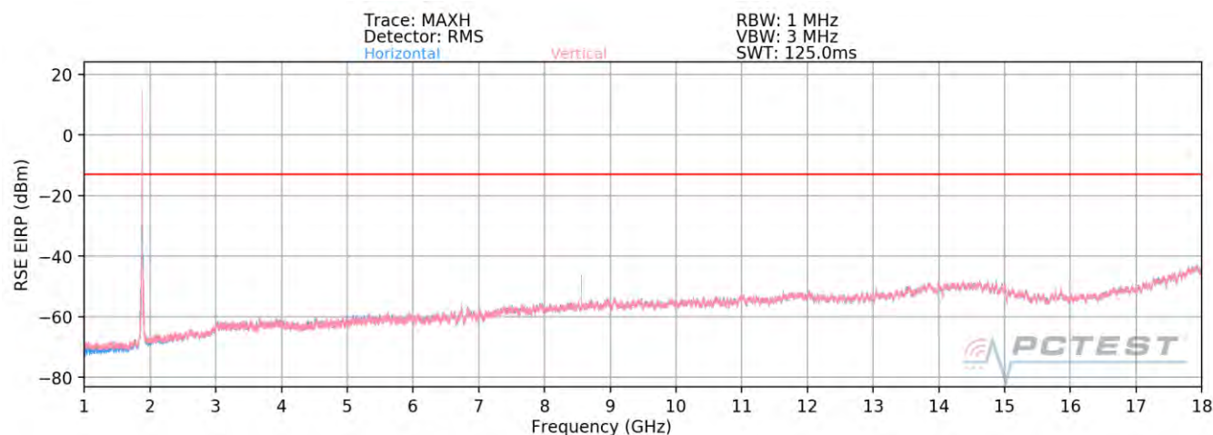
Plot 7-41. Ant 2-n261 Radiated Spurious Plot (1CC QPSK Mid Channel V Beam – ENDC Anchor Band 2)
