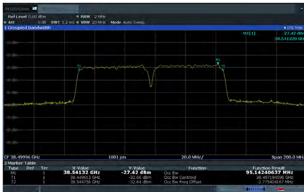
Plot 7-24. Ant 2 Occupied Bandwidth Plot (50MHz-2CC – pi/2-BPSK – Mid Channel)
