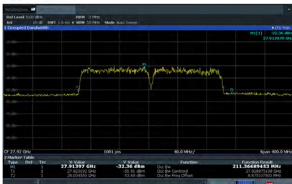
Plot 7-15. Ant 2 Occupied Bandwidth Plot (100MHz-2CC – 64QAM – Mid Channel)
