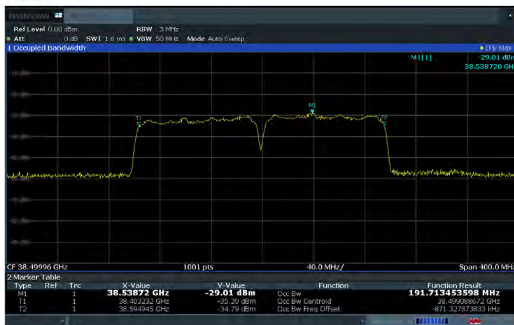
Plot 7-29. Ant 2 Occupied Bandwidth Plot (100MHz-2CC – QPSK – Mid Channel)
