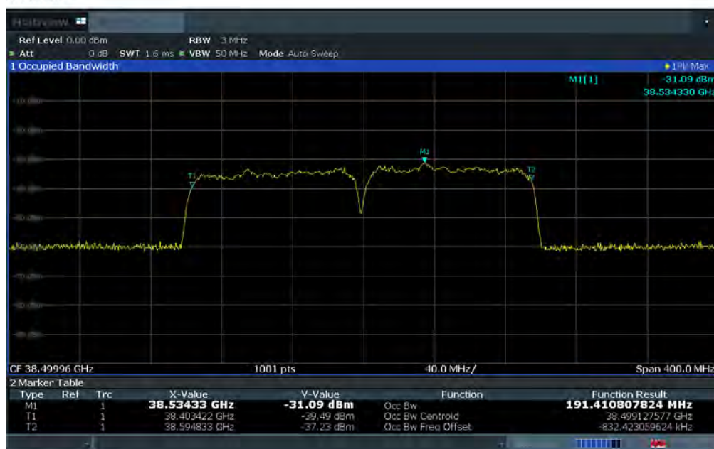
Plot 7-31. Ant 2 Occupied Bandwidth Plot (100MHz-2CC – 64QAM – Mid Channel)
