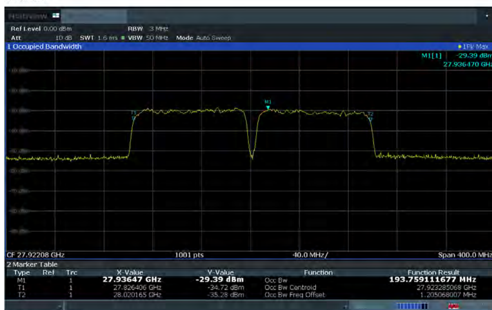
Plot 7-16. Ant 2 Occupied Bandwidth Plot (100MHz-2CC – pi/2-BPSK – Mid Channel)
