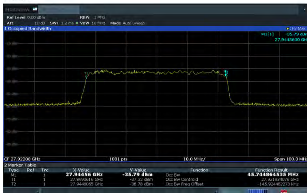
Plot 7-3. Ant 2 Occupied Bandwidth Plot (50MHz-1CC – 64QAM – Mid Channel)
