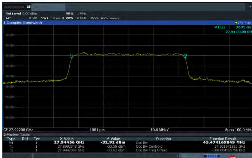
Plot 7-1. Ant 2 Occupied Bandwidth Plot (50MHz-1CC – QPSK – Mid Channel)
