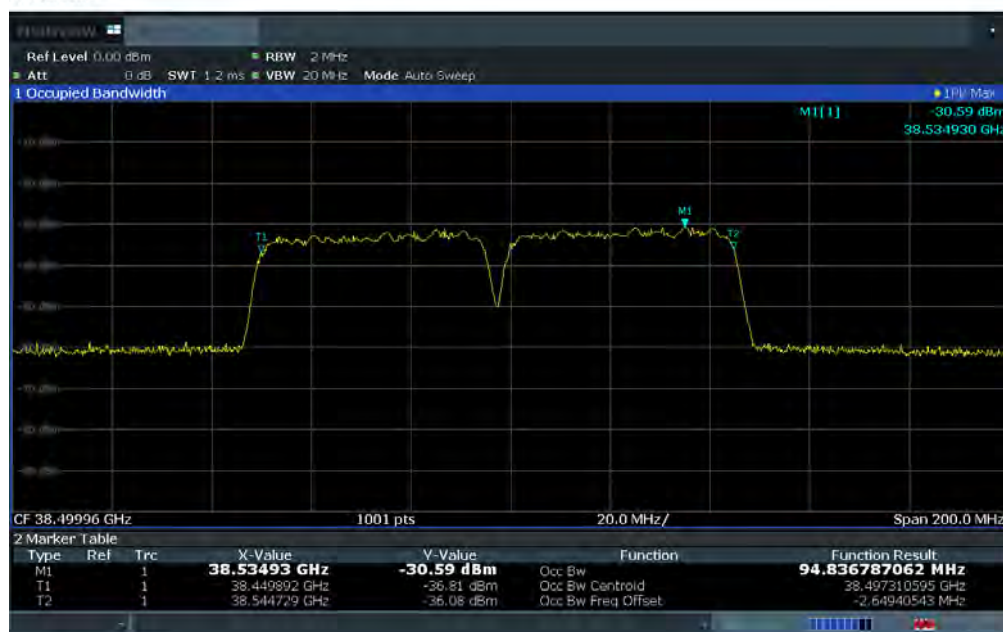
Plot 7-23. Ant 2 Occupied Bandwidth Plot (50MHz-2CC – 64QAM – Mid Channel)
