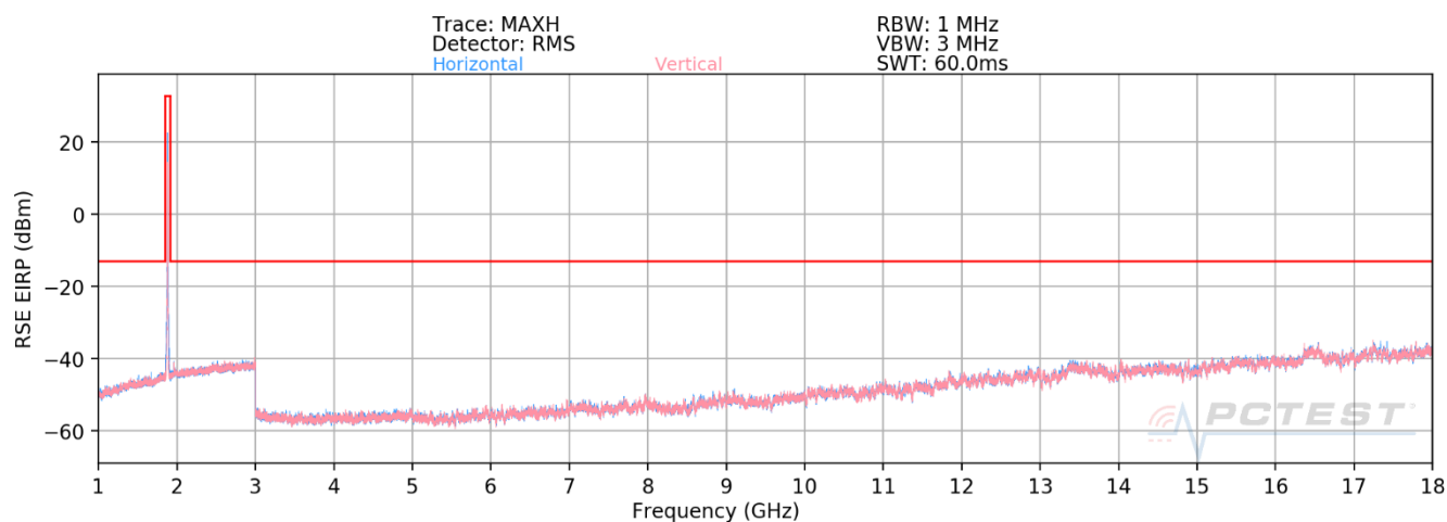
Plot 7-96. Radiated Spurious Plot above 1GHz (PCS WCDMA Mode)
