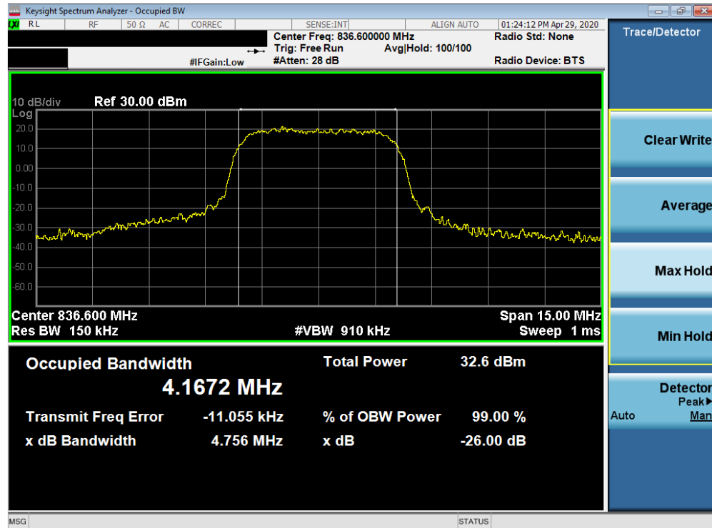
Plot 7-6. Occupied Bandwidth Plot (Cellular WCDMA Mode)
