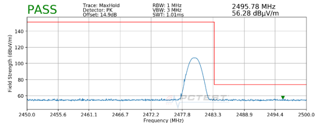
Plot 7-49. Radiated Restricted Upper Band Edge Measurement with WCP (Peak)
