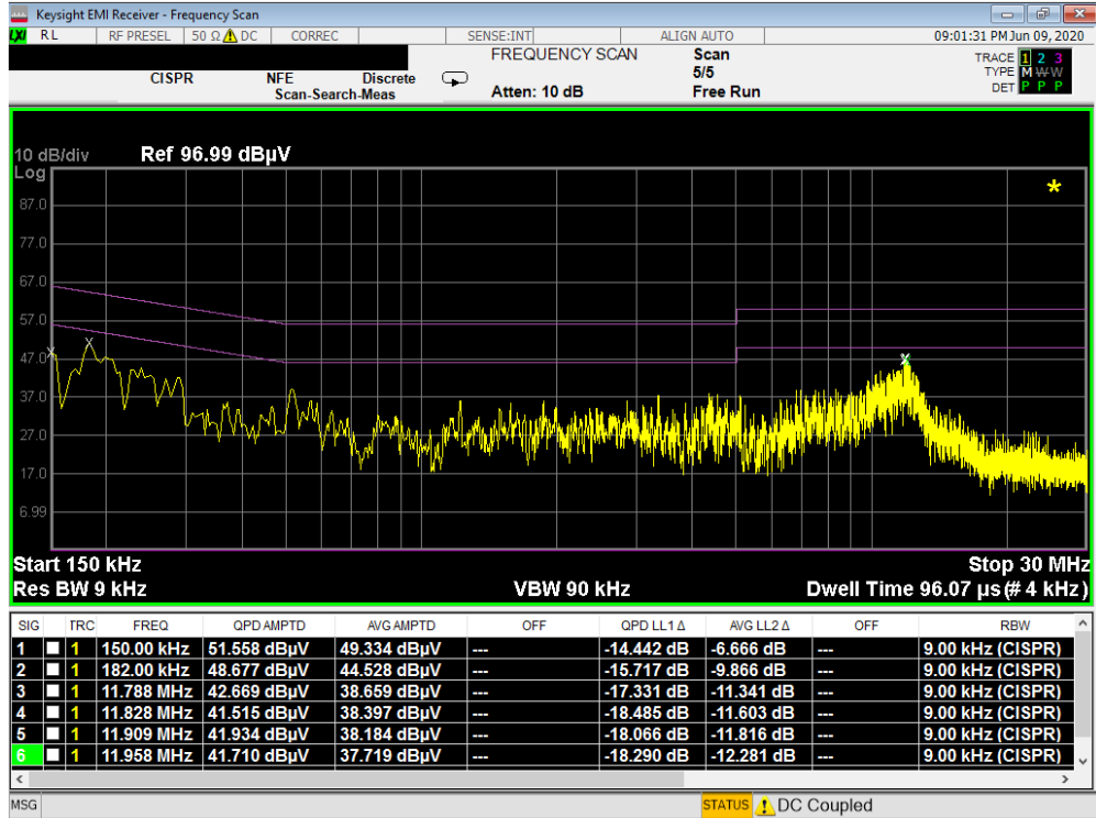
Plot 7-53. Line-Conducted Test Plot (L1) with WCP
