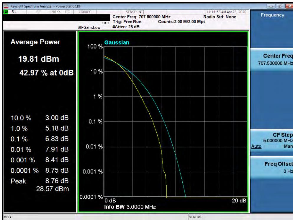
Plot 7-512. PAR Plot (Band 12 - 3.0MHz 256-QAM - Full RB Configuration)
