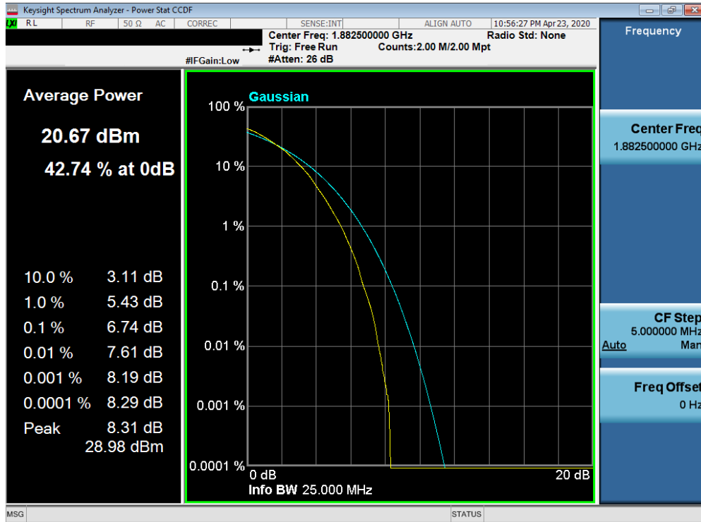
Plot 7-563. PAR Plot (Band 25/2 - 15.0MHz 64-QAM - Full RB Configuration)
