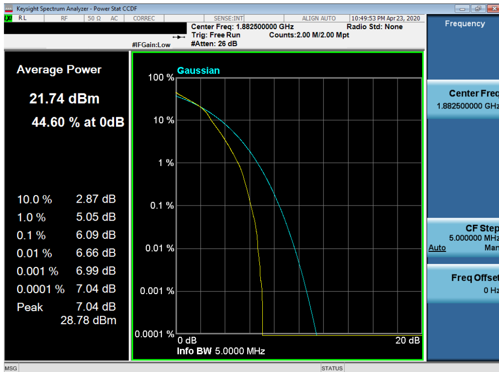
Plot 7-554. PAR Plot (Band 25/2 - 5.0MHz 16-QAM - Full RB Configuration)
