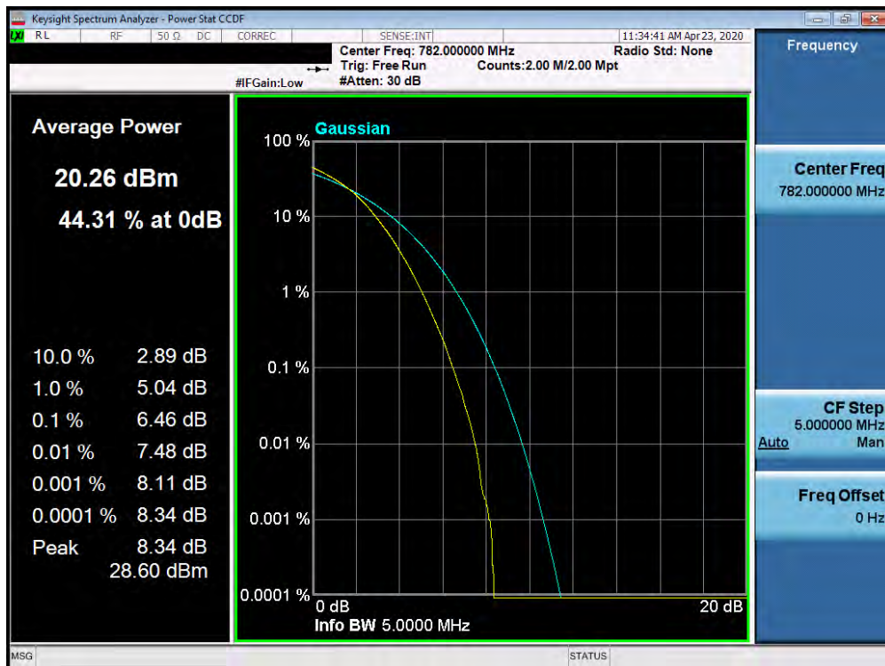
Plot 7-524. PAR Plot (Band 13 - 5.0MHz 256-QAM - Full RB Configuration)
