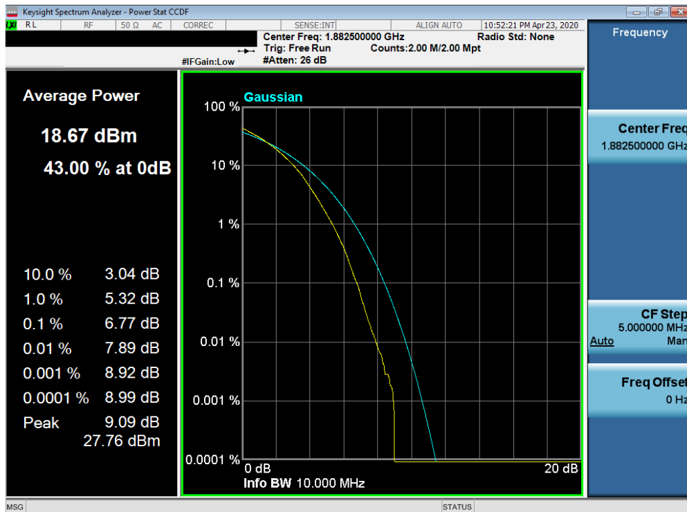
Plot 7-560. PAR Plot (Band 25/2 - 10.0MHz 256-QAM - Full RB Configuration)
