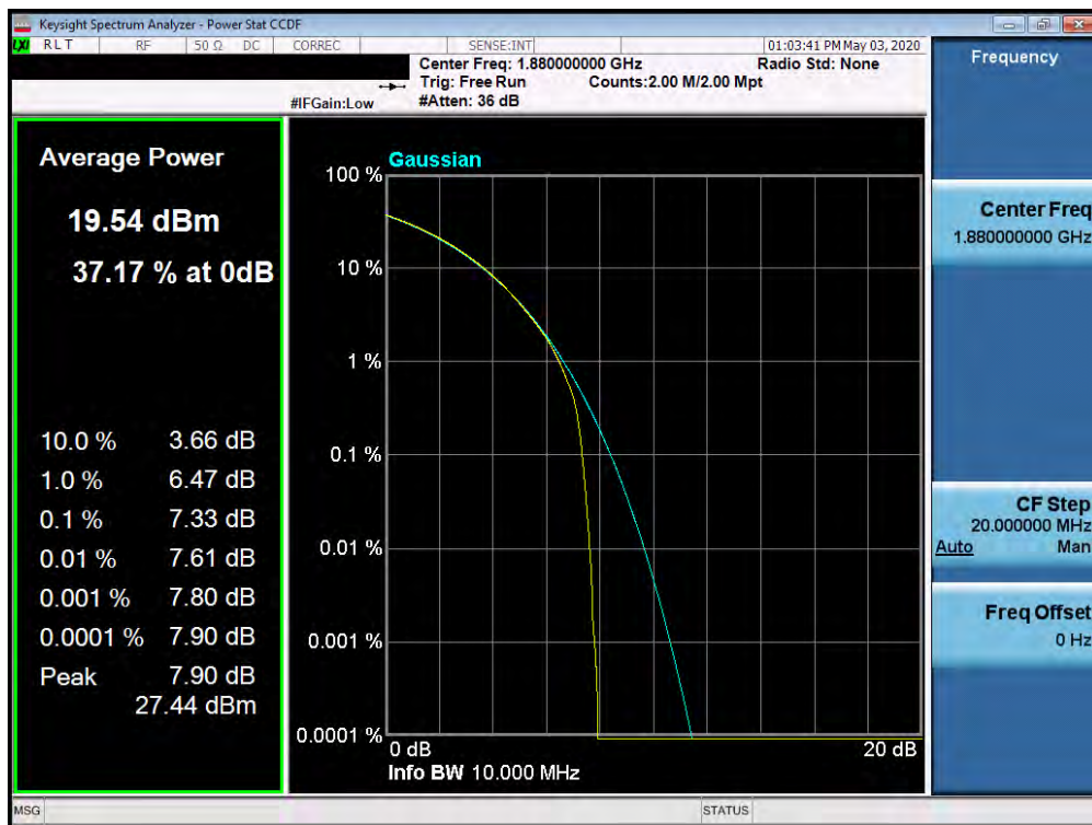
Plot 7-574. PAR Plot (Band n25/2 - 10.0MHz 16-QAM - Full RB Configuration)
