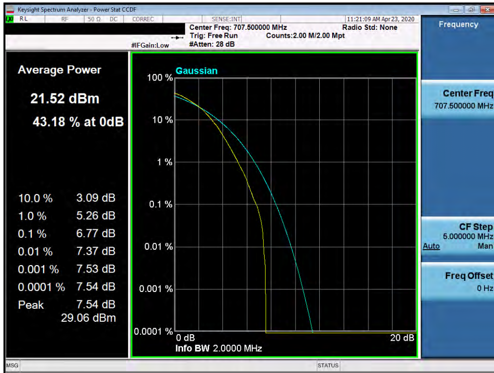
Plot 7-507. PAR Plot (Band 12 - 1.4MHz 64-QAM - Full RB Configuration)
