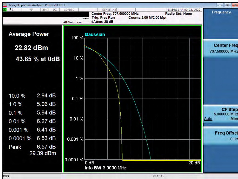
Plot 7-510. PAR Plot (Band 12 - 3.0MHz 16-QAM - Full RB Configuration)
