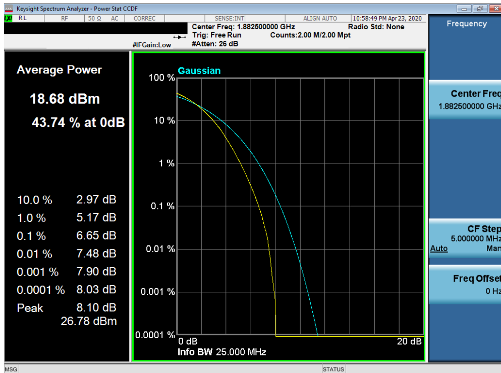
Plot 7-568. PAR Plot (Band 25/2 - 20.0MHz 256-QAM - Full RB Configuration)
