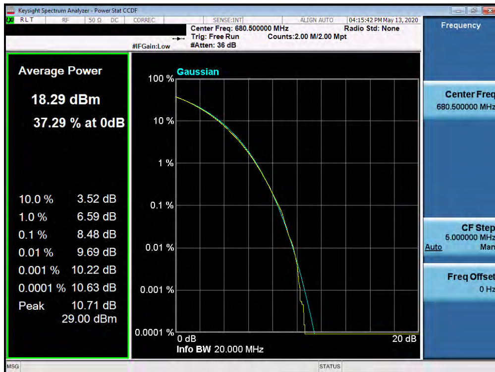
Plot 7-504. PAR Plot (Band n71 - 20.0MHz 256-QAM - Full RB Configuration)
