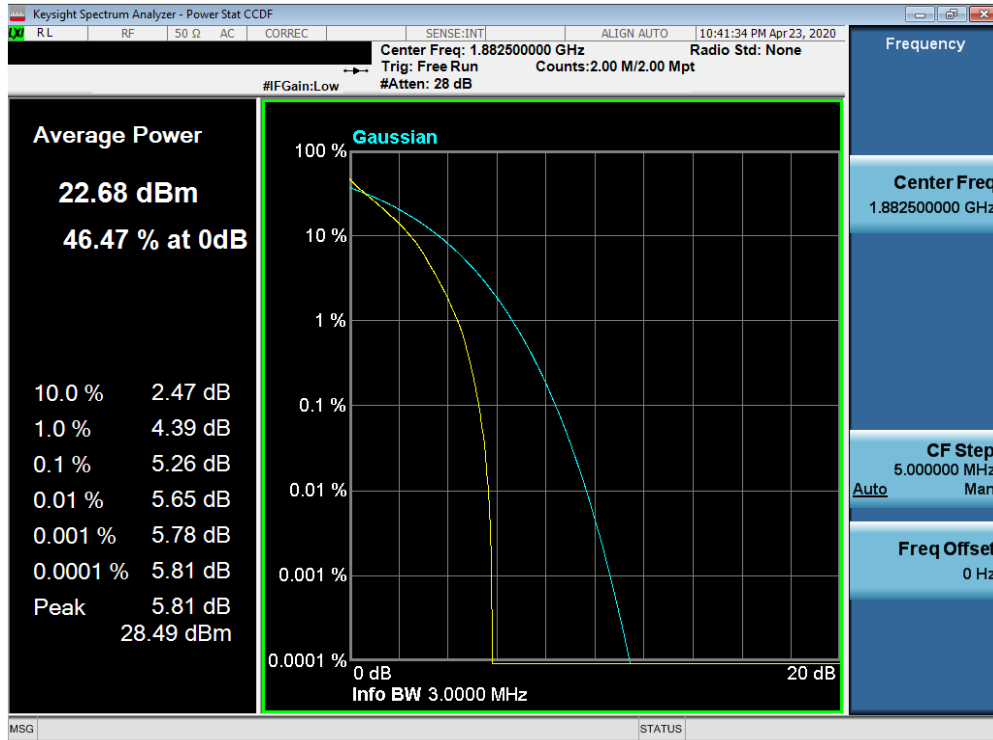
Plot 7-549. PAR Plot (Band 25/2 - 3.0MHz QPSK - Full RB Configuration)
