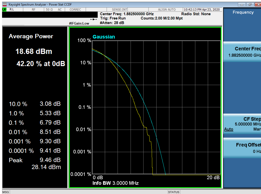
Plot 7-552. PAR Plot (Band 25/2 - 3.0MHz 256-QAM - Full RB Configuration)
