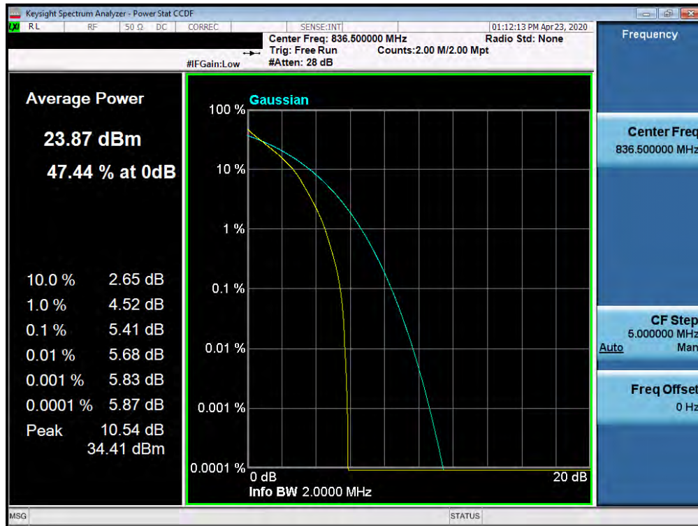
Plot 7-529. PAR Plot (Band 5 - 1.4MHz QPSK - Full RB Configuration)
