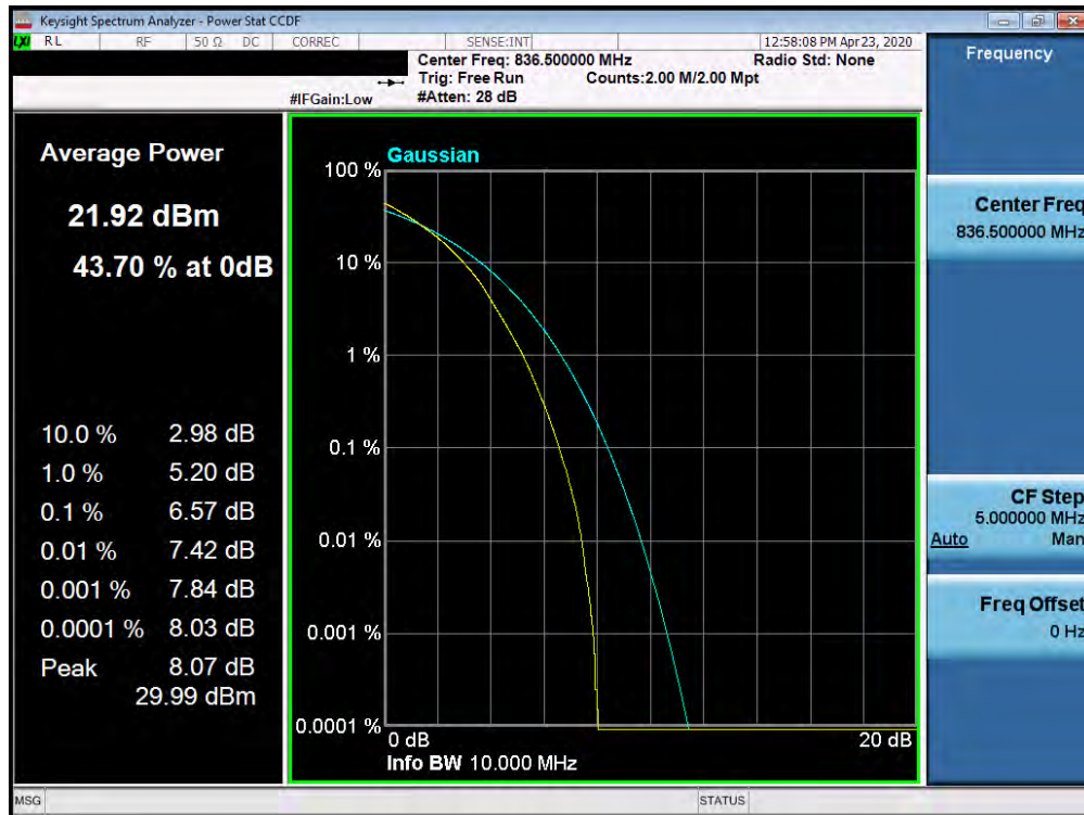
Plot 7-543. PAR Plot (Band 5 - 10.0MHz 64-QAM - Full RB Configuration)
