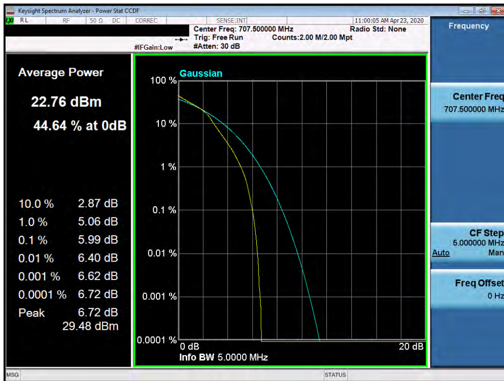
Plot 7-514. PAR Plot (Band 12 - 5.0MHz 16-QAM - Full RB Configuration)
