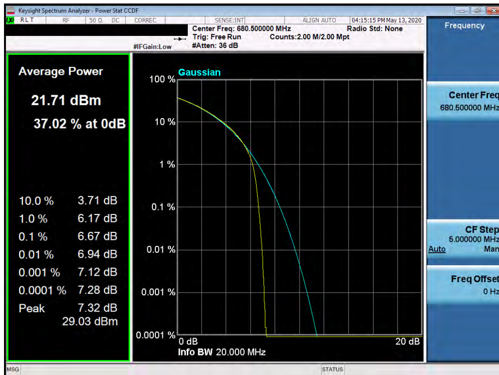
Plot 7-502. PAR Plot (Band n71 - 20.0MHz 16-QAM - Full RB Configuration)
