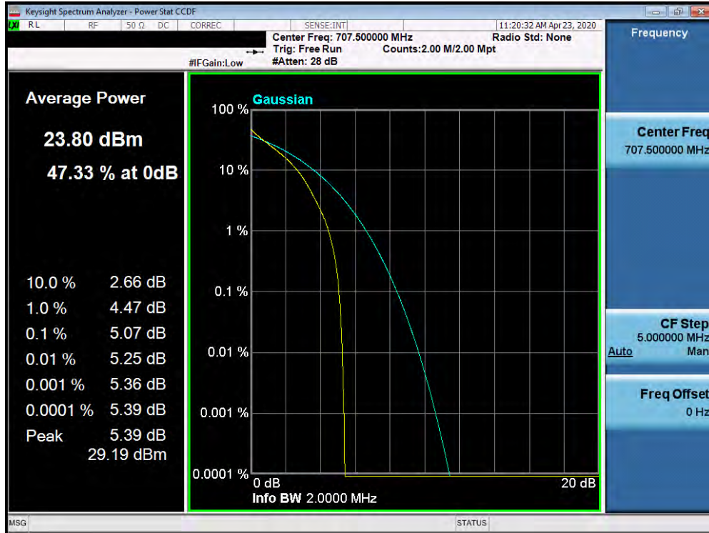
Plot 7-505. PAR Plot (Band 12 - 1.4MHz QPSK - Full RB Configuration)
