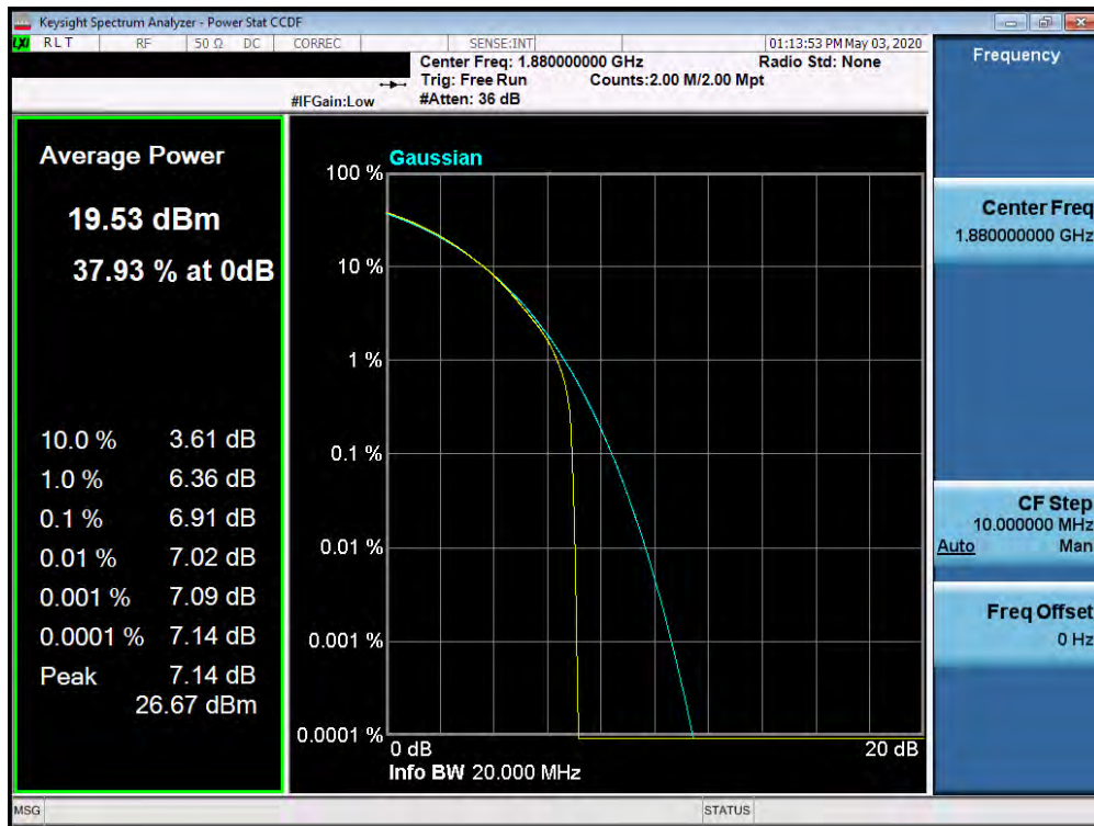
Plot 7-570. PAR Plot (Band n25/2 - 5.0MHz 16-QAM - Full RB Configuration)
