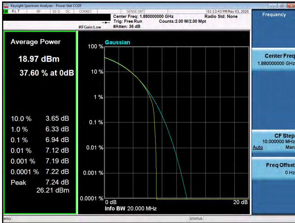
Plot 7-571. PAR Plot (Band n25/2 - 5.0MHz 64-QAM - Full RB Configuration)
