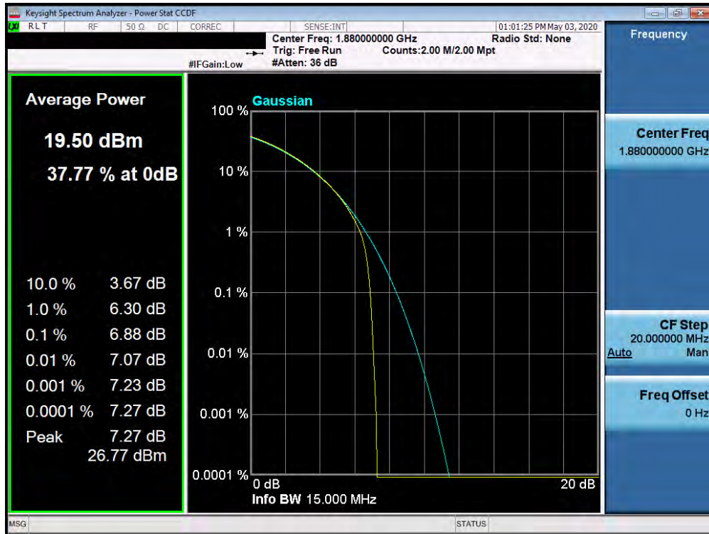
Plot 7-577. PAR Plot (Band n25/2 - 15.0MHz QPSK - Full RB Configuration)
