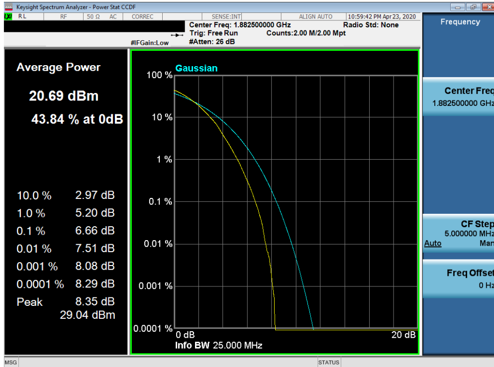
Plot 7-567. PAR Plot (Band 25/2 - 20.0MHz 64-QAM - Full RB Configuration)
