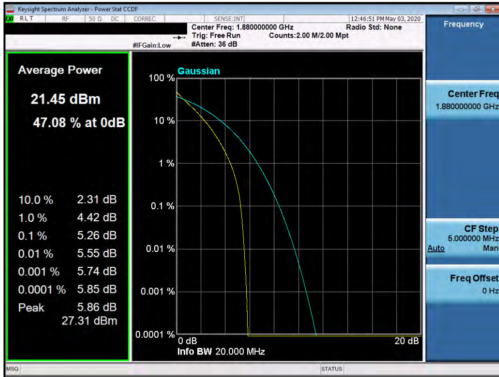
Plot 7-581. PAR Plot (Band n25/2 - 20.0MHz QPSK - Full RB Configuration)
