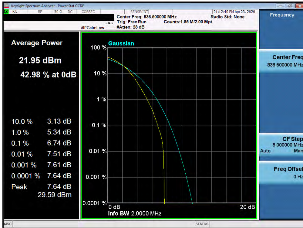
Plot 7-531. PAR Plot (Band 5 - 1.4MHz 64-QAM - Full RB Configuration)
