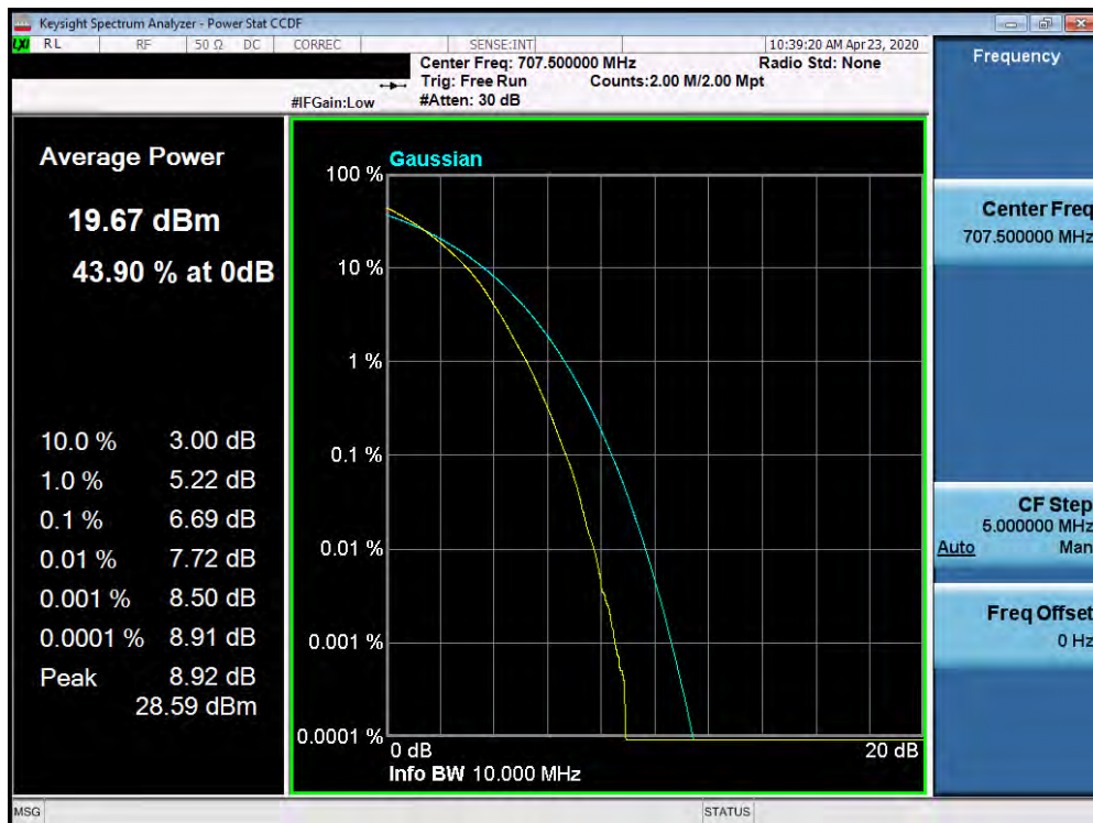
Plot 7-520. PAR Plot (Band 12 - 10.0MHz 256-QAM - Full RB Configuration)
