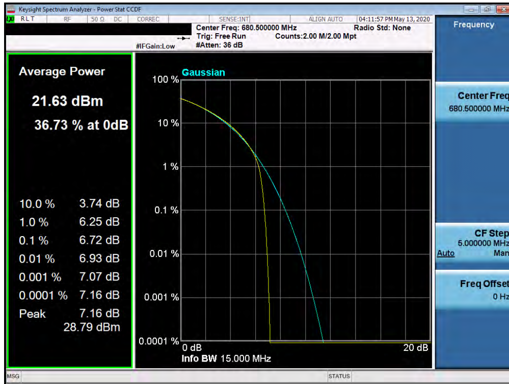
Plot 7-497. PAR Plot (Band n71 - 15.0MHz QPSK - Full RB Configuration)
