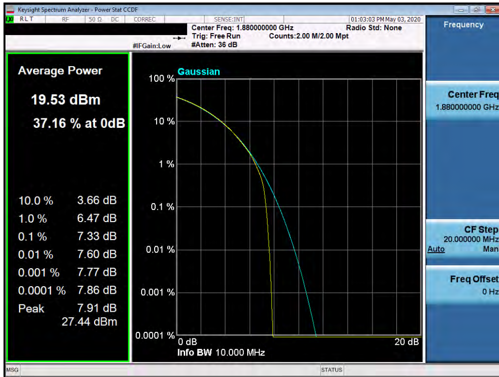
Plot 7-573. PAR Plot (Band n25/2 - 10.0MHz QPSK - Full RB Configuration)
