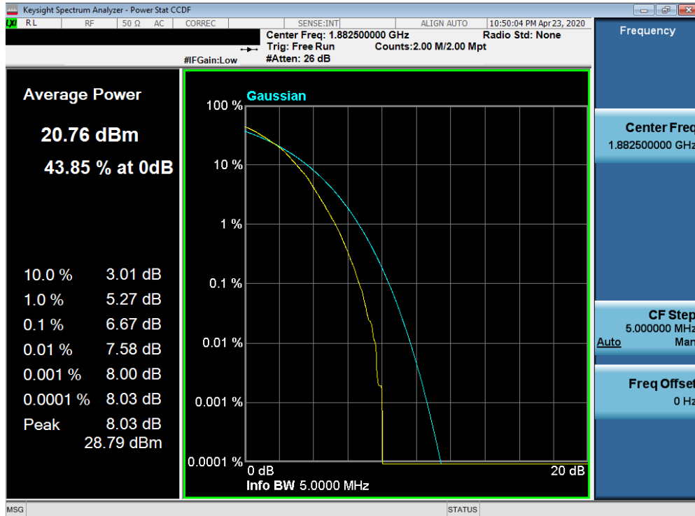
Plot 7-555. PAR Plot (Band 25/2 - 5.0MHz 64-QAM - Full RB Configuration)
