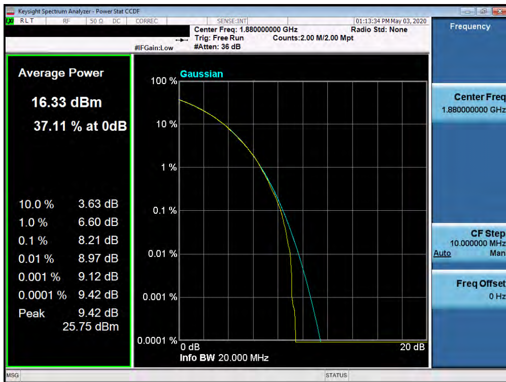
Plot 7-572. PAR Plot (Band n25/2 - 5.0MHz 256-QAM - Full RB Configuration)
