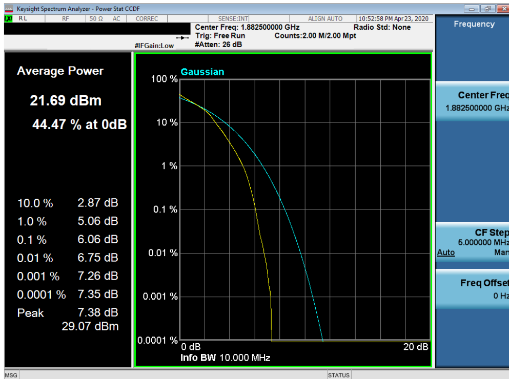
Plot 7-558. PAR Plot (Band 25/2 - 10.0MHz 16-QAM - Full RB Configuration)
