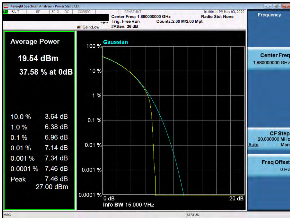
Plot 7-578. PAR Plot (Band n25/2 - 15.0MHz 16-QAM - Full RB Configuration)
