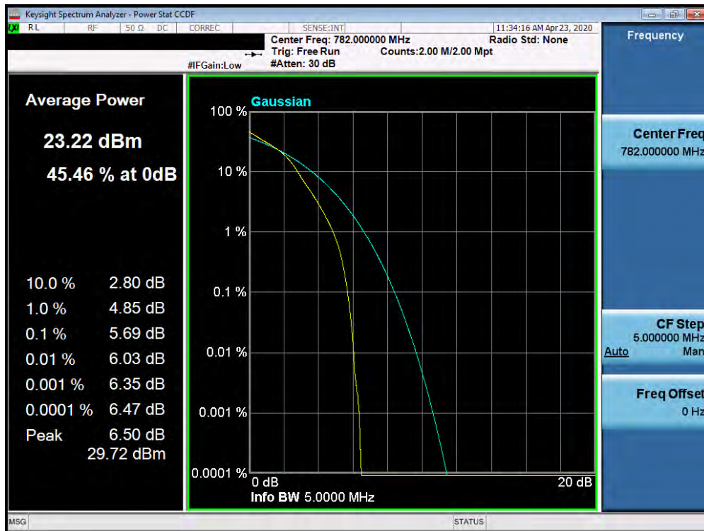
Plot 7-522. PAR Plot (Band 13 - 5.0MHz 16-QAM - Full RB Configuration)
