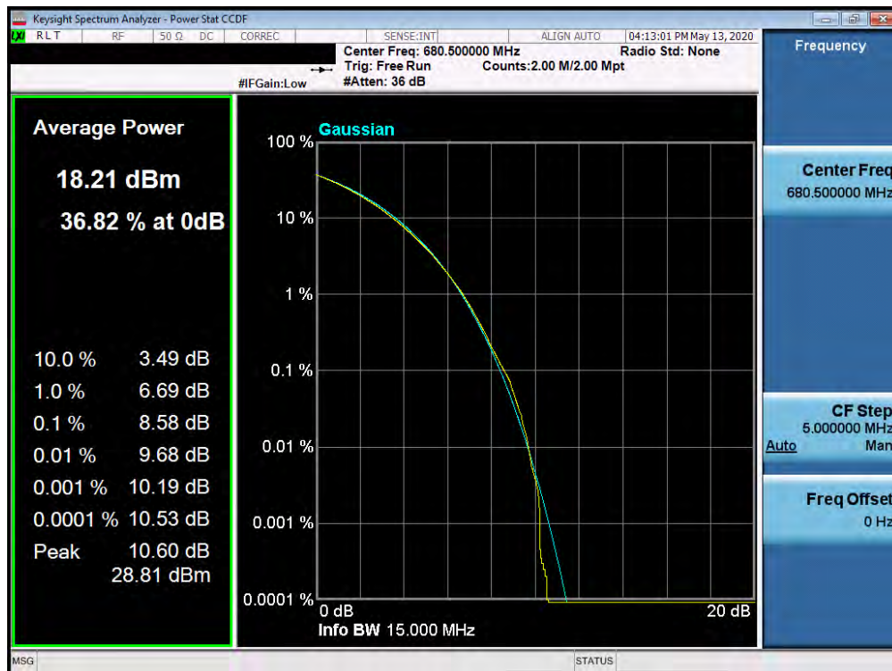
Plot 7-500. PAR Plot (Band n71 - 15.0MHz 256-QAM - Full RB Configuration)
