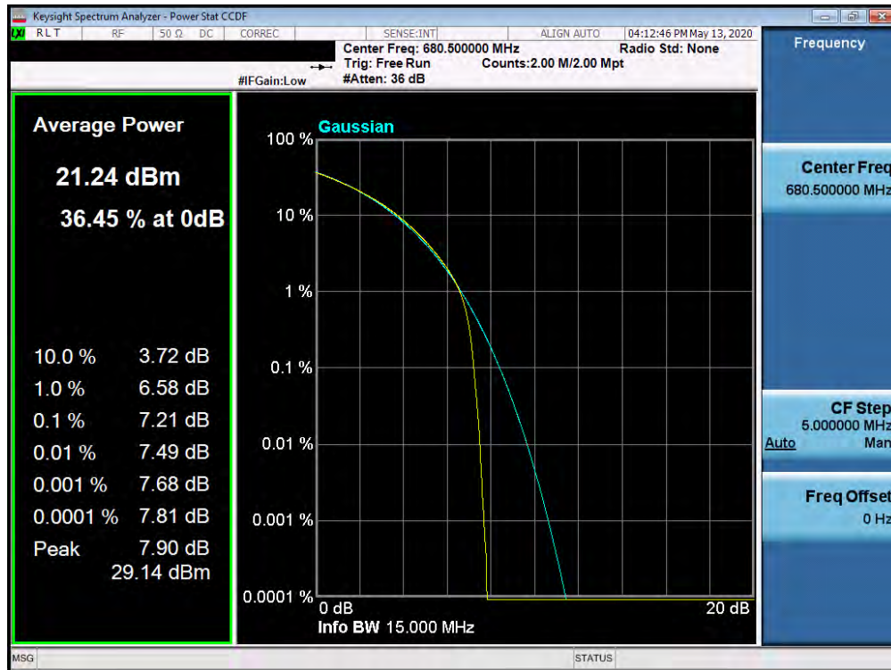
Plot 7-499. PAR Plot (Band n71 - 15.0MHz 64-QAM - Full RB Configuration)
