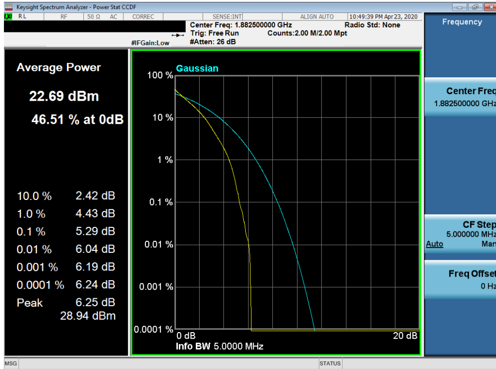
Plot 7-553. PAR Plot (Band 25/2 - 5.0MHz QPSK - Full RB Configuration)
