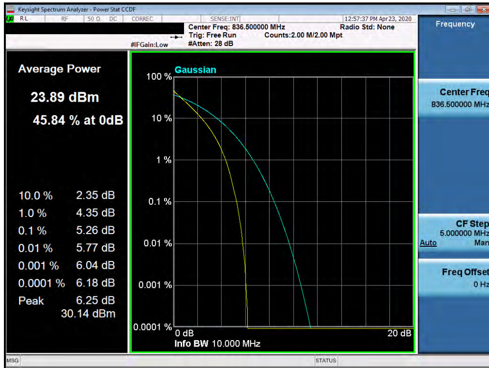
Plot 7-541. PAR Plot (Band 5 - 10.0MHz QPSK - Full RB Configuration)
