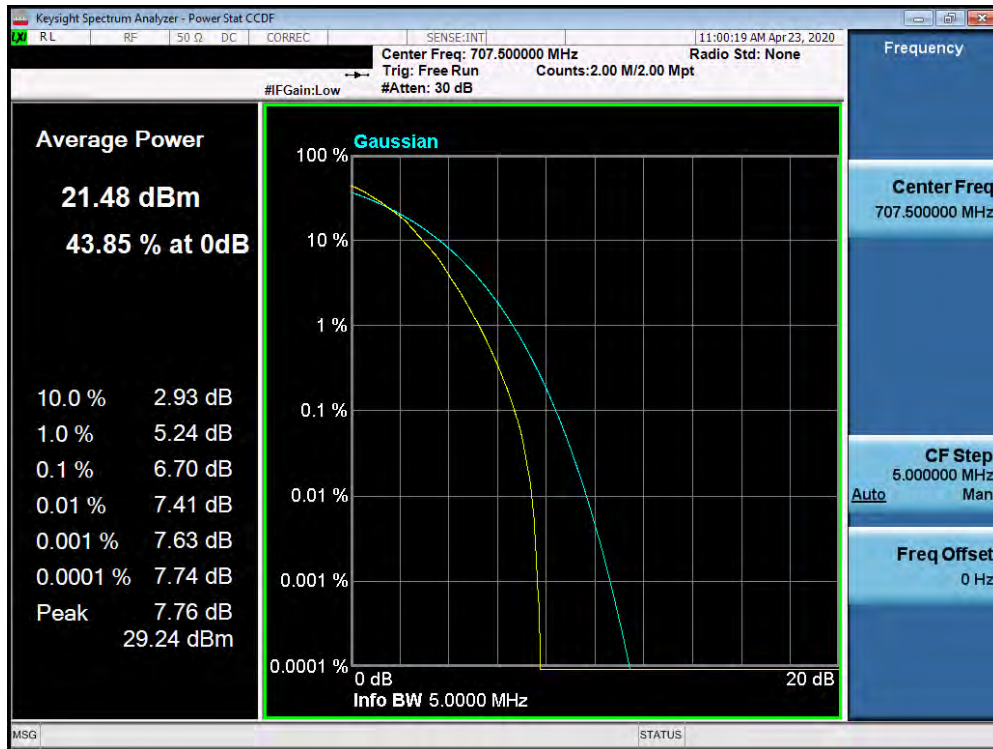
Plot 7-515. PAR Plot (Band 12 - 5.0MHz 64-QAM - Full RB Configuration)
