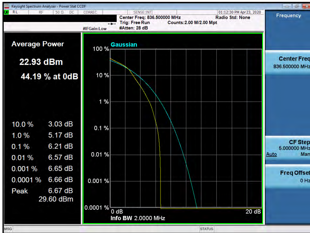
Plot 7-530. PAR Plot (Band 5 - 1.4MHz 16-QAM - Full RB Configuration)
