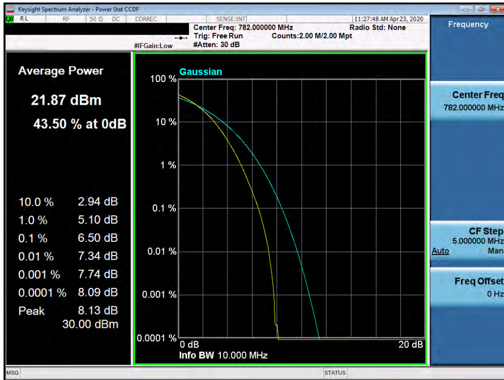
Plot 7-527. PAR Plot (Band 13 - 10.0MHz 64-QAM - Full RB Configuration)
