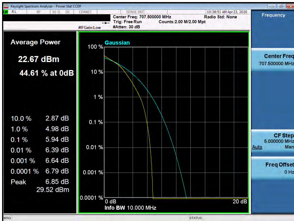
Plot 7-518. PAR Plot (Band 12 - 10.0MHz 16-QAM - Full RB Configuration)
