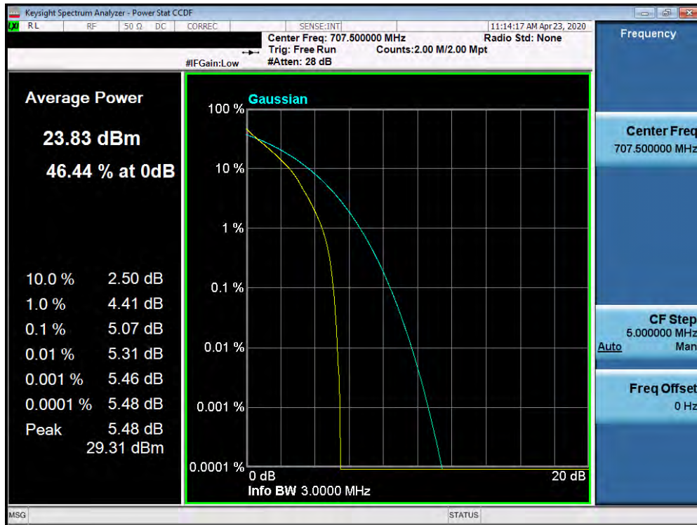
Plot 7-509. PAR Plot (Band 12 - 3.0MHz QPSK - Full RB Configuration)
