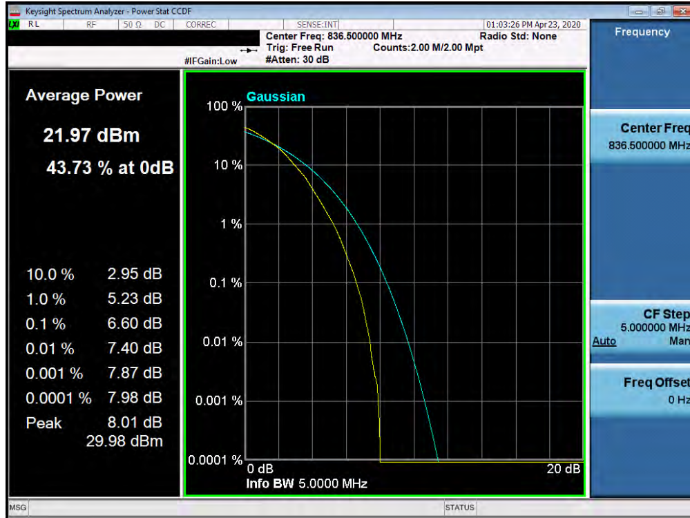
Plot 7-539. PAR Plot (Band 5 - 5.0MHz 64-QAM - Full RB Configuration)
