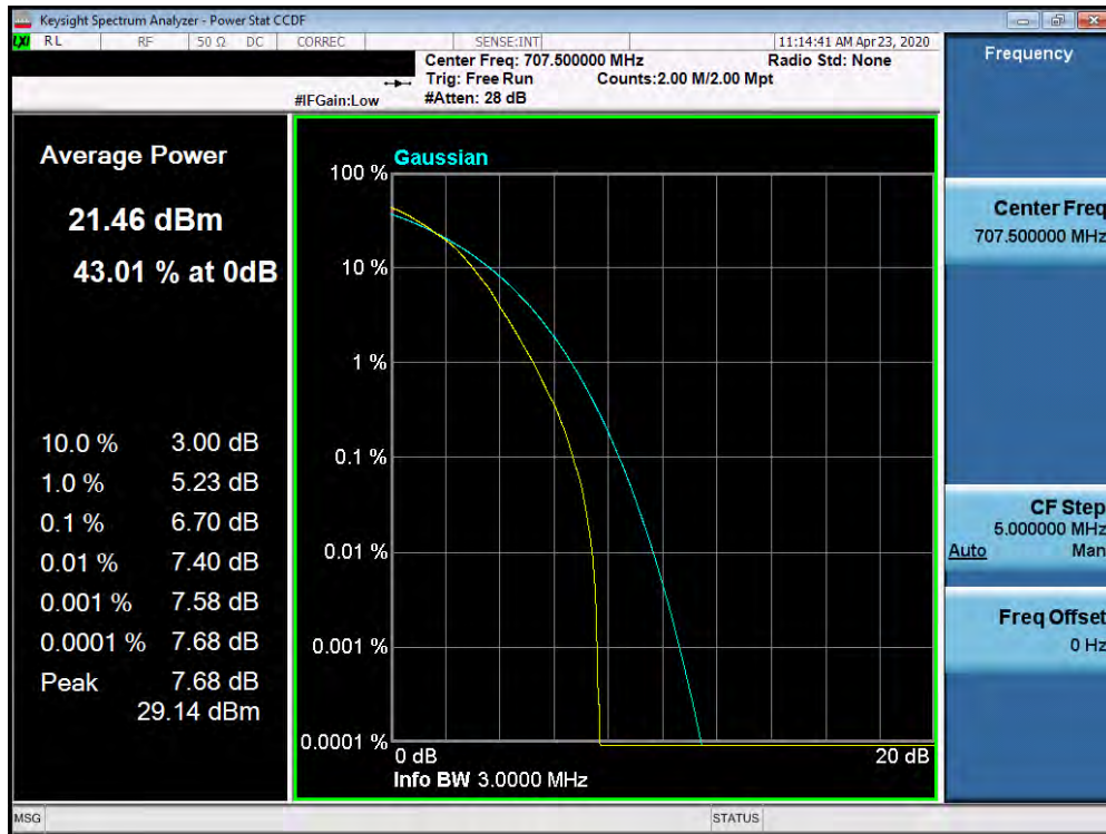
Plot 7-511. PAR Plot (Band 12 - 3.0MHz 64-QAM - Full RB Configuration)
