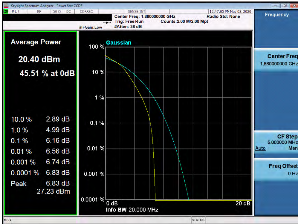
Plot 7-582. PAR Plot (Band n25/2 - 20.0MHz 16-QAM - Full RB Configuration)
