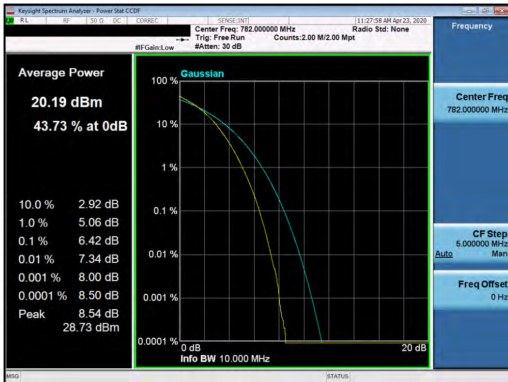
Plot 7-528. PAR Plot (Band 13 - 10.0MHz 256-QAM - Full RB Configuration)
