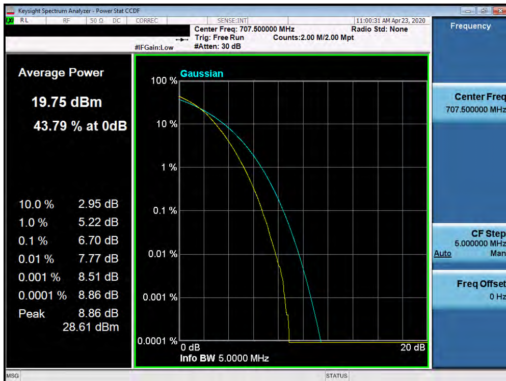
Plot 7-516. PAR Plot (Band 12 - 5.0MHz 256-QAM - Full RB Configuration)
