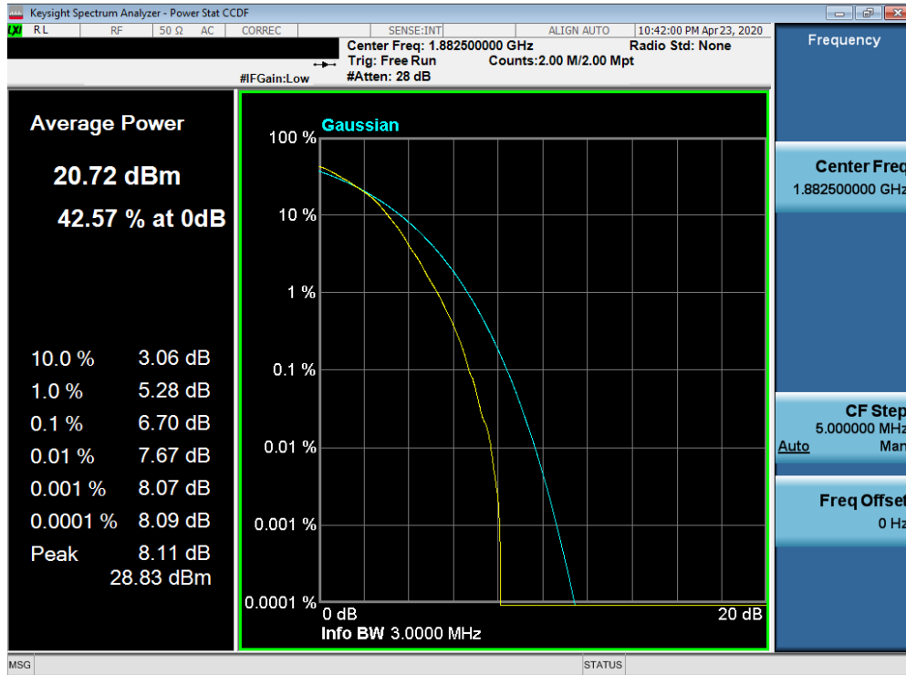
Plot 7-551. PAR Plot (Band 25/2 - 3.0MHz 64-QAM - Full RB Configuration)
