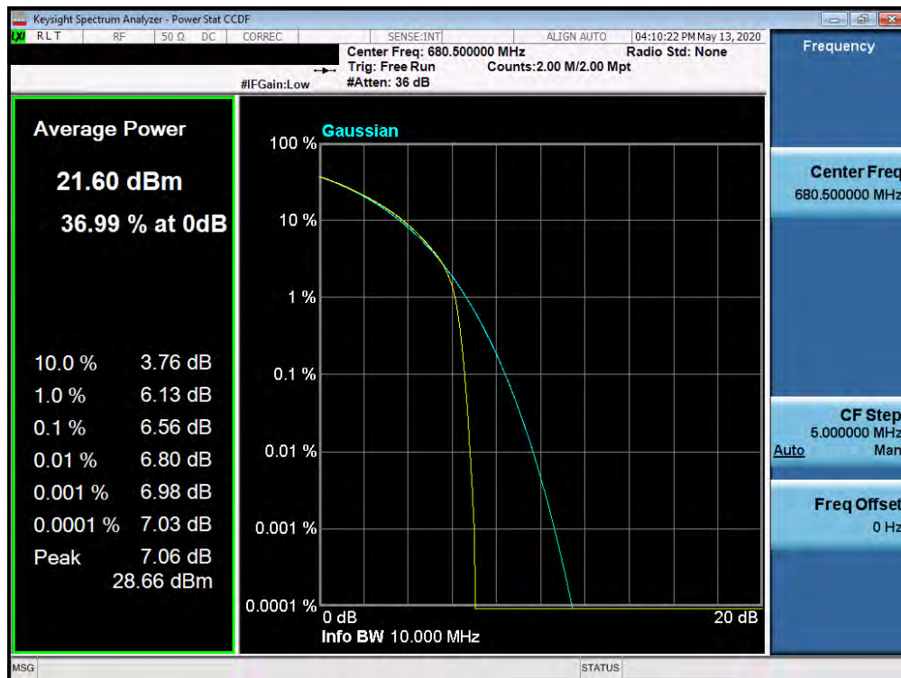
Plot 7-494. PAR Plot (Band n71 - 10.0MHz 16-QAM - Full RB Configuration)
