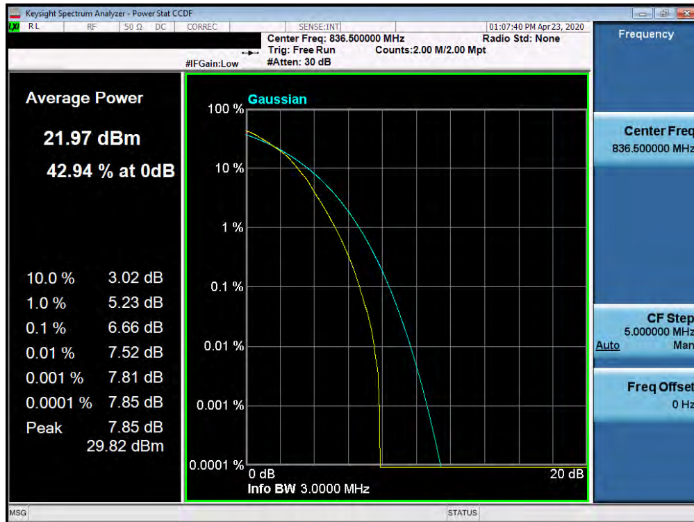
Plot 7-535. PAR Plot (Band 5 - 3.0MHz 64-QAM - Full RB Configuration)
