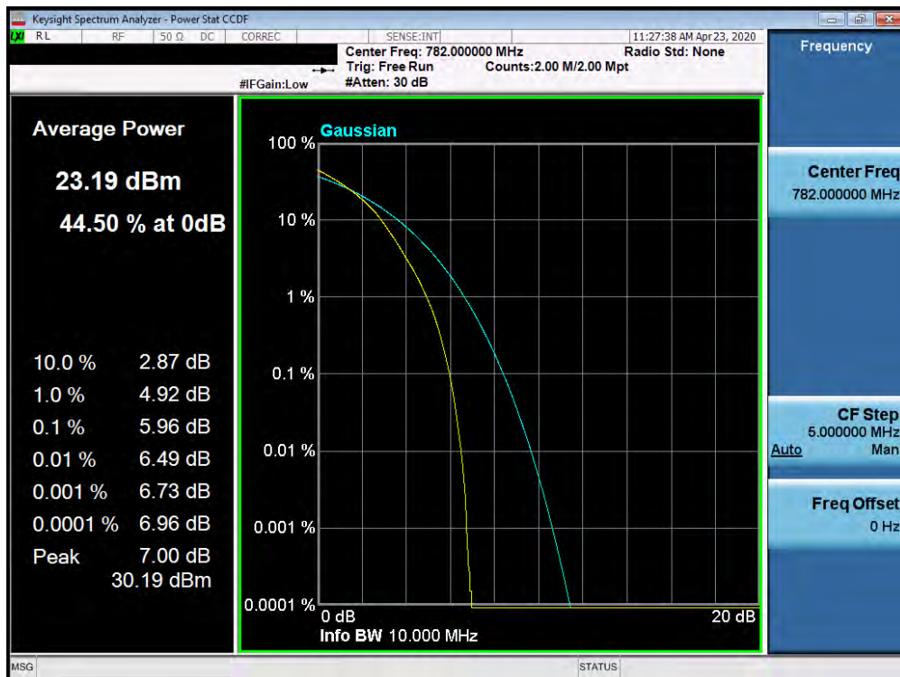
Plot 7-526. PAR Plot (Band 13 - 10.0MHz 16-QAM - Full RB Configuration)
