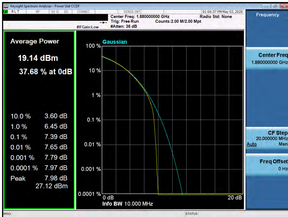
Plot 7-576. PAR Plot (Band n25/2 - 10.0MHz 256-QAM - Full RB Configuration)
