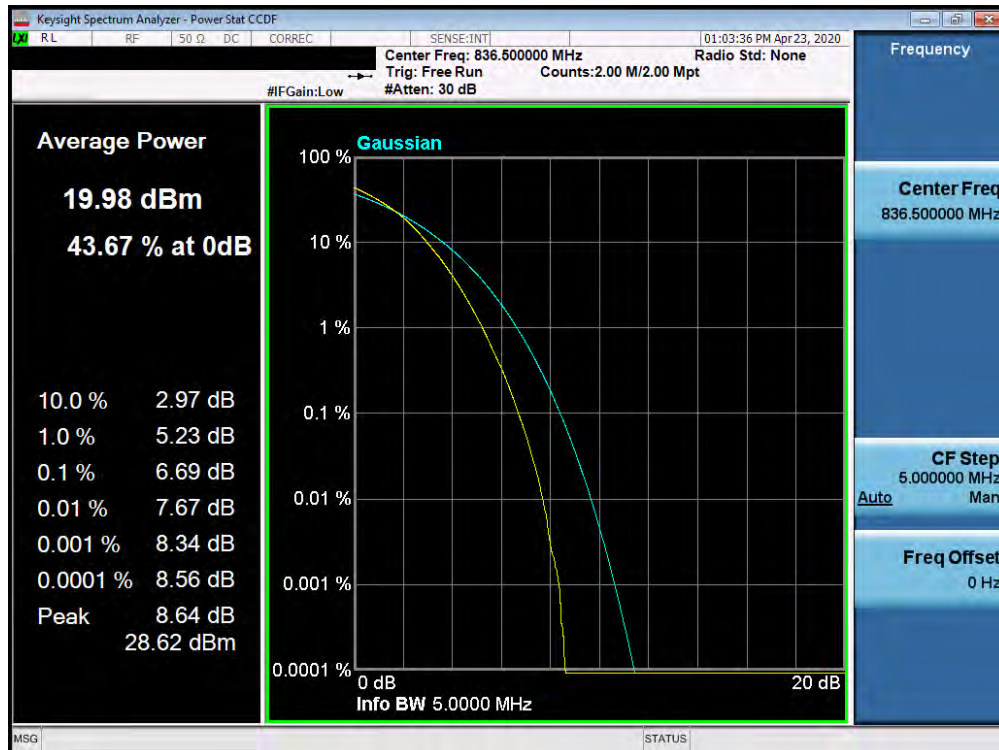
Plot 7-540. PAR Plot (Band 5 - 5.0MHz 256-QAM - Full RB Configuration)
