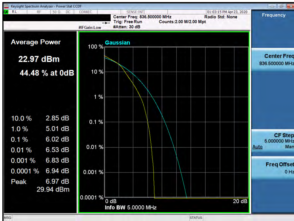
Plot 7-538. PAR Plot (Band 5 - 5.0MHz 16-QAM - Full RB Configuration)
