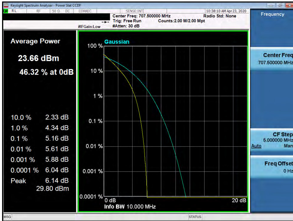
Plot 7-517. PAR Plot (Band 12 - 10.0MHz QPSK - Full RB Configuration)
