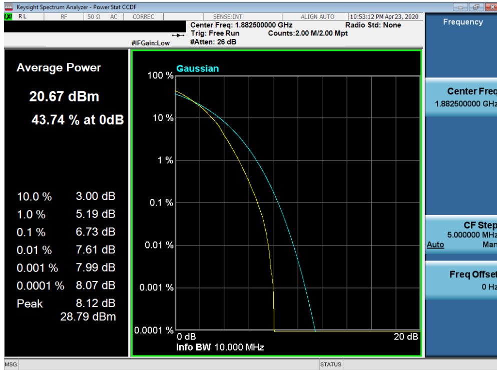
Plot 7-559. PAR Plot (Band 25/2 - 10.0MHz 64-QAM - Full RB Configuration)
