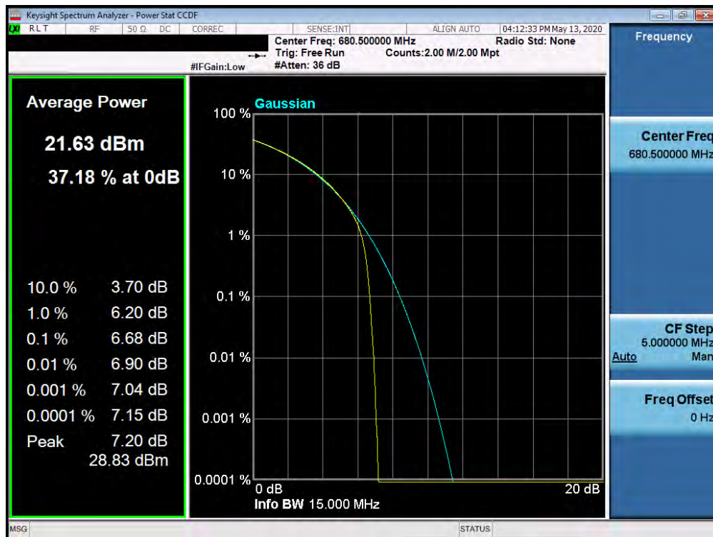
Plot 7-498. PAR Plot (Band n71 - 15.0MHz 16-QAM - Full RB Configuration)
