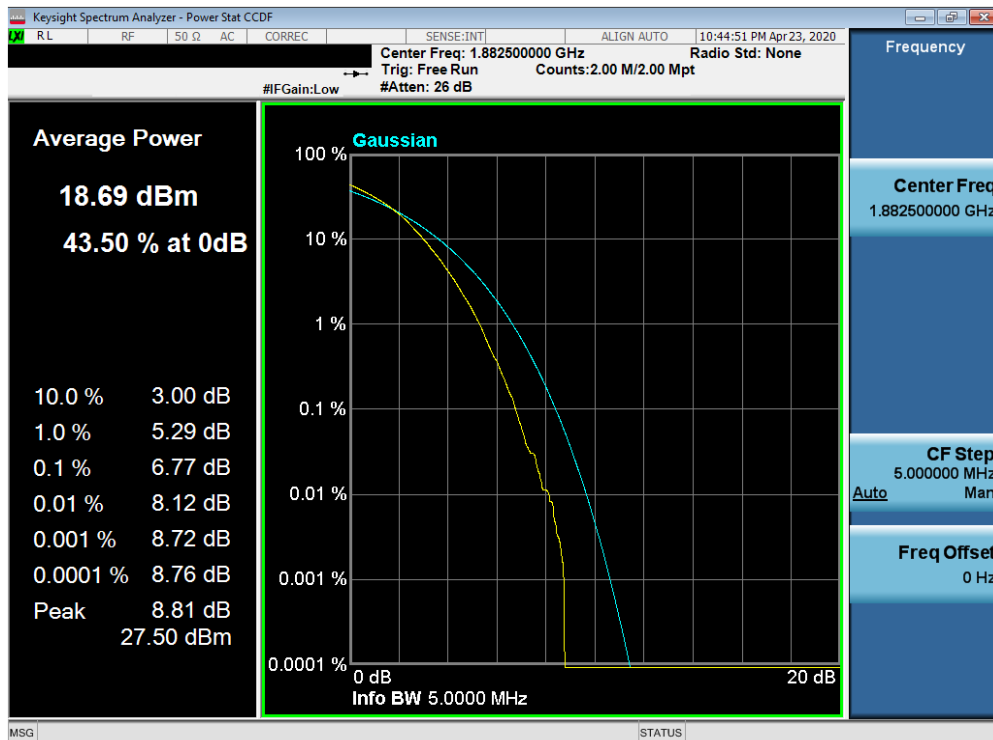
Plot 7-556. PAR Plot (Band 25/2 - 5.0MHz 256-QAM - Full RB Configuration)
