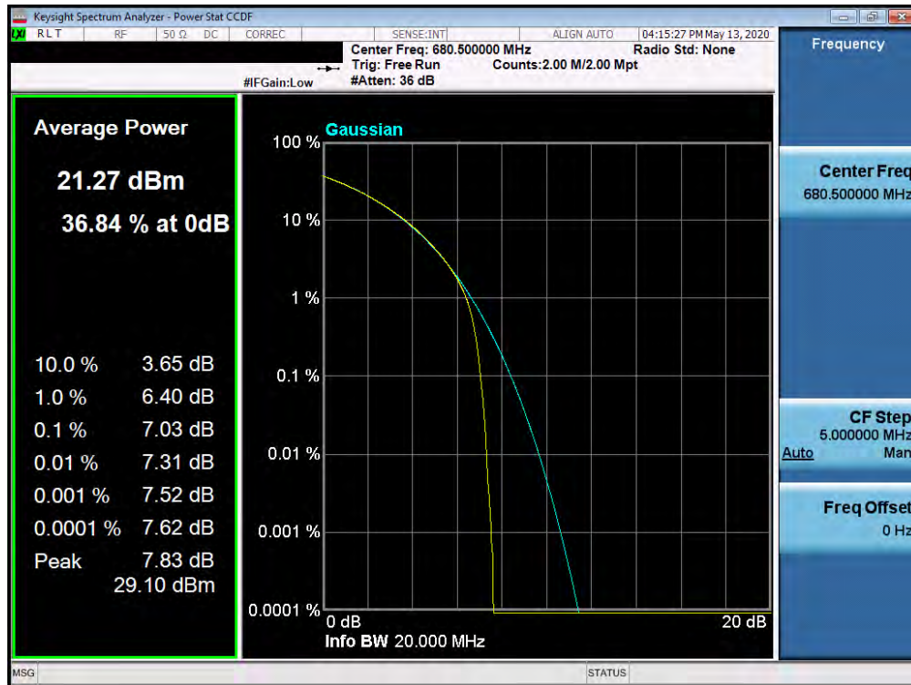
Plot 7-503. PAR Plot (Band n71 - 20.0MHz 64-QAM - Full RB Configuration)
