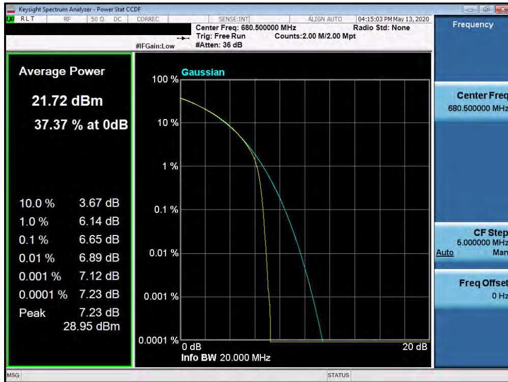
Plot 7-501. PAR Plot (Band n71 - 20.0MHz QPSK - Full RB Configuration)
