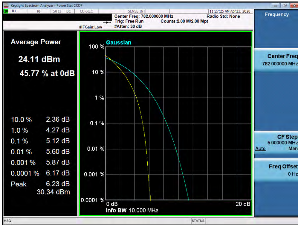
Plot 7-525. PAR Plot (Band 13 - 10.0MHz QPSK - Full RB Configuration)
