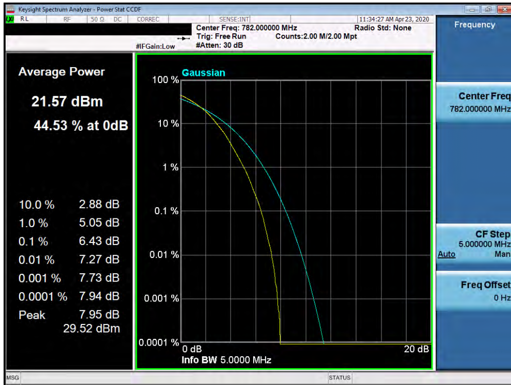
Plot 7-523. PAR Plot (Band 13 - 5.0MHz 64-QAM - Full RB Configuration)
