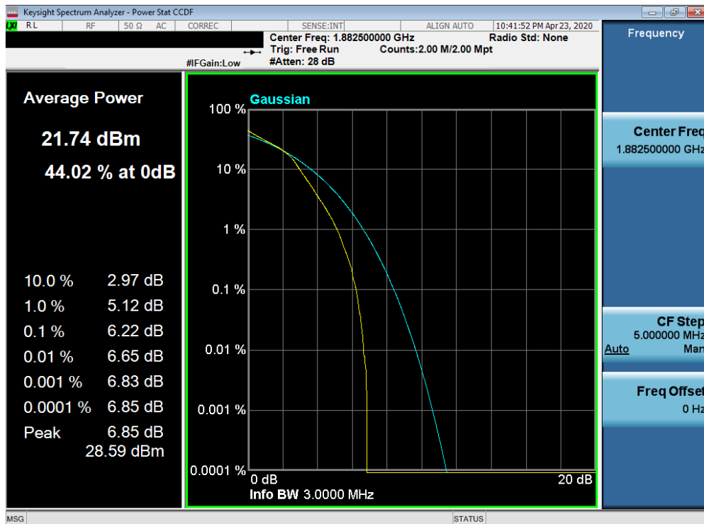
Plot 7-550. PAR Plot (Band 25/2 - 3.0MHz 16-QAM - Full RB Configuration)
