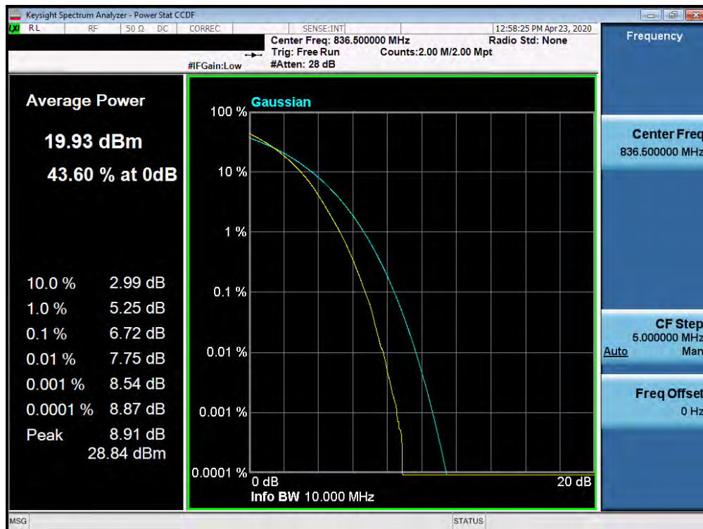
Plot 7-544. PAR Plot (Band 5 - 10.0MHz 256-QAM - Full RB Configuration)
