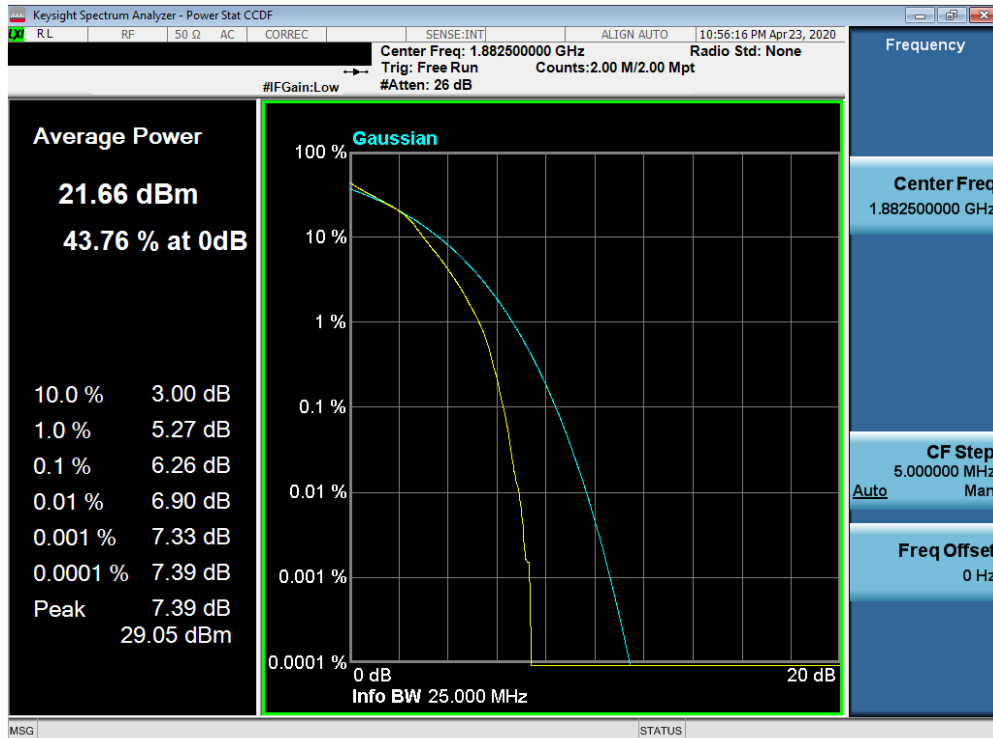
Plot 7-562. PAR Plot (Band 25/2 - 15.0MHz 16-QAM - Full RB Configuration)
