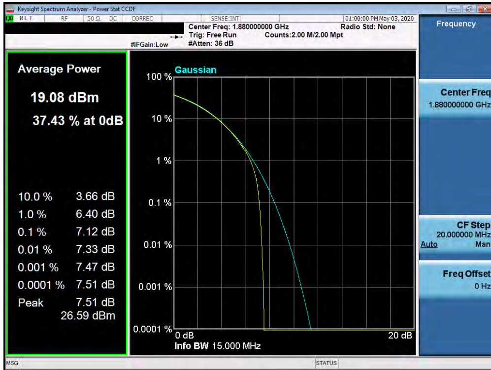
Plot 7-579. PAR Plot (Band n25/2 - 15.0MHz 64-QAM - Full RB Configuration)
