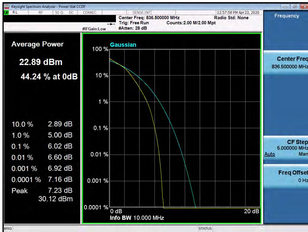
Plot 7-542. PAR Plot (Band 5 - 10.0MHz 16-QAM - Full RB Configuration)
