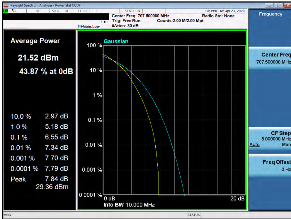
Plot 7-519. PAR Plot (Band 12 - 10.0MHz 64-QAM - Full RB Configuration)
