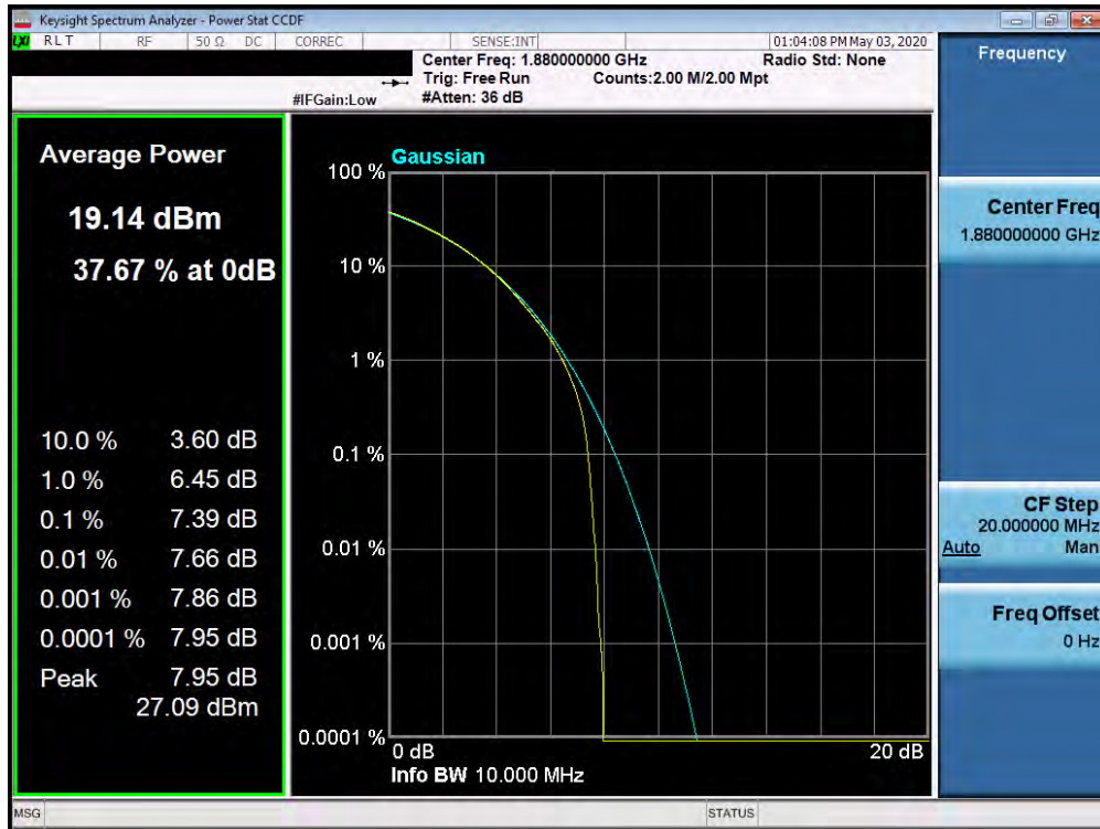
Plot 7-575. PAR Plot (Band n25/2 - 10.0MHz 64-QAM - Full RB Configuration)
