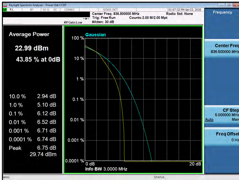
Plot 7-534. PAR Plot (Band 5 - 3.0MHz 16-QAM - Full RB Configuration)
