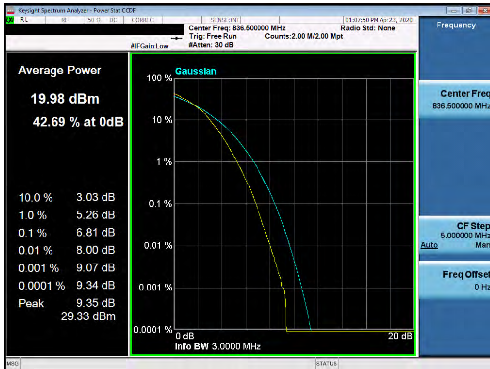
Plot 7-536. PAR Plot (Band 5 - 3.0MHz 256-QAM - Full RB Configuration)
