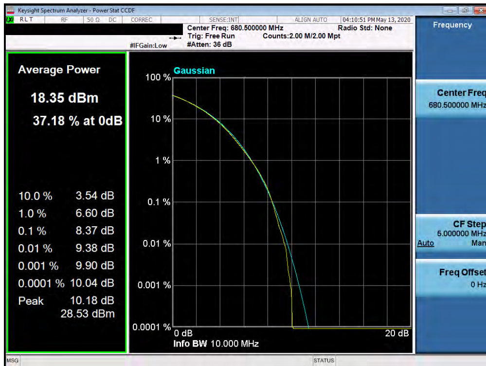
Plot 7-496. PAR Plot (Band n71 - 10.0MHz 256-QAM - Full RB Configuration)
