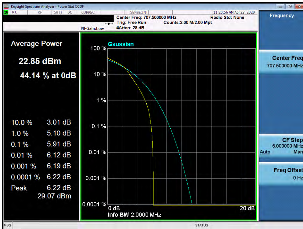
Plot 7-506. PAR Plot (Band 12 - 1.4MHz 16-QAM - Full RB Configuration)
