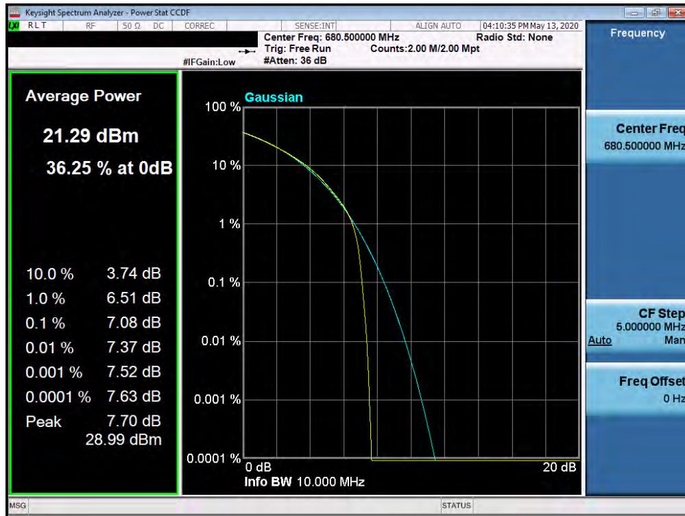
Plot 7-495. PAR Plot (Band n71 - 10.0MHz 64-QAM - Full RB Configuration)
