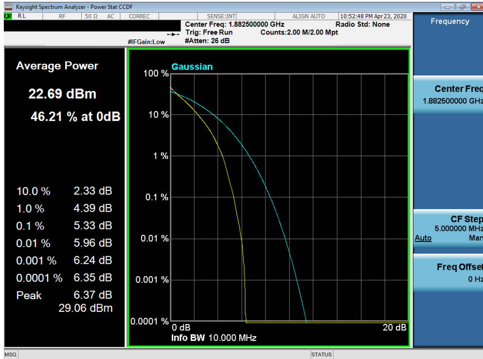
Plot 7-557. PAR Plot (Band 25/2 - 10.0MHz QPSK - Full RB Configuration)
