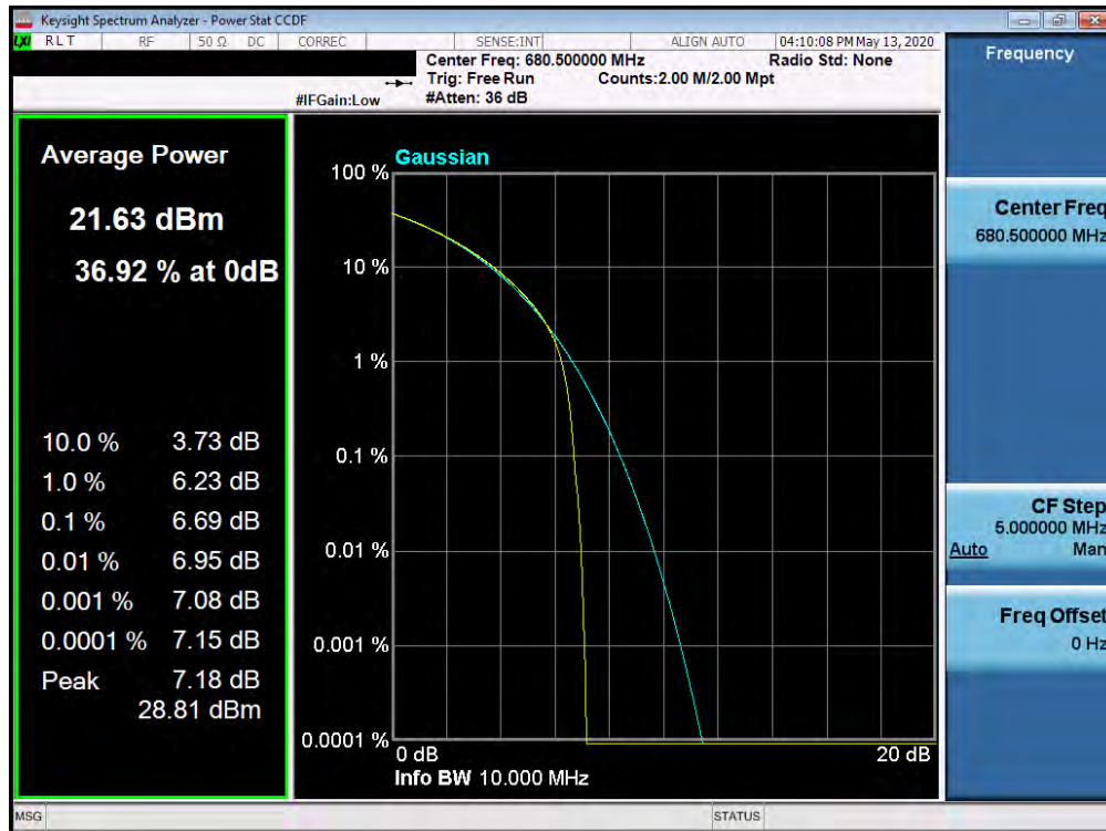
Plot 7-493. PAR Plot (Band n71 - 10.0MHz QPSK - Full RB Configuration)
