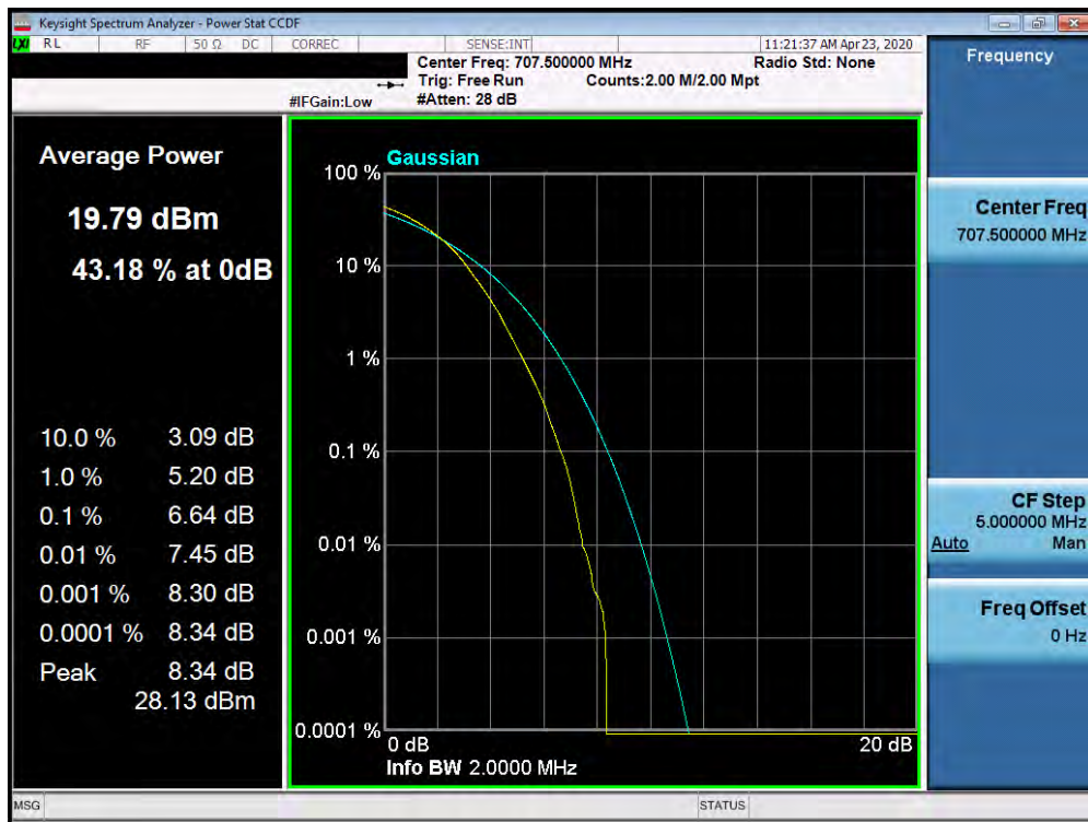
Plot 7-508. PAR Plot (Band 12 - 1.4MHz 256-QAM - Full RB Configuration)
