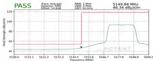
Plot 7-397. Radiated Lower Band Edge Plot MIMO (Average – UNII Band 1 – 242 Tones)
