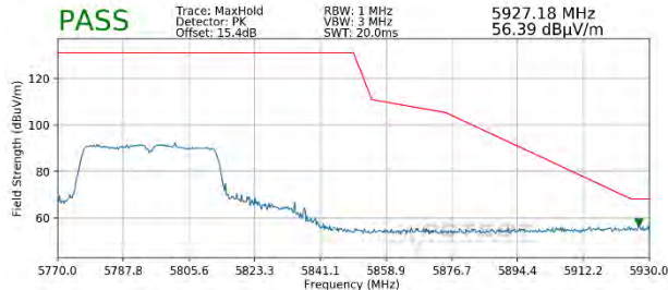
Plot 7-389. Radiated Upper Band Edge Plot SISO ANT2 (Peak - UNII Band 3 - 484 Tones)
