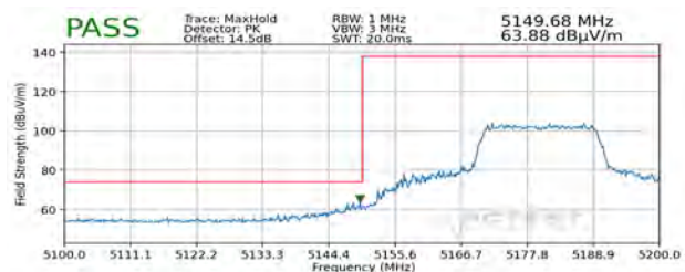
Plot 7-377. Radiated Lower Band Edge Plot SISO ANT2 (Peak - UNII Band 1 - 242 Tones)
