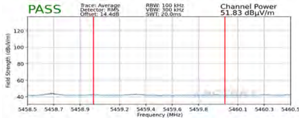
Plot 7-373. Radiated Lower Band Edge Plot SISO ANT1 (Average - UNII Band 2C - 996 Tones)
