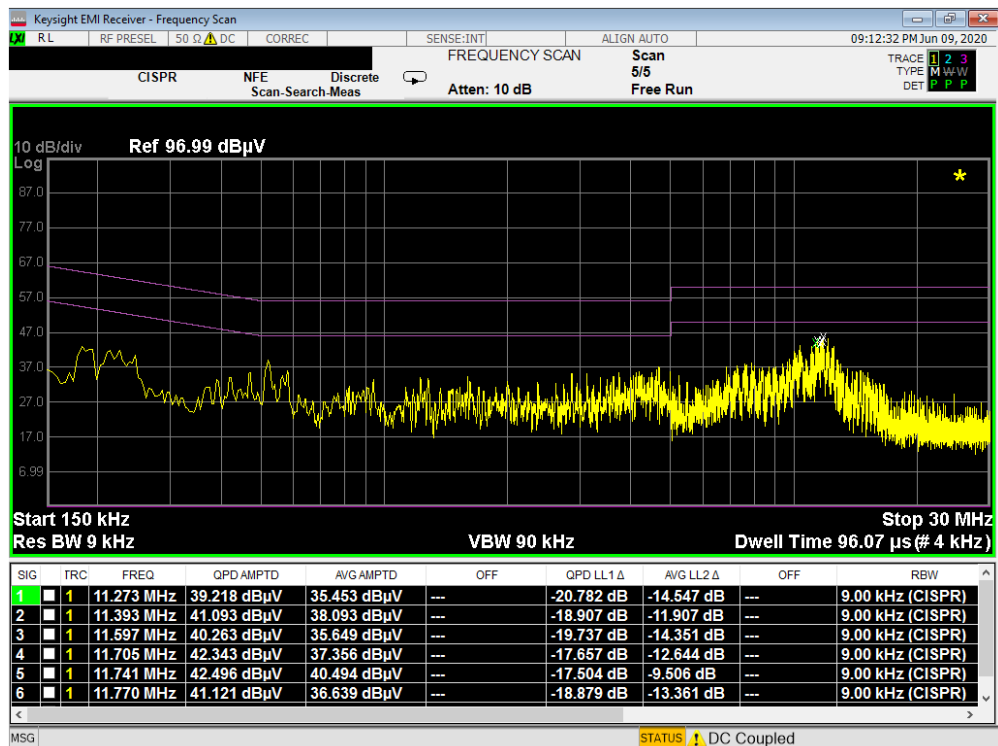
Plot 7-9. Line-Conducted Test Plot (N) with WCP
