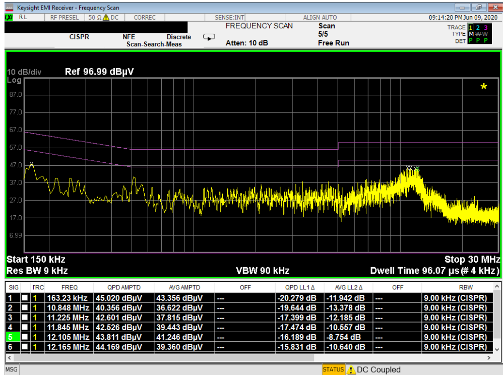
Plot 7-8. Line-Conducted Test Plot (L1) with WCP
