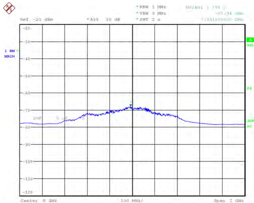
Plot 7-106. UWB Peak Power Measurement - ANT 2 - CH.9 – SP1 – HPRF
