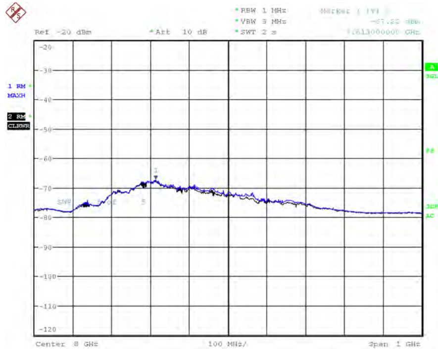
Plot 7-84. UWB Peak Power Measurement - ANT 2 - CH.9 – SP3 – BPRF
