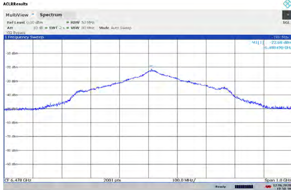
Plot 7-62. UWB Peak Power Measurement - ANT 1 - CH.5 - SP0 – BPRF
