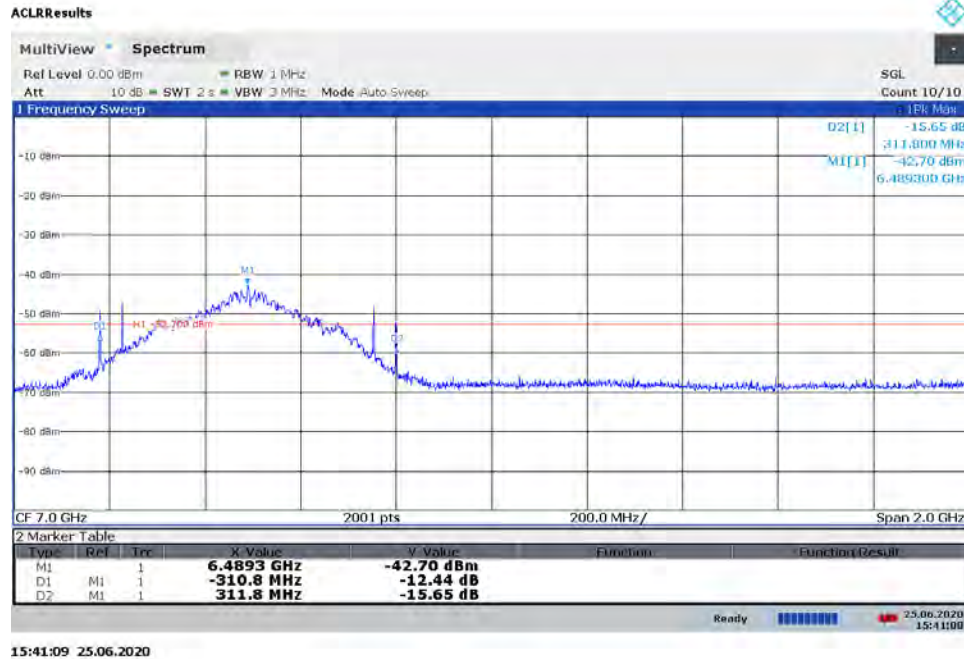
Plot 7-13. BANDWIDTH Plot - ANT1 - CH.5 - SP0 – Preamble 11
