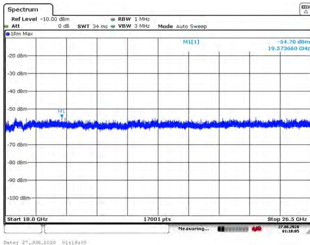
Plot 7-129. Radiated Spurious Pre-Scan 18 - 26.5 GHz - CH.9 - ANT 1
