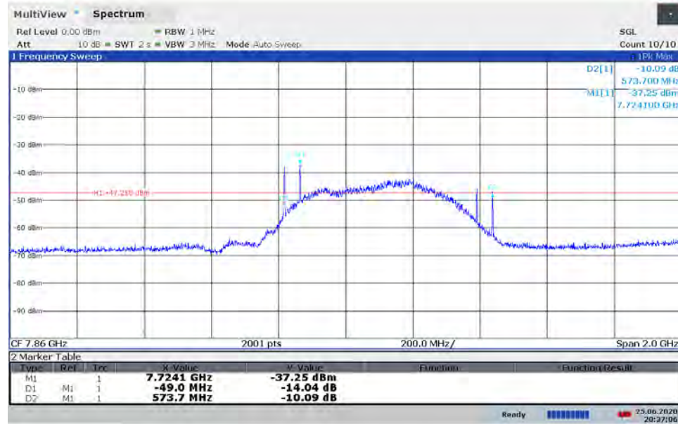
Plot 7-39. BANDWIDTH Plot - ANT1 - CH.9 – SP3 – Preamble 10
