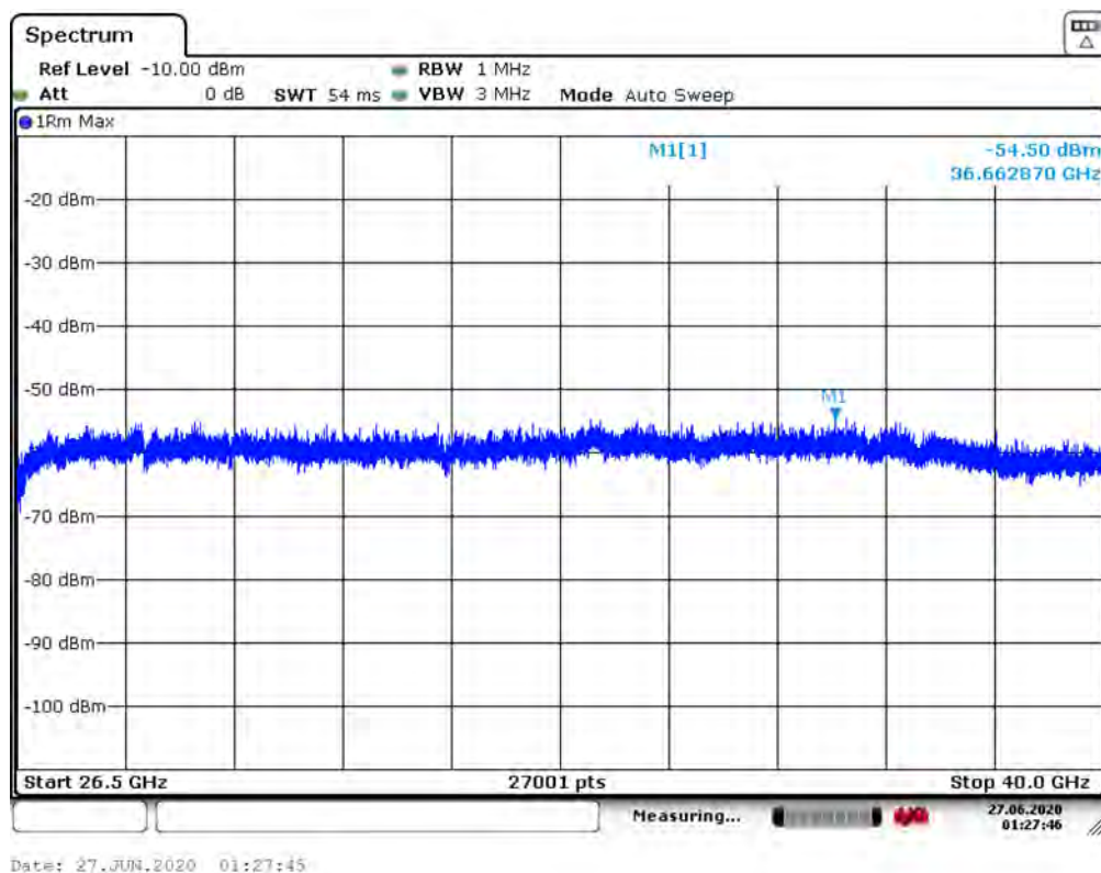
Plot 7-130. Radiated Spurious Pre-Scan 26.5 – 40.0 GHz - CH.9 - ANT 1
