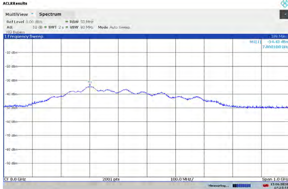
Plot 7-84. UWB Peak Power Measurement - ANT 2 - CH.9 – SP3 – BPRF
