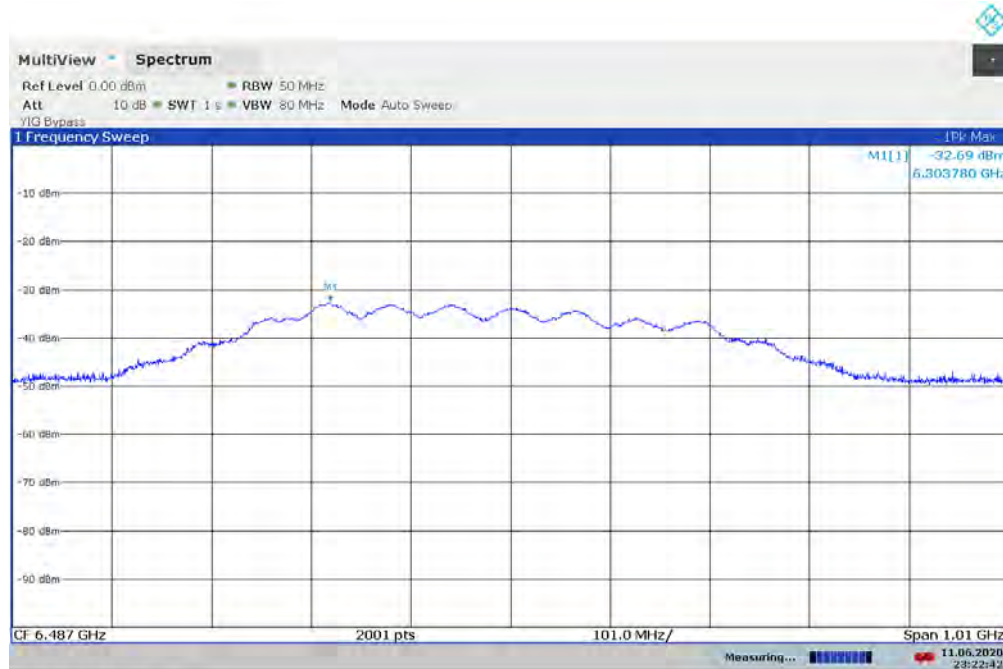
Plot 7-78. UWB Peak Power Measurement - ANT 2 - CH.5 – SP3 – BPRF
