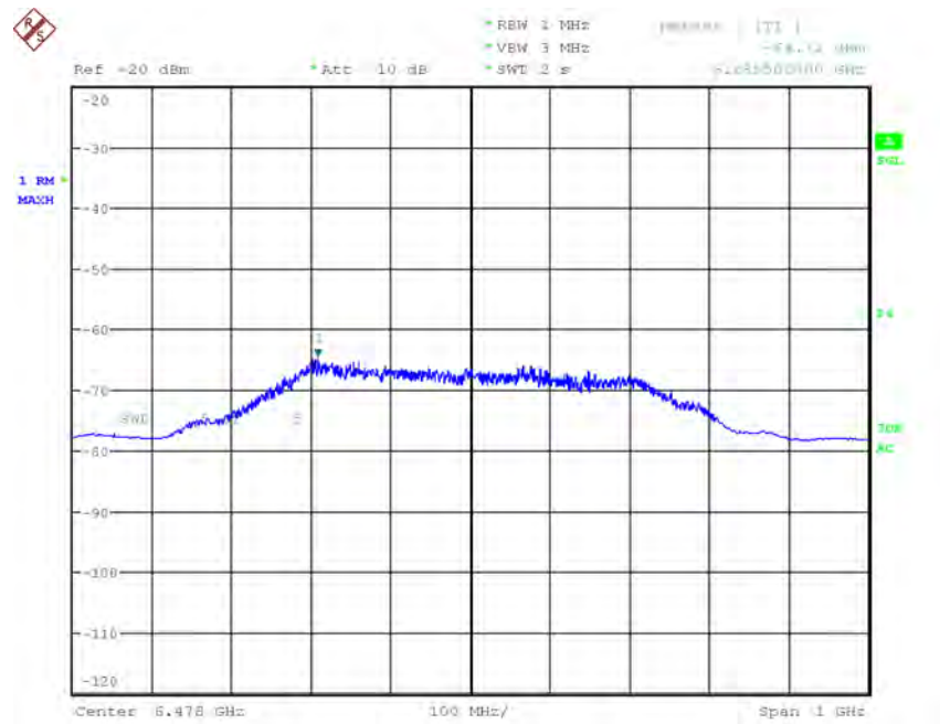
Plot 7-98. UWB Peak Power Measurement - ANT 2 - CH.5 - SP0 – HPRF
