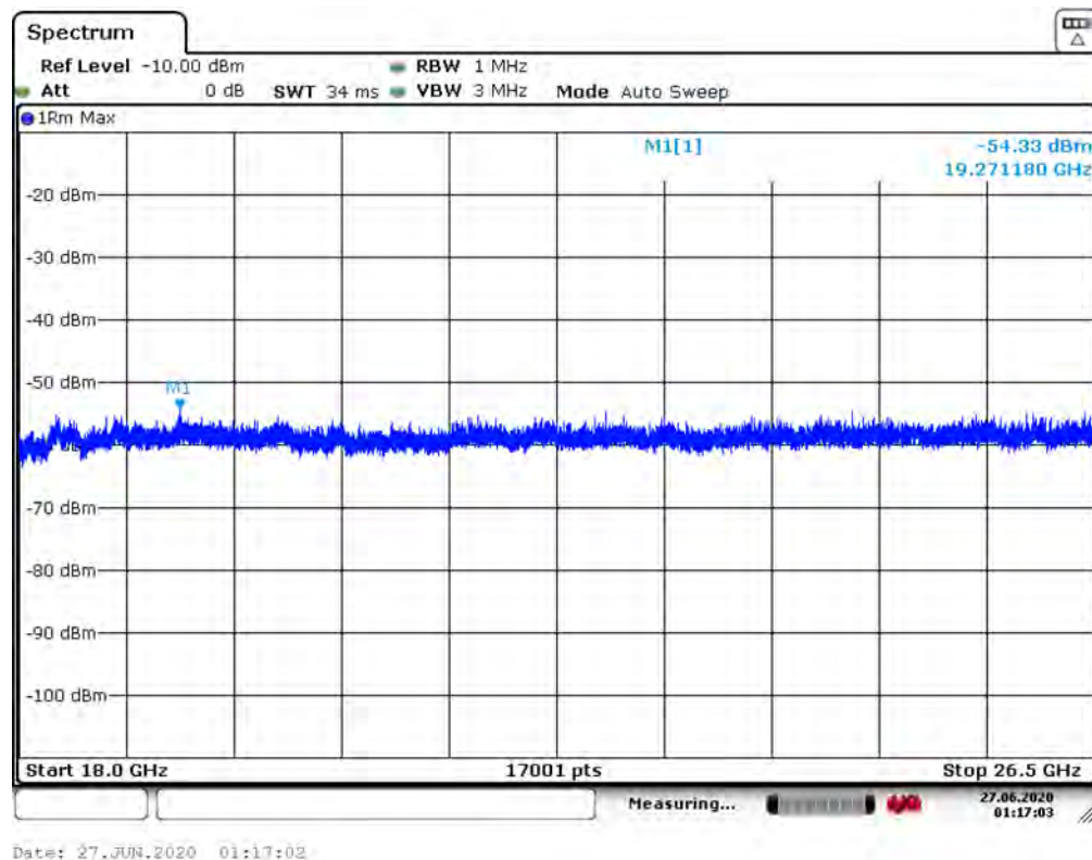
Plot 7-122. Radiated Spurious Pre-Scan 18 - 26.5 GHz - CH.5 - ANT 2
