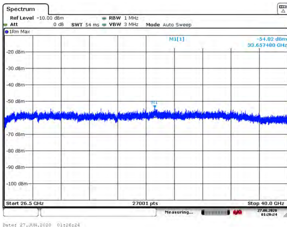
Plot 7-137. Radiated Spurious Pre-Scan 26.5 – 40.0 GHz - CH.9 - ANT 2
