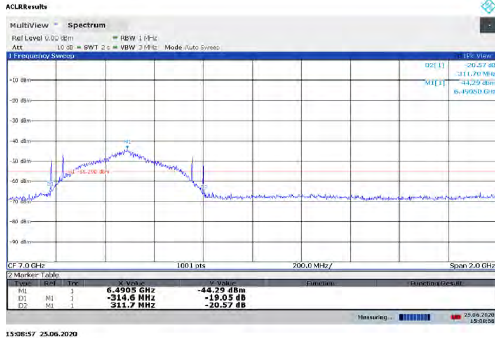
Plot 7-3. BANDWIDTH Plot - ANT1 - CH.5 – SP3 – Preamble 9
