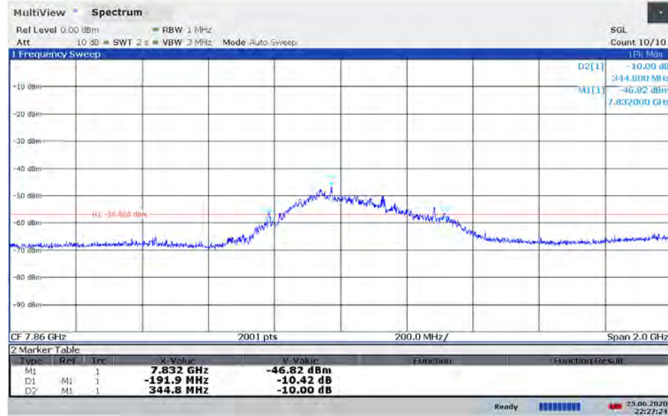
Plot 7-47. BANDWIDTH Plot - ANT1 - CH.9 – SP1 – Preamble 11
