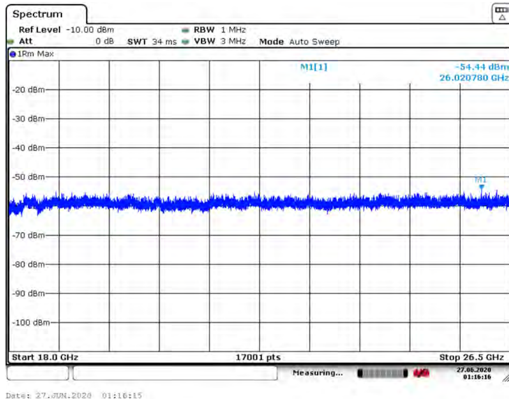
Plot 7-115. Radiated Spurious Pre-Scan 18 - 26.5 GHz - CH.5 - ANT 1
