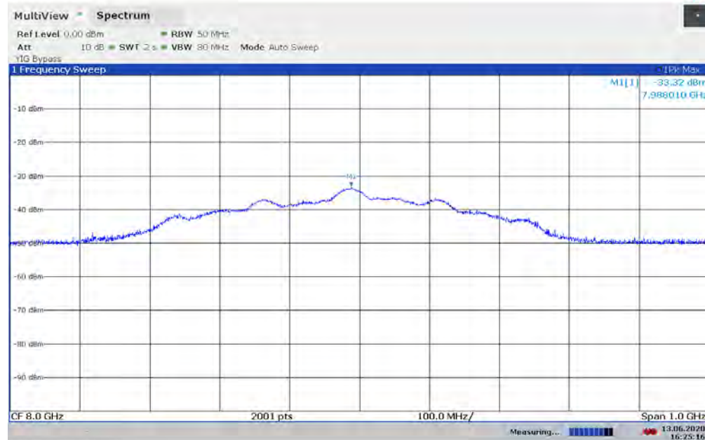
Plot 7-94. UWB Peak Power Measurement - ANT 1 - CH.9 – SP1 – HPRF
