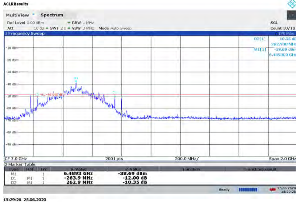
Plot 7-7. BANDWIDTH Plot - ANT1 - CH.5 - SP0 - Preamble 10
