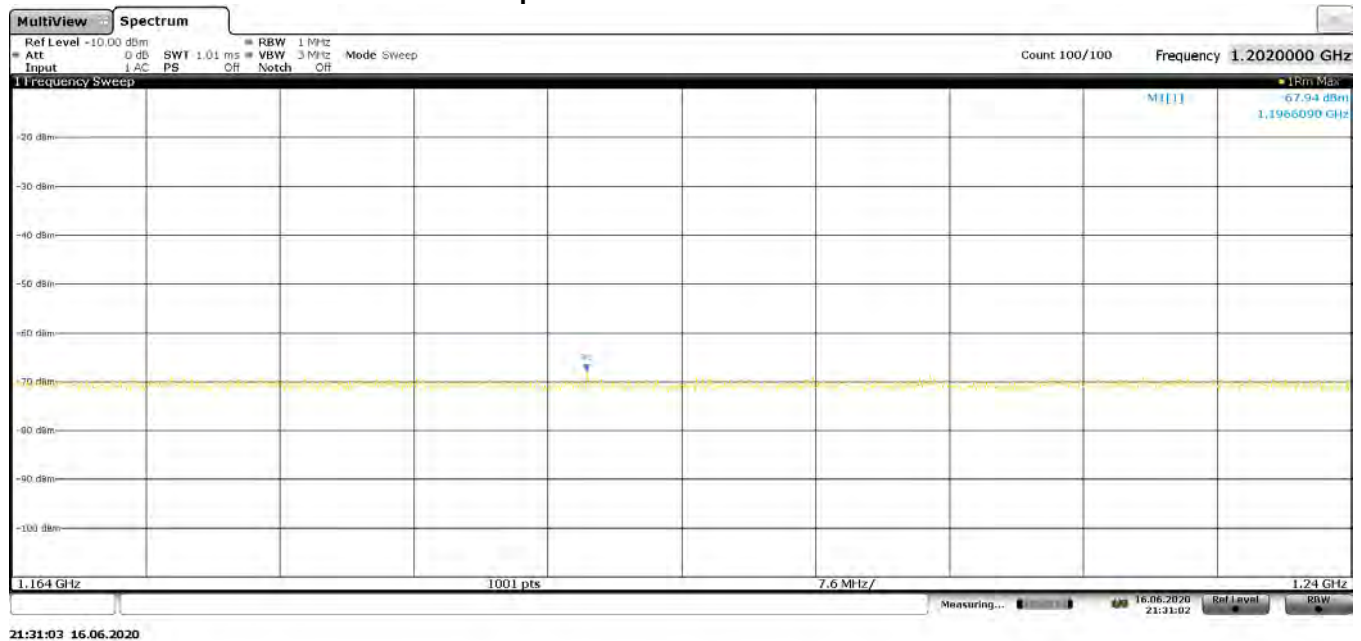
Plot 7-118. Radiated Spurious Pre-Scan 1161 - 1240 MHz - CH.5 - ANT 2
