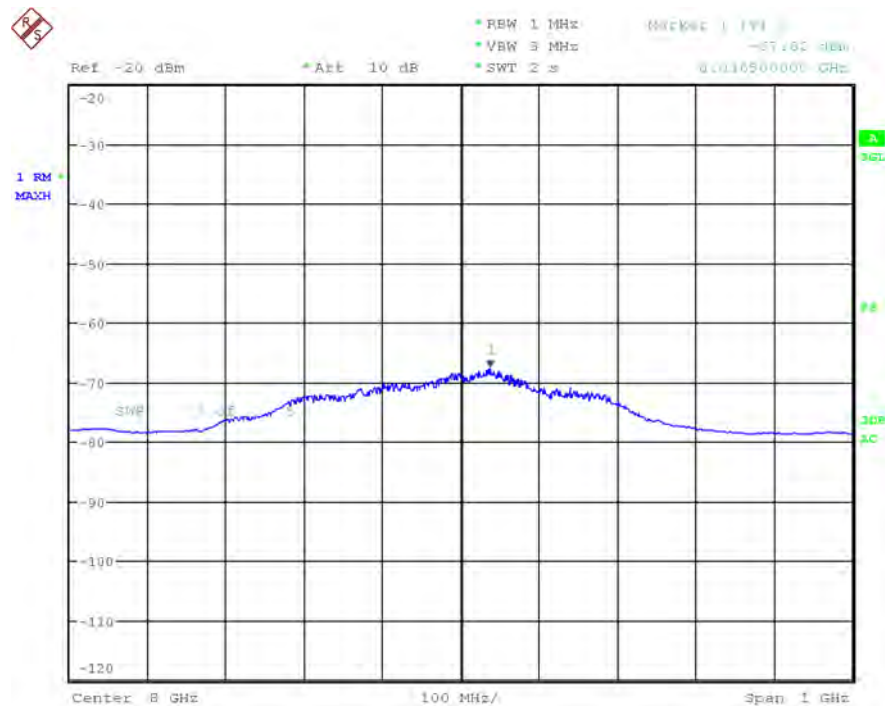
Plot 7-94. UWB Peak Power Measurement - ANT 1 - CH.9 – SP1 – HPRF
