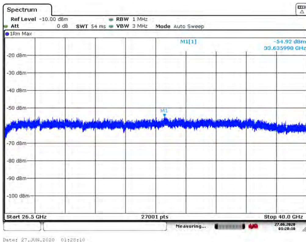
Plot 7-116. Radiated Spurious Pre-Scan 26.5 – 40.0 GHz - CH.5 - ANT 1
