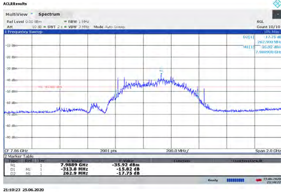
Plot 7-55. BANDWIDTH Plot – ANT1 - CH.9 - SP0 – Preamble 27
