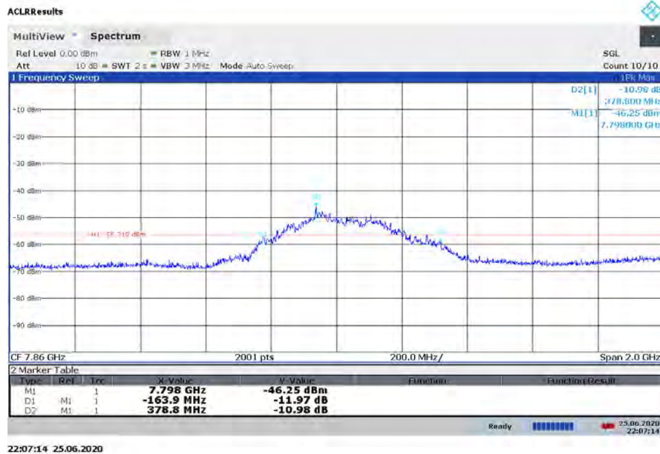
Plot 7-52. BANDWIDTH Plot 7-- ANT2 - CH.9 - SP0 – Preamble 12
