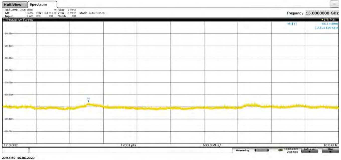
Plot 7-128. Radiated Spurious Pre-Scan 12000 - 18000 MHz - CH.9 - ANT 1
