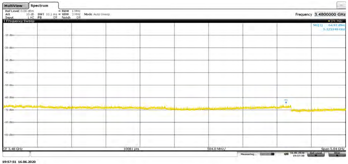
Plot 7-110. Radiated Spurious Pre-Scan 960 - 6000 MHz - CH.5 - ANT 1
