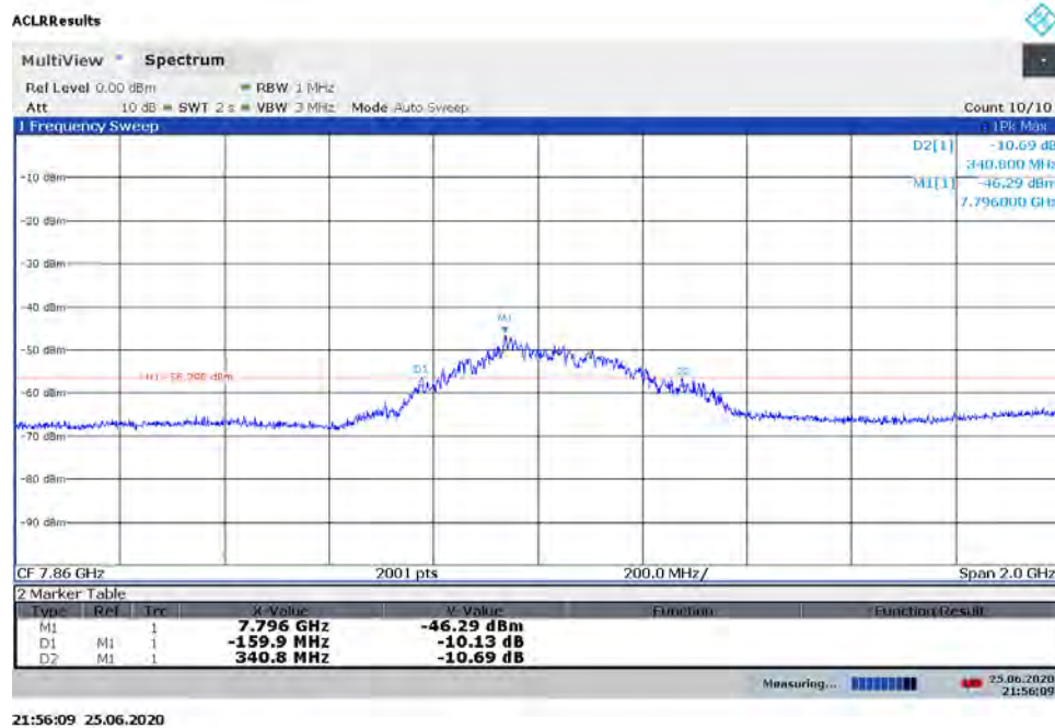
Plot 7-54. BANDWIDTH Plot – ANT2 - CH.9 – SP3 – Preamble 12
