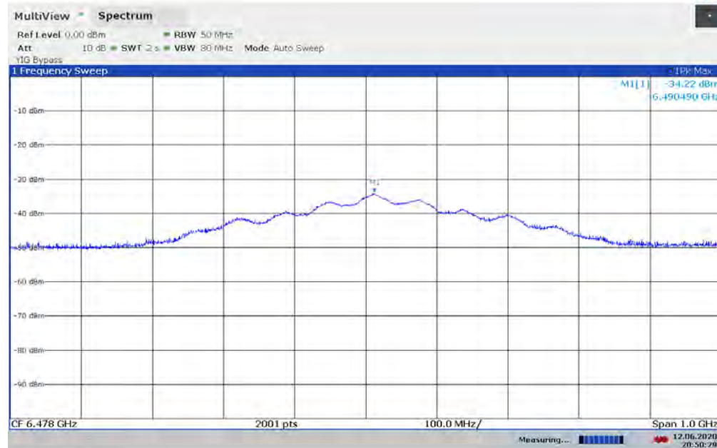
Plot 7-90. UWB Peak Power Measurement - ANT 1 - CH.5 – SP3 – HPRF
