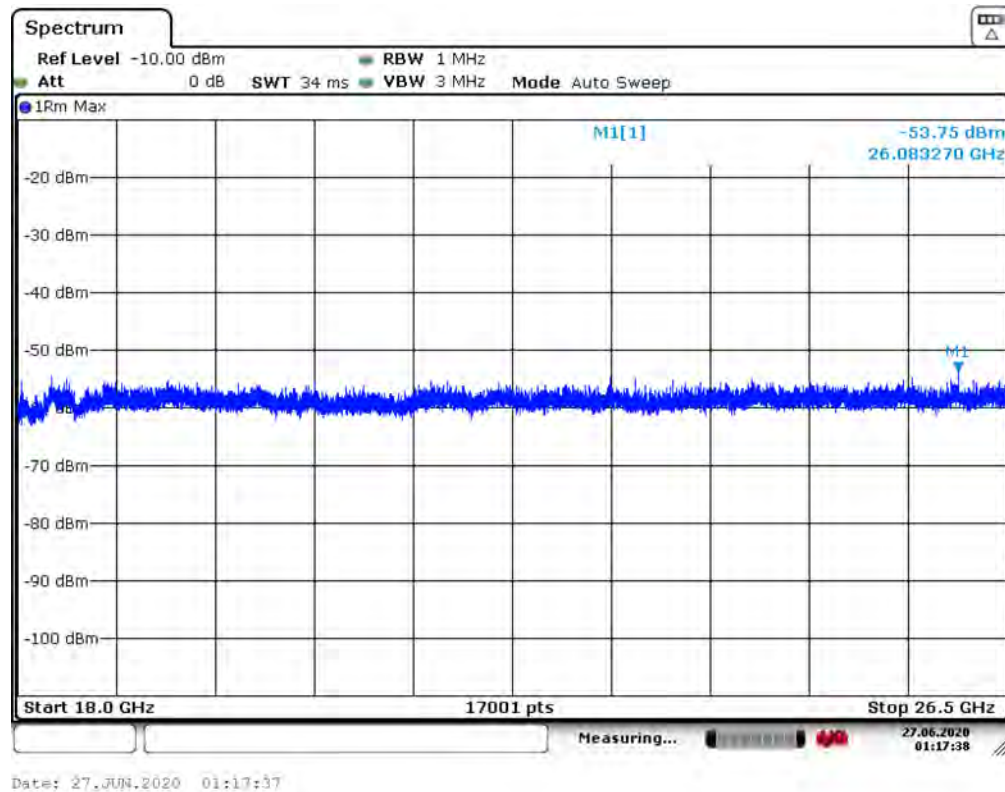
Plot 7-136. Radiated Spurious Pre-Scan 18 - 26.5 GHz - CH.9 - ANT 2
