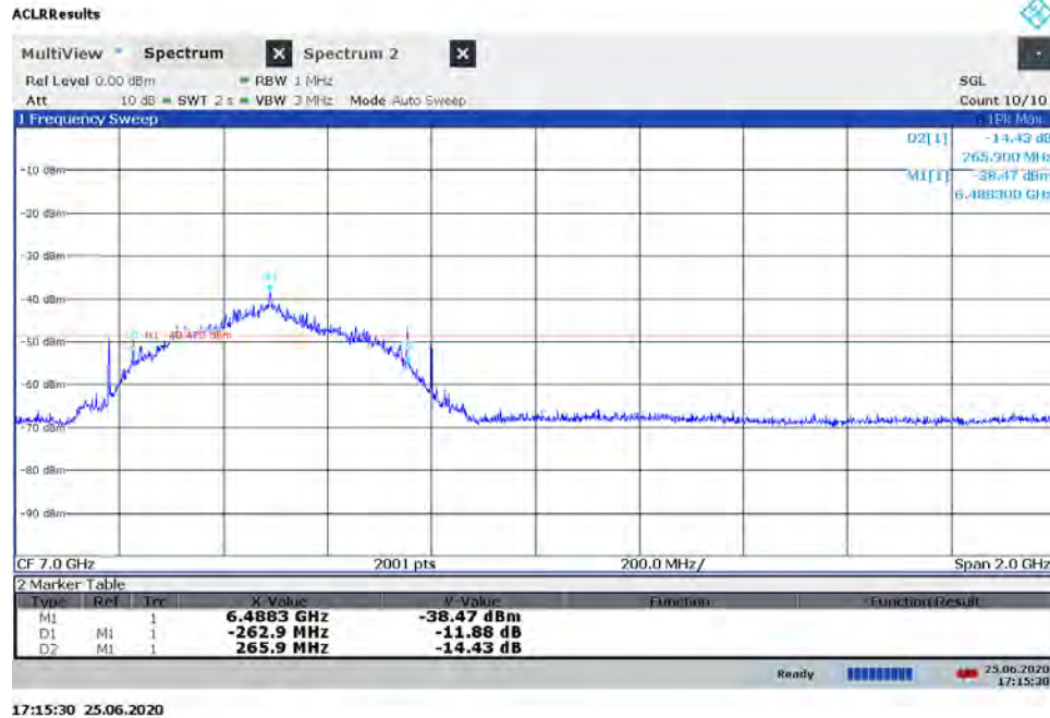
Plot 7-25. BANDWIDTH Plot – ANT1 - CH.5 - SP0 – Preamble 27
