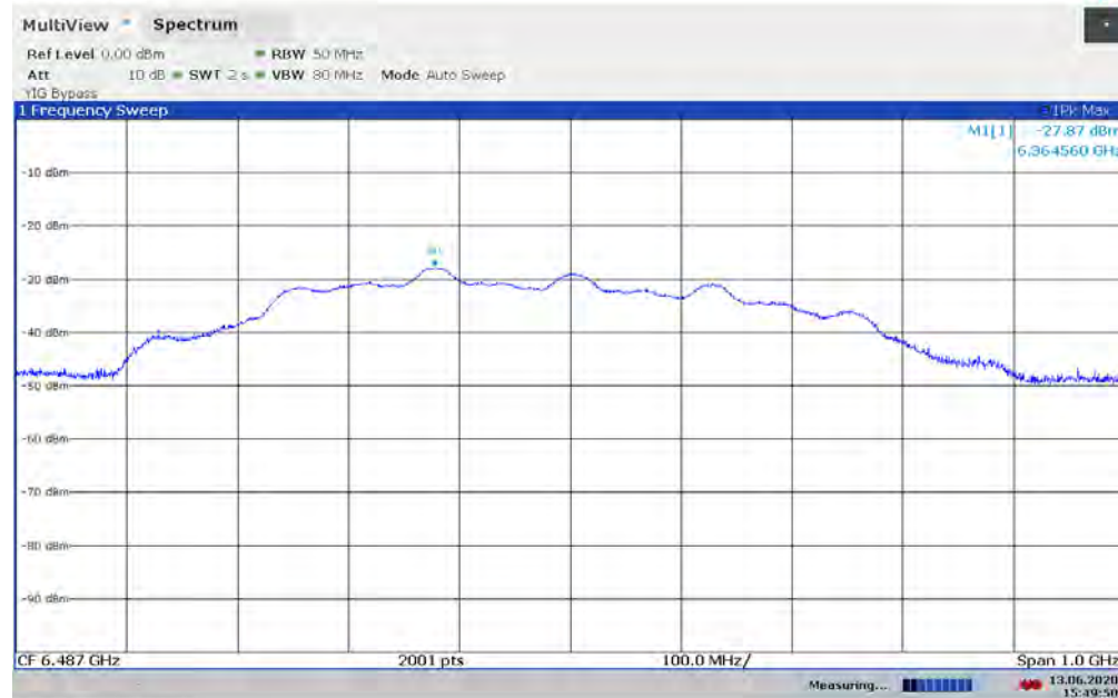
Plot 7-98. UWB Peak Power Measurement - ANT 2 - CH.5 - SP0 – HPRF
