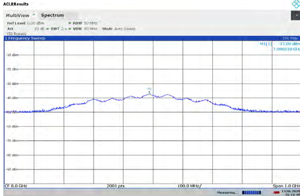
Plot 7-96. UWB Peak Power Measurement - ANT 1 - CH.9 – SP3 – HPRF
