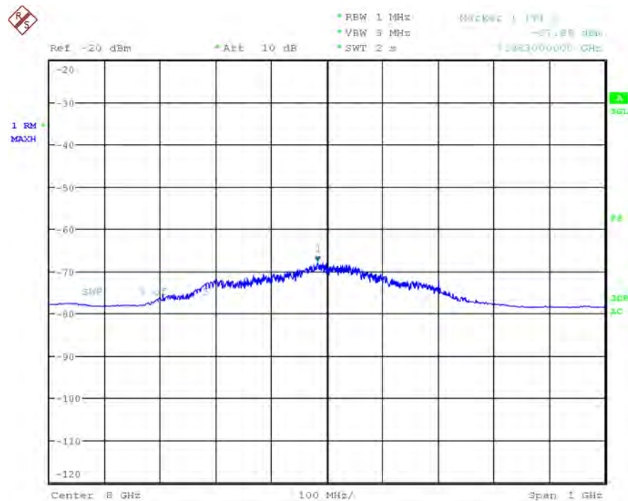
Plot 7-104. UWB Peak Power Measurement - ANT 2 - CH.9 - SP0 - HPRF
