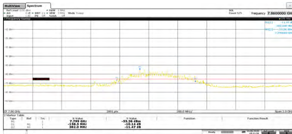
Plot 7-39. BANDWIDTH Plot - ANT1 - CH.9 – SP3 – Preamble 10
