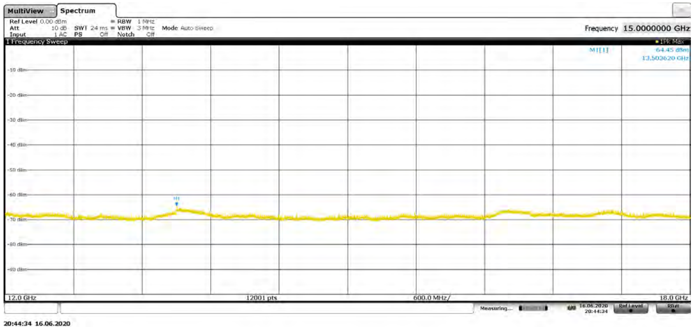
Plot 7-121. Radiated Spurious Pre-Scan 12000 - 18000 MHz - CH.5 - ANT 2
