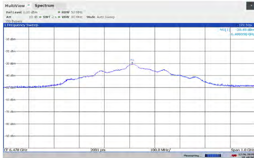
Plot 7-88. UWB Peak Power Measurement - ANT 1 - CH.5 – SP1 – HPRF
