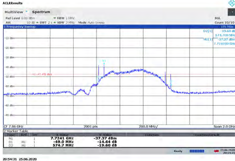
Plot 7-51. BANDWIDTH Plot 7-- ANT1 - CH.9 – SP3 – Preamble 12
