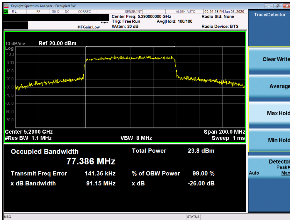
Plot 7-24. 26dB Bandwidth Plot SISO ANT1 (80MHz BW 802.11ax (UNII Band 2A) – Ch. 58)
