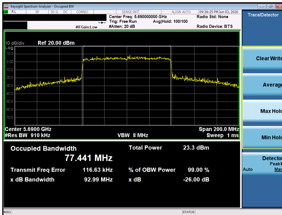
Plot 7-45. 26dB Bandwidth Plot SISO ANT1 (80MHz BW 802.11ax (UNII Band 2C) - Ch. 138)
