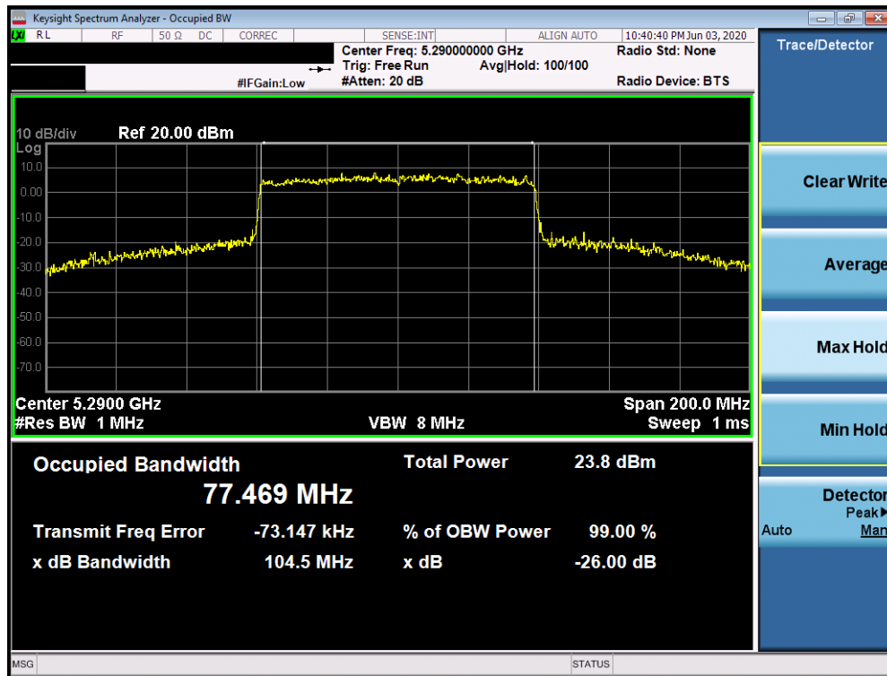
Plot 7-75. 26dB Bandwidth Plot SISO ANT2 (80MHz BW 802.11ax (UNII Band 2A) – Ch. 58)
