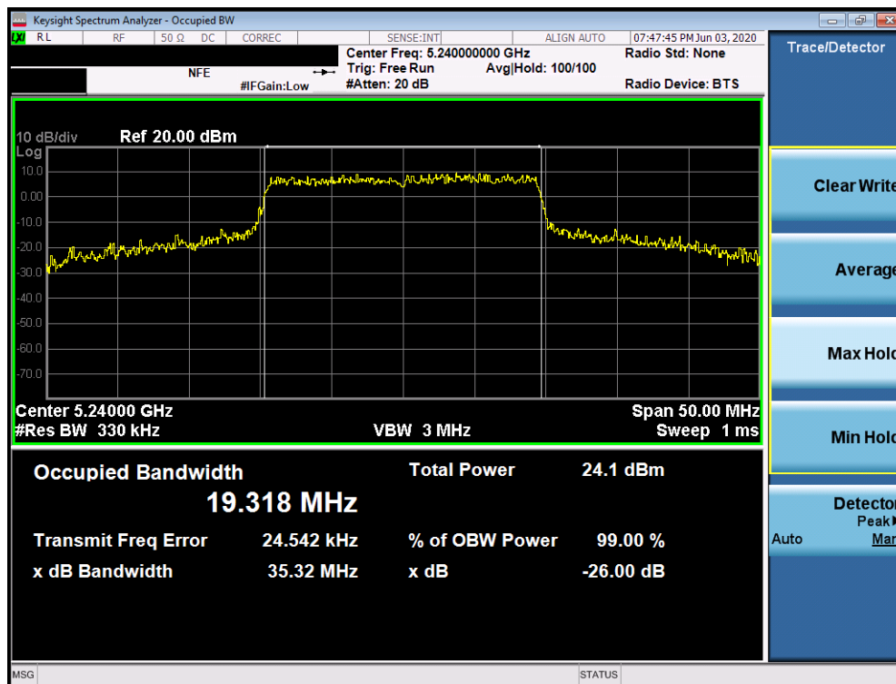
Plot 7-4. 26dB Bandwidth Plot SISO ANT1 (20MHz BW 802.11ax (UNII Band 1) – Ch. 48)
