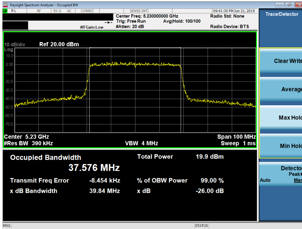
Plot 7-58. 26dB Bandwidth Plot SISO ANT2 (40MHz BW 802.11ax (UNII Band 1) – Ch. 46)
