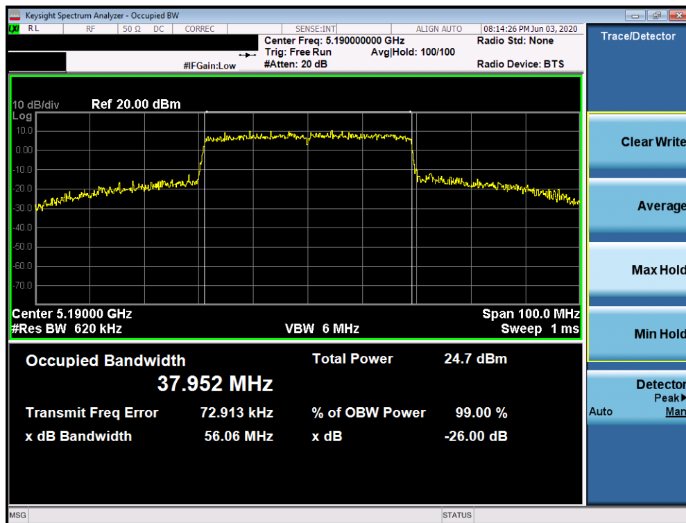
Plot 7-9. 26dB Bandwidth Plot SISO ANT1 (40MHz BW 802.11ax (UNII Band 1) – Ch. 38)
