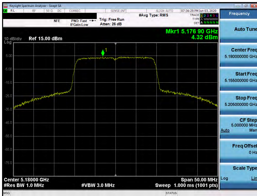
Plot 7-133. Power Spectral Density Plot SISO ANT1 (20MHz BW 802.11ax (UNII Band 1) – Ch. 36)
