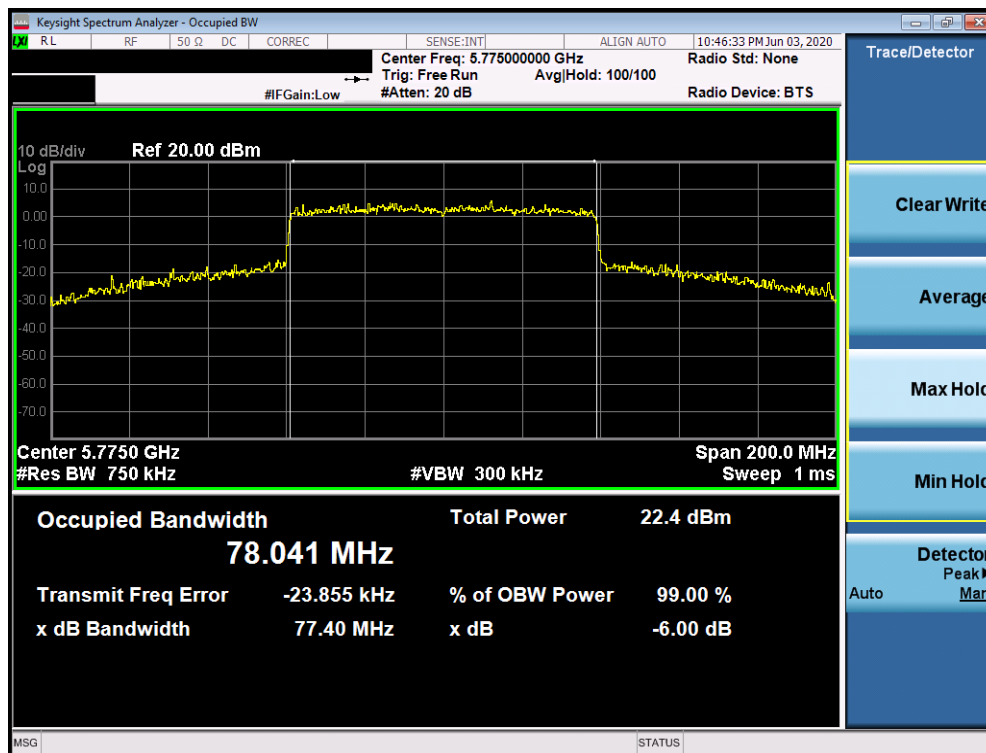
Plot 7-126. 6dB Bandwidth Plot SISO ANT2 (80MHz BW 802.11ax (UNII Band 3) – Ch. 155)
