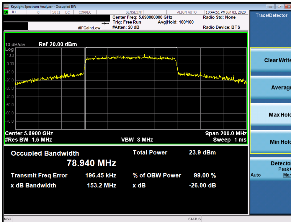
Plot 7-96. 26dB Bandwidth Plot SISO ANT2 (80MHz BW 802.11ax (UNII Band 2C) – Ch. 138)
