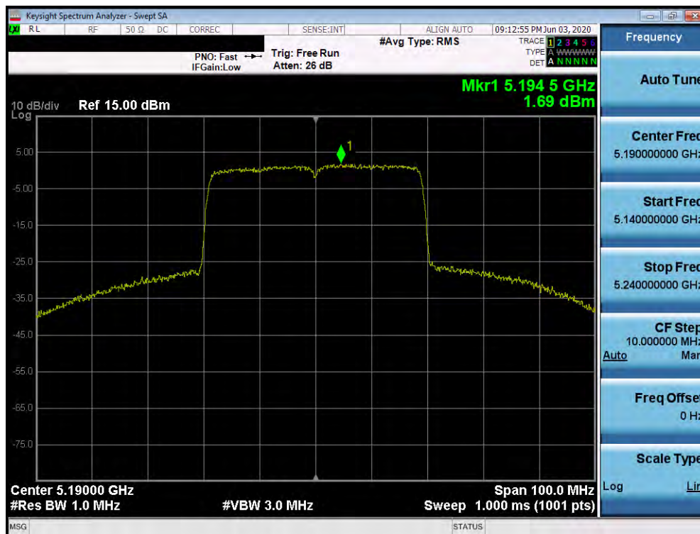
Plot 7-138. Power Spectral Density Plot SISO ANT1 (40MHz BW 802.11ax (UNII Band 1) – Ch. 38)
