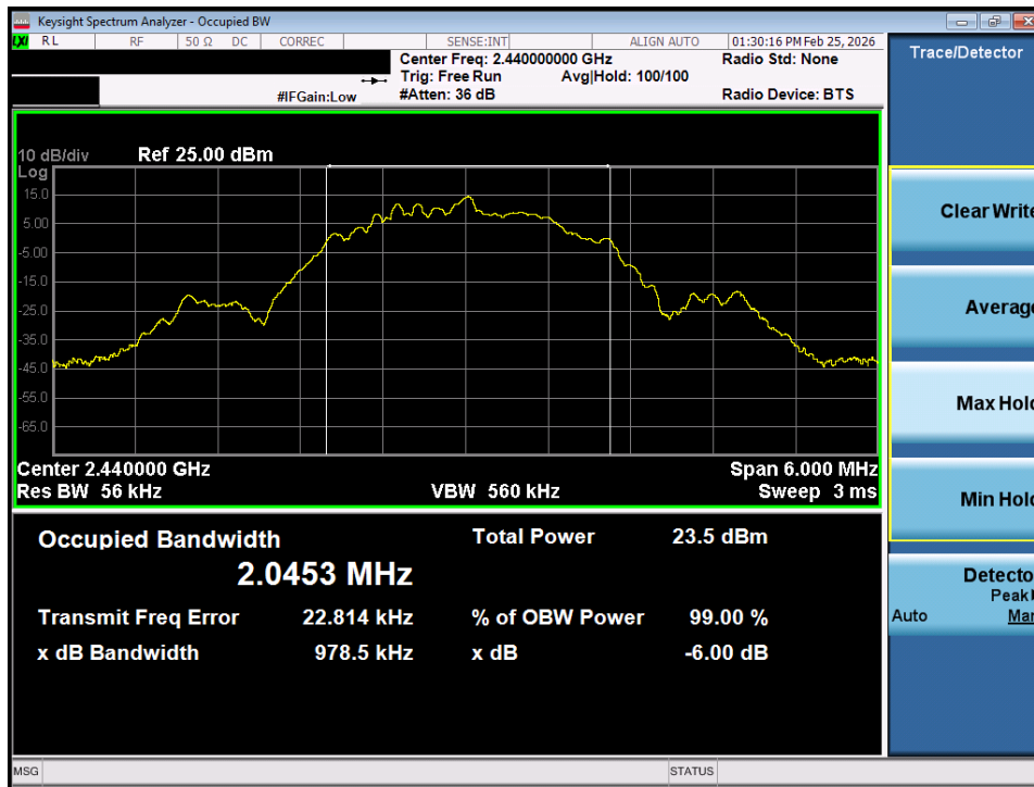
Plot 7-23. OBW Plot (Bluetooth (LE), 2Mbps – Ch. 17) – SISO ANT1
