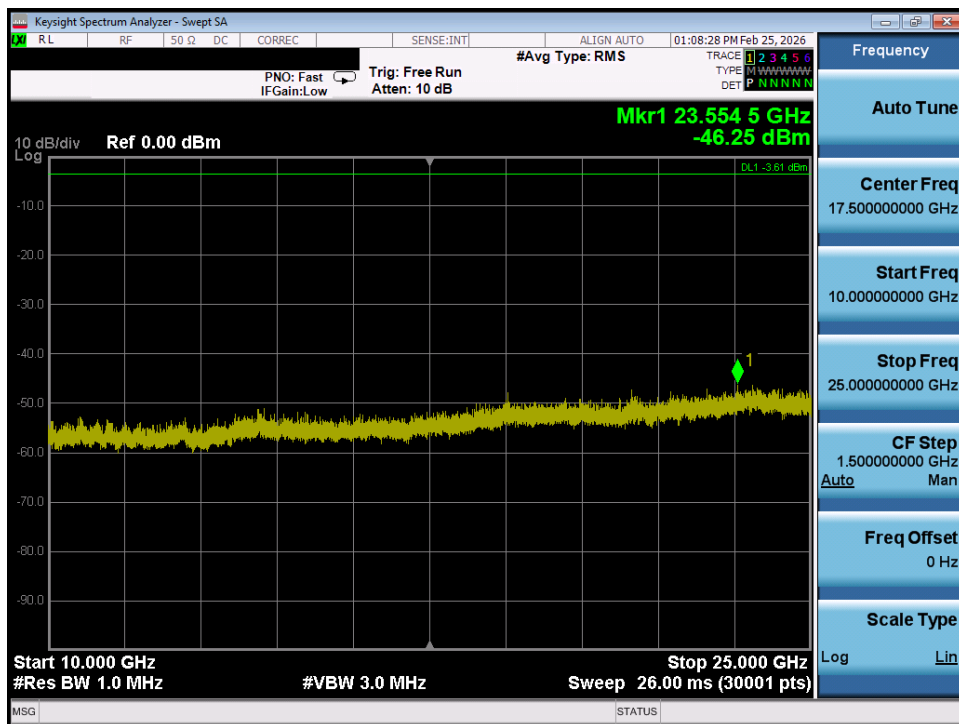
Plot 7-60. Conducted Spurious Plot (Bluetooth (LE), 1Mbps – Ch. 17) – Ant 1
