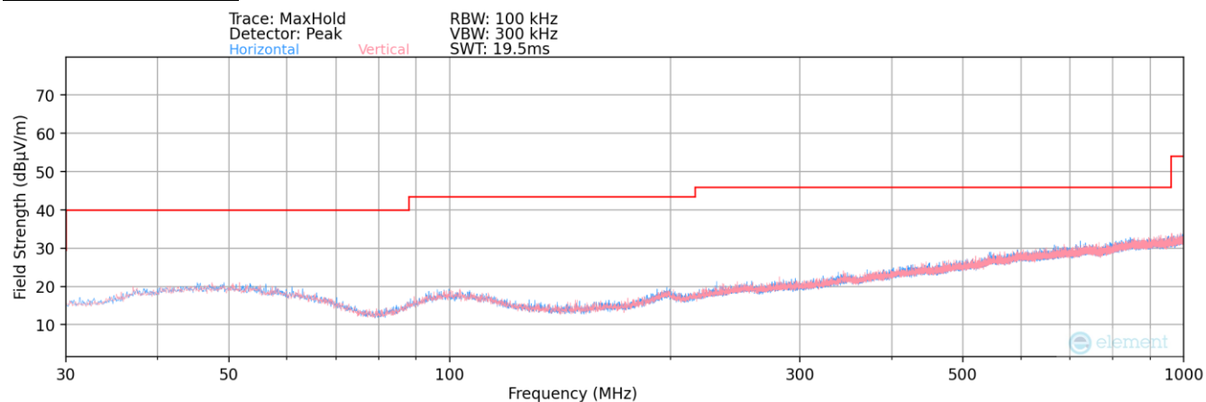
Plot 7-69. Radiated Spurious Plot below 1GHz – Ant 1
