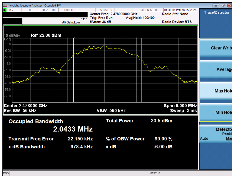
Plot 7-24. OBW Plot (Bluetooth (LE), 2Mbps – Ch. 36) – SISO ANT1
