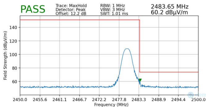
Plot 7-68. Radiated Restricted Upper Band Edge Measurement (Peak) – Ant 1
