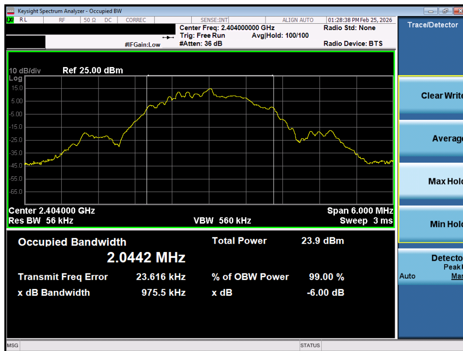
Plot 7-22. OBW Plot (Bluetooth (LE), 2Mbps – Ch. 0) – SISO ANT1
