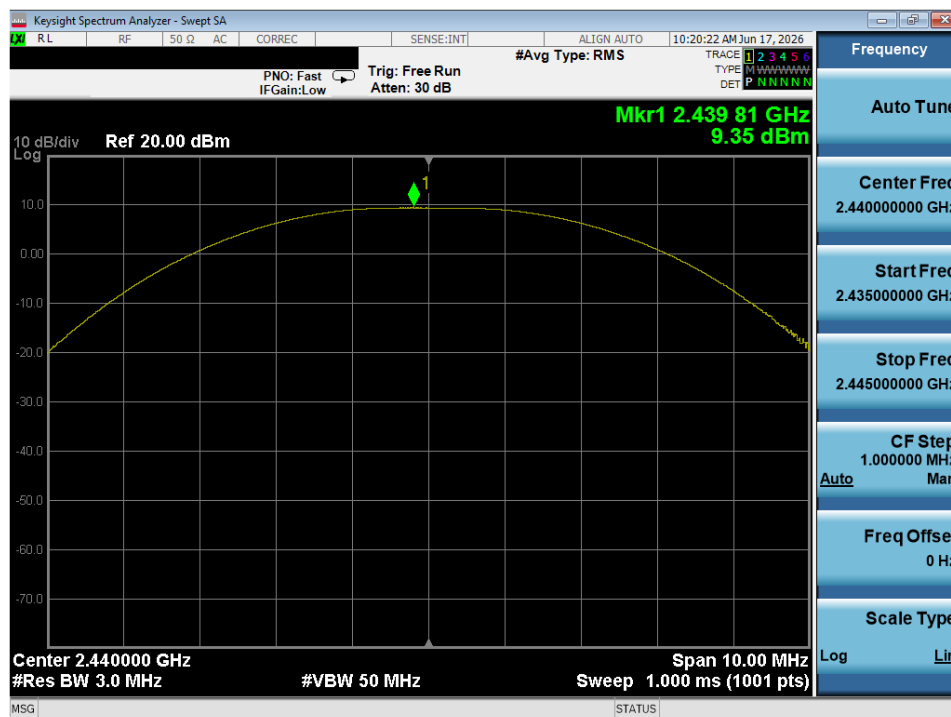
Plot 9-2. Peak Conducted Power(Spot-check)
