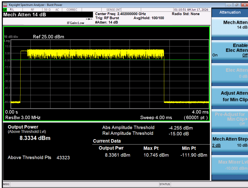
Plot 7-22. Average Conducted Power (2Mbps - Ch. 0) - SISO ANT 1
