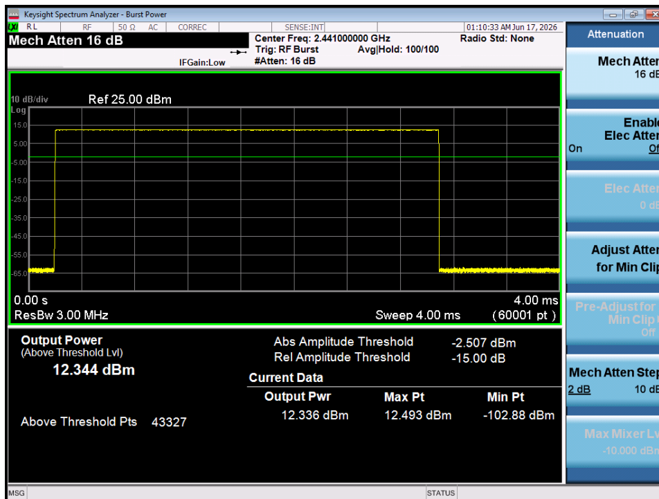
Plot 7-20. Average Conducted Power (1Mbps - Ch. 39) - SISO ANT 1
