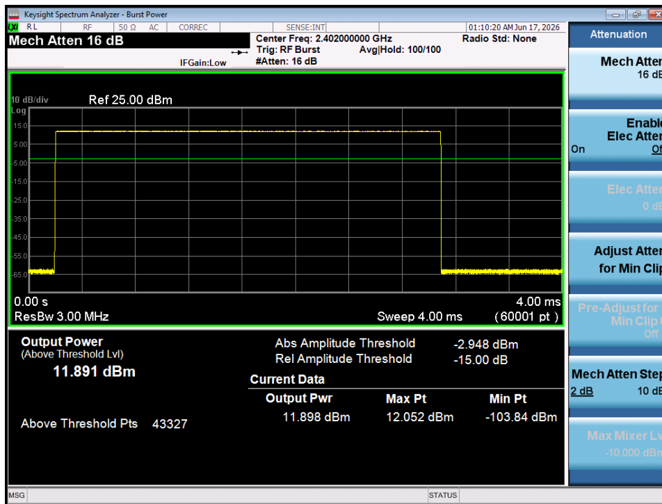
Plot 7-19. Average Conducted Power (1Mbps - Ch. 0) - SISO ANT 1
