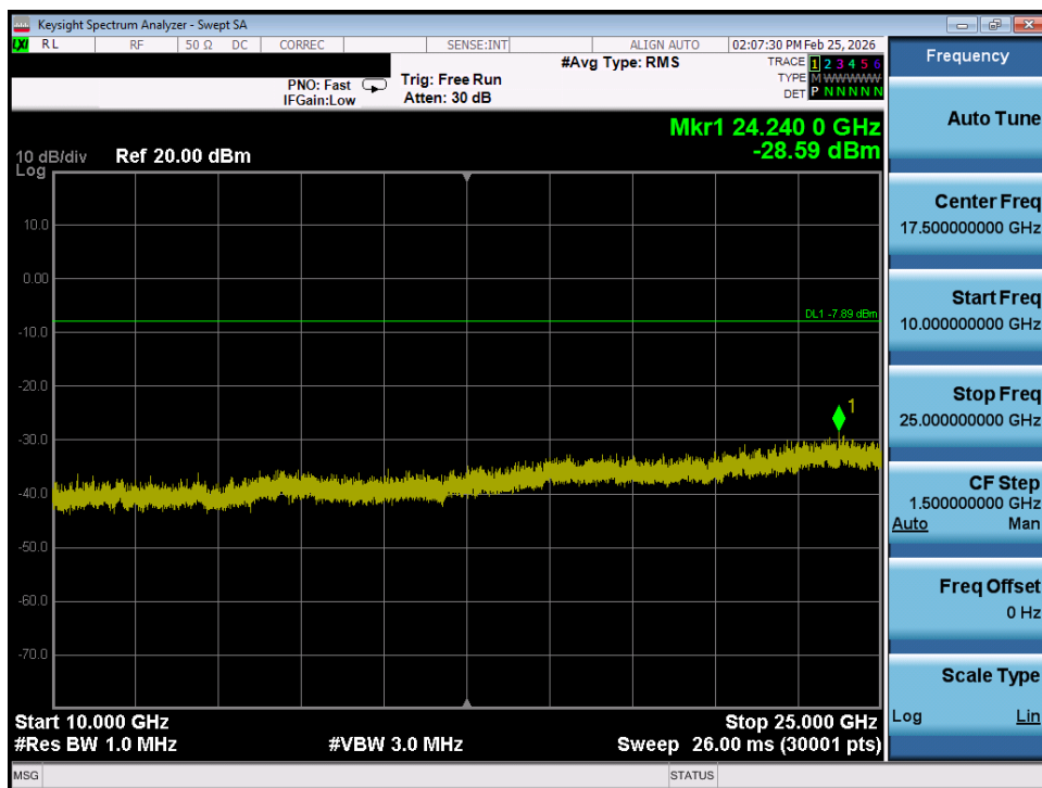
Plot 7-39. Conducted Spurious Plot (Bluetooth, 3Mbps – Ch. 39) – SISO ANT 1
