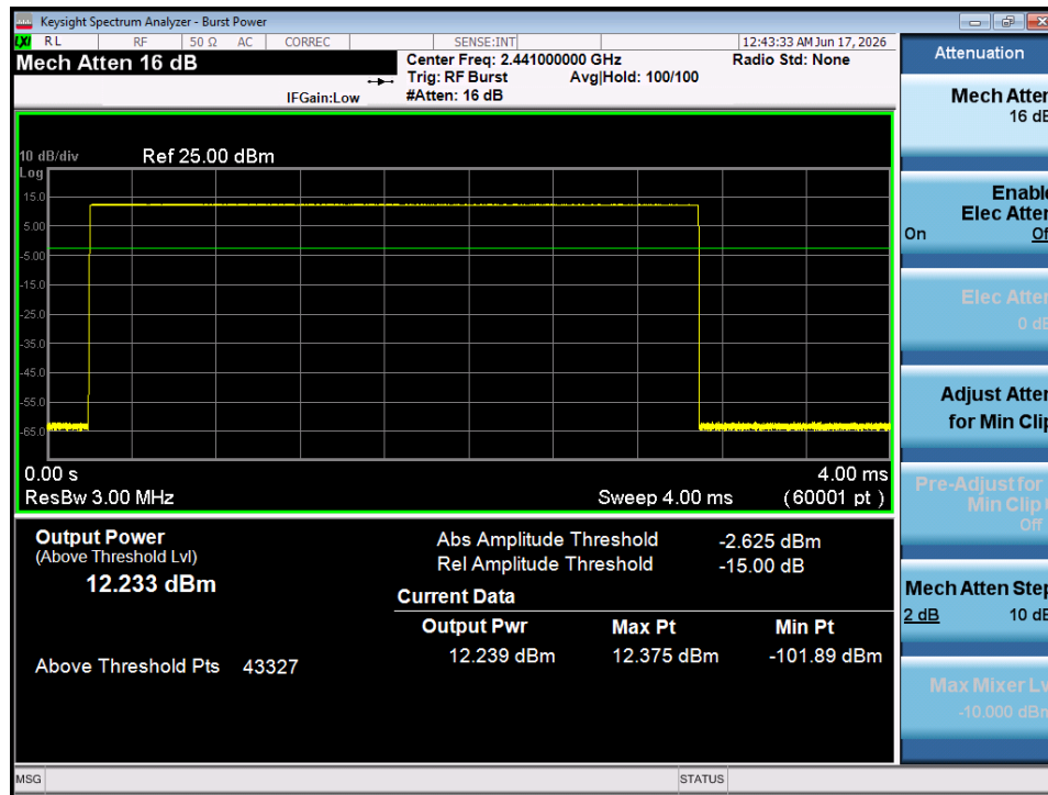
Plot 9-2. Average Conducted Power(Spot-check)
