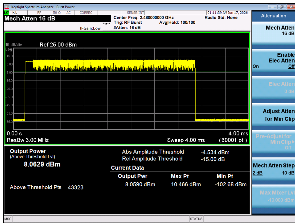
Plot 7-24. Average Conducted Power (2Mbps - Ch. 78) - SISO ANT 1
