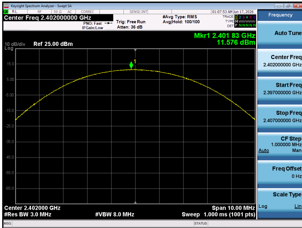
Plot 7-16. Peak Conducted Power (3Mbps – Ch. 0) – SISO ANT 1
