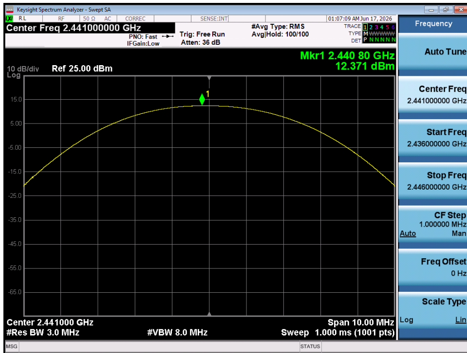
Plot 7-11. Peak Conducted Power (1Mbps – Ch. 39) – SISO ANT 1
