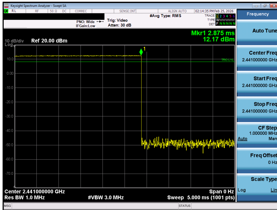
Plot 7-33. Time of Occupancy Plot (Bluetooth) – SISO Ant 1
