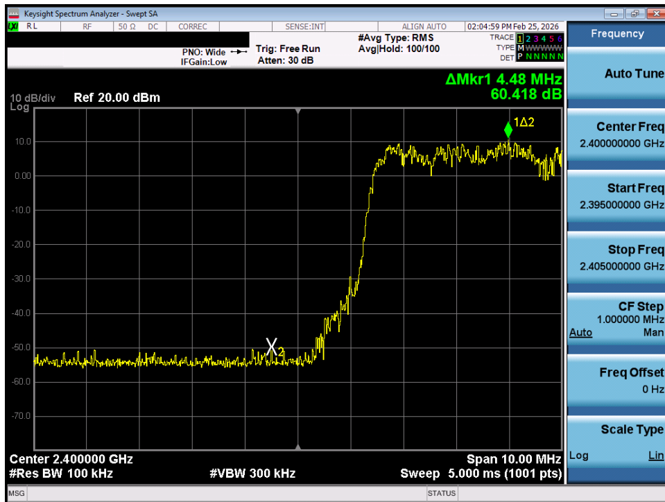
Plot 7-30. Band Edge Plot (Bluetooth with Hopping Enabled, 3 Mbps) – SISO ANT 1
