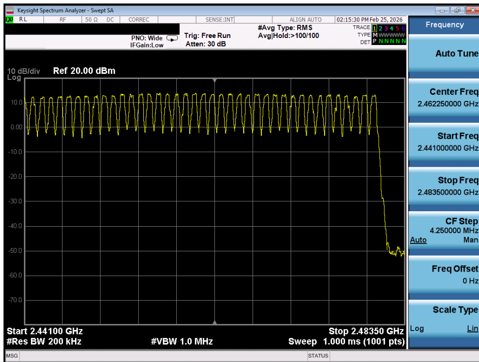
Plot 7-35. High End Spectrum Channel Hopping Plot (Bluetooth) – SISO Ant 1
