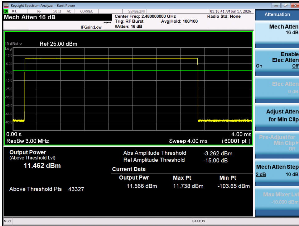
Plot 7-21. Average Conducted Power (1Mbps - Ch. 78) - SISO ANT 1
