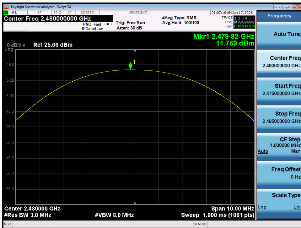
Plot 7-12. Peak Conducted Power (1Mbps – Ch. 78) – SISO ANT 1
