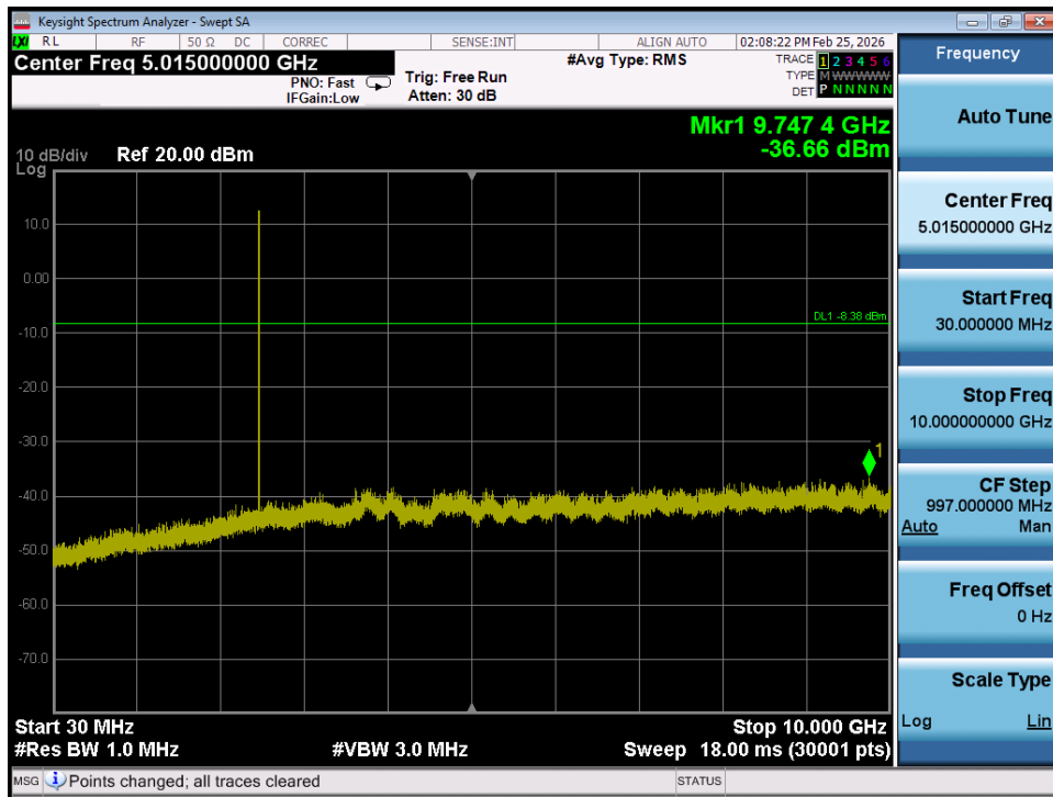
Plot 7-40. Conducted Spurious Plot (Bluetooth, 3Mbps – Ch. 78) – SISO ANT 1
