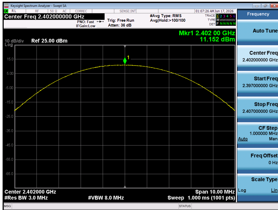
Plot 7-13. Peak Conducted Power (2Mbps – Ch. 0) – SISO ANT 1
