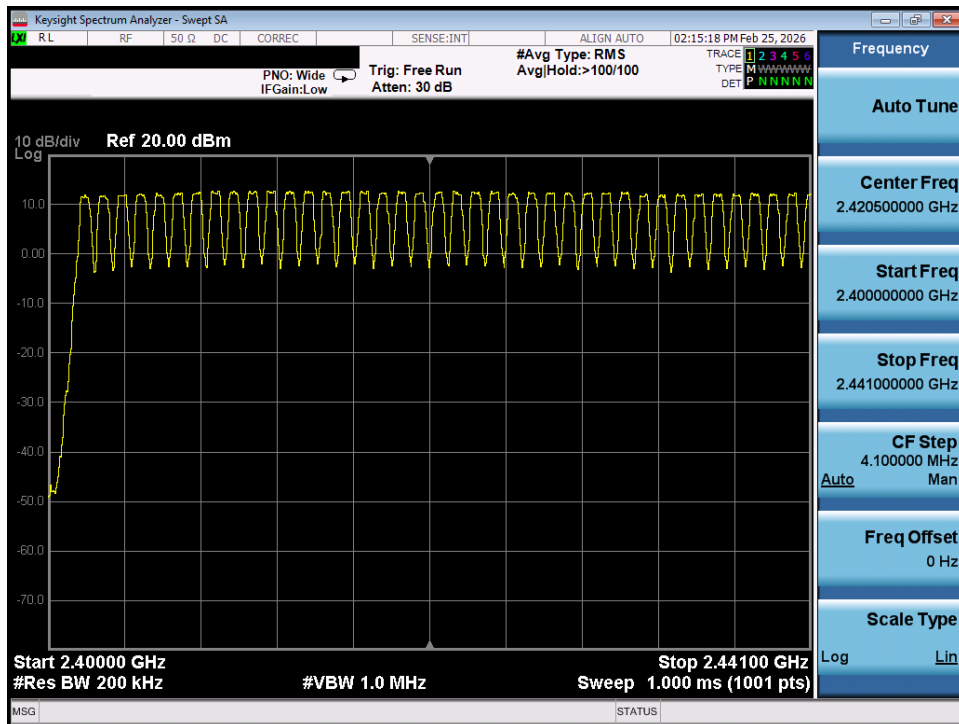
Plot 7-34. Low End Spectrum Channel Hopping Plot (Bluetooth) – SISO Ant 1
