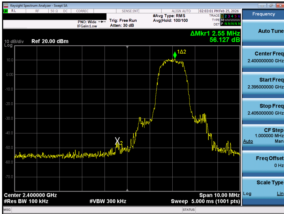
Plot 7-28. Band Edge Plot (Bluetooth with Hopping Disabled, 3 Mbps – Ch. 0) – SISO ANT 1
