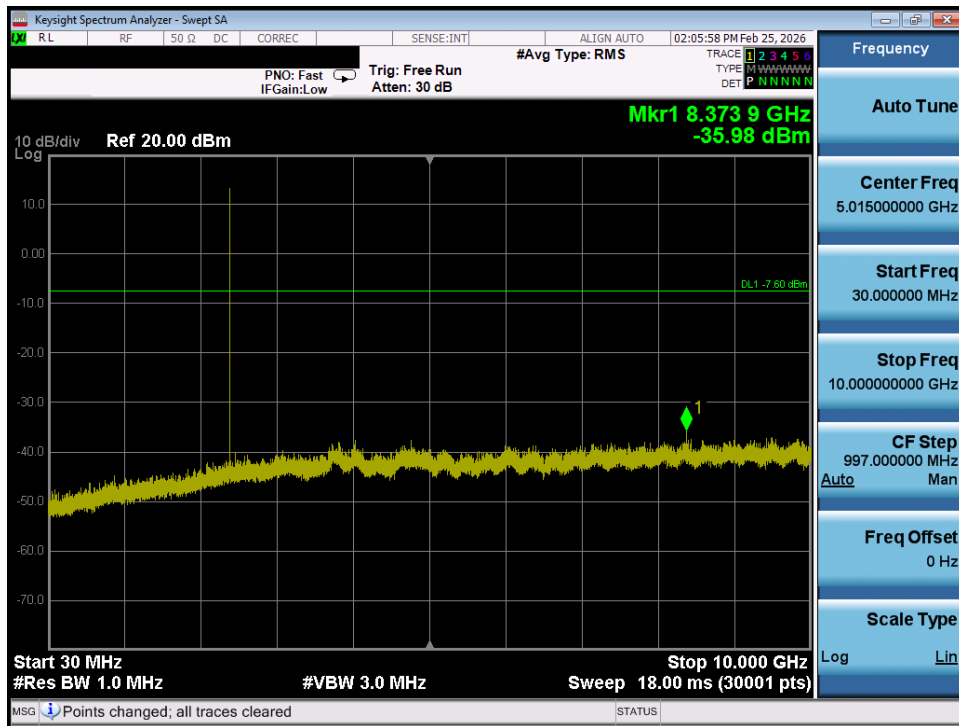
Plot 7-36. Conducted Spurious Plot (Bluetooth, 3Mbps – Ch. 0) – SISO ANT 1
