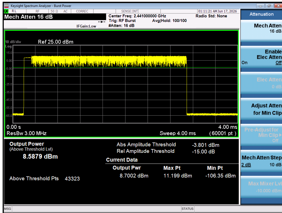
Plot 7-23. Average Conducted Power (2Mbps - Ch. 39) - SISO ANT 1
