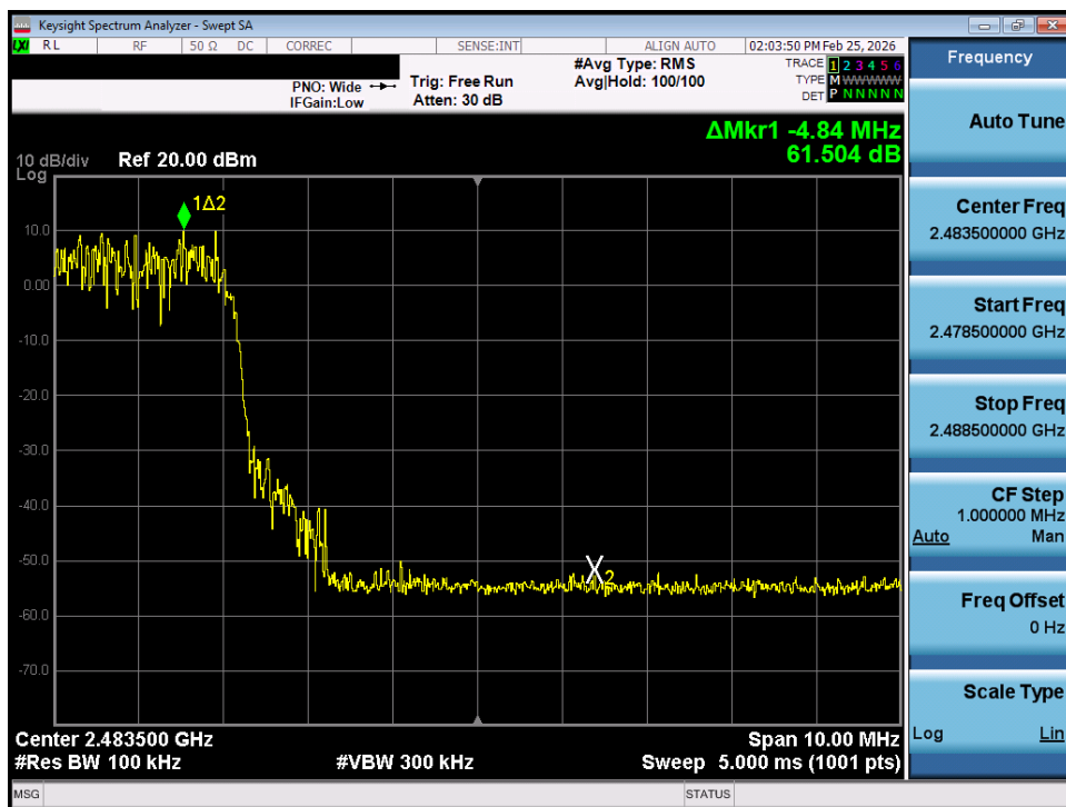
Plot 7-31. Band Edge Plot (Bluetooth with Hopping Enabled, 3 Mbps) – SISO ANT 1
