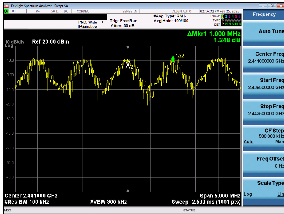
Plot 7-32. Channel Spacing Plot (Bluetooth) – SISO Ant 1
