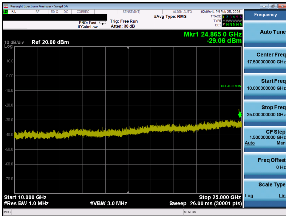
Plot 7-41. Conducted Spurious Plot (Bluetooth, 3Mbps – Ch. 78) – SISO ANT 1
