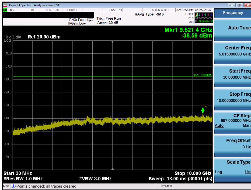
Plot 7-38. Conducted Spurious Plot (Bluetooth, 3Mbps – Ch. 39) – SISO ANT 1
