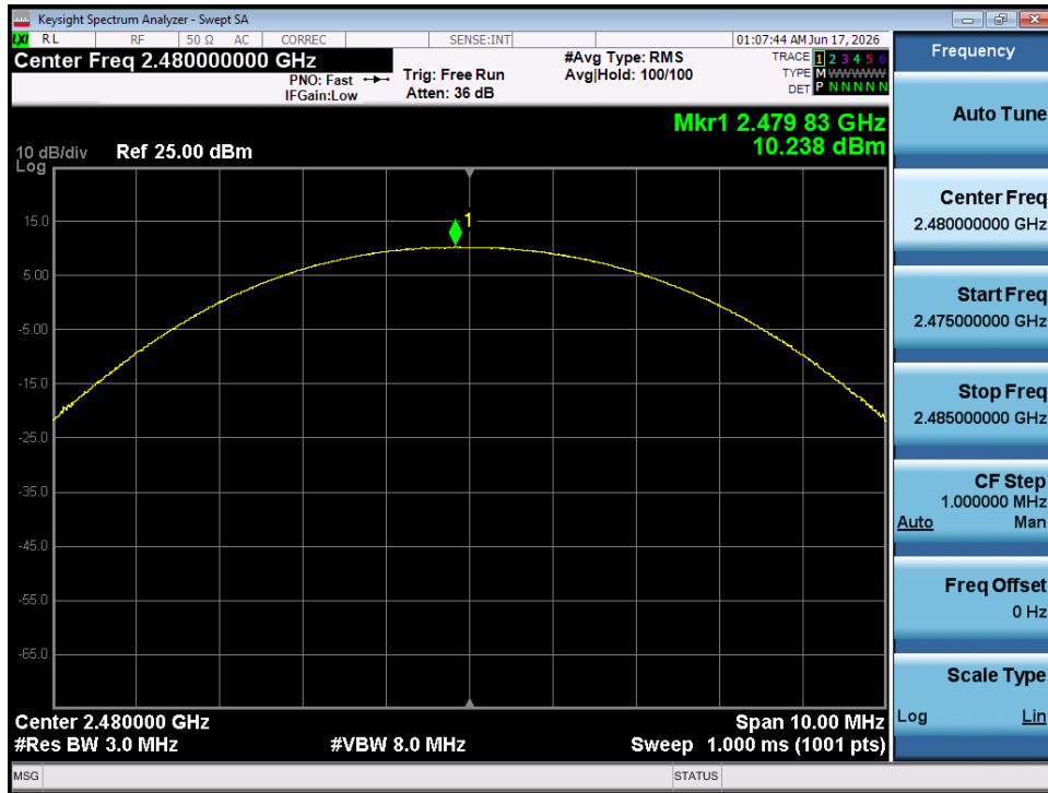
Plot 7-15. Peak Conducted Power (2Mbps – Ch. 78) – SISO ANT 1
