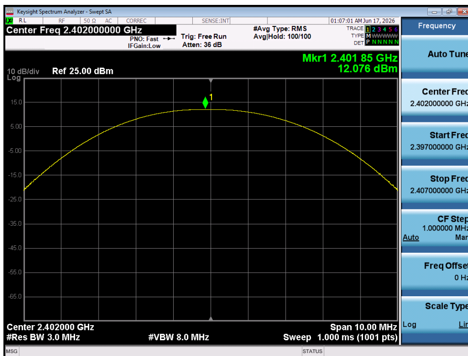
Plot 7-10. Peak Conducted Power (1Mbps – Ch. 0) – SISO ANT 1
