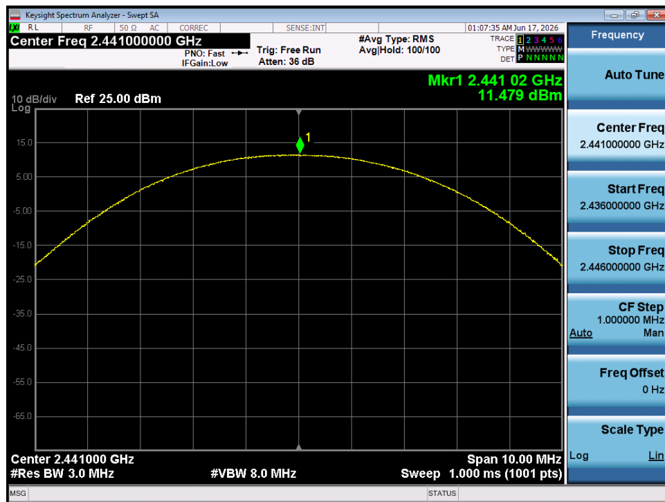
Plot 7-14. Peak Conducted Power (2Mbps – Ch. 39) – SISO ANT 1
