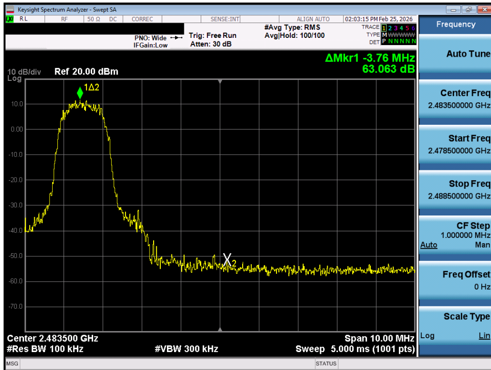
Plot 7-29. Band Edge Plot (Bluetooth with Hopping Disabled, 3 Mbps – Ch. 78) – SISO ANT 1
