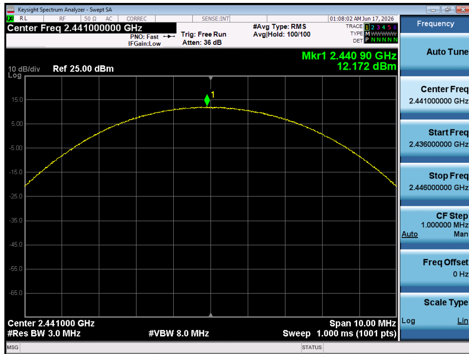
Plot 7-17. Peak Conducted Power (3Mbps – Ch. 39) – SISO ANT 1
