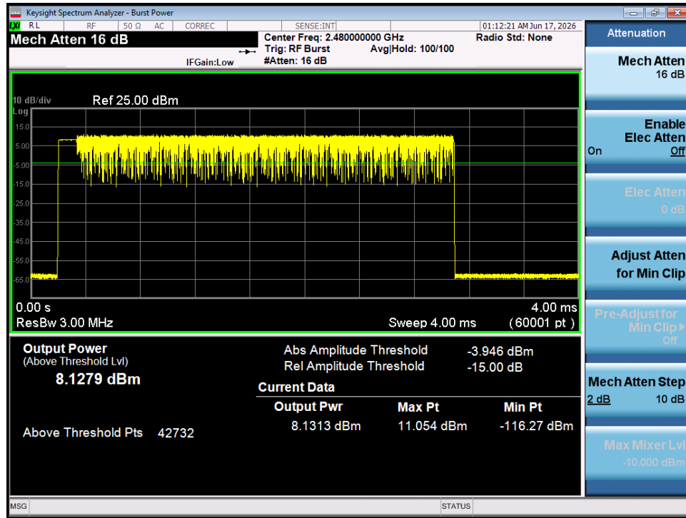
Plot 7-27. Average Conducted Power (3Mbps – Ch. 78) – SISO ANT 1
