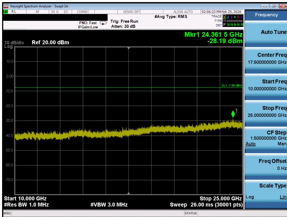
Plot 7-37. Conducted Spurious Plot (Bluetooth, 3Mbps – Ch. 0) – SISO ANT 1
