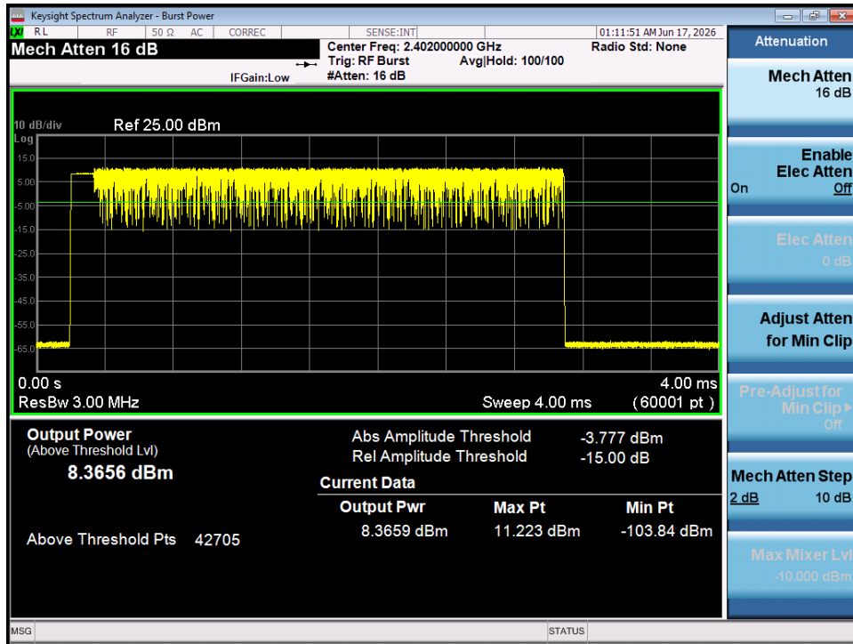
Plot 7-25. Average Conducted Power (3Mbps - Ch. 0) - SISO ANT 1
