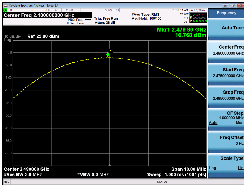
Plot 7-18. Peak Conducted Power (3Mbps – Ch. 78) – SISO ANT 1
