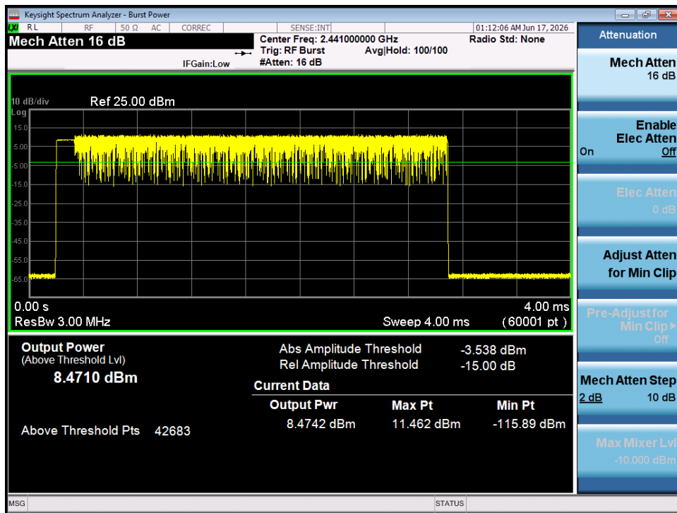
Plot 7-26. Average Conducted Power (3Mbps - Ch. 39) - SISO ANT 1
