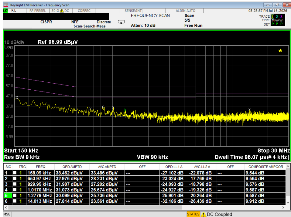
Plot 7-19. Line Conducted Plot (N) – File Transfer – SM-O200J
