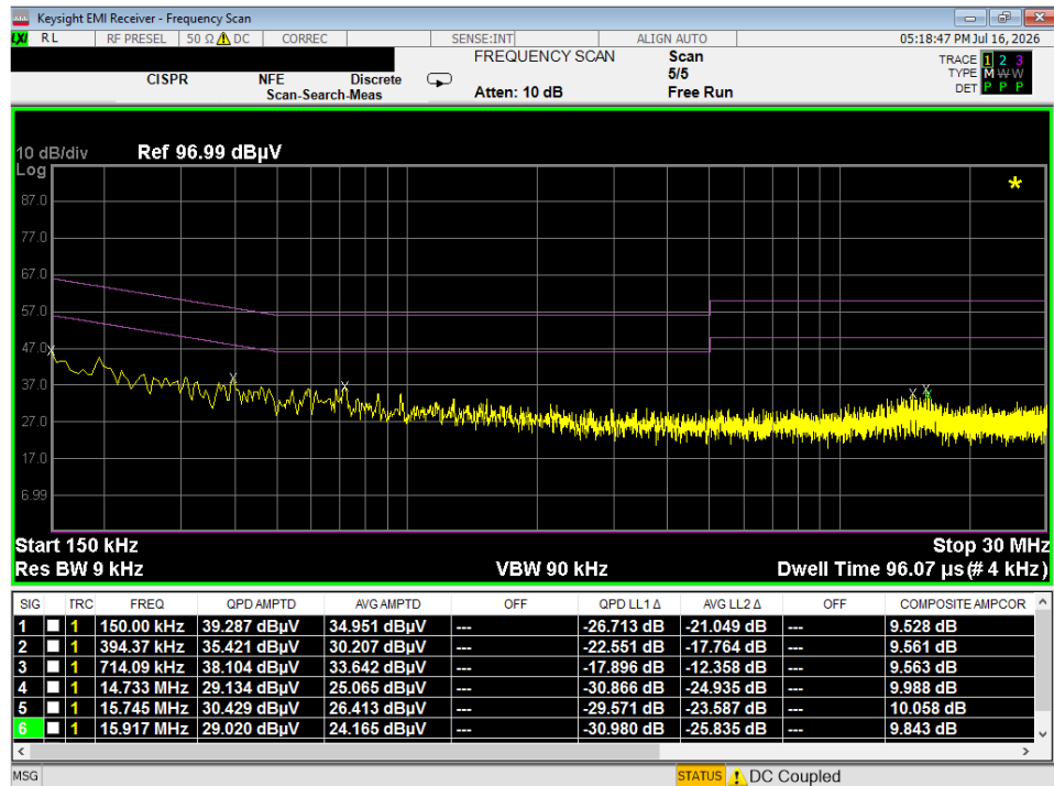
Plot 7-17. Line Conducted Plot (N) – Audio Playback – SM-O200J
