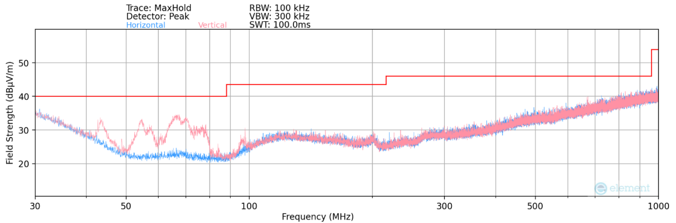
Plot 7-13. Radiated Emissions 30MHz – 1GHz
