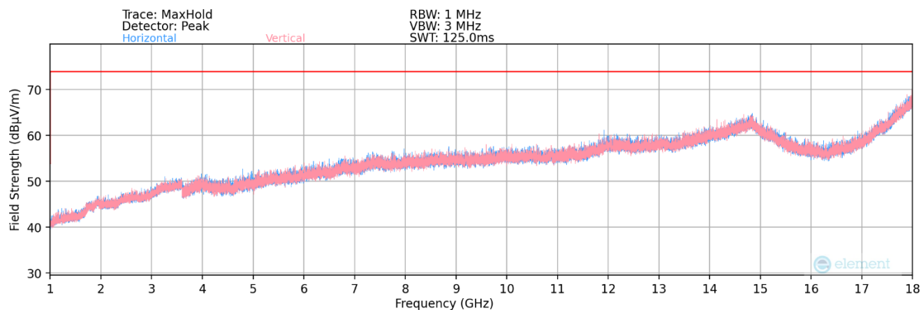
Plot 7-8. Radiated Emissions 1GHz – 18GHz
