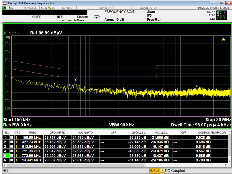
Plot 7-16. Line Conducted Plot (L1) – Audio Playback – SM-O200J
