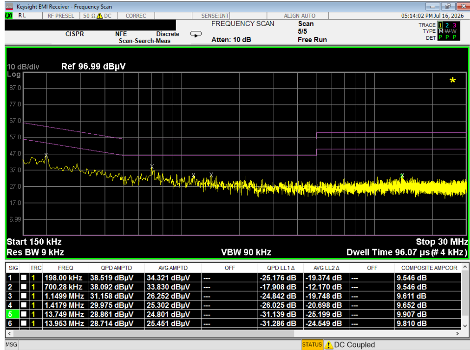
Plot 7-14. Line Conducted Plot (L1) – Video Recording – SM-O200J
