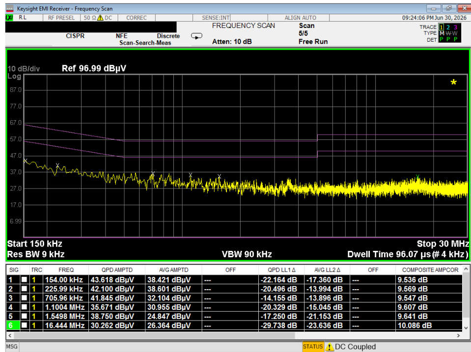
Plot 7-21. Line Conducted Plot (N) – Charging Case – SM-O200J
