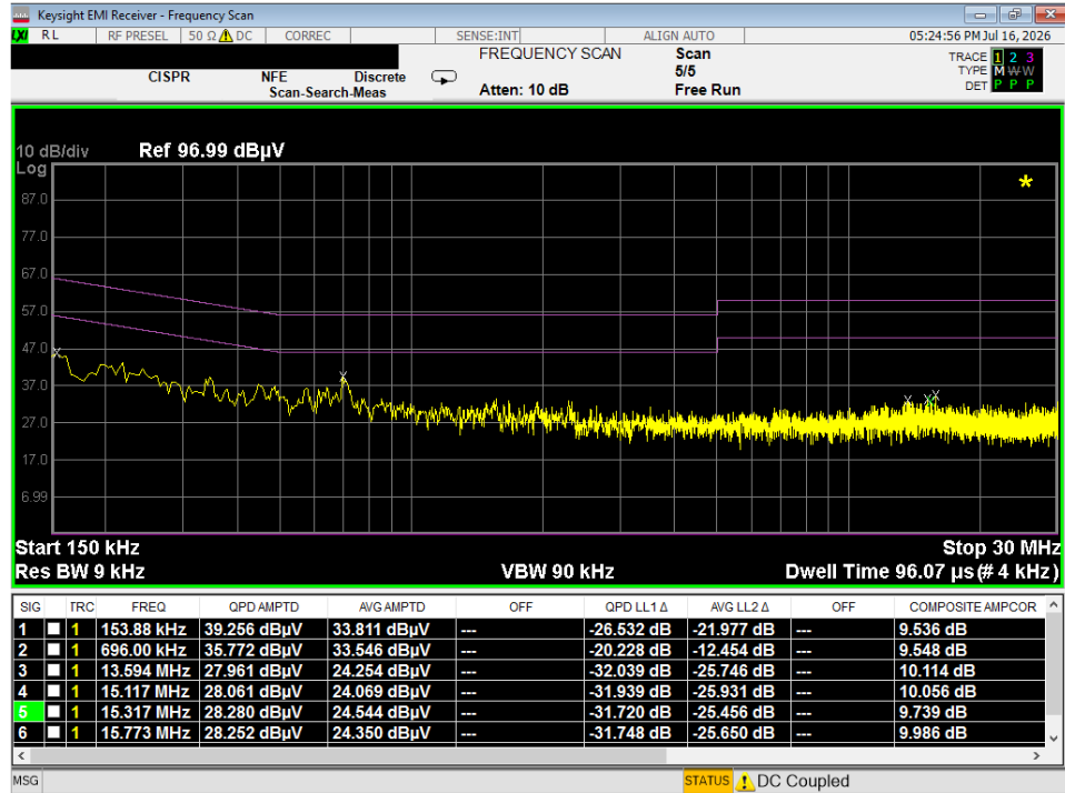
Plot 7-18. Line Conducted Plot (L1) – File Transfer – SM-O200J
