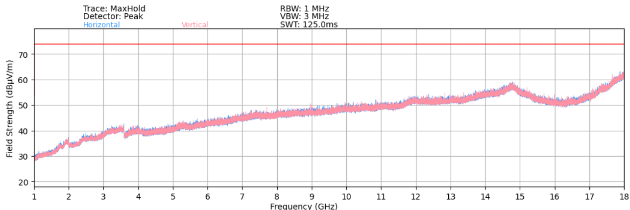
Plot 7-6. Radiated Emissions 1GHz – 18GHz
