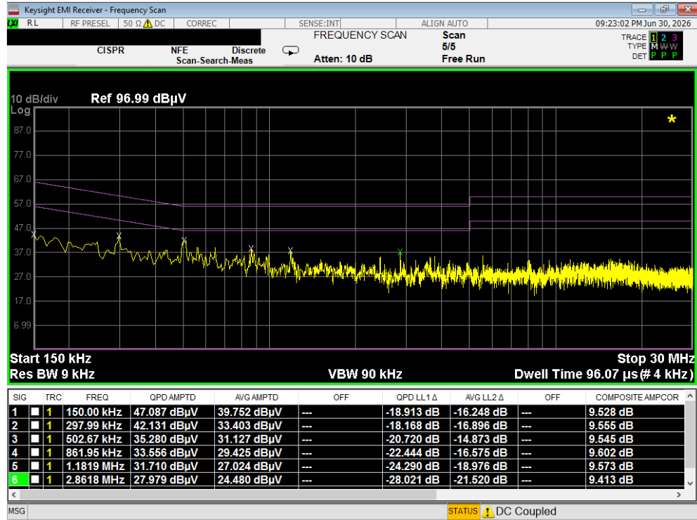
Plot 7-20. Line Conducted Plot (L1) – Charging Case – SM-O200J
