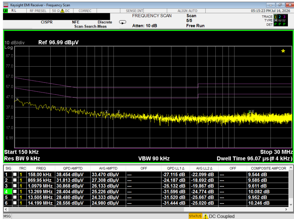
Plot 7-15. Line Conducted Plot (N) – Video Recording – SM-O200J
