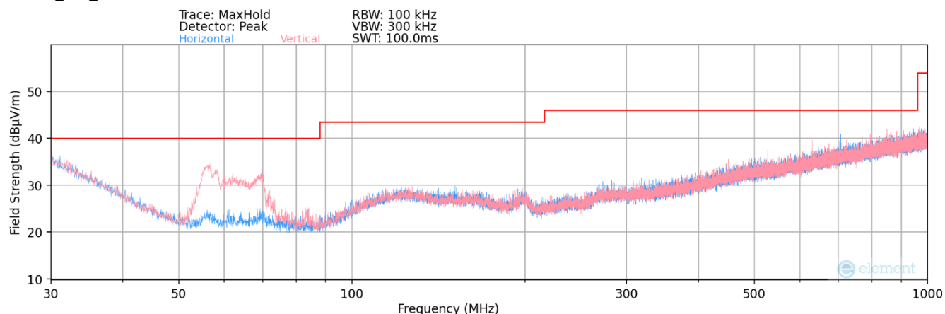
Plot 7-7. Radiated Emissions 30MHz – 1GHz
