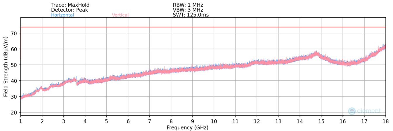
Plot 7-4. Radiated Emissions 1GHz – 18GHz
