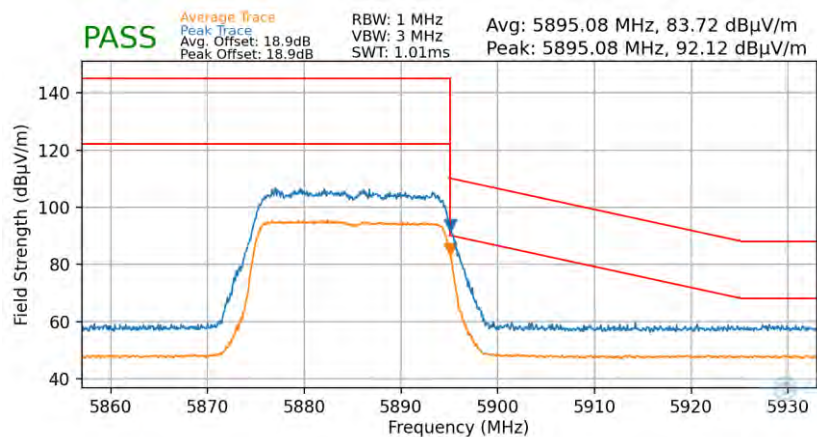
Plot 7-80. Radiated Upper Band Edge Plot (Average & Peak – UNII Band 4)
