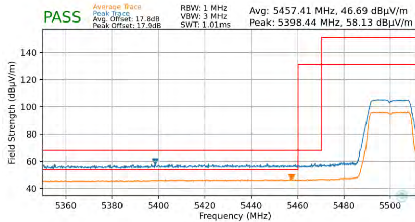
Plot 7-77. Radiated Lower Band Edge Plot (Average & Peak – UNII Band 2C)
