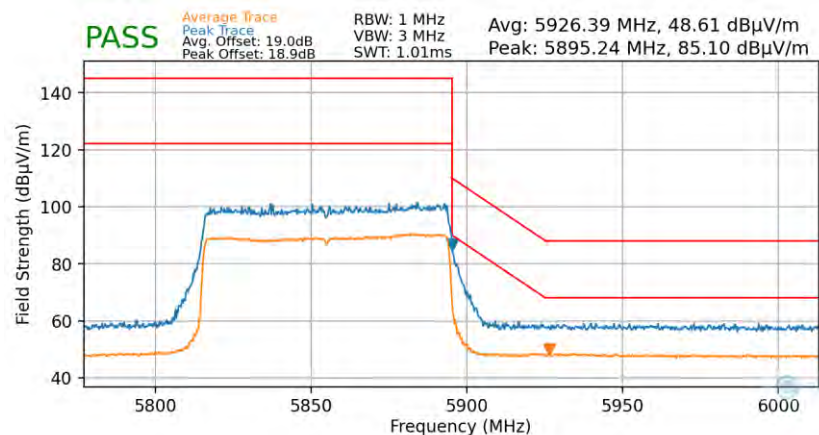
Plot 7-92. Radiated Upper Band Edge Plot (Average & Peak – UNII Band 4)
