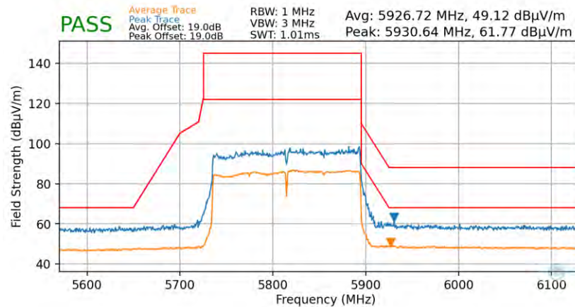
Plot 7-97. Radiated Upper Band Edge Plot (Average & Peak – UNII Band 4)
