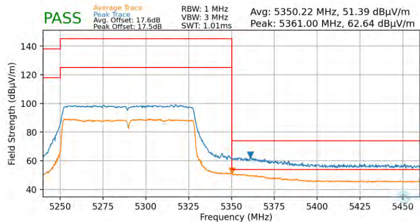
Plot 7-88. Radiated Upper Band Edge Plot (Average & Peak – UNII Band 2A)
