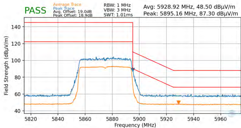
Plot 7-86. Radiated Upper Band Edge Plot (Average & Peak – UNII Band 4)
