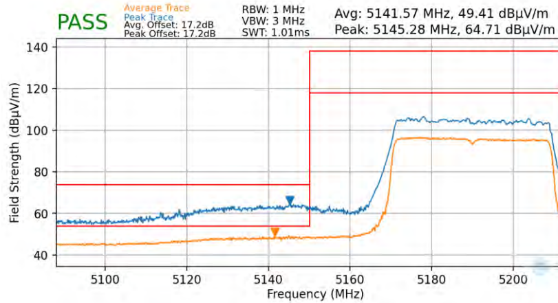
Plot 7-85. Radiated Lower Band Edge Plot (Average & Peak – UNII Band 1 – 484 Tones)
