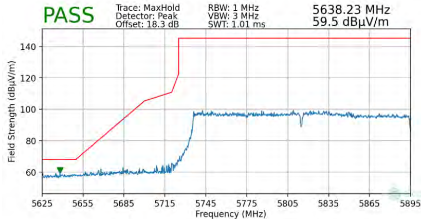
Plot 7-100. Radiated Lower Band Edge Plot (Peak – UNII Band 4 – 2x996T)
