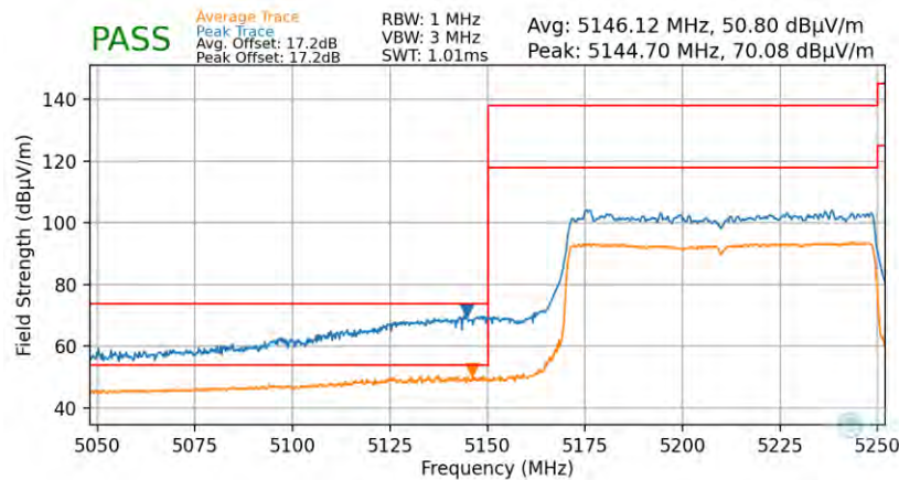
Plot 7-91. Radiated Lower Band Edge Plot (Average & Peak – UNII Band 1 – 996 Tones)
