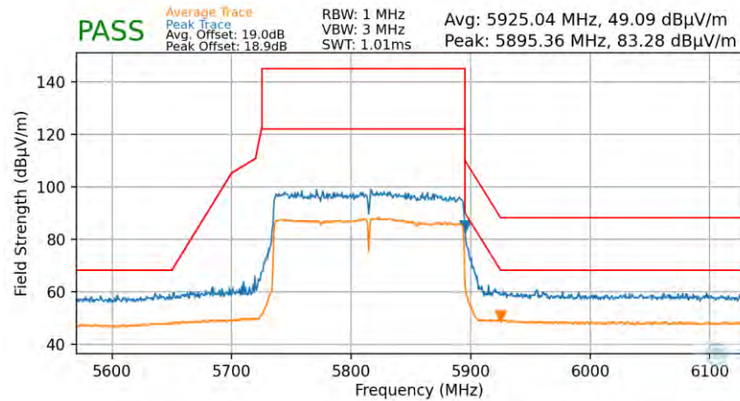
Plot 7-101. Radiated Upper Band Edge Plot (Average & Peak – UNII Band 4 – 2x996T)
