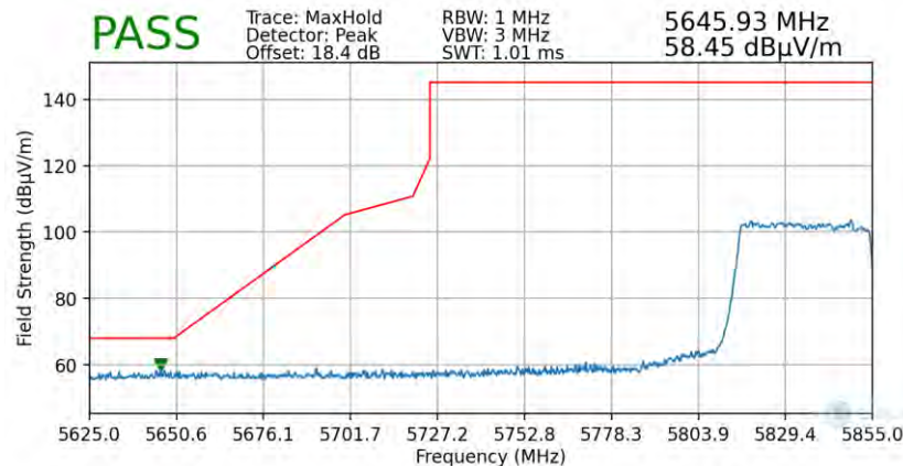
Plot 7-89. Radiated Lower Band Edge Plot (Peak – UNII Band 4 – 484 Tones)
