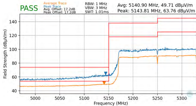
Plot 7-97. Radiated Lower Band Edge Plot (Average & Peak – UNII Band 1 – 2x996T)
