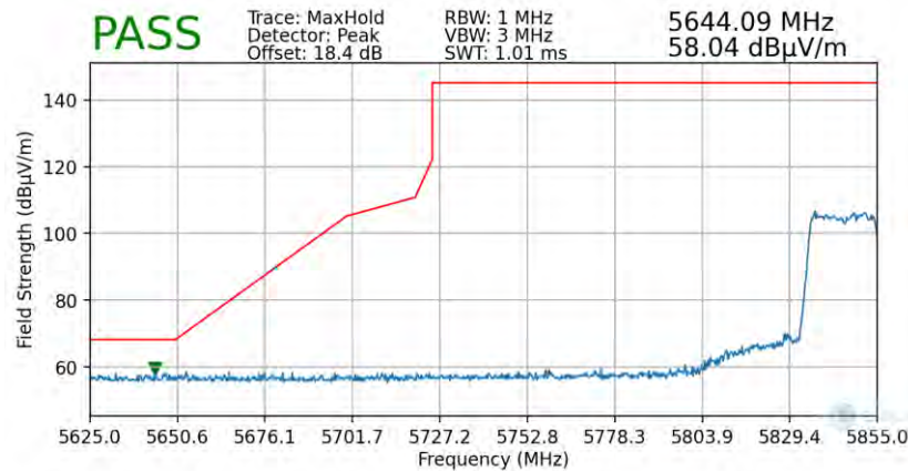
Plot 7-83. Radiated Lower Band Edge Plot (Peak – UNII Band 4 – 242 Tones)
