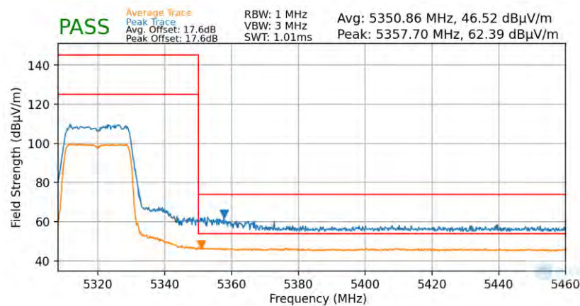
Plot 7-80. Radiated Upper Band Edge Plot (Average & Peak – UNII Band 2A – 242 Tones)
