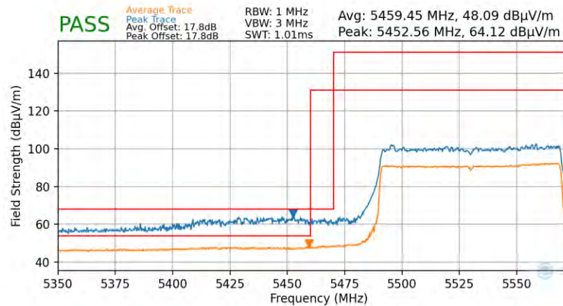
Plot 7-93. Radiated Lower Band Edge Plot (Average & Peak – UNII Band 2C – 996 Tones)
