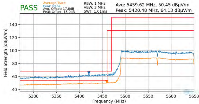
Plot 7-99. Radiated Lower Band Edge Plot (Average & Peak – UNII Band 2C – 2x996T)
