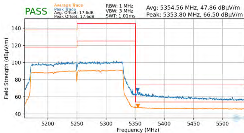
Plot 7-98. Radiated Upper Band Edge Plot (Average & Peak – UNII Band 2A – 2x996T)
