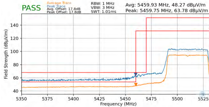
Plot 7-87. Radiated Lower Band Edge Plot (Average & Peak – UNII Band 2C – 484 Tones)
