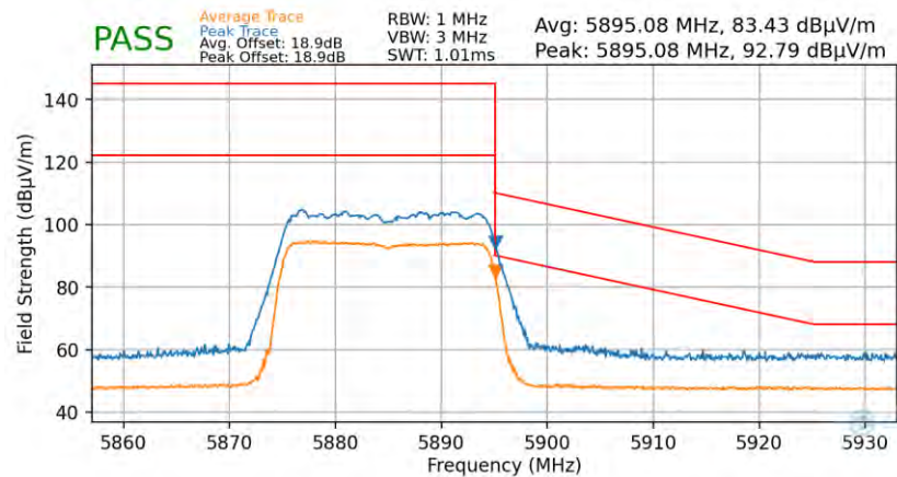
Plot 7-84. Radiated Upper Band Edge Plot (Average & Peak – UNII Band 4 – 242 Tones)
