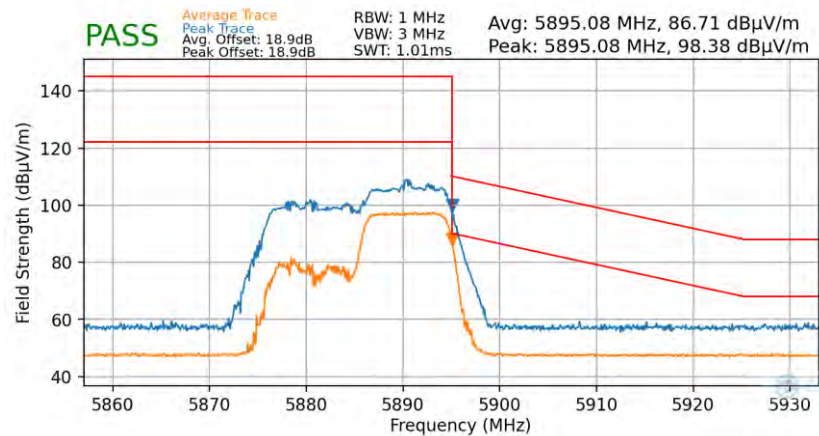
Plot 7-78. Radiated Upper Band Edge Plot (Average & Peak - UNII Band 4 - 106 Tones)
