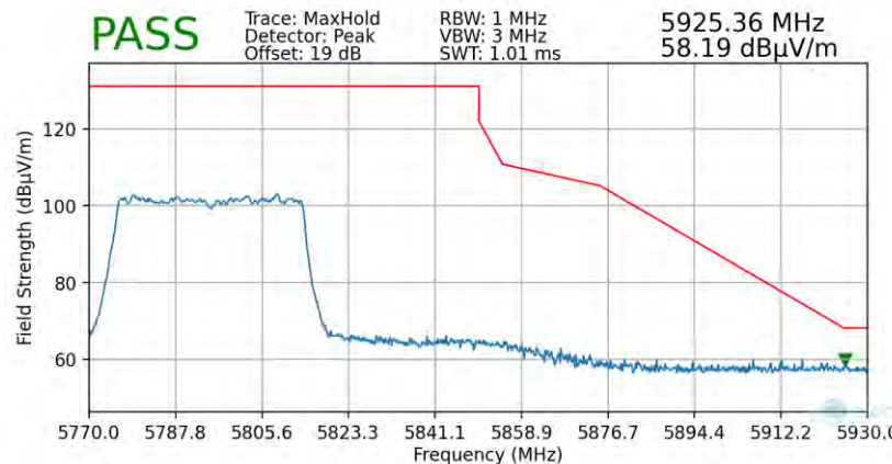
Plot 7-88. Radiated Upper Band Edge Plot (Peak – UNII Band 3 – 484 Tones)
