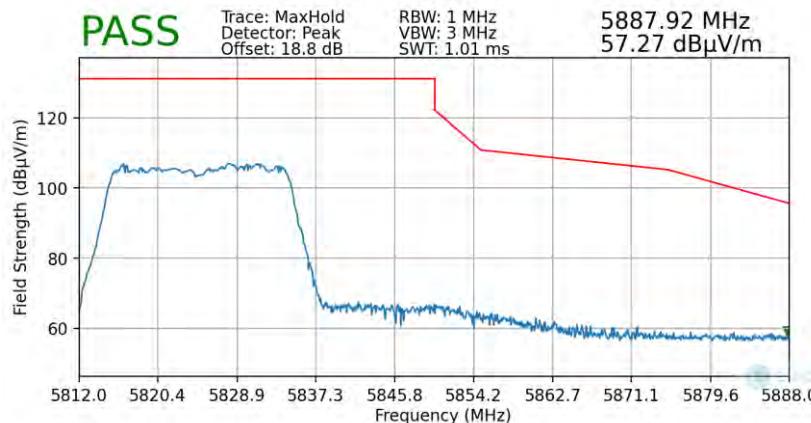
Plot 7-82. Radiated Upper Band Edge Plot (Peak – UNII Band 3 – 242 Tones)
