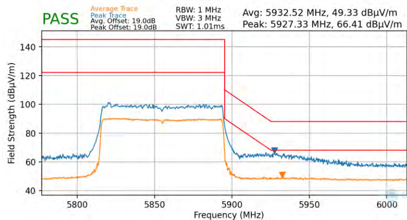
Plot 7-96. Radiated Upper Band Edge Plot (Average & Peak – UNII Band 4 – 996 Tones)
