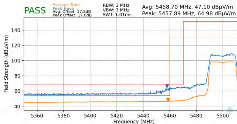
Plot 7-81. Radiated Lower Band Edge Plot (Average & Peak – UNII Band 2C – 242 Tones)
