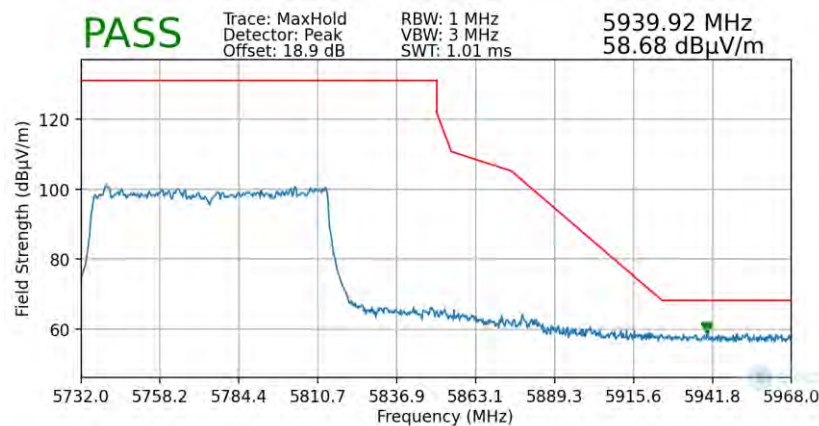
Plot 7-94. Radiated Upper Band Edge Plot (Peak – UNII Band 3 – 996 Tones)
