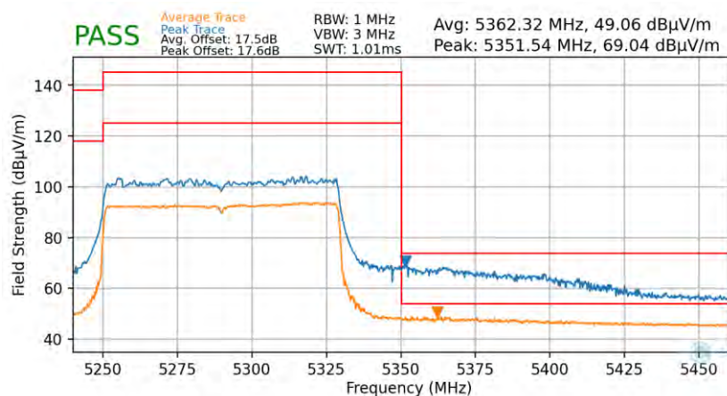
Plot 7-92. Radiated Upper Band Edge Plot (Average & Peak – UNII Band 2A – 996 Tones)
