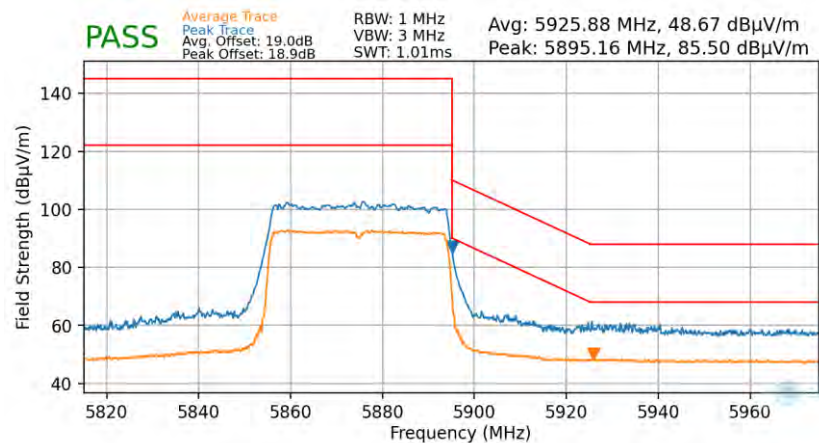
Plot 7-90. Radiated Upper Band Edge Plot (Average & Peak – UNII Band 4 – 484 Tones)
