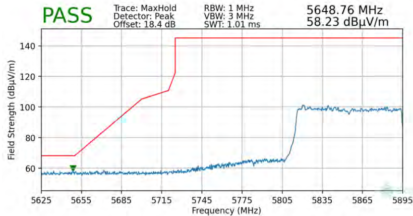
Plot 7-95. Radiated Lower Band Edge Plot (Peak – UNII Band 4 – 996 Tones)
