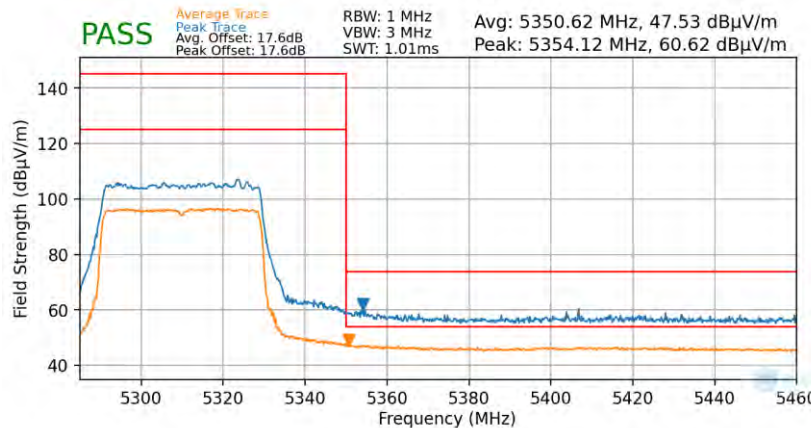
Plot 7-86. Radiated Upper Band Edge Plot (Average & Peak – UNII Band 2A – 484 Tones)
