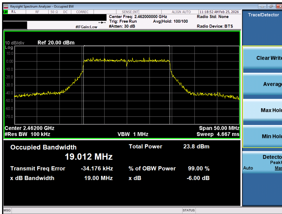
Plot 7-12. 6dB Bandwidth Plot SISO ANT1 (802.11ax (2.4GHz) – Ch. 11)
