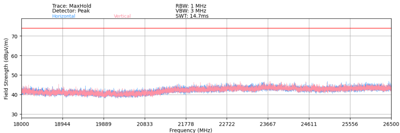
Plot 7-63. Radiated Spurious Plot above 18GHz
