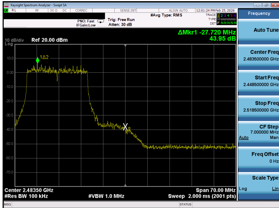
Plot 7-24. Band Edge Plot SISO ANT1 (802.11ax OFDMA – 242 Tones – Ch. 11)
