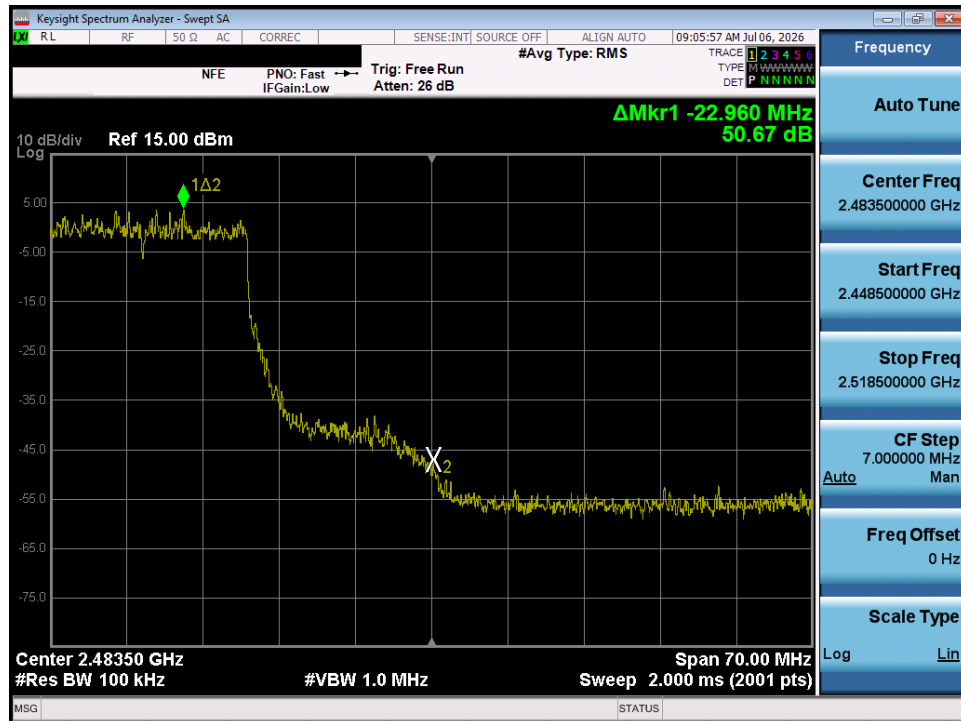
Plot 7-23. Band Edge Plot SISO ANT1 (802.11ax OFDMA – 242 Tones – Ch. 10)
