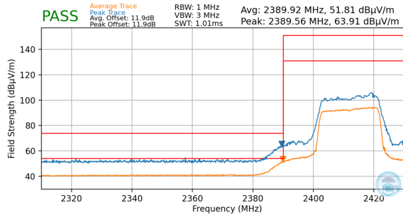
Plot 7-48. Radiated Restricted Lower Band Edge Measurement (Average & Peak – 242 Tones)
