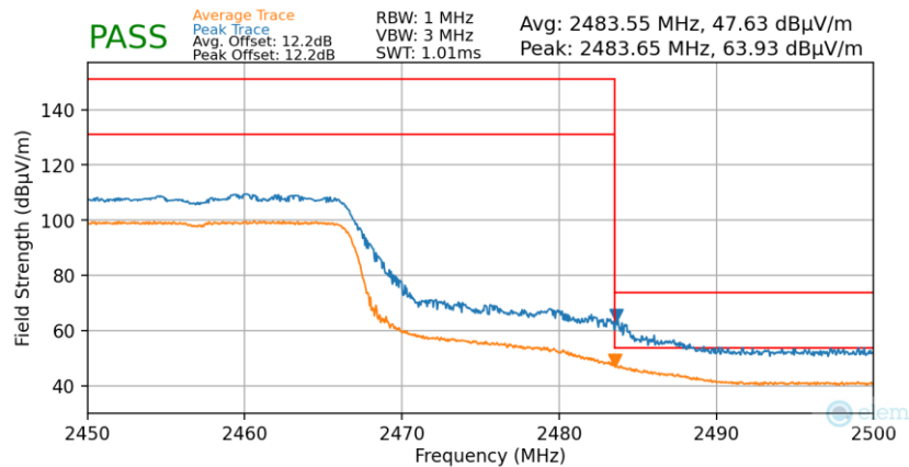
Plot 7-50. Radiated Restricted Upper Band Edge Measurement (Average & Peak – 242 Tones)
