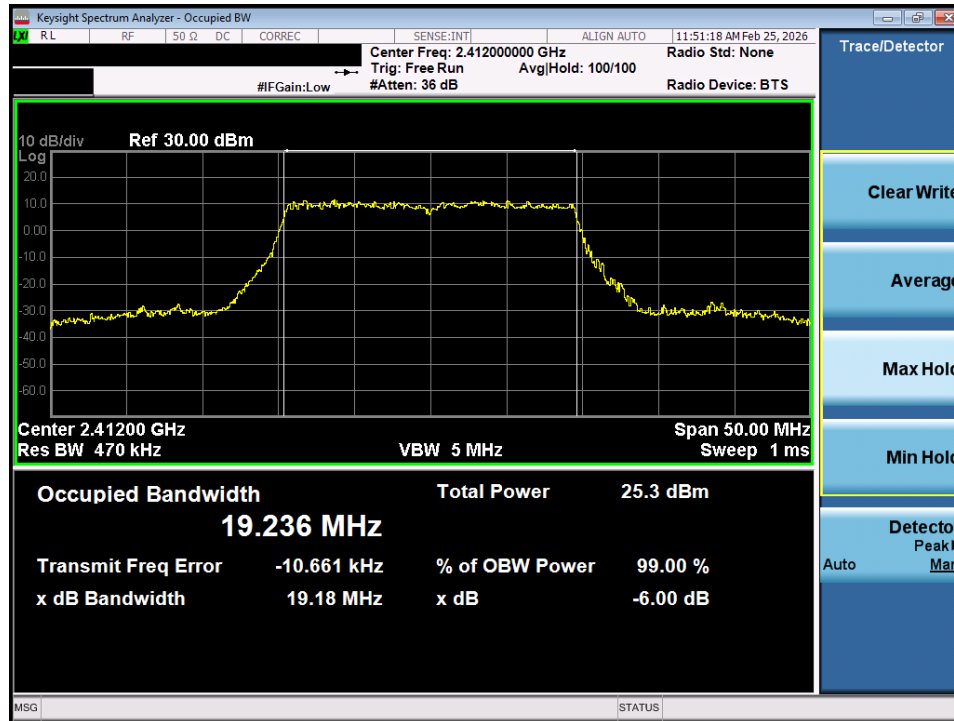
Plot 7-10. OBW Plot SISO ANT1 (802.11ax OFDMA – 242 Tones – Ch. 1)
