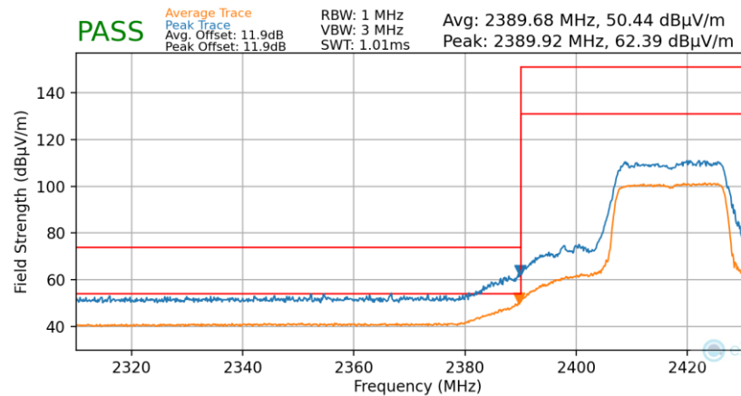
Plot 7-49. Radiated Restricted Lower Band Edge Measurement (Average & Peak – 242 Tones)
