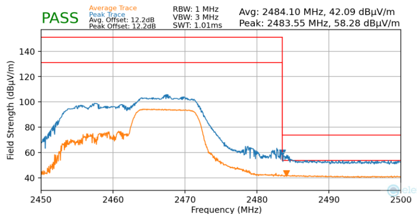
Plot 7-47. Radiated Restricted Upper Band Edge Measurement (Average & Peak – 106 Tones)
