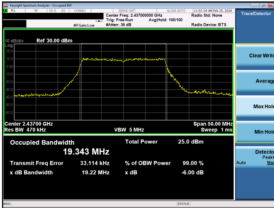
Plot 7-11. OBW Plot SISO ANT1 (802.11ax OFDMA – 242 Tones – Ch. 6)
