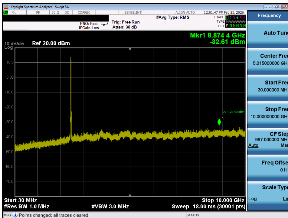
Plot 7-35. Conducted Spurious Plot SISO ANT1 (802.11ax OFDMA – 242 Tones – Ch. 11)
