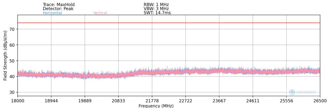
Plot 7-45. Radiated Spurious Plot above 18GHz (802.11ax OFDMA – 242 Tones)
