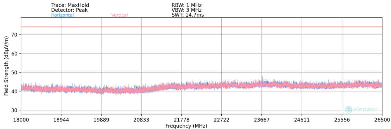
Plot 7-41. Radiated Spurious Plot above 18GHz (802.11ax OFDMA – 26 Tones)
