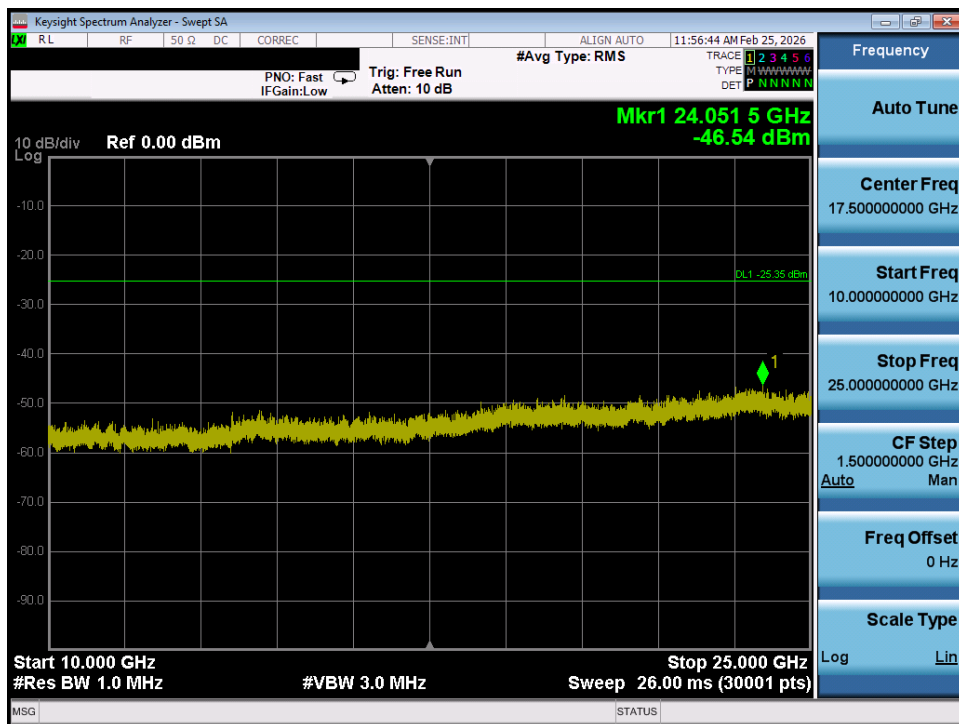
Plot 7-28. Conducted Spurious Plot SISO ANT1 (802.11ax OFDMA – 26 Tones – Ch. 6)
