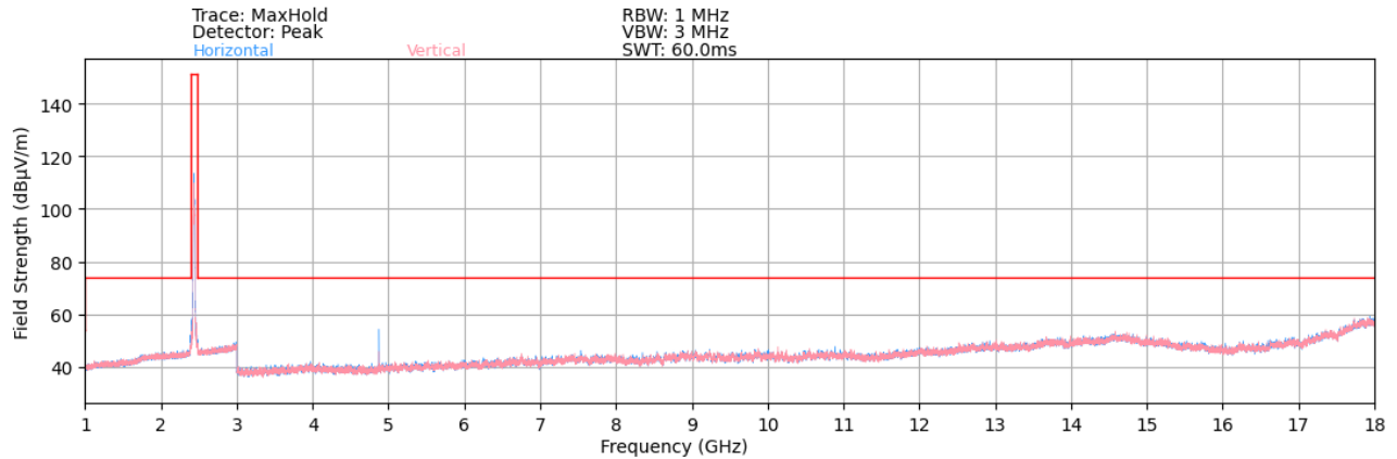
Plot 7-39. Radiated Spurious Plot above 1GHz (802.11ax OFDMA – 26 Tones – Ch. 6)
