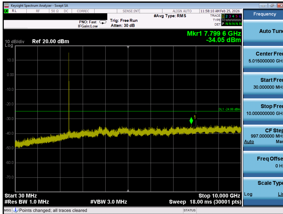
Plot 7-25. Conducted Spurious Plot SISO ANT1 (802.11ax OFDMA – 26 Tones – Ch. 1)
