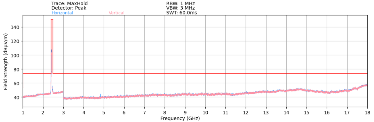
Plot 7-42. Radiated Spurious Plot above 1GHz (802.11ax OFDMA – 242 Tones – Ch. 1)
