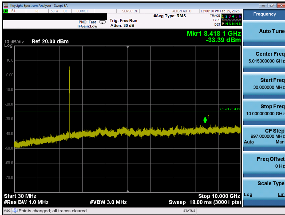
Plot 7-29. Conducted Spurious Plot SISO ANT1 (802.11ax OFDMA – 26 Tones – Ch. 11)
