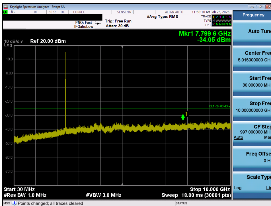
Plot 7-37. Conducted Spurious Plot SISO ANT1 (802.11ax OFDMA – 26 Tones – Ch. 1)
