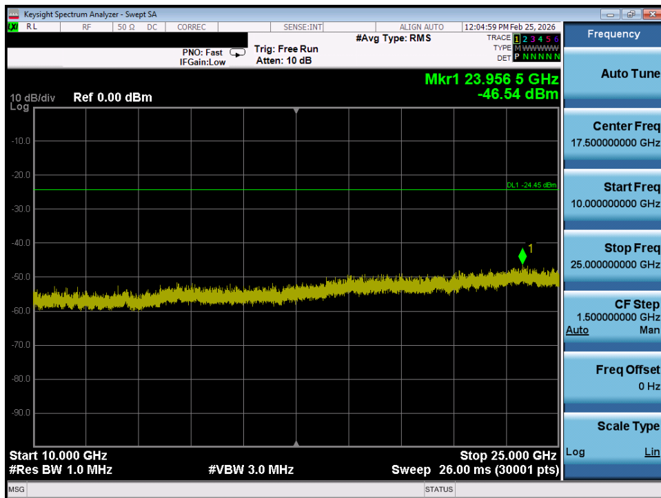
Plot 7-32. Conducted Spurious Plot SISO ANT1 (802.11ax OFDMA – 242 Tones – Ch. 1)
