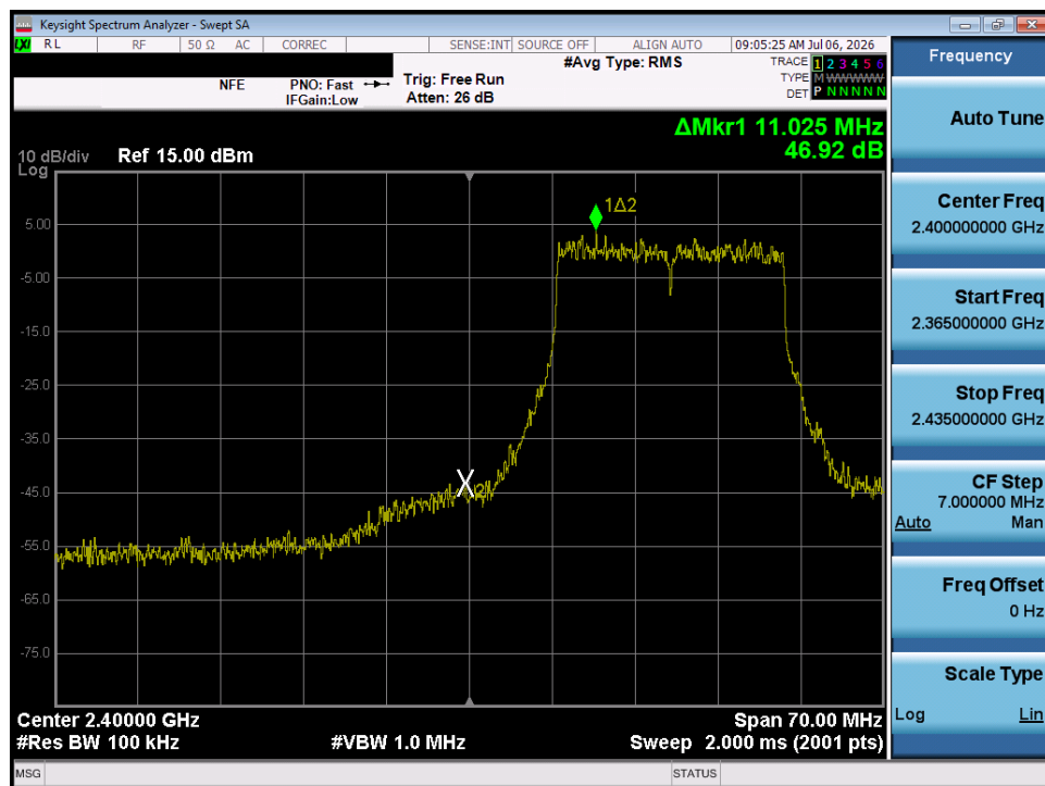
Plot 7-22. Band Edge Plot SISO ANT1 (802.11ax OFDMA – 242 Tones – Ch. 2)
