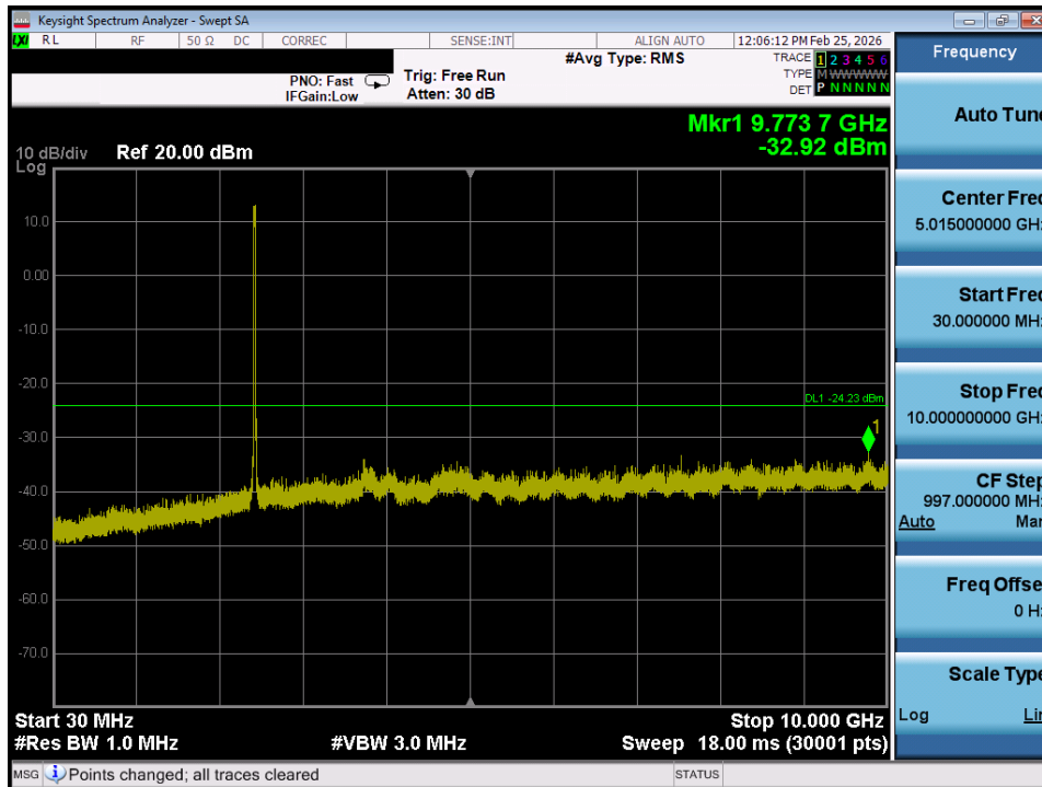
Plot 7-33. Conducted Spurious Plot SISO ANT1 (802.11ax OFDMA – 242 Tones – Ch. 6)
