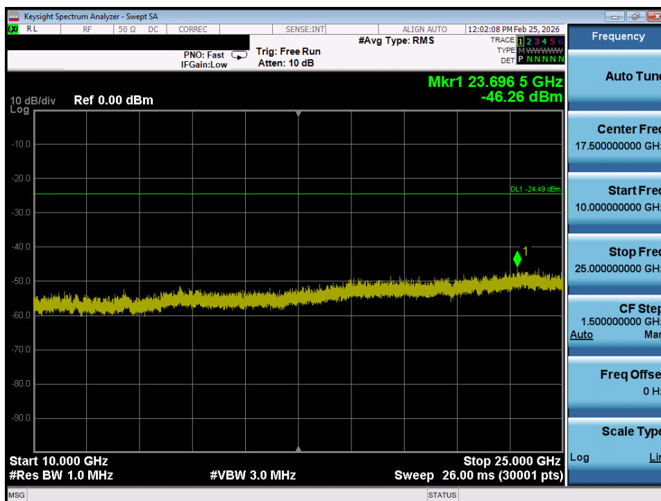
Plot 7-36. Conducted Spurious Plot SISO ANT1 (802.11ax OFDMA – 242 Tones – Ch. 11)
