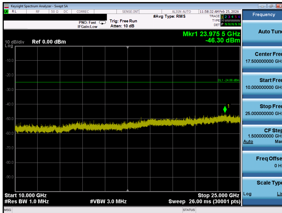
Plot 7-26. Conducted Spurious Plot SISO ANT1 (802.11ax OFDMA – 26 Tones – Ch. 1)
