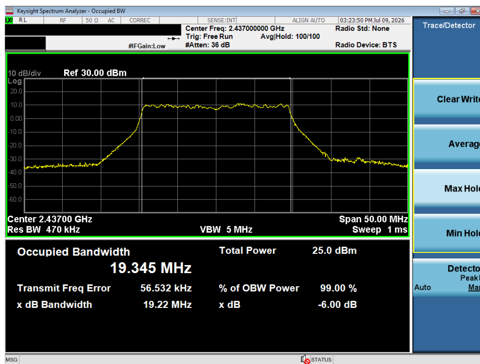
Plot 9-1. Occupied Bandwidth Plot (Spot-check)
