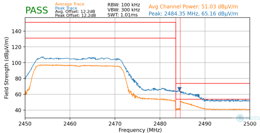
Plot 7-51. Radiated Restricted Upper Band Edge Measurement (Average & Peak – 242 Tones)
