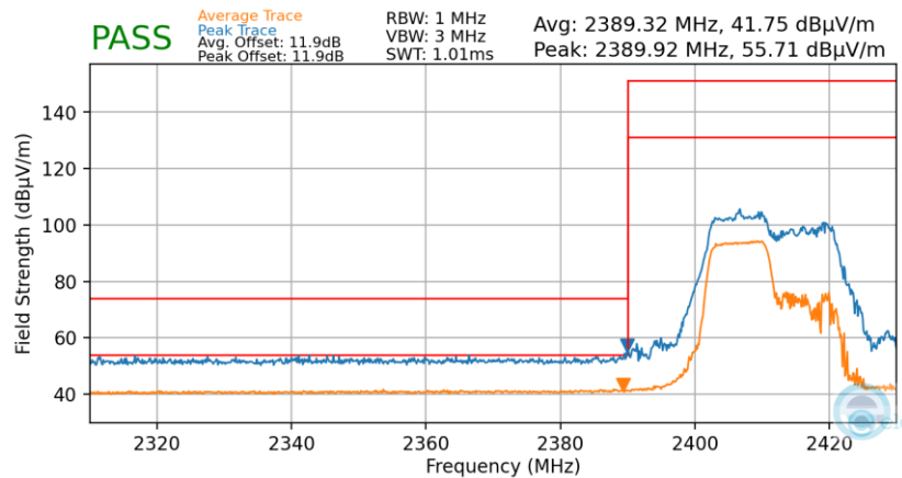
Plot 7-46. Radiated Restricted Lower Band Edge Measurement (Average & Peak – 106 Tones)
