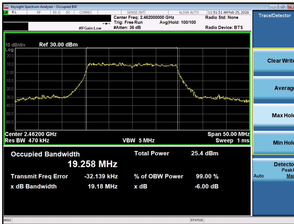
Plot 7-12. OBW Plot SISO ANT1 (802.11ax OFDMA – 242 Tones – Ch. 11)
