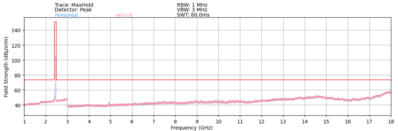
Plot 7-44. Radiated Spurious Plot above 1GHz (802.11ax OFDMA – 242 Tones – Ch. 11)
