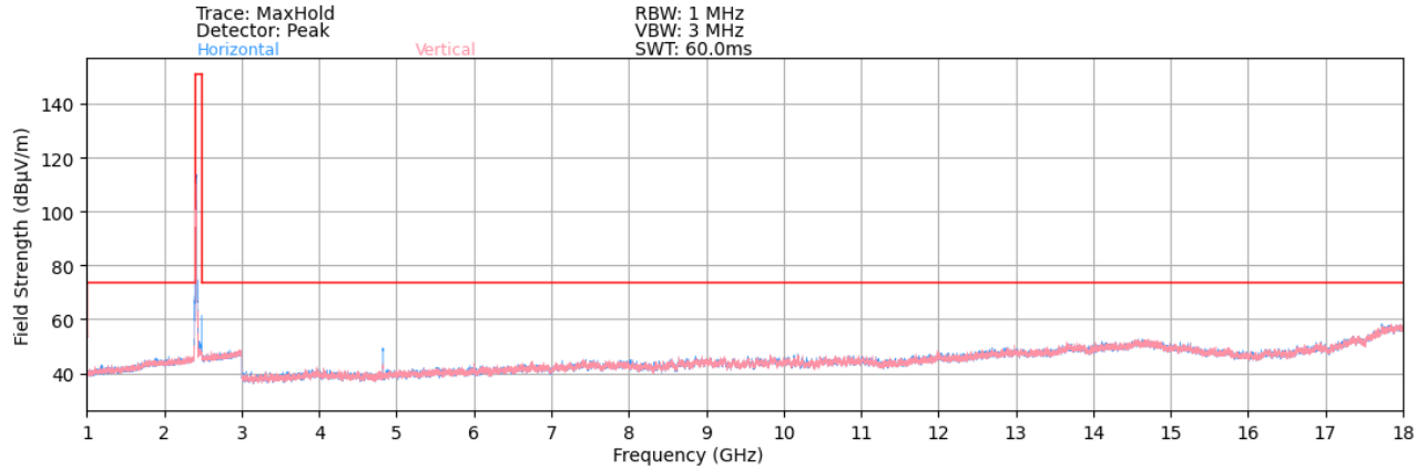
Plot 7-38. Radiated Spurious Plot above 1GHz (802.11ax OFDMA – 26 Tones – Ch. 1)
