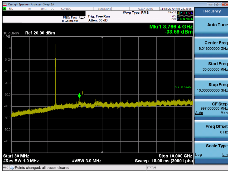
Plot 7-27. Conducted Spurious Plot SISO ANT1 (802.11ax OFDMA – 26 Tones – Ch. 6)
