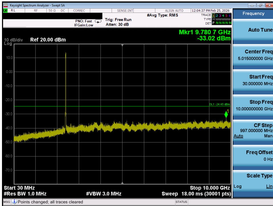
Plot 7-31. Conducted Spurious Plot SISO ANT1 (802.11ax OFDMA – 242 Tones – Ch. 1)
