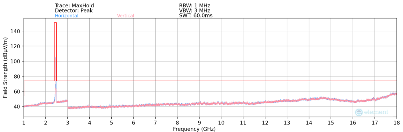
Plot 7-40. Radiated Spurious Plot above 1GHz (802.11ax OFDMA – 26 Tones – Ch. 11)
