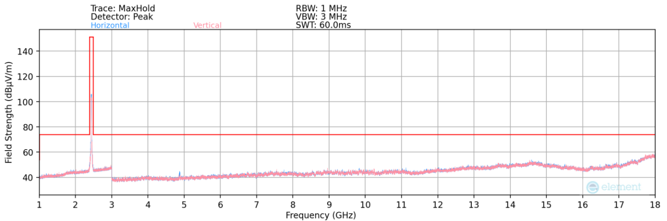
Plot 7-43. Radiated Spurious Plot above 1GHz (802.11ax OFDMA – 242 Tones – Ch. 6)
