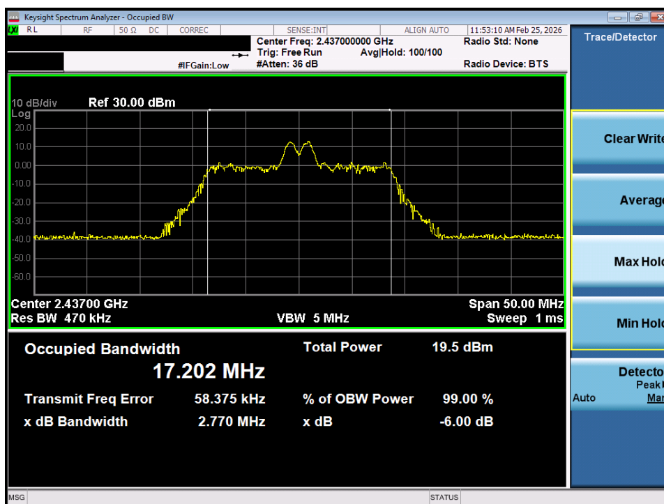
Plot 7-8. OBW Plot SISO ANT1 (802.11ax OFDMA – 26 Tones – Ch. 6)
