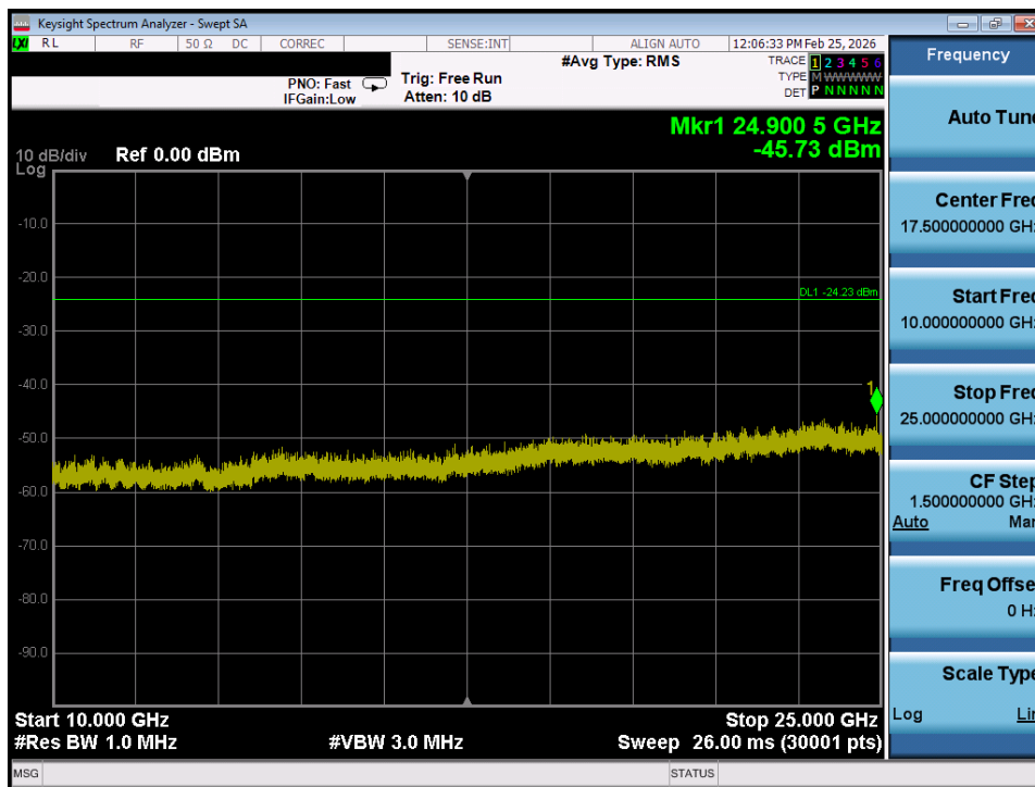
Plot 7-34. Conducted Spurious Plot SISO ANT1 (802.11ax OFDMA – 242 Tones – Ch. 6)
