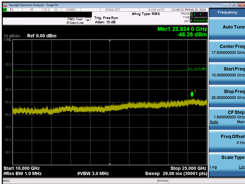
Plot 7-30. Conducted Spurious Plot SISO ANT1 (802.11ax OFDMA – 26 Tones – Ch. 11)
