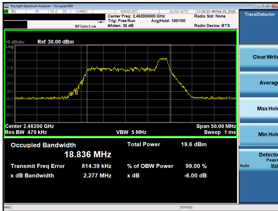
Plot 7-9. OBW Plot SISO ANT1 (802.11ax OFDMA – 26 Tones – Ch. 11)
