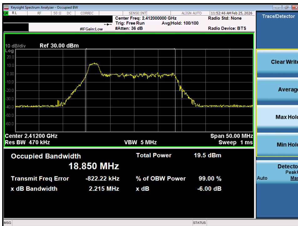
Plot 7-7. OBW Plot SISO ANT1 (802.11ax OFDMA – 26 Tones – Ch. 1)
