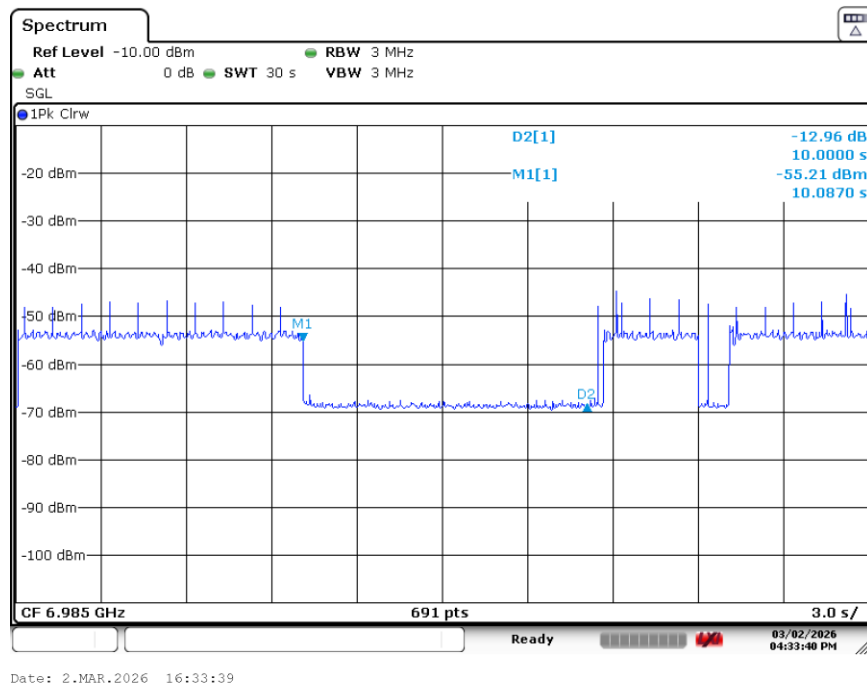
Plot 7-31. Contention Based Protocol Timing Plot (160MHz (UNII Band 8) – Ch. 207 Mid)
