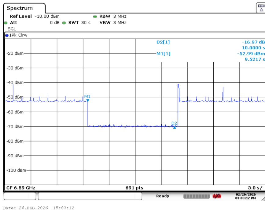
Plot 7-26. Contention Based Protocol Timing Plot (160MHz (UNII Band 7) – Ch. 143 Low)
