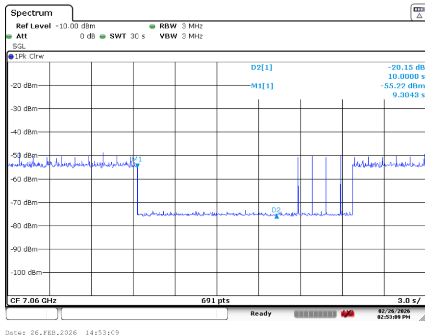
Plot 7-32. Contention Based Protocol Timing Plot (160MHz (UNII Band 8) – Ch. 207 High)
