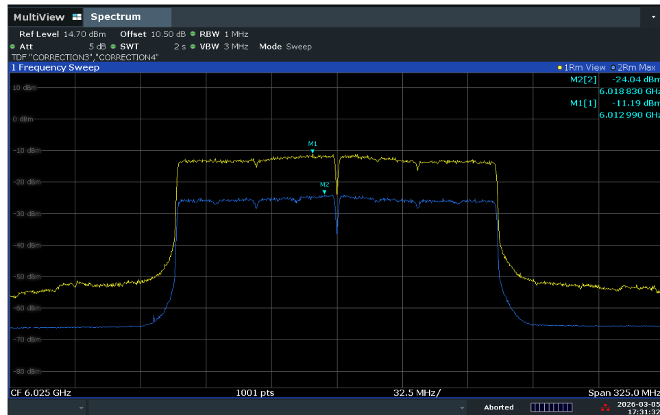
Plot 7-36. Power Spectral Density Plot – ANT1 (160MHz Bandwidth, RSSI level at Low (yellow) and High (blue))
