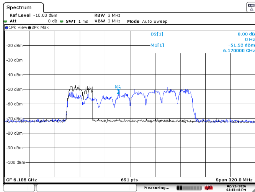
Plot 7-34. CBP 160MHz Channel - Injection Center – [6185 MHz]
