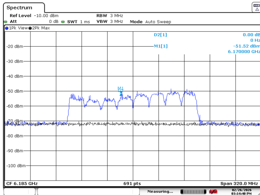
Plot 7-33. CBP 160MHz Channel - Injection Lower Edge – [6110 MHz]
