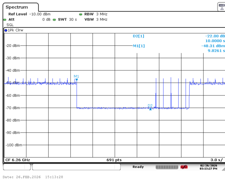
Plot 7-20. Contention Based Protocol Timing Plot (160MHz (UNII Band 5) – Ch. 47 High)
