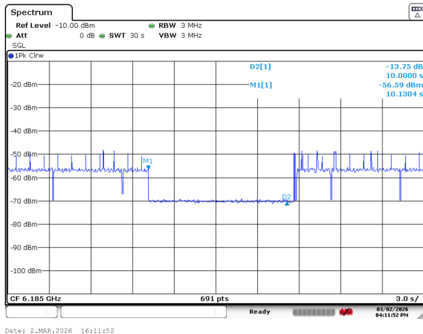
Plot 7-19. Contention Based Protocol Timing Plot (160MHz (UNII Band 5) – Ch. 47 Mid)
