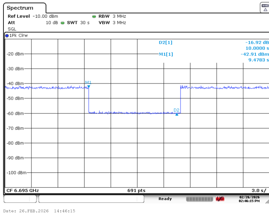
Plot 7-25. Contention Based Protocol Timing Plot (20MHz (UNII Band 7) – Ch. 149)
