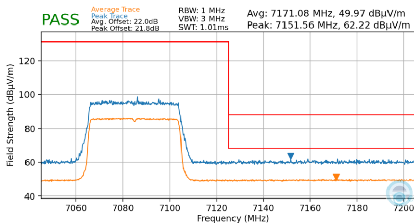
Plot 7-47. Radiated Upper Band Edge Plot SISO (Average & Peak – UNII Band 8)
