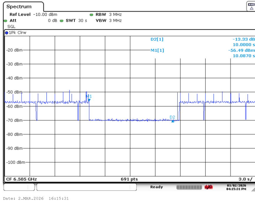
Plot 7-23. Contention Based Protocol Timing Plot (160MHz (UNII Band 6) – Ch. 111 Mid)
