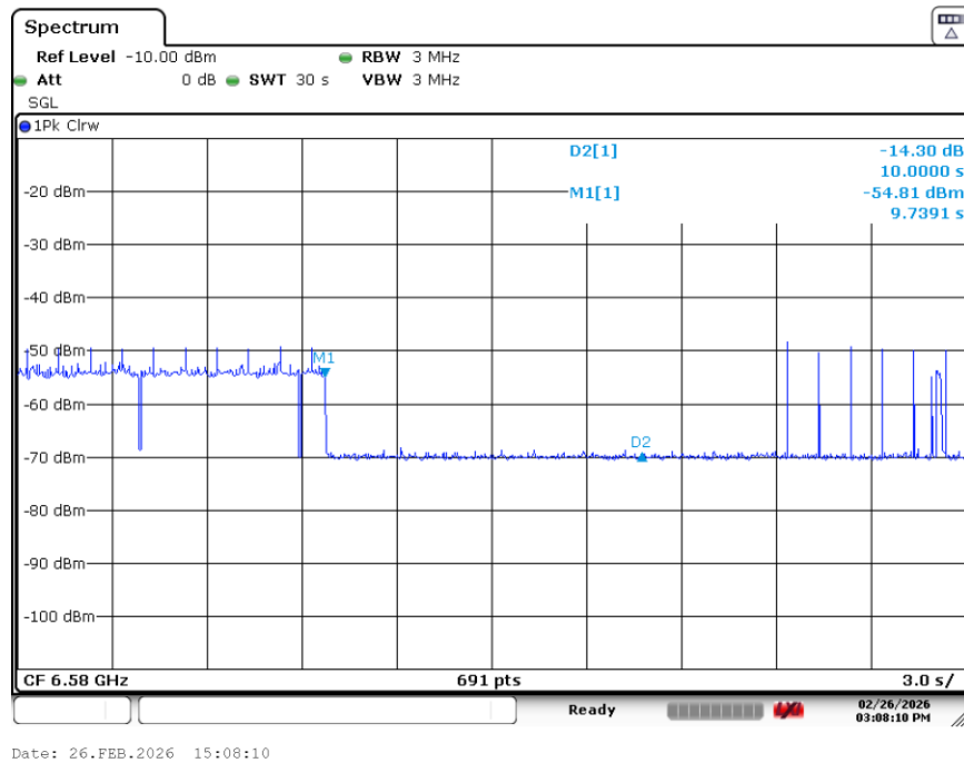
Plot 7-24. Contention Based Protocol Timing Plot (160MHz (UNII Band 6) – Ch. 111 High)
