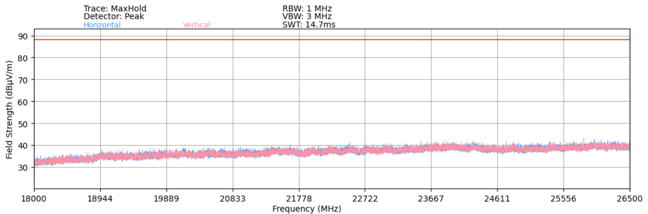
Plot 7-42. Radiated Spurious Plot 18GHz - 26.5GHz (802.11a)
