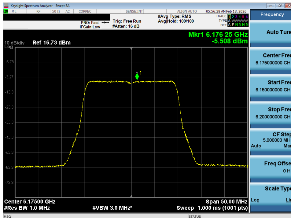
Plot 7-7. Power Spectral Density Plot SISO ANT1 (20MHz 802.11ax (UNII Band 5) – Ch. 45) - VLP
