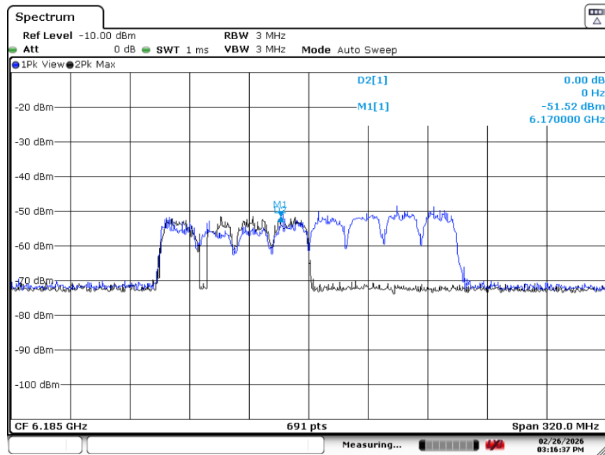
Plot 7-35. CBP 160MHz Channel - Injection Upper Edge – [6260 MHz]
