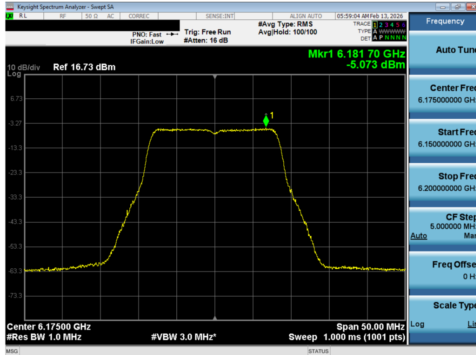
Plot 7-6. Power Spectral Density Plot SISO ANT1 (20MHz 802.11a (UNII Band 5) – Ch. 45) - VLP
