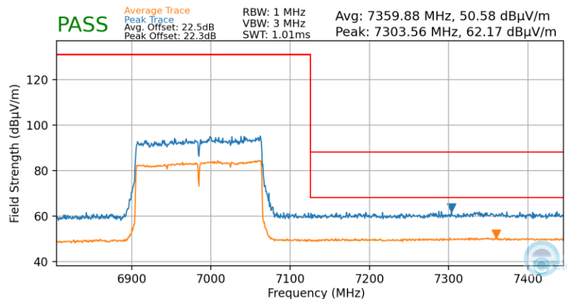
Plot 7-50. Radiated Upper Band Edge Plot SISO (Average & Peak – UNII Band 8)
