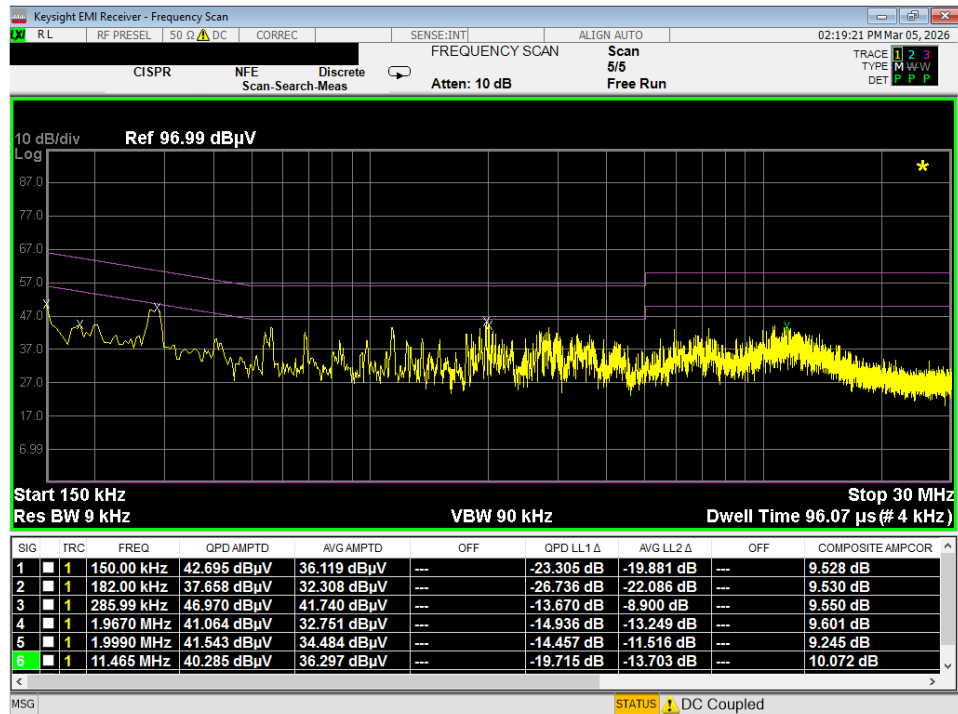
Plot 7-51. Line Conducted Plot with 802.11a UNII Band 5 (L1)
