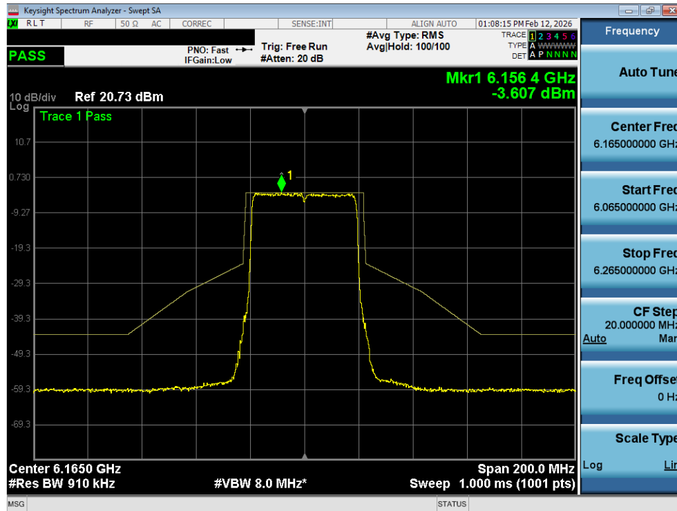
Plot 7-13. In Band Emissions Plot SISO ANT1 (40MHz 802.11ax (UNII Band 5) – Ch. 43) - LPI
