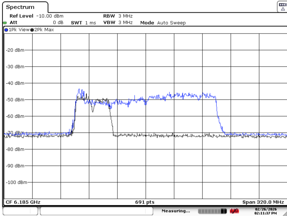
Plot 7-34. CBP 160MHz Channel - Injection Center – [6185 MHz]
