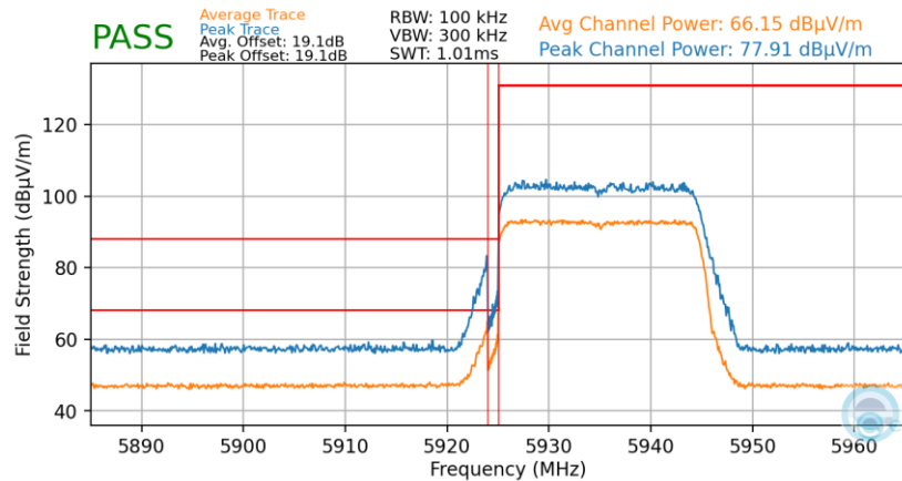
Plot 7-43. Radiated Lower Band Edge Plot SISO (Average & Peak – UNII Band 5)
