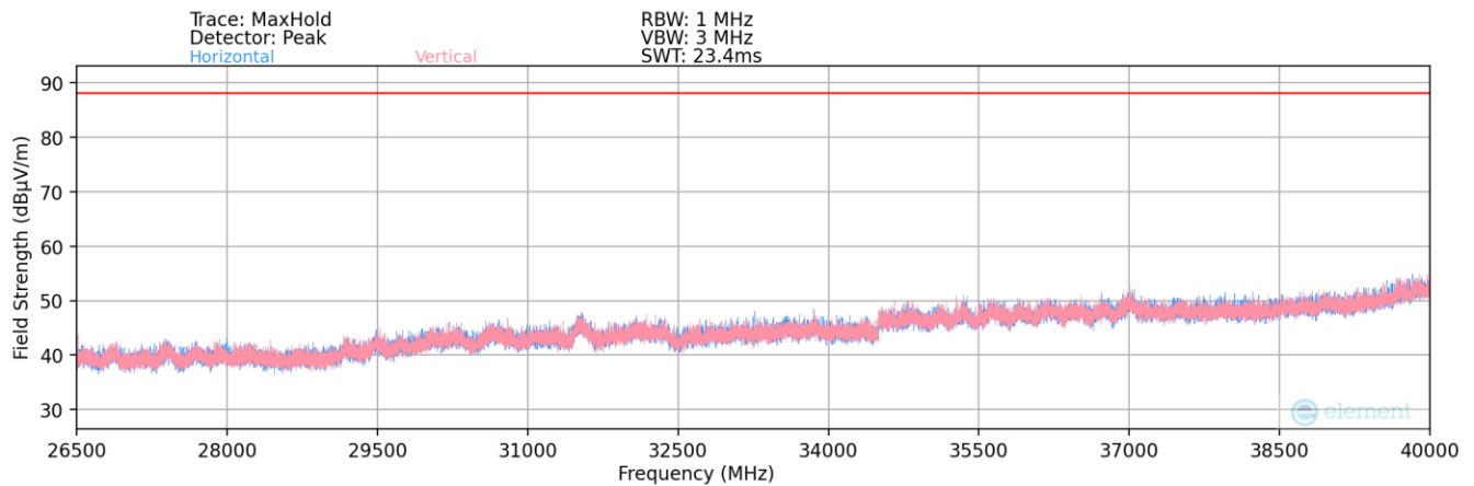
Plot 7-42. Radiated Spurious Plot 26.5GHz - 40GHz (802.11a)
