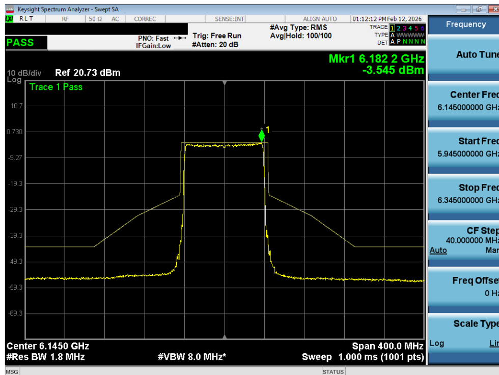
Plot 7-14. In Band Emissions Plot SISO ANT1 (80MHz 802.11ax (UNII Band 5) – Ch. 39) - LPI
