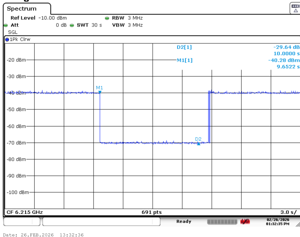
Plot 7-17. Contention Based Protocol Timing Plot (20MHz (UNII Band 5) – Ch. 53)
