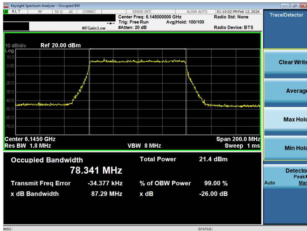
Plot 7-4. 26dB Bandwidth Plot SISO ANT1 (80MHz 802.11ax (UNII Band 5) – Ch. 39) – LPI
