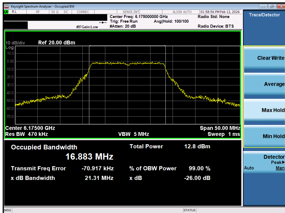
Plot 7-1. 26dB Bandwidth Plot SISO ANT1 (20MHz 802.11a (UNII Band 5) – Ch. 45) - LPI
