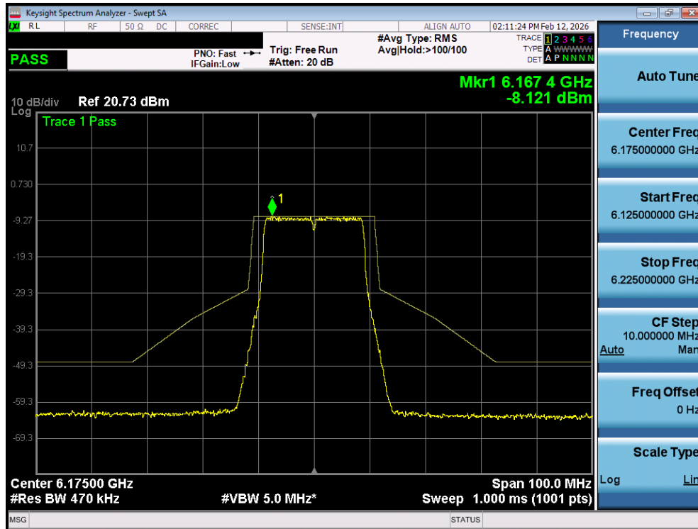
Plot 7-12. In Band Emissions Plot SISO ANT1 (20MHz 802.11ax (UNII Band 5) – Ch. 45) - LPI
