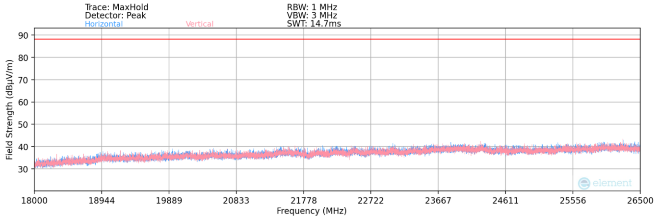
Plot 7-41. Radiated Spurious Plot 18GHz - 26.5GHz (802.11a)
