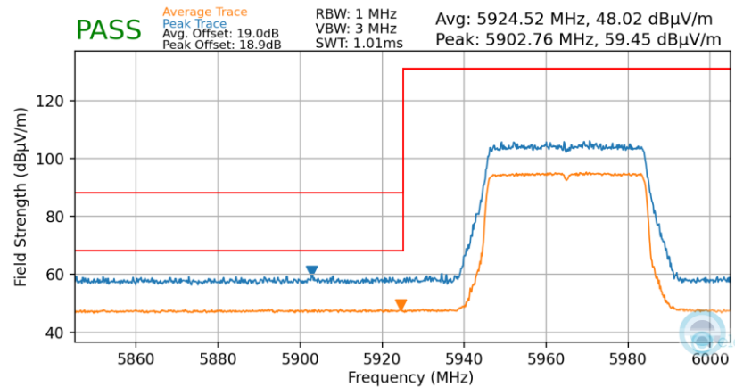
Plot 7-45. Radiated Lower Band Edge Plot SISO (Average & Peak – UNII Band 5)
