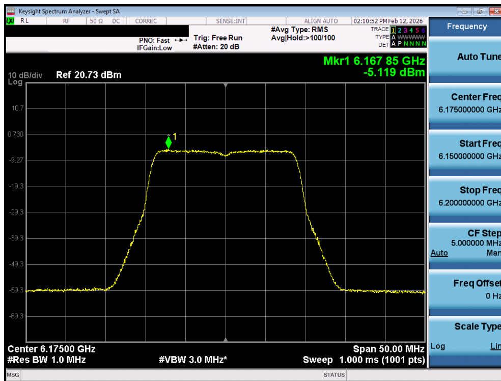
Plot 7-7. Power Spectral Density Plot SISO ANT1 (20MHz 802.11ax (UNII Band 5) – Ch. 45) - LPI
