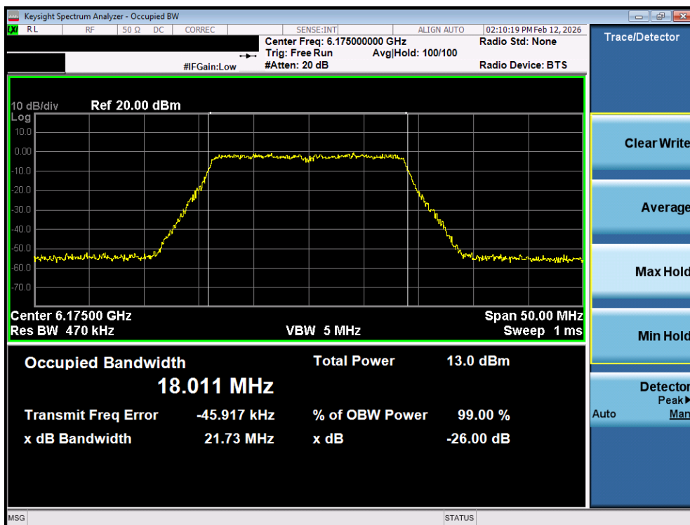
Plot 7-2. 26dB Bandwidth Plot SISO ANT1 (20MHz 802.11ax (UNII Band 5) – Ch. 45) - LPI
