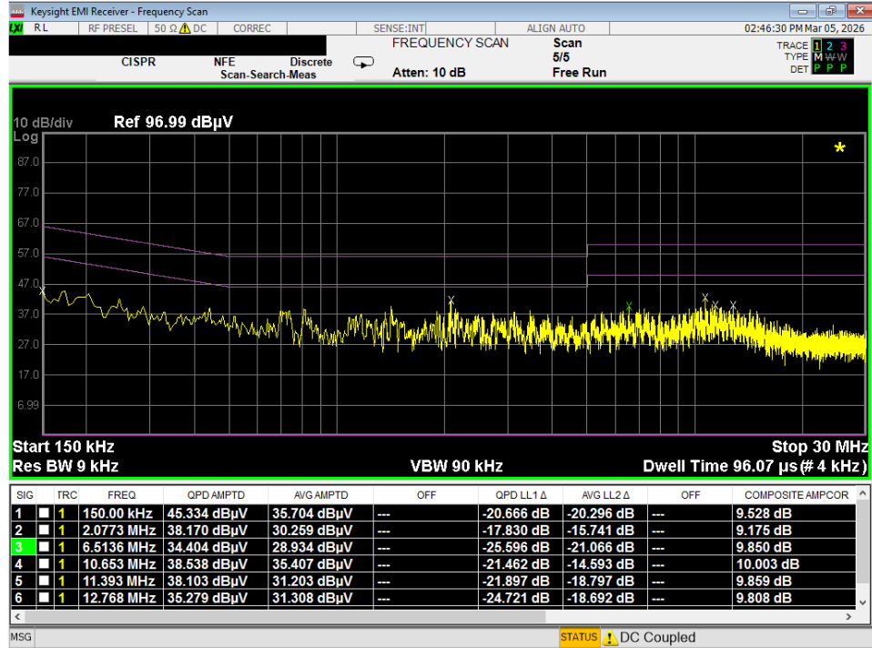
Plot 7-57. Line Conducted Plot with 802.11a UNII Band 8 (L1)
