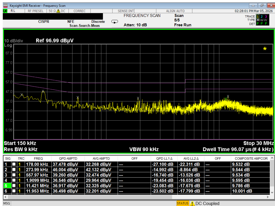
Plot 7-54. Line Conducted Plot with 802.11a UNII Band 6 (N)
