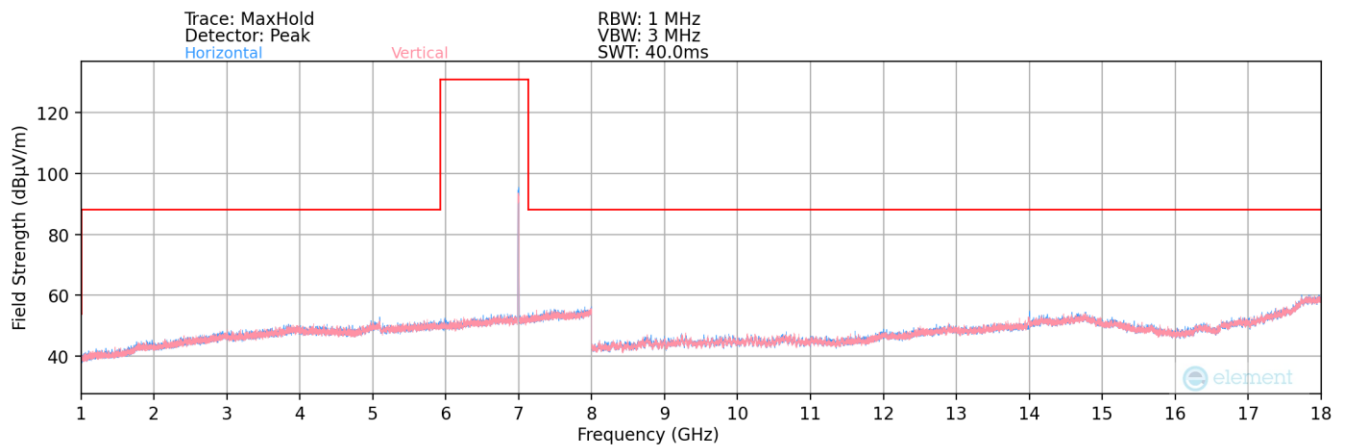
Plot 7-40. Radiated Spurious Plot 1GHz – 18GHz (802.11a – UNII Band 8 Ch. 209)
