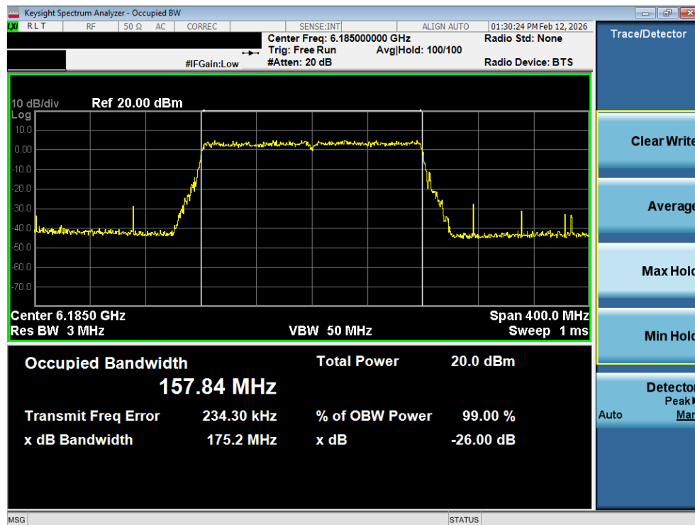
Plot 7-5. 26dB Bandwidth Plot SISO ANT1 (160MHz 802.11ax (UNII Band 5) – Ch. 47) - LPI
