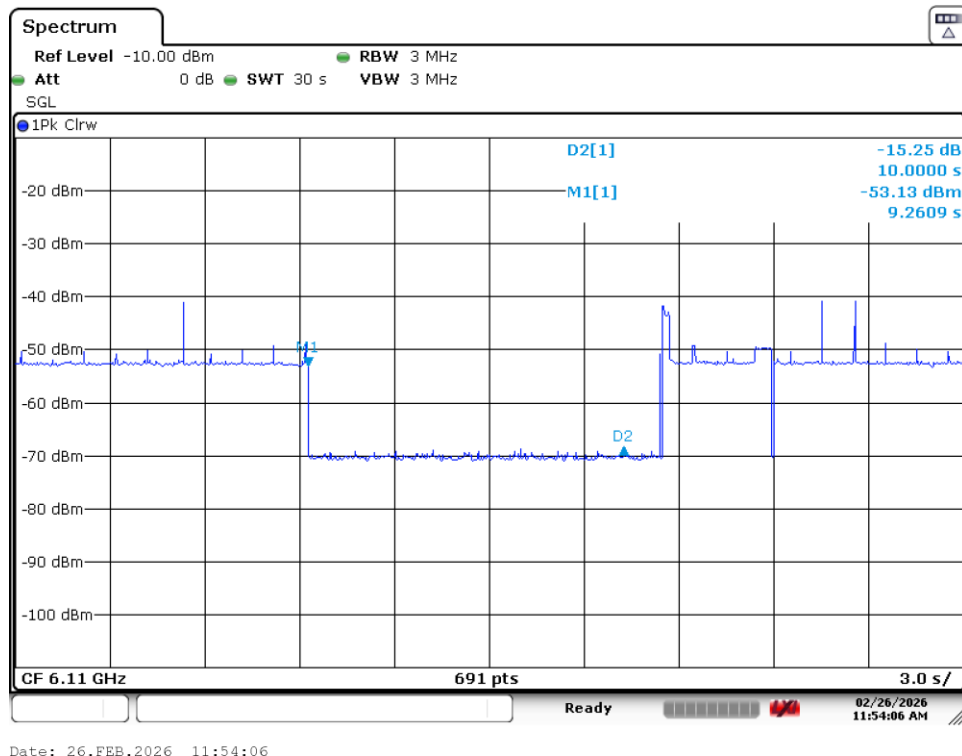
Plot 7-18. Contention Based Protocol Timing Plot (160MHz (UNII Band 5) – Ch. 47 Low)
