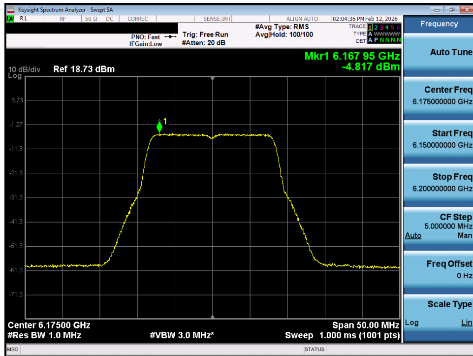
Plot 7-6. Power Spectral Density Plot SISO ANT1 (20MHz 802.11a (UNII Band 5) – Ch. 45) - LPI
