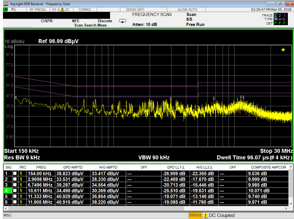
Plot 7-55. Line Conducted Plot with 802.11a UNII Band 7 (L1)
