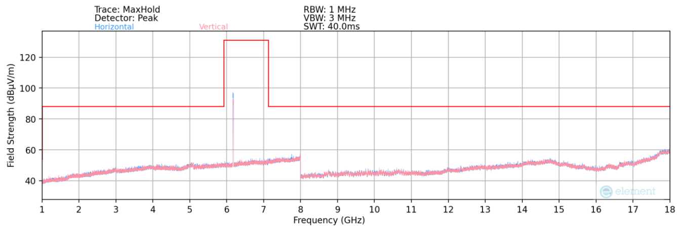
Plot 7-37. Radiated Spurious Plot 1GHz – 18GHz (802.11a – UNII Band 5 Ch. 45)
