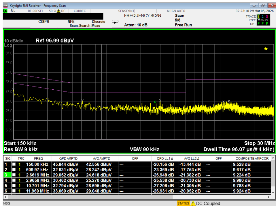
Plot 7-52. Line Conducted Plot with 802.11a UNII Band 5 (N)
