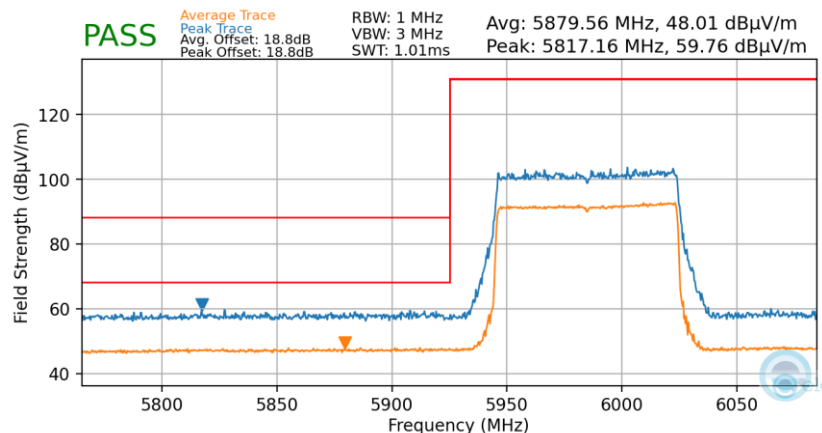
Plot 7-47. Radiated Lower Band Edge Plot SISO (Average & Peak – UNII Band 5)
