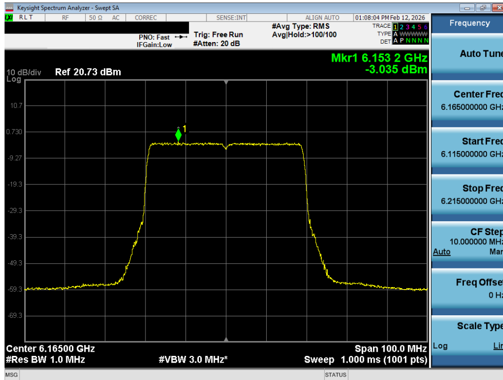
Plot 7-8. Power Spectral Density Plot SISO ANT1 (40MHz 802.11ax (UNII Band 5) – Ch. 43) - LPI
