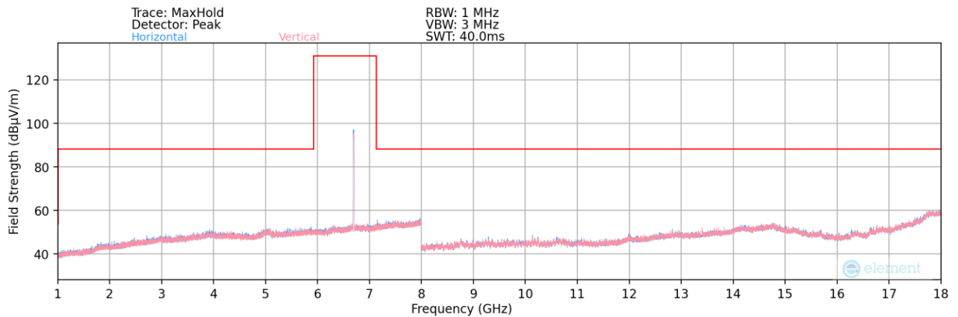
Plot 7-39. Radiated Spurious Plot 1GHz – 18GHz (802.11a – UNII Band 7 Ch. 149)
