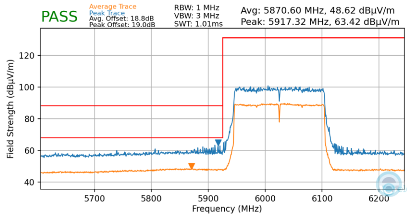
Plot 7-49. Radiated Lower Band Edge Plot SISO (Average & Peak – UNII Band 5)
