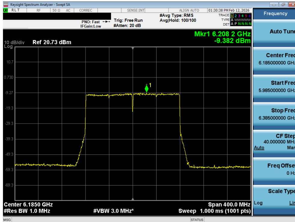
Plot 7-10. Power Spectral Density Plot SISO ANT1 (160MHz 802.11ax (UNII Band 5) – Ch. 47) - LPI
