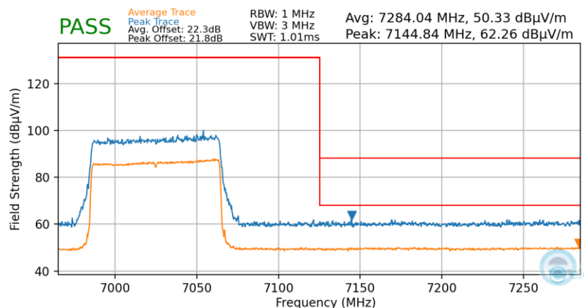
Plot 7-48. Radiated Upper Band Edge Plot SISO (Average & Peak – UNII Band 8)
