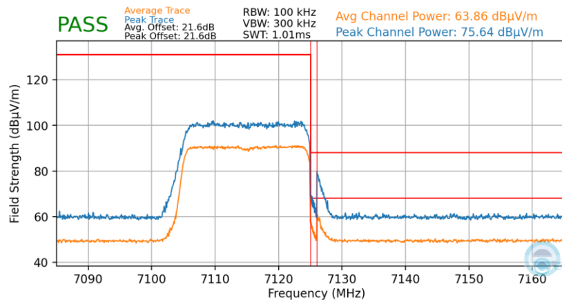
Plot 7-44. Radiated Upper Band Edge Plot SISO (Average & Peak – UNII Band 8)
