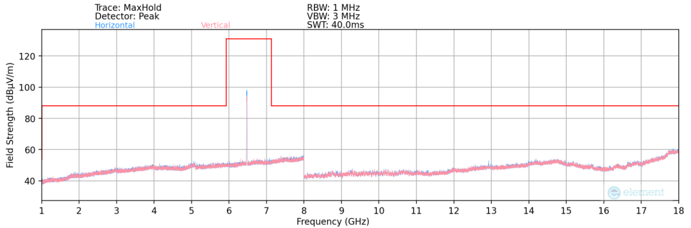
Plot 7-38. Radiated Spurious Plot 1GHz – 18GHz (802.11a – UNII Band 6 Ch. 105)
