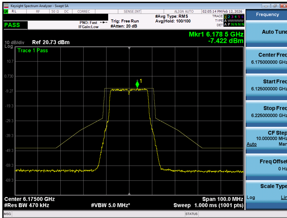
Plot 7-11. In Band Emissions Plot SISO ANT1 (20MHz 802.11a (UNII Band 5) – Ch. 45) - LPI
