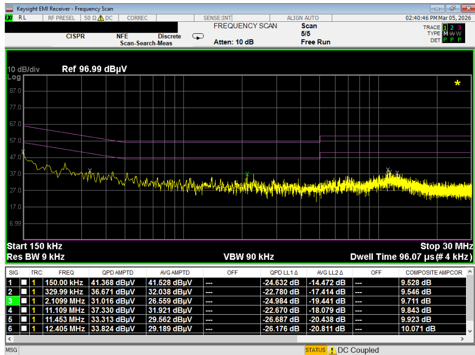
Plot 7-56. Line Conducted Plot with 802.11a UNII Band 7 (N)
