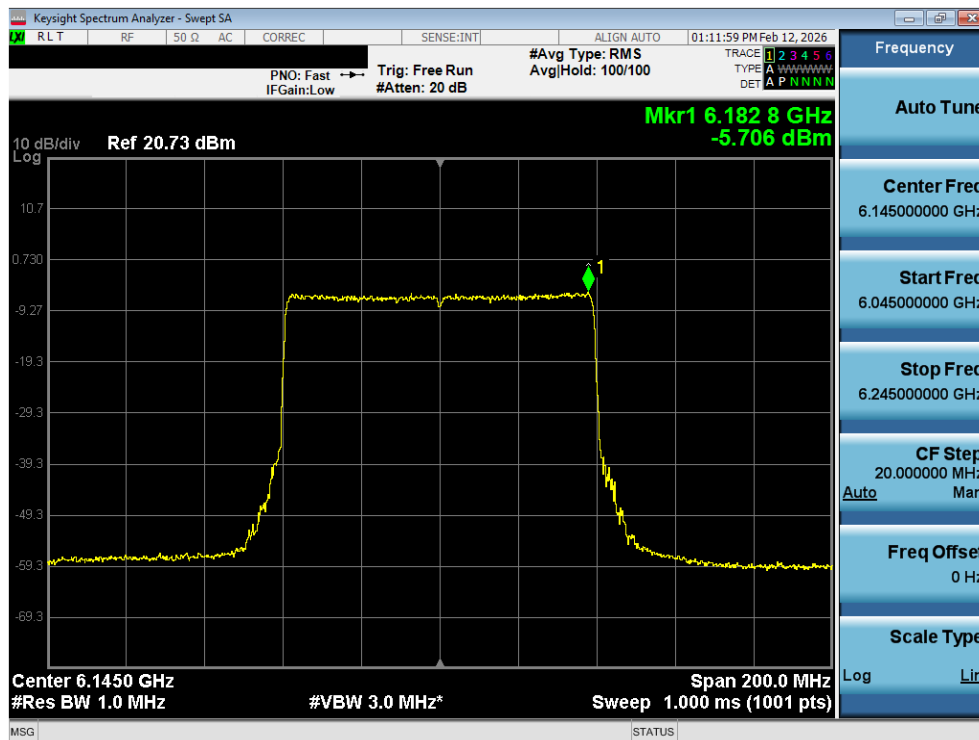
Plot 7-9. Power Spectral Density Plot SISO ANT1 (80MHz 802.11ax (UNII Band 5) – Ch. 39) - LPI
