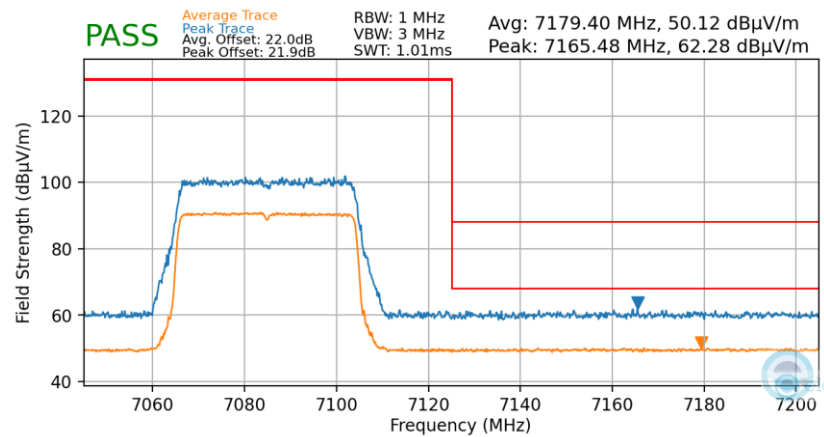
Plot 7-46. Radiated Upper Band Edge Plot SISO (Average & Peak – UNII Band 8)
