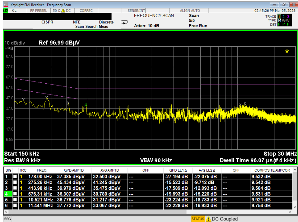
Plot 7-58. Line Conducted Plot with 802.11a UNII Band 8 (N)
