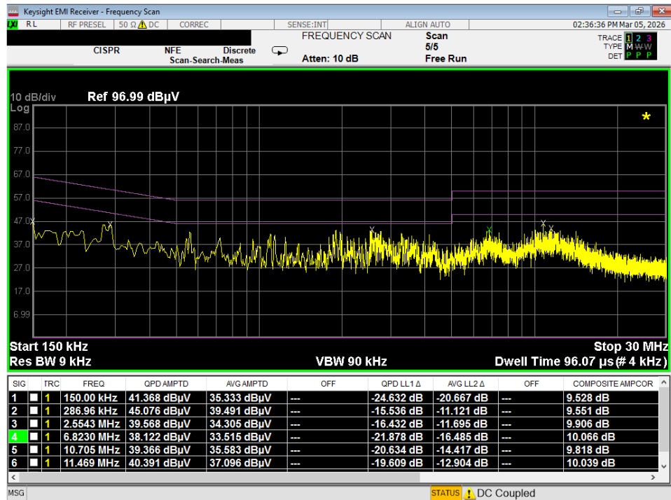
Plot 7-53. Line Conducted Plot with 802.11a UNII Band 6 (L1)
