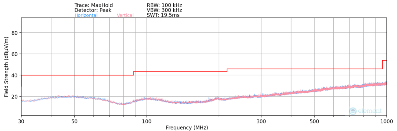
Plot 7-36. Radiated Spurious Plot below 1GHz (802.11a)
