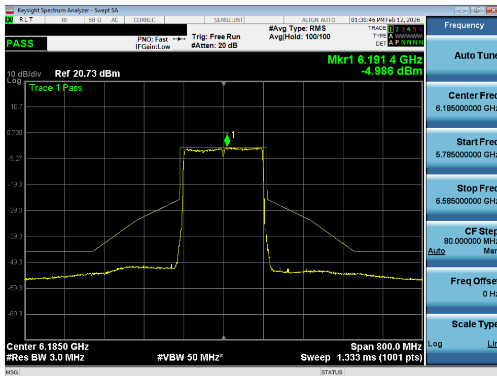
Plot 7-15. In Band Emissions Plot SISO ANT1 (160MHz 802.11ax (UNII Band 5) – Ch. 47) - LPI
