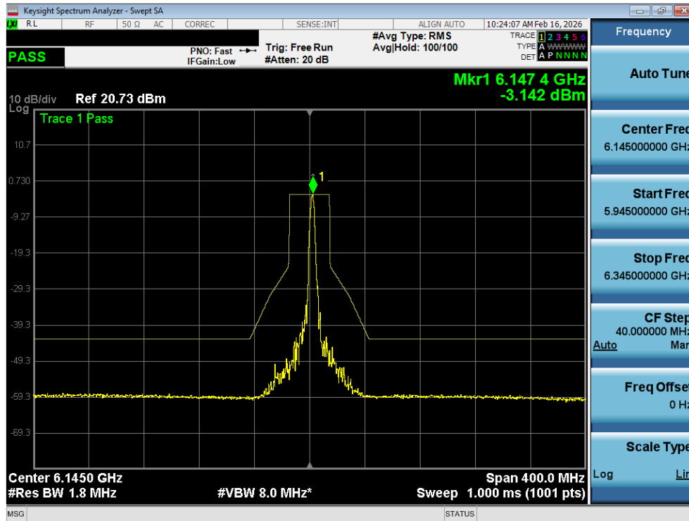
Plot 7-19. In Band Emissions Plot SISO ANT1 (80MHz 802.11ax (26 Tones) (UNII Band 5) – Ch. 39) - LPI
