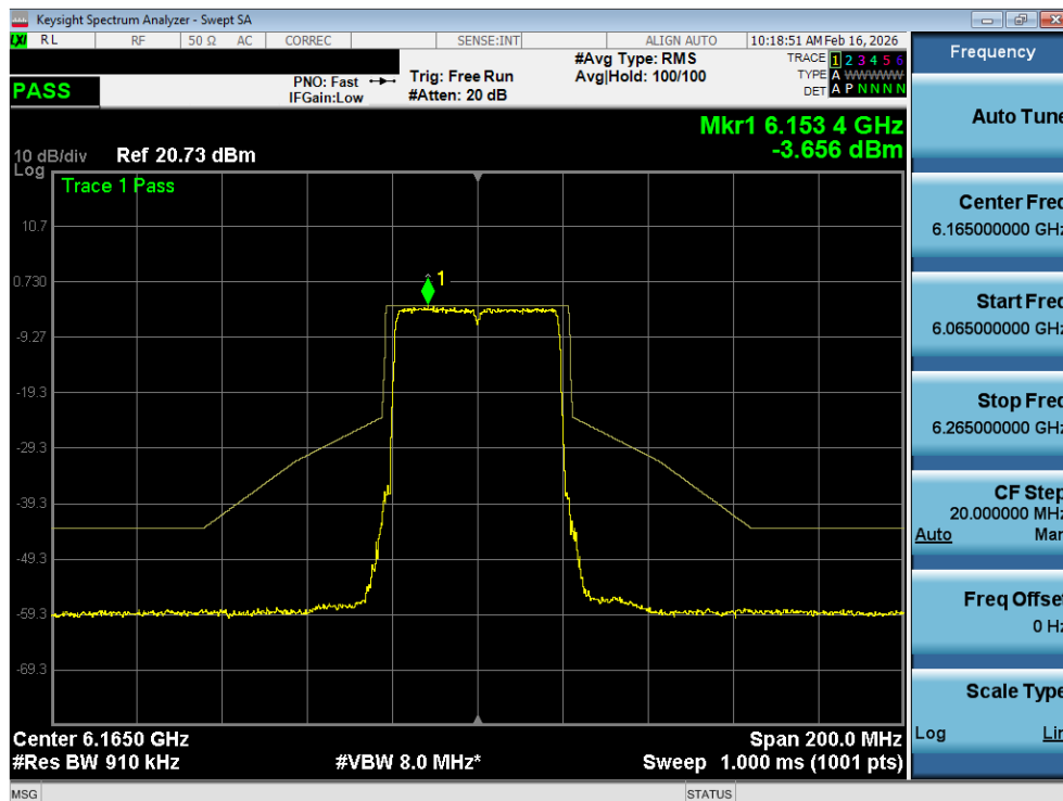
Plot 7-22. In Band Emissions Plot SISO ANT1 (40MHz 802.11ax (Full Tones) (UNII Band 5) – Ch. 43) - LPI
