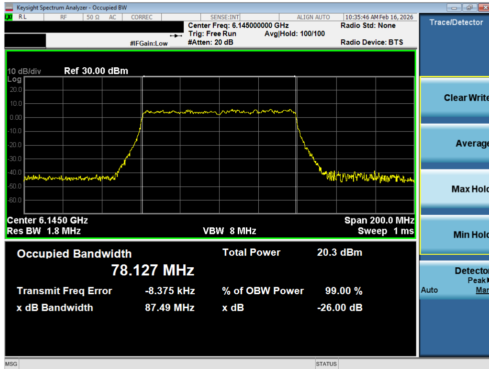
Plot 7-7. 26dB Bandwidth Plot SISO ANT1 (80MHz 802.11ax (Full Tones) (UNII Band 5) – Ch. 39) - LPI
