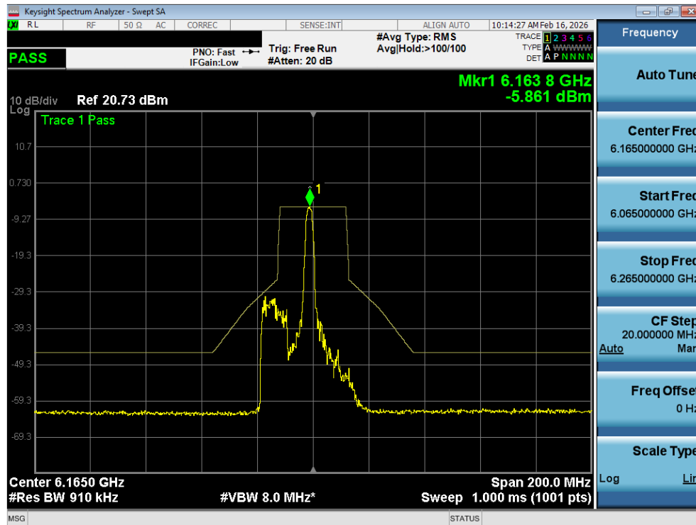
Plot 7-18. In Band Emissions Plot SISO ANT1 (40MHz 802.11ax (26 Tones) (UNII Band 5) – Ch. 43) - LPI
