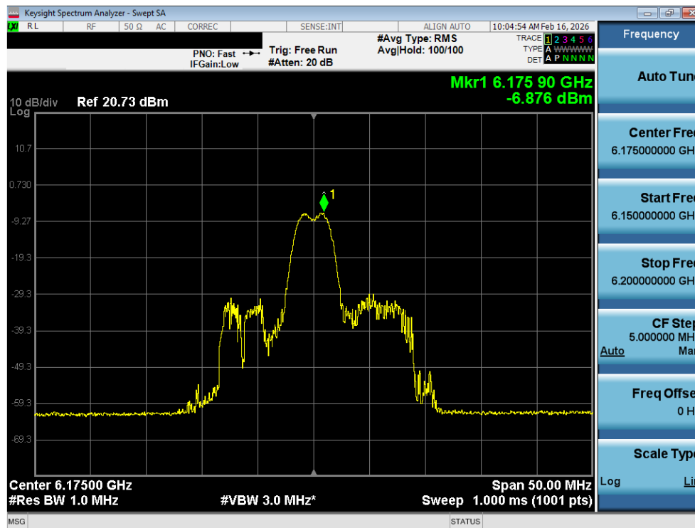
Plot 7-9. Power Spectral Density Plot SISO ANT1 (20MHz 802.11ax (26 Tones) (UNII Band 5) – Ch. 45) - LPI
