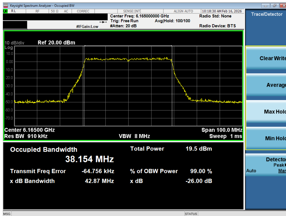
Plot 7-6. 26dB Bandwidth Plot SISO ANT1 (40MHz 802.11ax (Full Tones) (UNII Band 5) – Ch. 43) - LPI
