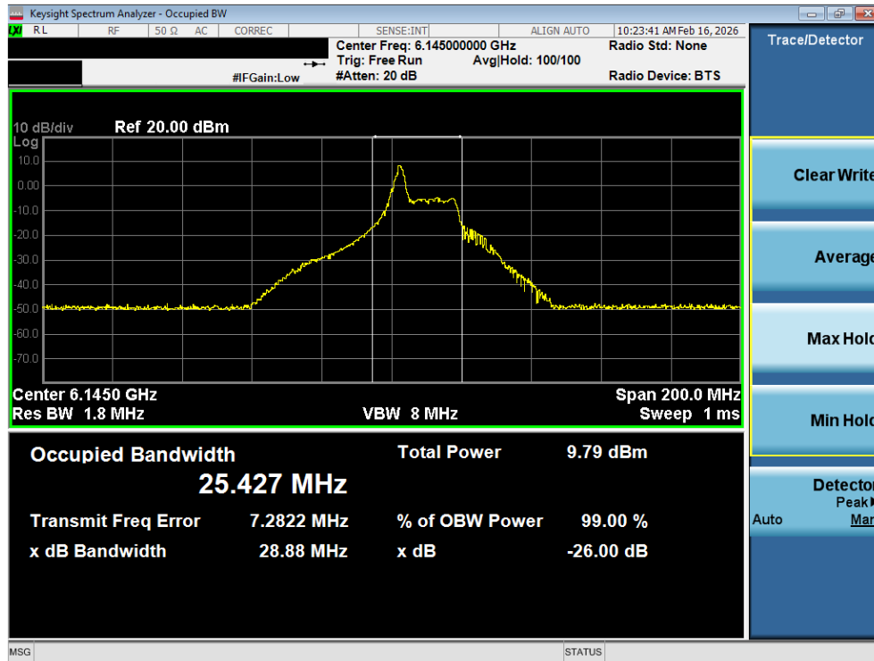
Plot 7-3. 26dB Bandwidth Plot SISO ANT1 (80MHz 802.11ax (26 Tones) (UNII Band 5) – Ch. 39) - LPI
