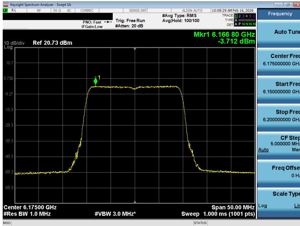
Plot 7-13. Power Spectral Density Plot SISO ANT1 (20MHz 802.11ax (Full Tones) (UNII Band 5) – Ch. 45) - LPI
