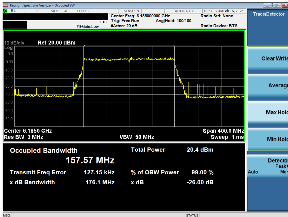
Plot 7-8. 26dB Bandwidth Plot SISO ANT1 (160MHz 802.11ax (Full Tones) (UNII Band 5) – Ch. 47) - LPI
