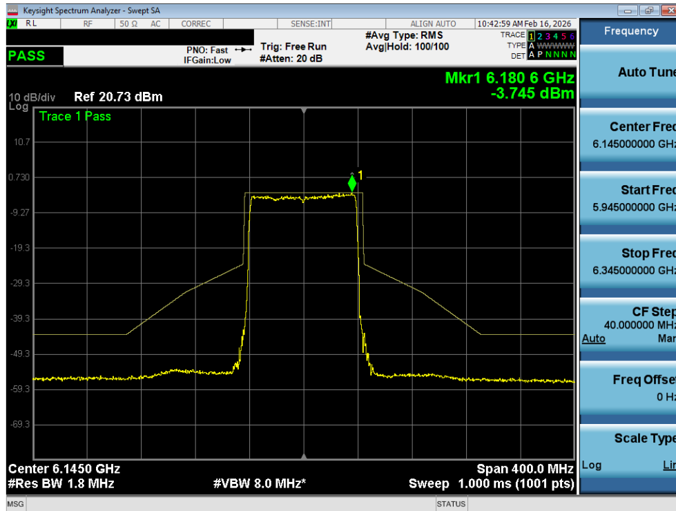
Plot 7-23. In Band Emissions Plot SISO ANT1 (80MHz 802.11ax (Full Tones) (UNII Band 5) – Ch. 39) - LPI
