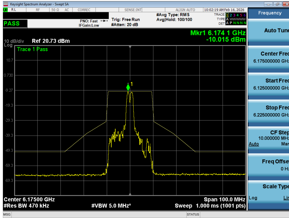
Plot 7-17. In Band Emissions Plot SISO ANT1 (20MHz 802.11ax (26 Tones) (UNII Band 5) – Ch. 45) - LPI
