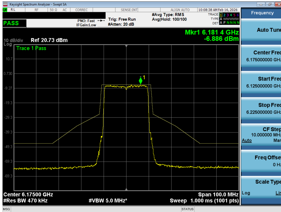
Plot 7-21. In Band Emissions Plot SISO ANT1 (20MHz 802.11ax (Full Tones) (UNII Band 5) – Ch. 45) - LPI
