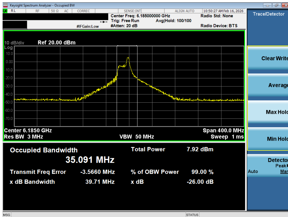
Plot 7-4. 26dB Bandwidth Plot SISO ANT1 (160MHz 802.11ax (26 Tones) (UNII Band 5) – Ch. 47) - LPI
