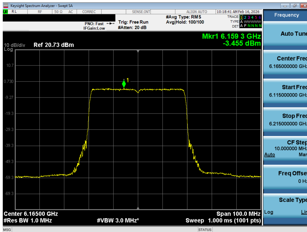
Plot 7-14. Power Spectral Density Plot SISO ANT1 (40MHz 802.11ax (Full Tones) (UNII Band 5) – Ch. 43) - LPI
