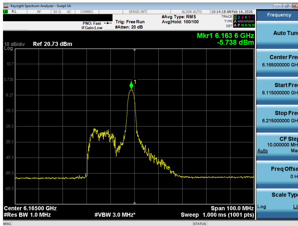
Plot 7-10. Power Spectral Density Plot SISO ANT1 (40MHz 802.11ax (26 Tones) (UNII Band 5) – Ch. 43) - LPI
