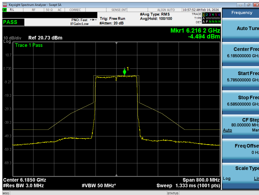
Plot 7-24. In Band Emissions Plot SISO ANT1 (160MHz 802.11ax (Full Tones) (UNII Band 5) – Ch. 47) - LPI
