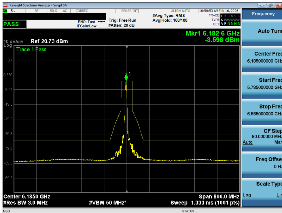
Plot 7-20. In Band Emissions Plot SISO ANT1 (160MHz 802.11ax (26 Tones) (UNII Band 5) – Ch. 47) - LPI
