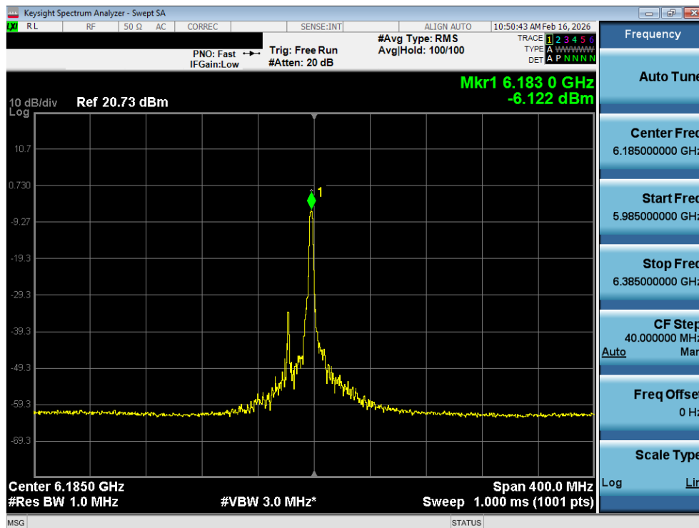
Plot 7-12. Power Spectral Density Plot SISO ANT1 (160MHz 802.11ax (26 Tones) (UNII Band 5) – Ch. 47) - LPI
