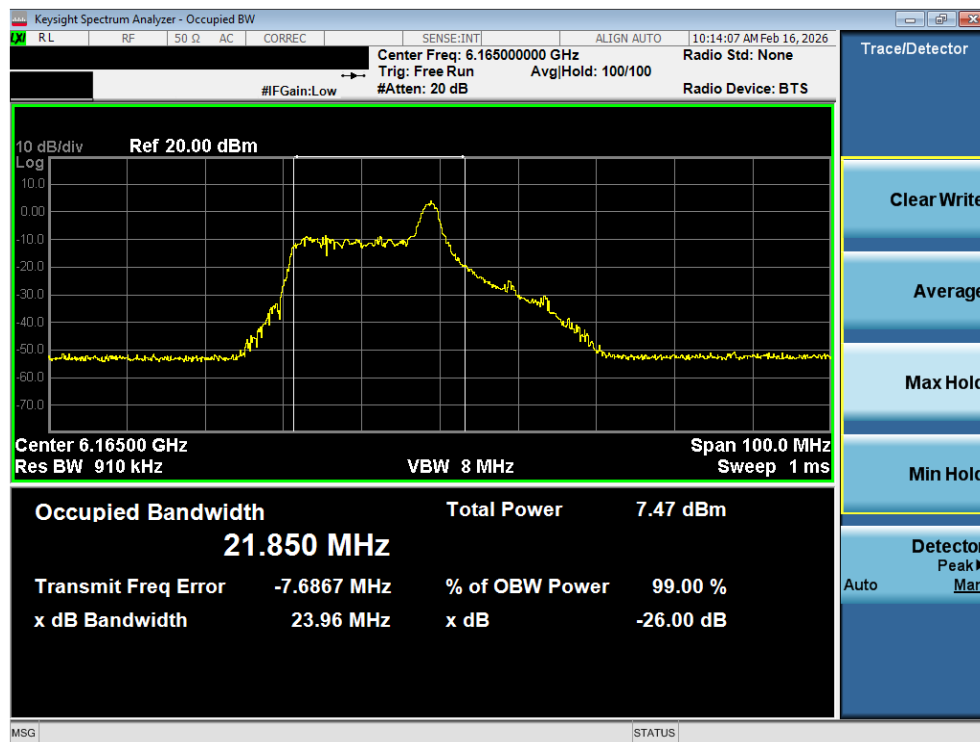
Plot 7-2. 26dB Bandwidth Plot SISO ANT1 (40MHz 802.11ax (26 Tones) (UNII Band 5) – Ch. 43) - LPI
