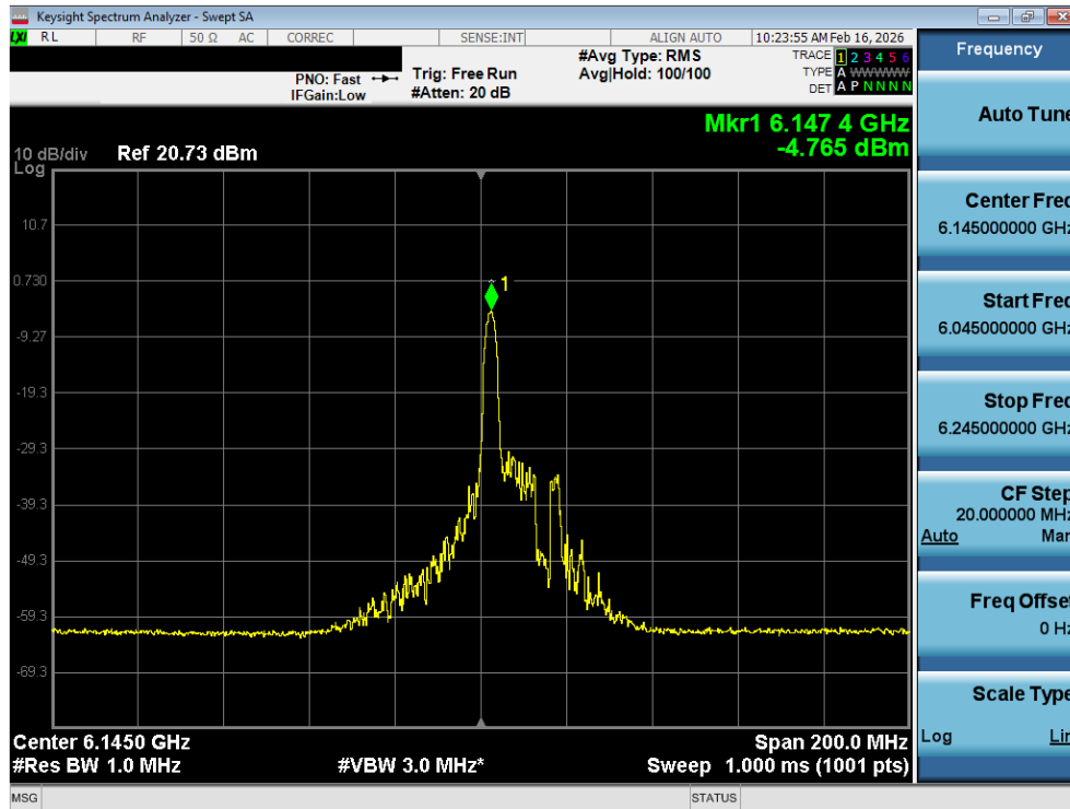
Plot 7-11. Power Spectral Density Plot SISO ANT1 (80MHz 802.11ax (26 Tones) (UNII Band 5) – Ch. 39) - LPI
