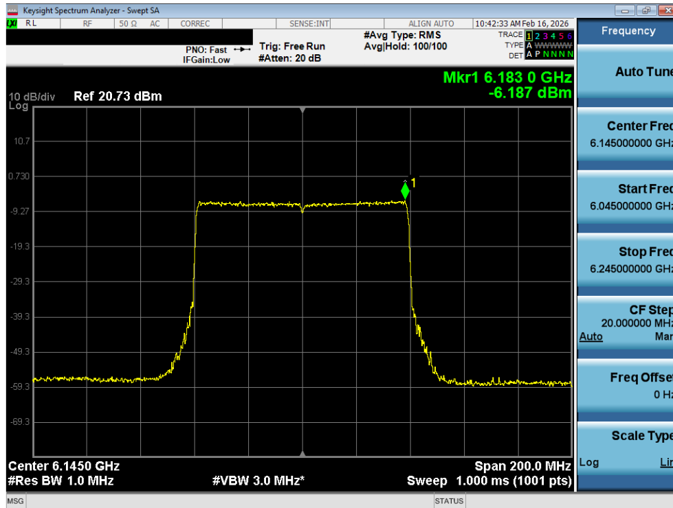
Plot 7-15. Power Spectral Density Plot SISO ANT1 (80MHz 802.11ax (Full Tones) (UNII Band 5) – Ch. 39) - LPI
