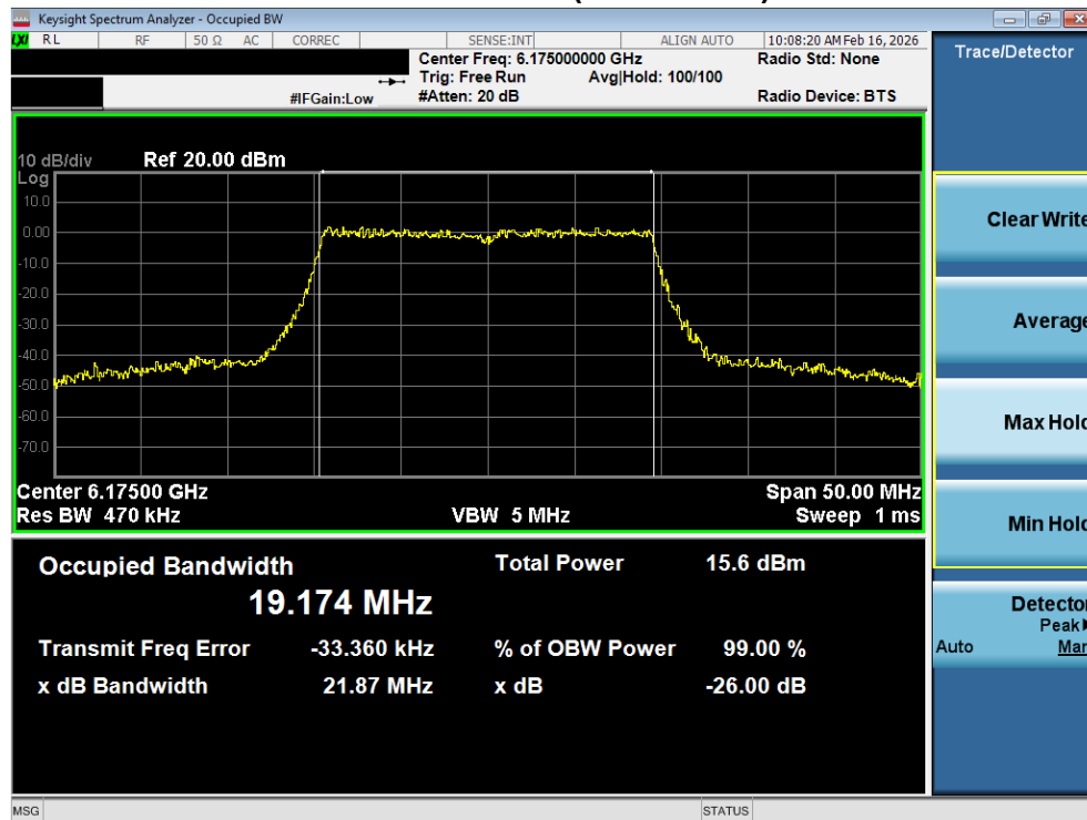
Plot 7-5. 26dB Bandwidth Plot SISO ANT1 (20MHz 802.11ax (Full Tones) (UNII Band 5) – Ch. 45) – LPI
