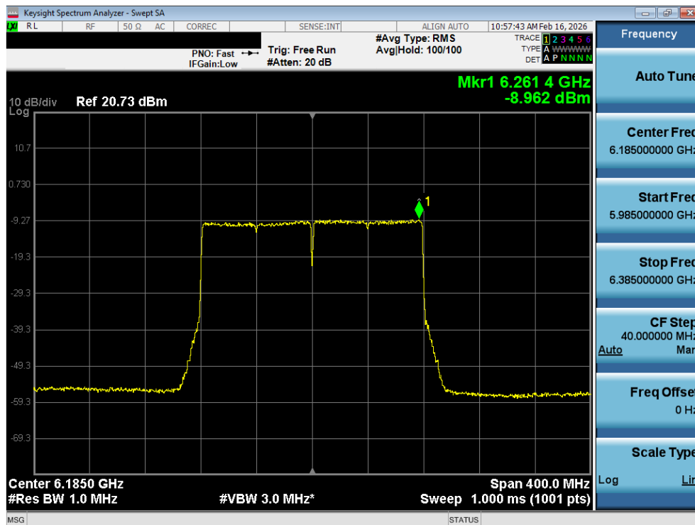
Plot 7-16. Power Spectral Density Plot SISO ANT1 (160MHz 802.11ax (Full Tones) (UNII Band 5) – Ch. 47) - LPI
