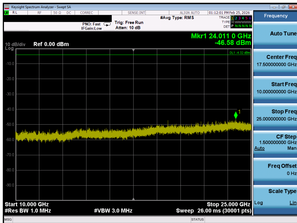
Plot 7-62. Conducted Spurious Plot (Bluetooth (LE), 1Mbps – Ch. 39) – Ant 1
