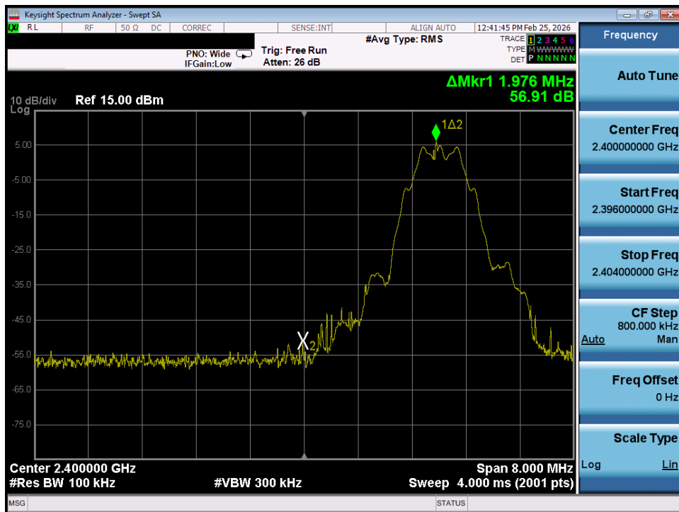
Plot 7-49. Band Edge Plot (Bluetooth (LE), 125kbps – Ch. 37) – Ant 1
