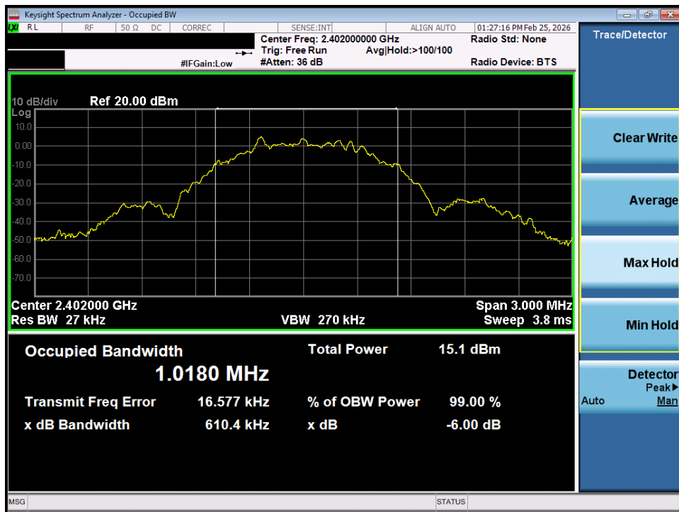
Plot 7-16. OBW Plot (Bluetooth (LE), 500kbps – Ch. 37) – SISO ANT1
