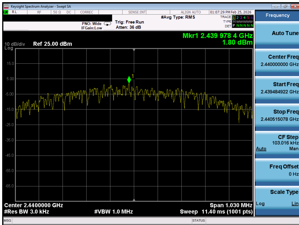
Plot 7-44. Power Spectral Density Plot (Bluetooth (LE), 1Mbps – Ch. 17) – Ant 1
