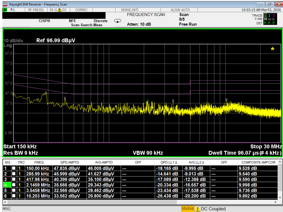
Plot 7-71. Line-Conducted Test Plot (N)
