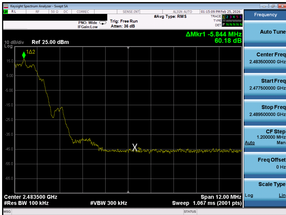
Plot 7-56. Band Edge Plot (Bluetooth (LE), 2Mbps - Ch. 36) - Ant 1
