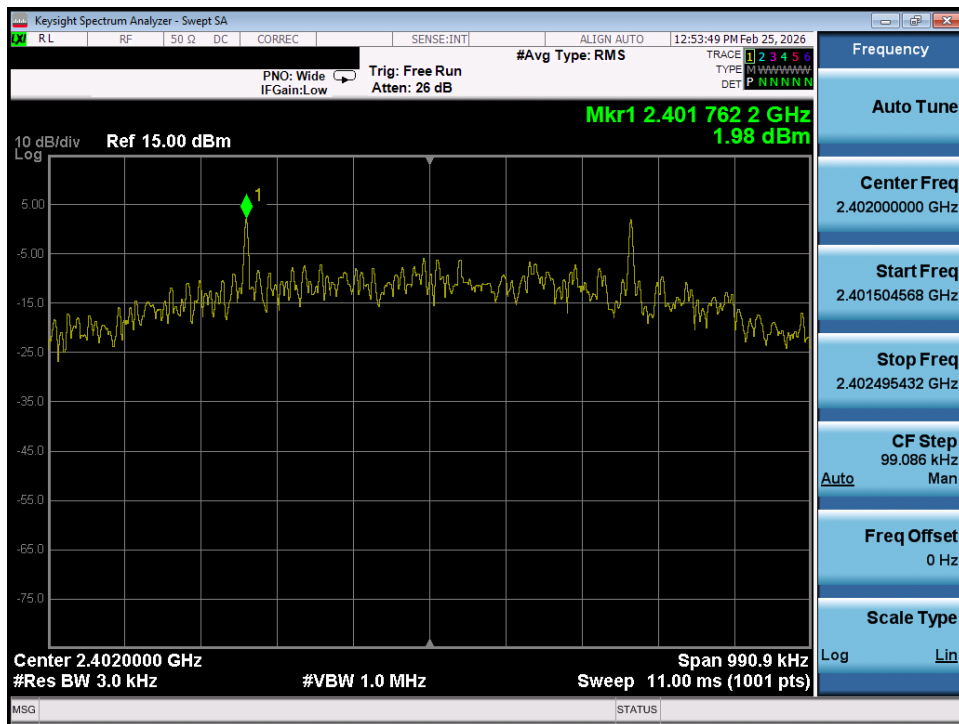
Plot 7-40. Power Spectral Density Plot (Bluetooth (LE), 500kbps – Ch. 37) – Ant 1
