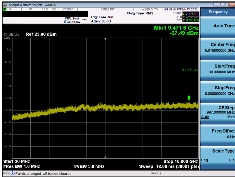
Plot 7-59. Conducted Spurious Plot (Bluetooth (LE), 1Mbps - Ch. 17) - Ant 1
