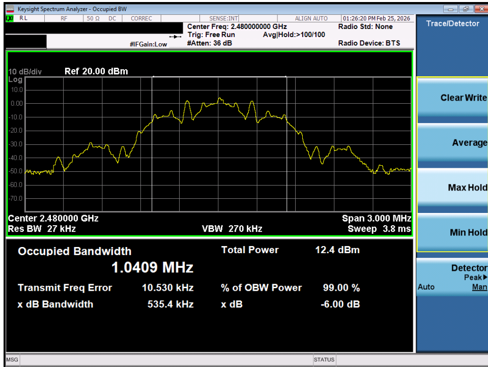
Plot 7-15. OBW Plot (Bluetooth (LE), 125kbps – Ch. 39) – SISO ANT1
