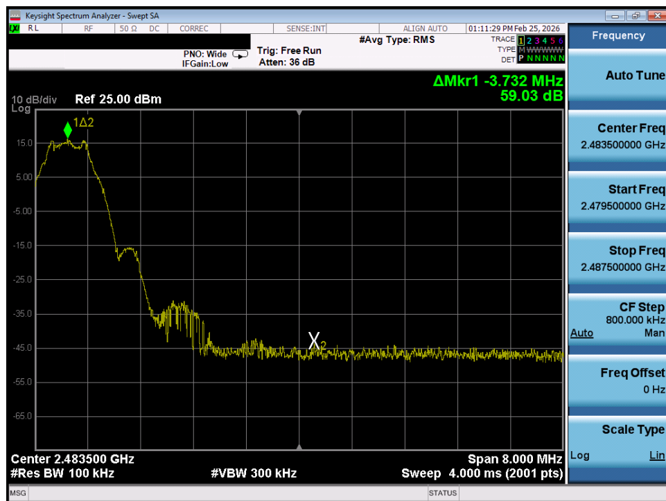
Plot 7-54. Band Edge Plot (Bluetooth (LE), 1Mbps - Ch. 39) - Ant 1
