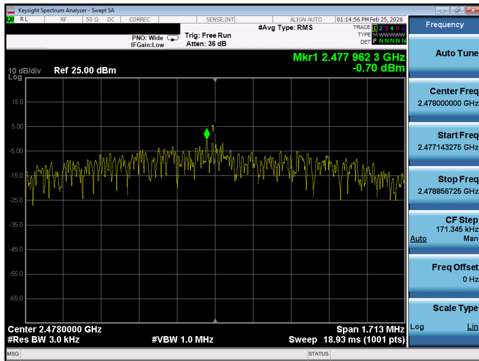
Plot 7-48. Power Spectral Density Plot (Bluetooth (LE), 2Mbps – Ch. 36) – Ant 1
