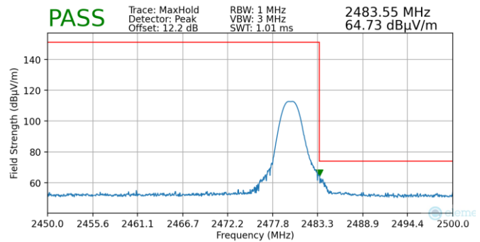
Plot 7-68. Radiated Restricted Upper Band Edge Measurement (Peak) – Ant 1
