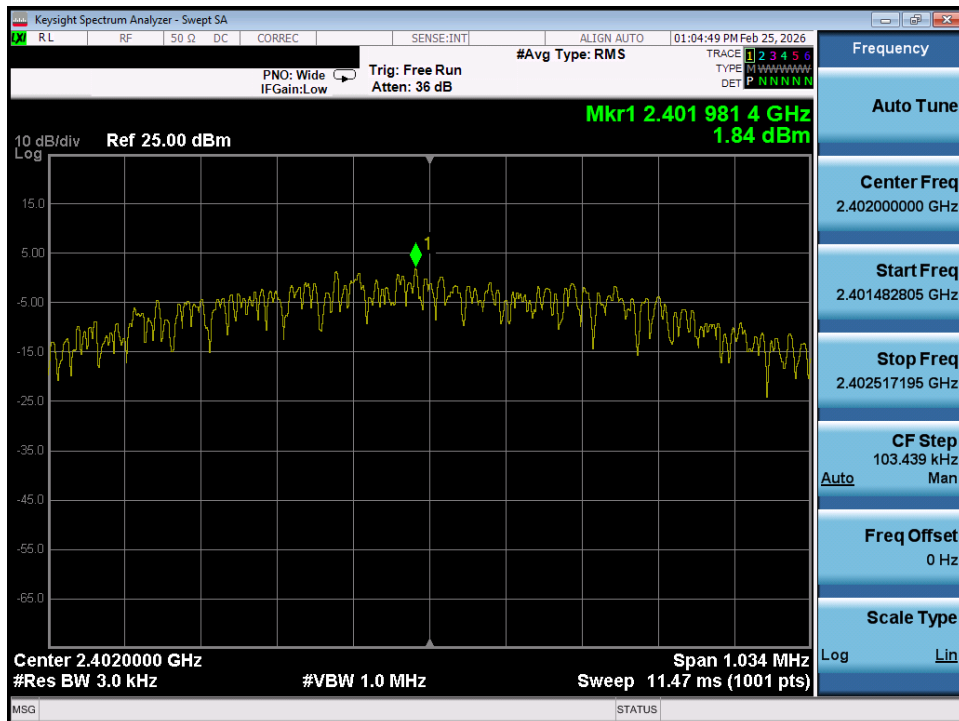
Plot 7-43. Power Spectral Density Plot (Bluetooth (LE), 1Mbps – Ch. 37) – Ant 1
