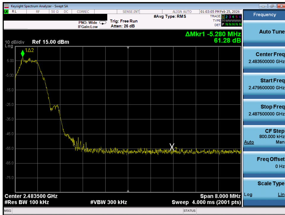
Plot 7-52. Band Edge Plot (Bluetooth (LE), 500kbps – Ch. 39) – Ant 1
