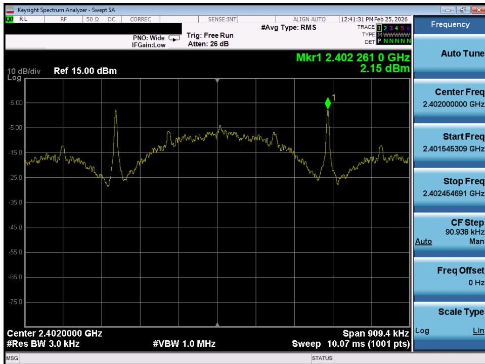
Plot 7-37. Power Spectral Density Plot (Bluetooth (LE), 125kbps – Ch. 37) – Ant 1
