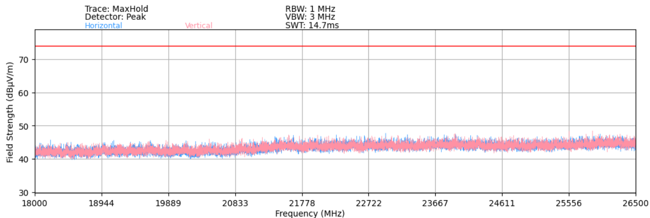
Plot 7-66. Radiated Spurious Plot above 18GHz (Bluetooth (LE)) – Ant 1
