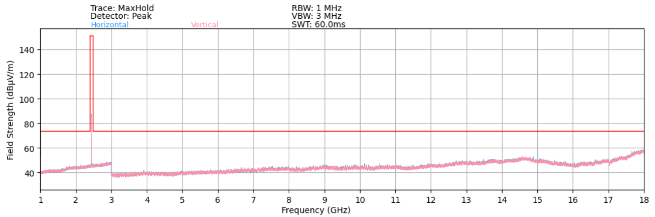
Plot 7-64. Radiated Spurious Plot above 1GHz (Bluetooth (LE) – Ch. 17) – Ant 1
