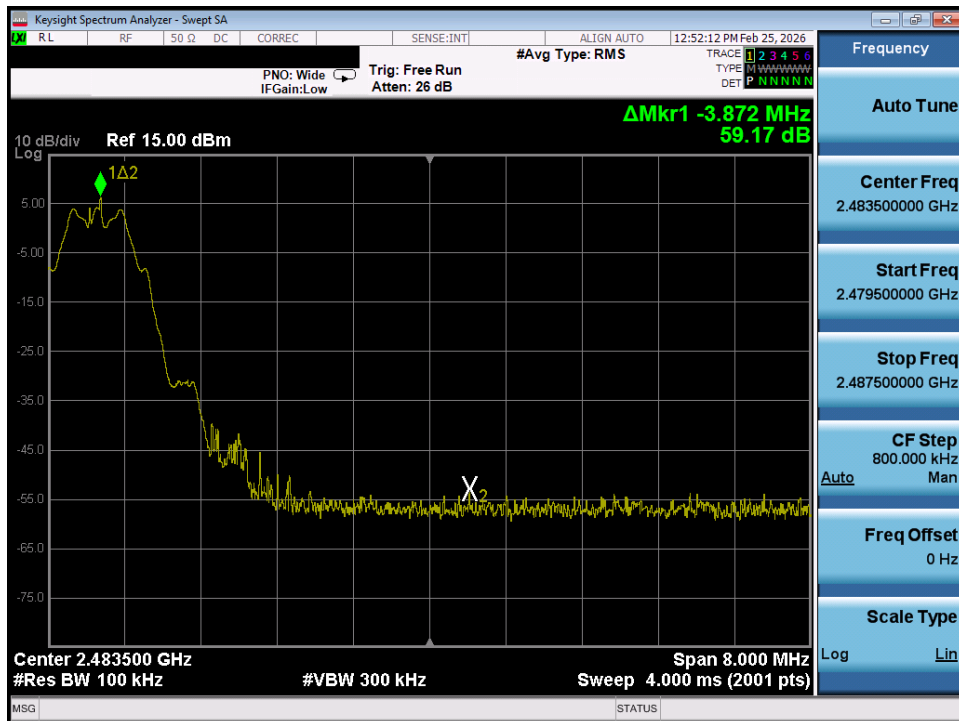
Plot 7-50. Band Edge Plot (Bluetooth (LE), 125kbps – Ch. 39) – Ant 1
