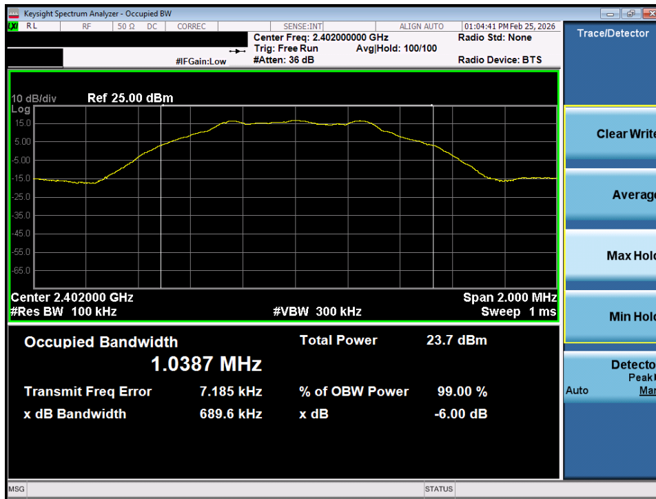
Plot 7-7. 6dB Bandwidth Plot (Bluetooth (LE), 1Mbps - Ch. 37) - Ant 1
