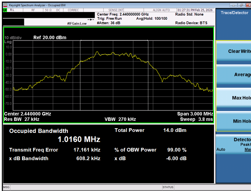
Plot 7-17. OBW Plot (Bluetooth (LE), 500kbps – Ch. 17) – SISO ANT1
