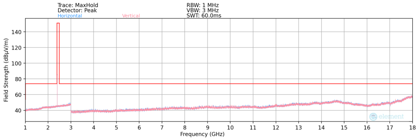
Plot 7-63. Radiated Spurious Plot above 1GHz (Bluetooth (LE) – Ch. 37) – Ant 1
