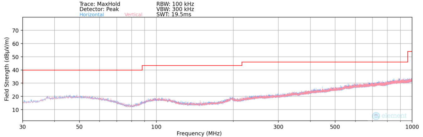
Plot 7-69. Radiated Spurious Plot below 1GHz – Ant 1
