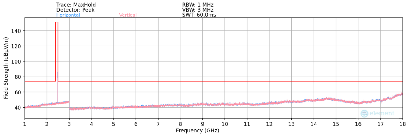
Plot 7-65. Radiated Spurious Plot above 1GHz (Bluetooth (LE) – Ch. 39) – Ant 1
