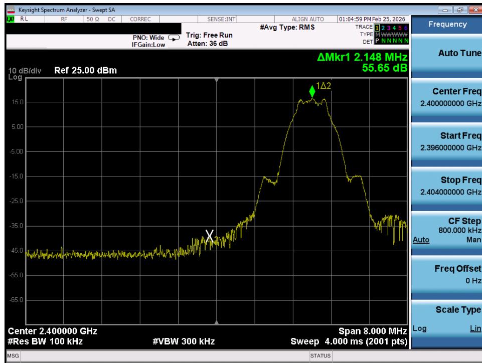
Plot 7-53. Band Edge Plot (Bluetooth (LE), 1Mbps - Ch. 37) - Ant 1
