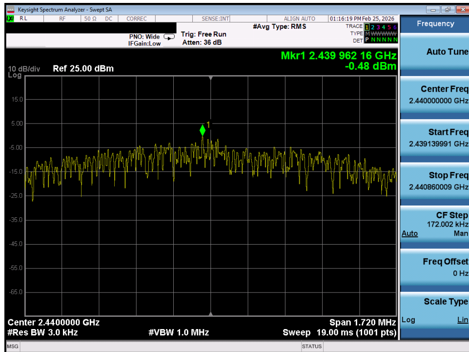
Plot 7-47. Power Spectral Density Plot (Bluetooth (LE), 2Mbps – Ch. 17) – Ant 1
