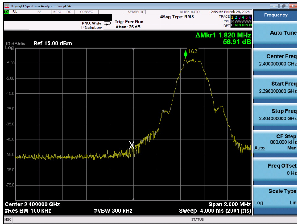
Plot 7-51. Band Edge Plot (Bluetooth (LE), 500kbps – Ch. 37) – Ant 1
