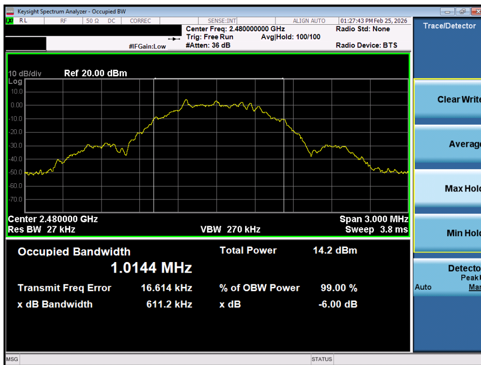
Plot 7-18. OBW Plot (Bluetooth (LE), 500kbps – Ch. 39) – SISO ANT1
