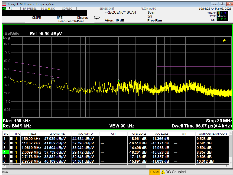
Plot 7-70. Line-Conducted Test Plot (L1)
