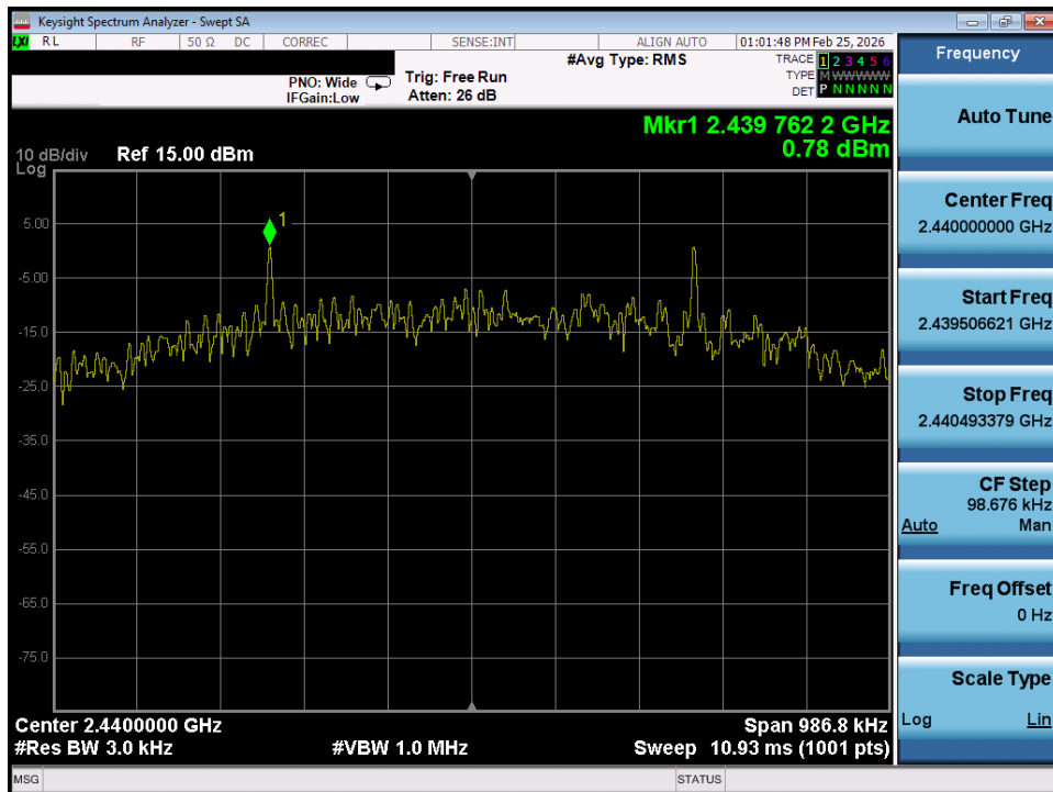
Plot 7-41. Power Spectral Density Plot (Bluetooth (LE), 500kbps – Ch. 17) – Ant 1
