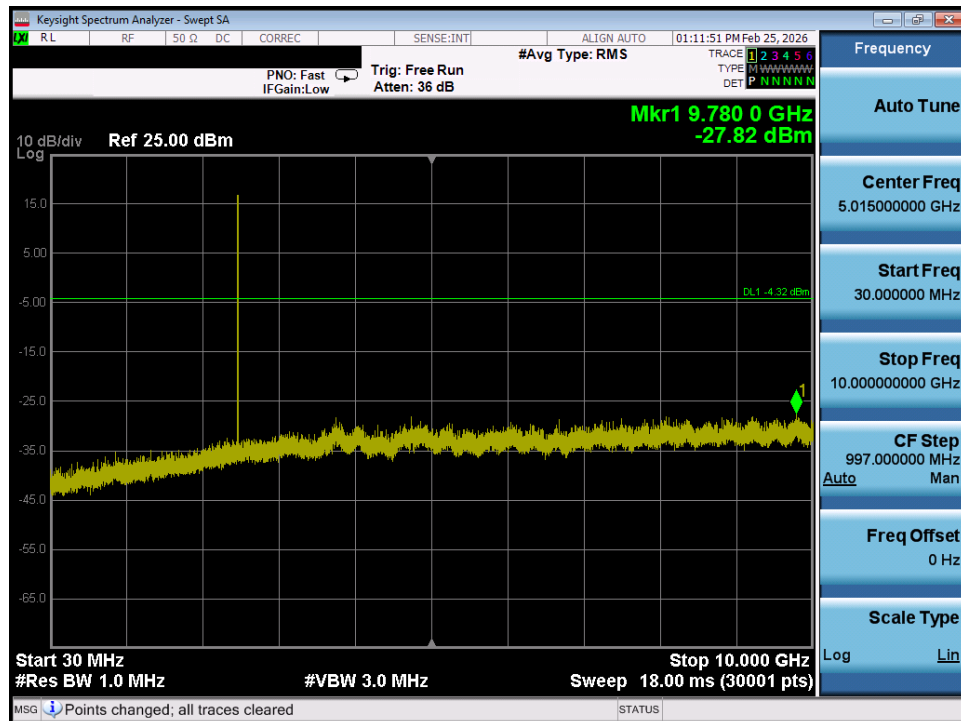
Plot 7-61. Conducted Spurious Plot (Bluetooth (LE), 1Mbps – Ch. 39) – Ant 1
