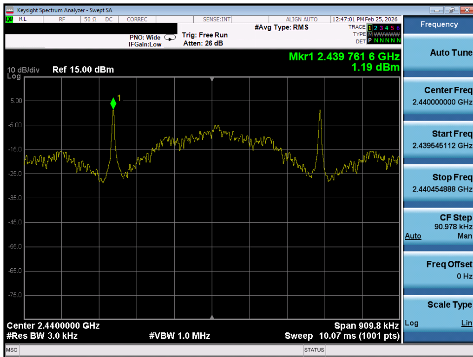
Plot 7-38. Power Spectral Density Plot (Bluetooth (LE), 125kbps – Ch. 17) – Ant 1
