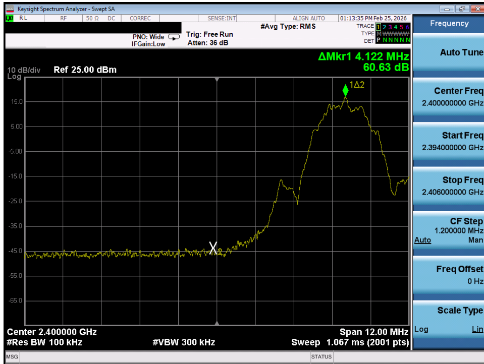
Plot 7-55. Band Edge Plot (Bluetooth (LE), 2Mbps - Ch. 0) - Ant 1
