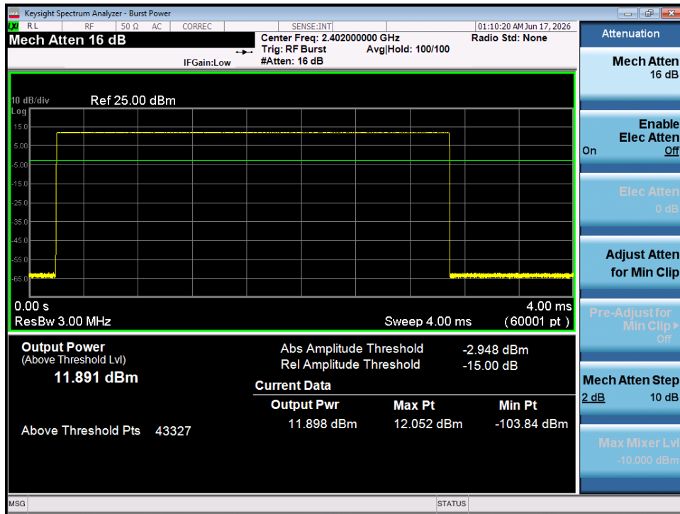
Plot 7-19. Average Conducted Power (1Mbps - Ch. 0) - SISO ANT 1
