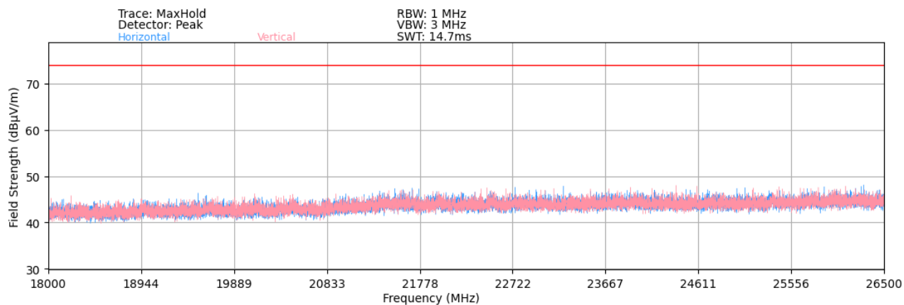
Plot 7-45. Radiated Spurious Plot above 18GHz – Ant 1
