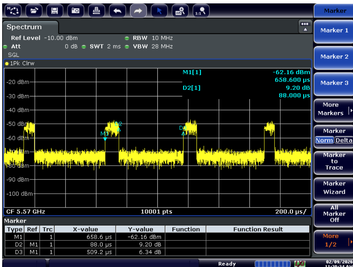
Figure 9-1. Band 2C Channel Loading
