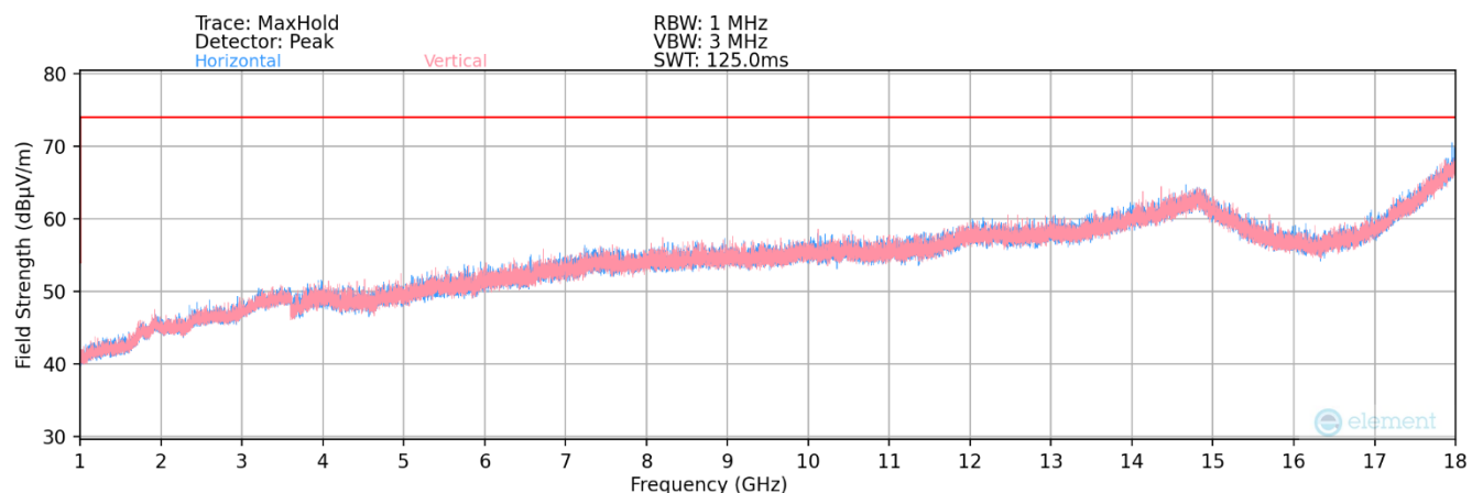
Plot 7-2. Radiated Emissions 1GHz – 18GHz
