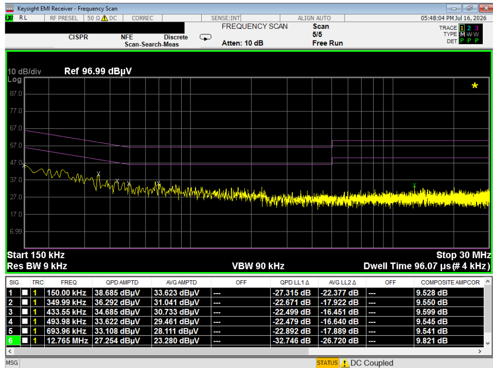
Plot 7-16. Line Conducted Plot (N) – Audio Playback – SM-O200P
