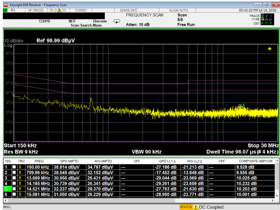
Plot 7-14. Line Conducted Plot (N) – Video Recording – SM-O200P
