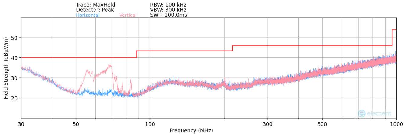
Plot 7-10. Radiated Emissions 30MHz – 1GHz
