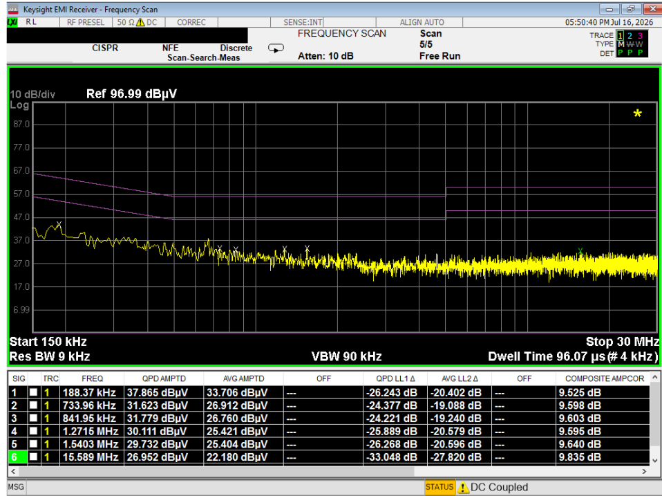
Plot 7-17. Line Conducted Plot (L1) – File Transfer – SM-O200P
