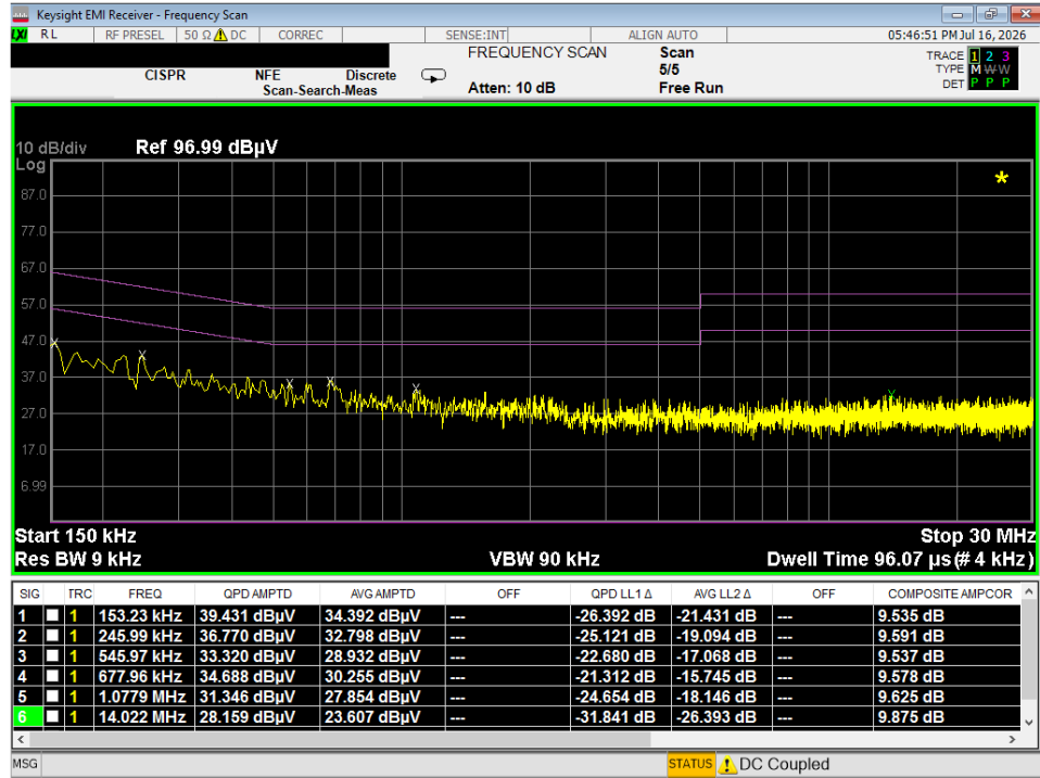
Plot 7-15. Line Conducted Plot (L1) – Audio Playback – SM-O200P
