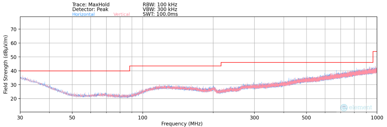
Plot 7-3. Radiated Emissions 30MHz – 1GHz
