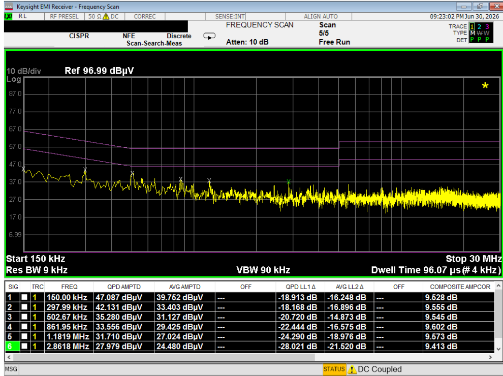
Plot 7-19. Line Conducted Plot (L1) – Charging Case – SM-O200P
