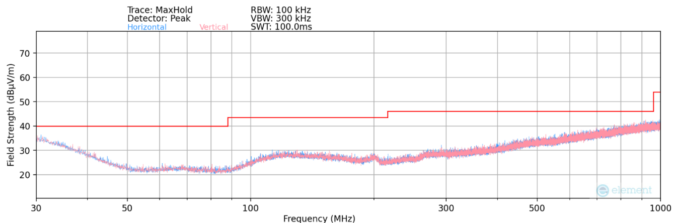
Plot 7-5. Radiated Emissions 30MHz – 1GHz
