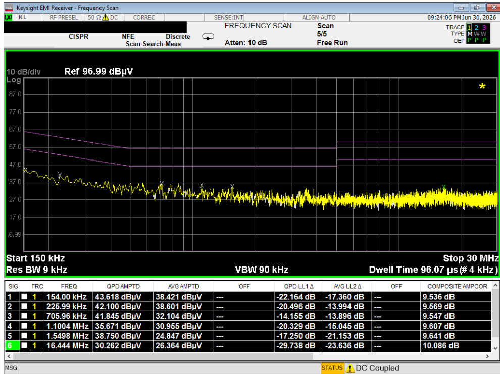
Plot 7-20. Line Conducted Plot (N) – Charging Case – SM-O200P
