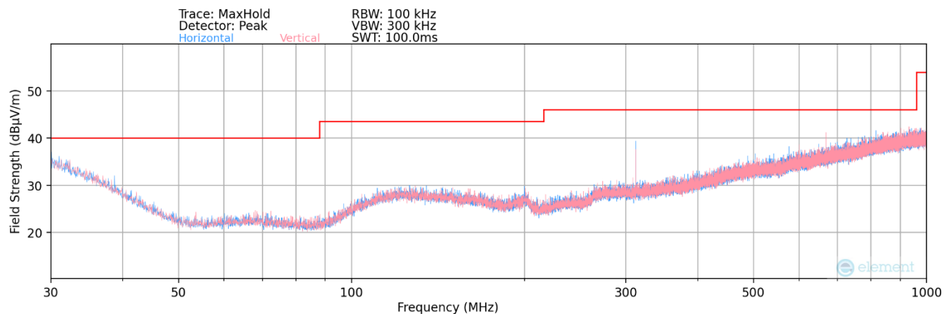
Plot 7-1. Radiated Emissions 30MHz – 1GHz
