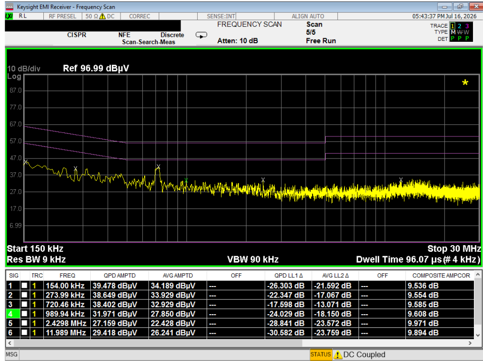
Plot 7-13. Line Conducted Plot (L1) – Video Recording – SM-O200P
