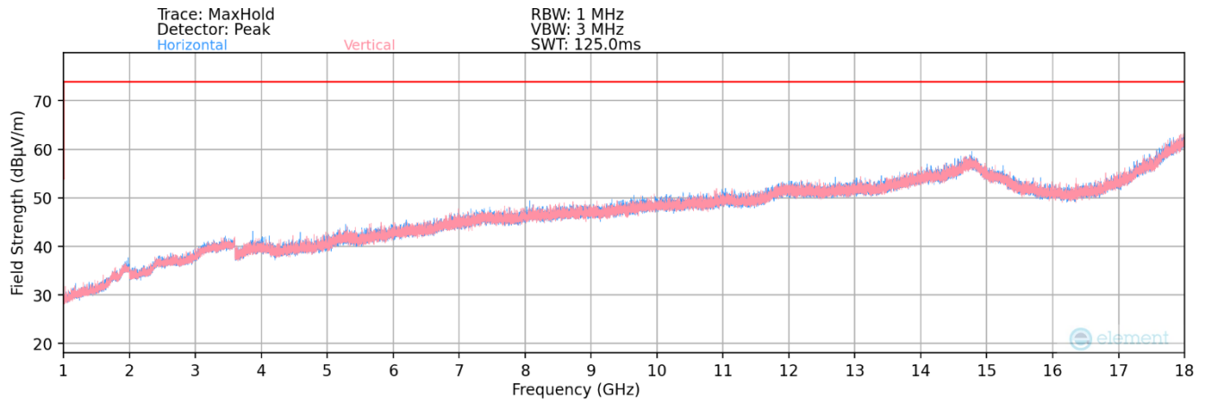
Plot 7-4. Radiated Emissions 1GHz – 18GHz
