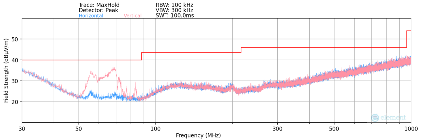
Plot 7-11. Radiated Emissions 30MHz – 1GHz
