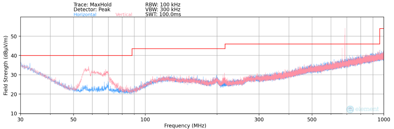
Plot 7-12. Radiated Emissions 30MHz – 1GHz
