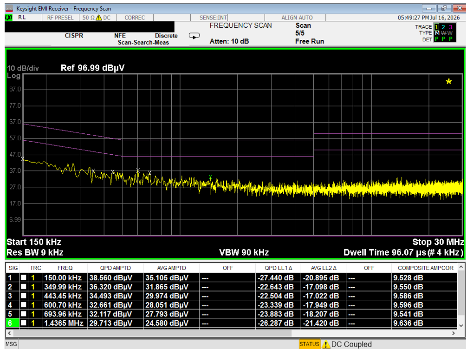
Plot 7-18. Line Conducted Plot (N) – File Transfer – SM-O200P
