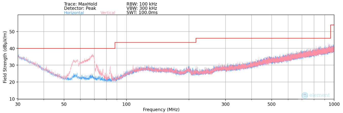
Plot 7-9. Radiated Emissions 30MHz – 1GHz
