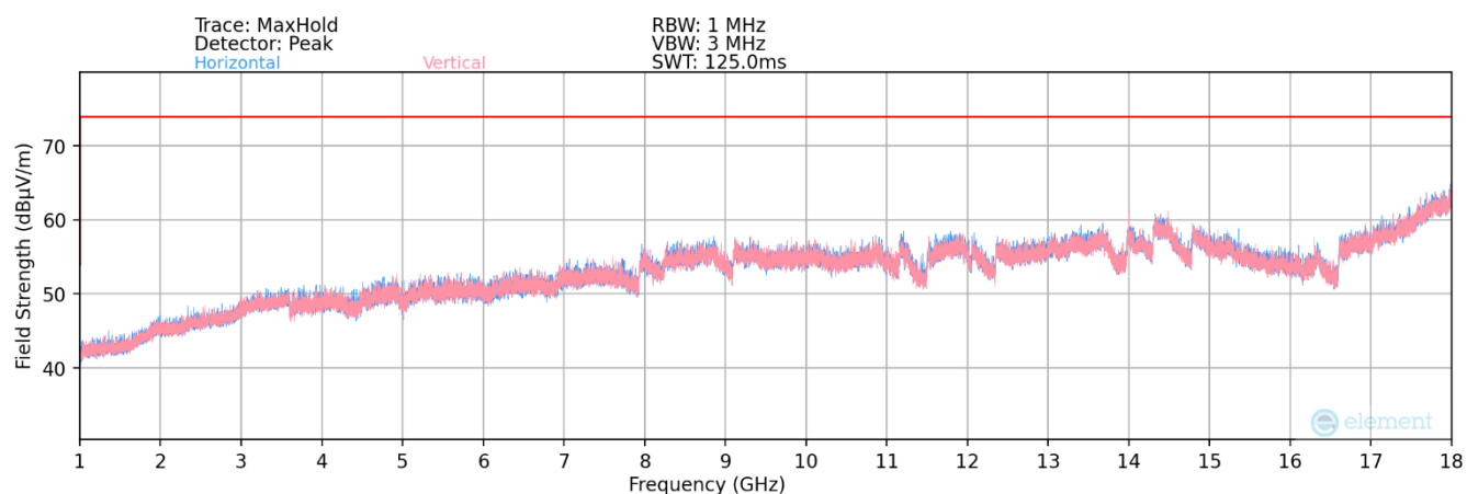
Plot 7-6. Radiated Emissions 1GHz – 18GHz
