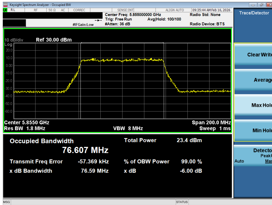
Plot 7-38. OBW Plot SISO ANT1 (80MHz BW 802.11ac (UNII Band 3/4) – Ch. 171)
