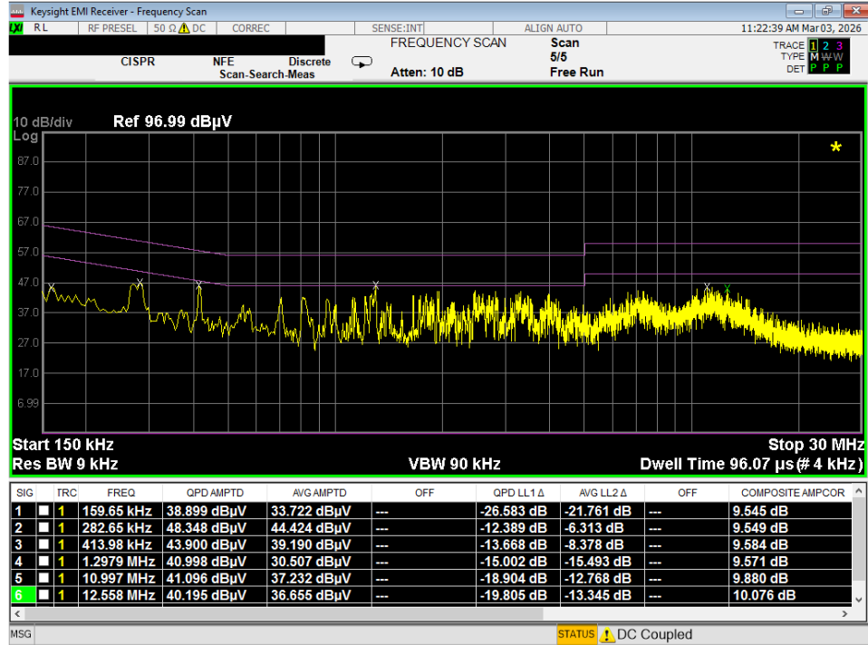
Plot 7-100. Line Conducted Plot with 802.11a UNII Band 2A (L1)
