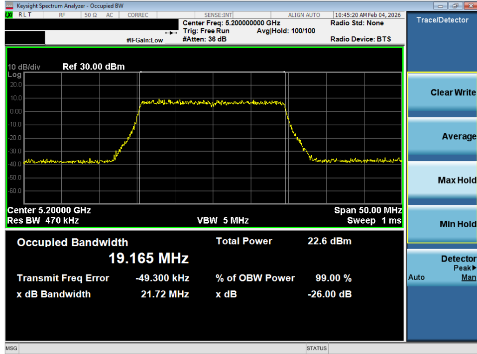
Plot 7-3. 26dB Bandwidth Plot SISO ANT1 (20MHz BW 802.11ax (UNII Band 1) – Ch. 40)
