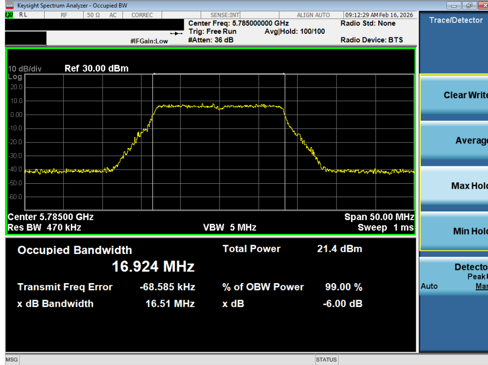
Plot 7-26. OBW Plot SISO ANT1 (802.11a (UNII Band 3) – Ch. 157)
