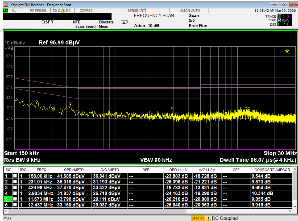
Plot 7-103. Line Conducted Plot with 802.11a UNII Band 2C (N)
