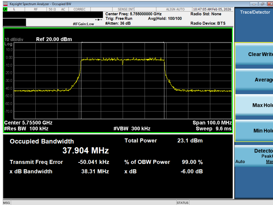
Plot 7-14. 6dB Bandwidth Plot SISO ANT1 (40MHz BW 802.11ax (UNII Band 3) – Ch. 151)
