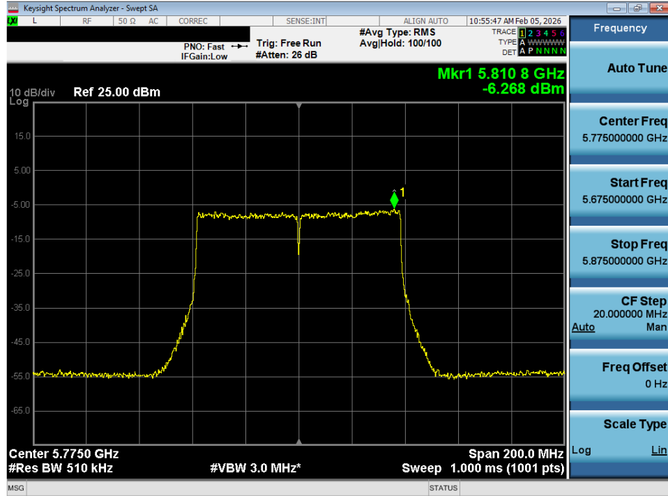
Plot 7-56. Power Spectral Density Plot SISO ANT1 (80MHz BW 802.11ac (UNII Band 3) – Ch. 155)
