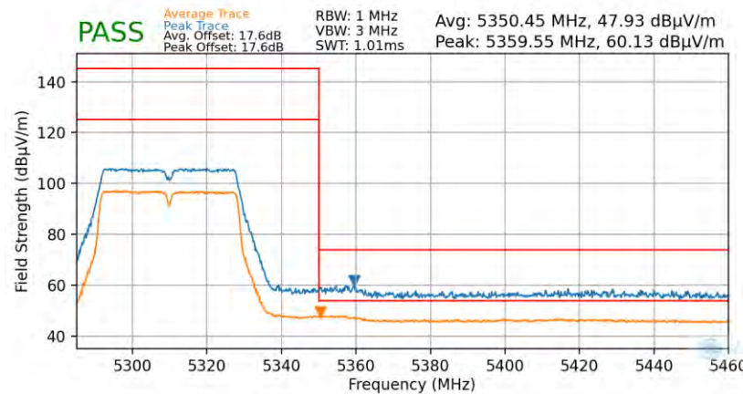
Plot 7-82. Radiated Upper Band Edge Plot (Average & Peak – UNII Band 2A)
