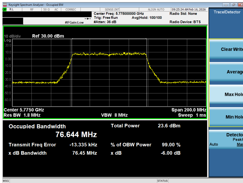
Plot 7-31. OBW Plot SISO ANT1 (80MHz BW 802.11ac (UNII Band 3) – Ch. 155)
