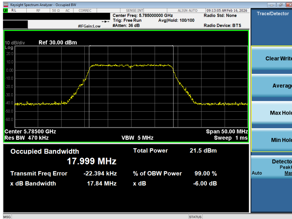
Plot 7-27. OBW Plot SISO ANT1 (20MHz BW 802.11n (UNII Band 3) – Ch. 157)
