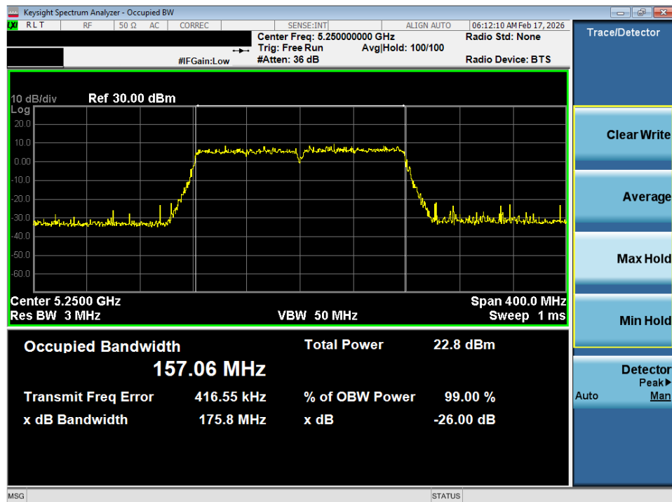
Plot 7-8. 26dB Bandwidth Plot SISO ANT1 (160MHz BW 802.11ac (UNII Band 1/2A) – Ch. 50)
