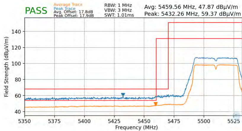
Plot 7-83. Radiated Lower Band Edge Plot (Average & Peak – UNII Band 2C)
