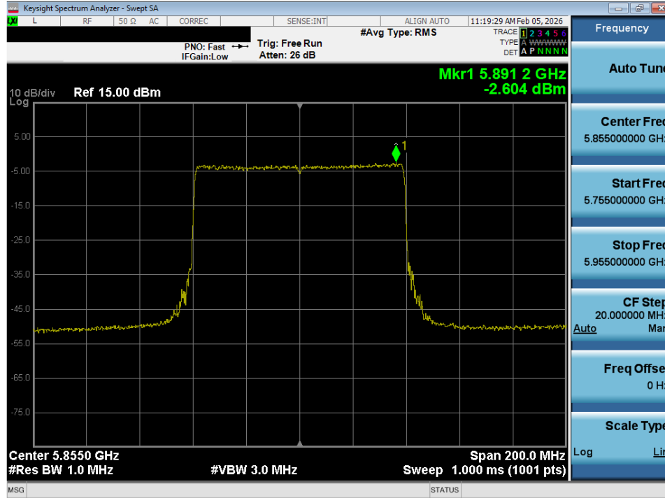
Plot 7-64. Power Spectral Density Plot SISO ANT1 (80MHz BW 802.11ax (UNII Band 3/4) – Ch. 171)
