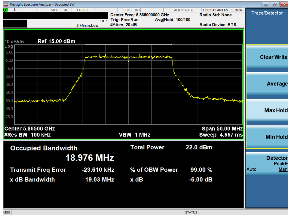
Plot 7-19. 6dB Bandwidth Plot SISO ANT1 (20MHz BW 802.11ax (UNII Band 4) – Ch. 173)
