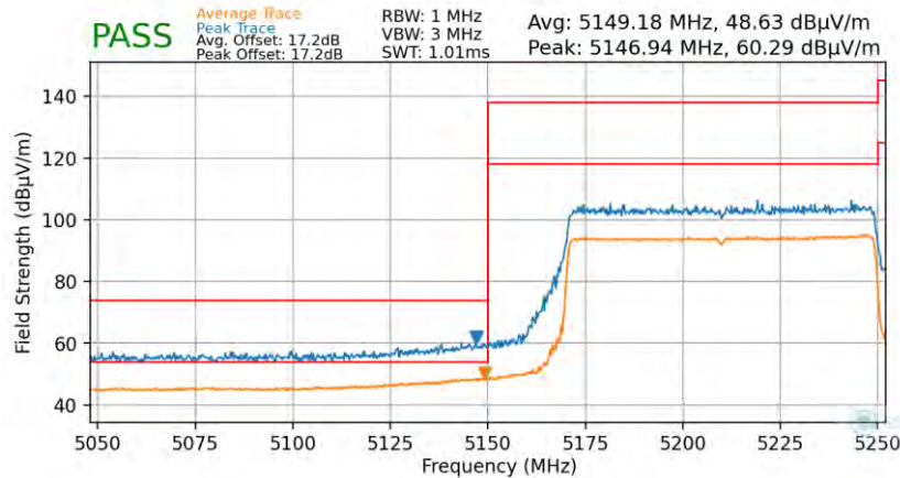
Plot 7-87. Radiated Lower Band Edge Plot (Average & Peak – UNII Band 1)
