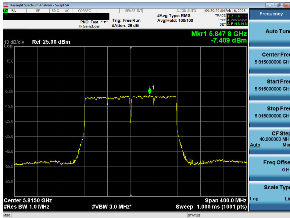
Plot 7-65. Power Spectral Density Plot SISO ANT1 (160MHz BW 802.11ac (UNII Band 3/4) – Ch. 163)
