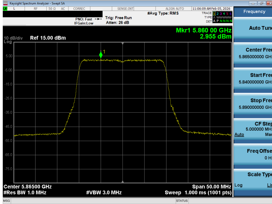
Plot 7-60. Power Spectral Density Plot SISO ANT1 (20MHz BW 802.11ax (UNII Band 4) – Ch. 173)
