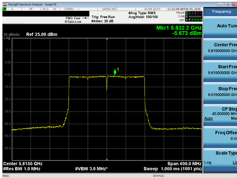
Plot 7-66. Power Spectral Density Plot SISO ANT1 (160MHz BW 802.11ax (UNII Band 3/4) – Ch. 163)
