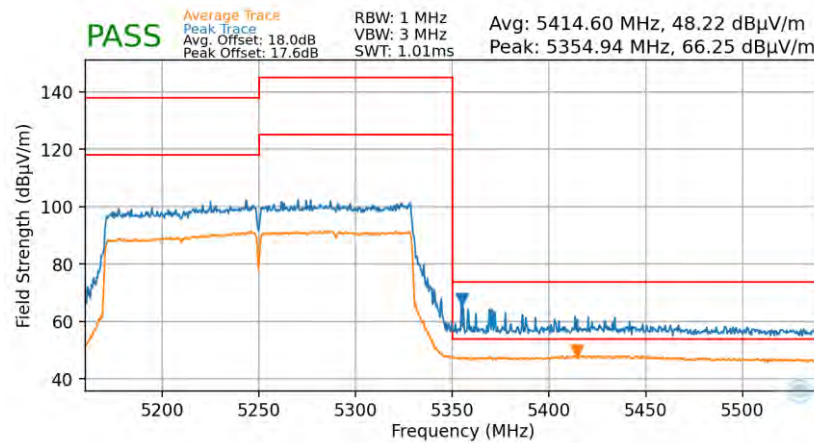
Plot 7-94. Radiated Upper Band Edge Plot (Average & Peak – UNII Band 2A)
