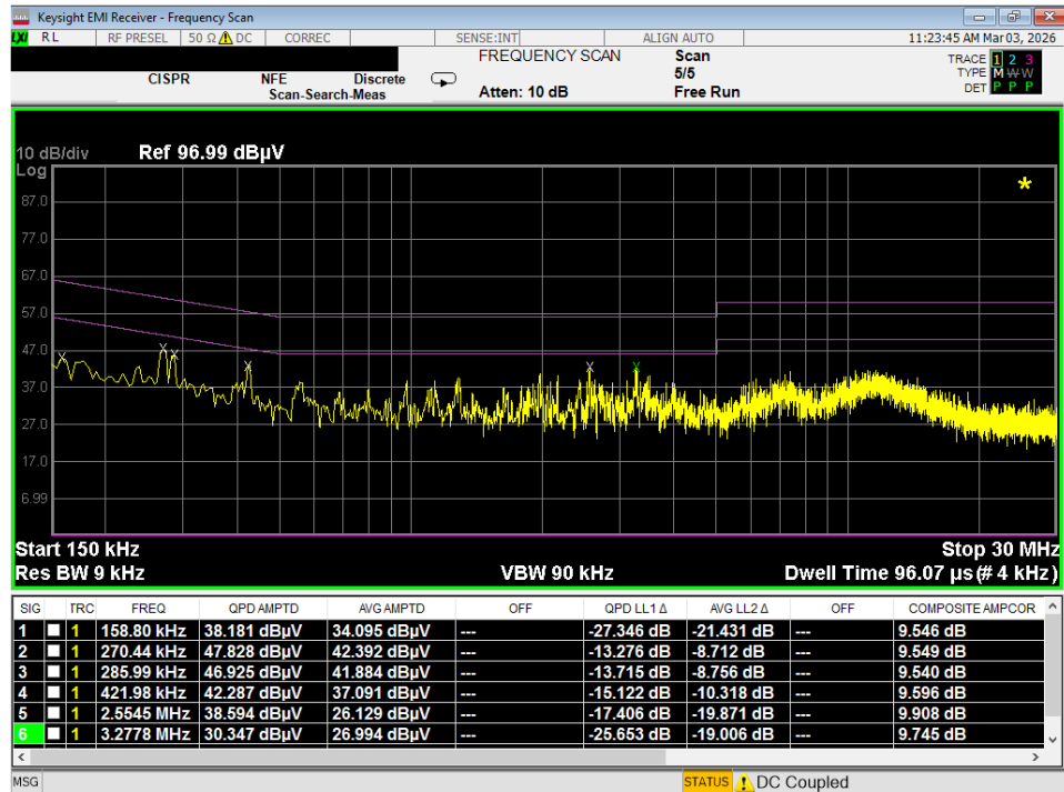
Plot 7-101. Line Conducted Plot with 802.11a UNII Band 2A (N)
