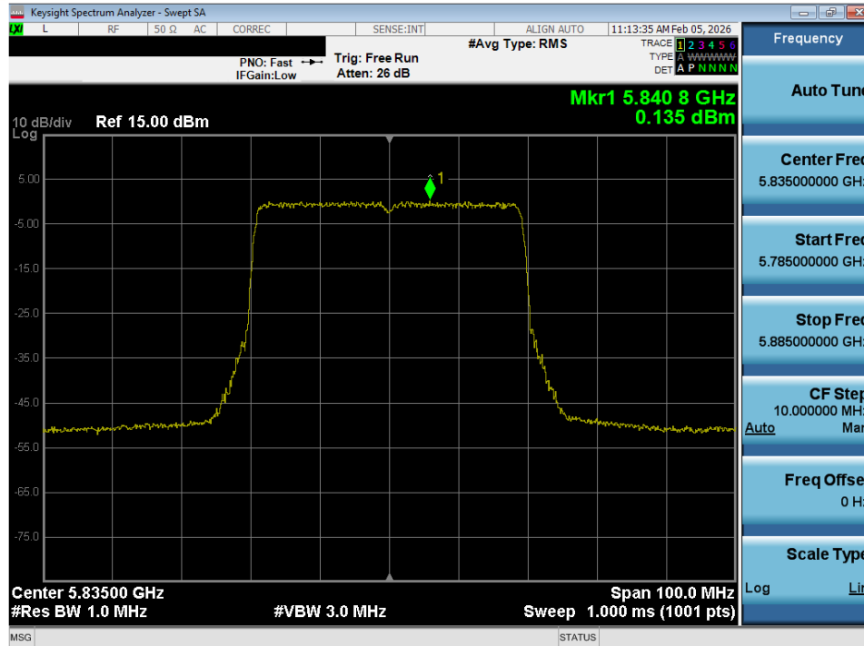
Plot 7-62. Power Spectral Density Plot SISO ANT1 (40MHz BW 802.11ax (UNII Band 3/4) – Ch. 167)
