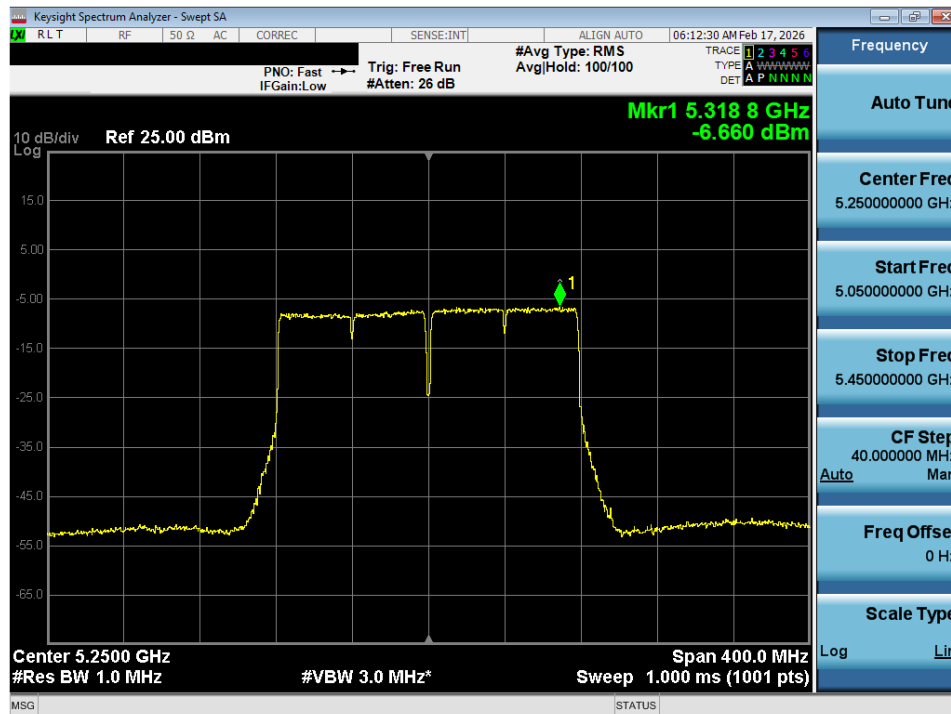
Plot 7-49. Power Spectral Density Plot SISO ANT1 (160MHz BW 802.11ac (UNII Band 1/2A) – Ch. 50)
