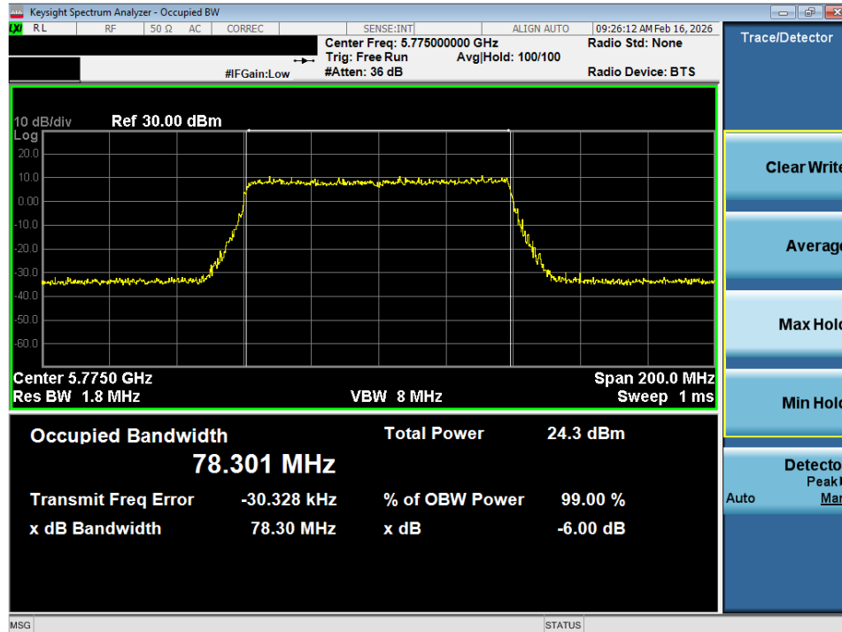
Plot 7-32. OBW Plot SISO ANT1 (80MHz BW 802.11ax (UNII Band 3) – Ch. 155)
