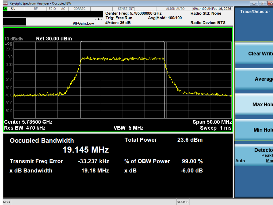
Plot 7-28. OBW Plot SISO ANT1 (20MHz BW 802.11ax (UNII Band 3) – Ch. 157)
