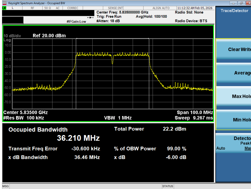
Plot 7-20. 6dB Bandwidth Plot SISO ANT1 (40MHz BW 802.11n (UNII Band 3/4) – Ch. 167)
