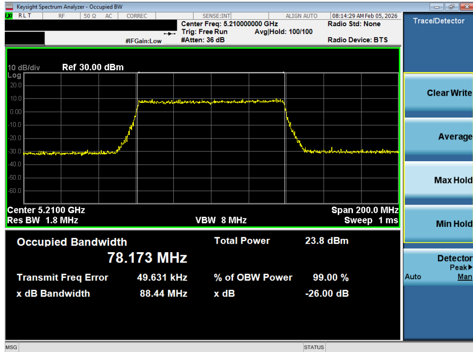
Plot 7-7. 26dB Bandwidth Plot SISO ANT1 (80MHz BW 802.11ax (UNII Band 1) – Ch. 42)
