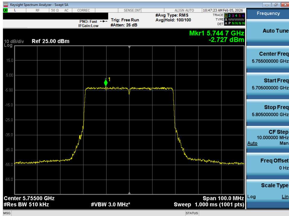
Plot 7-55. Power Spectral Density Plot SISO ANT1 (40MHz BW 802.11ax (UNII Band 3) – Ch. 151)
