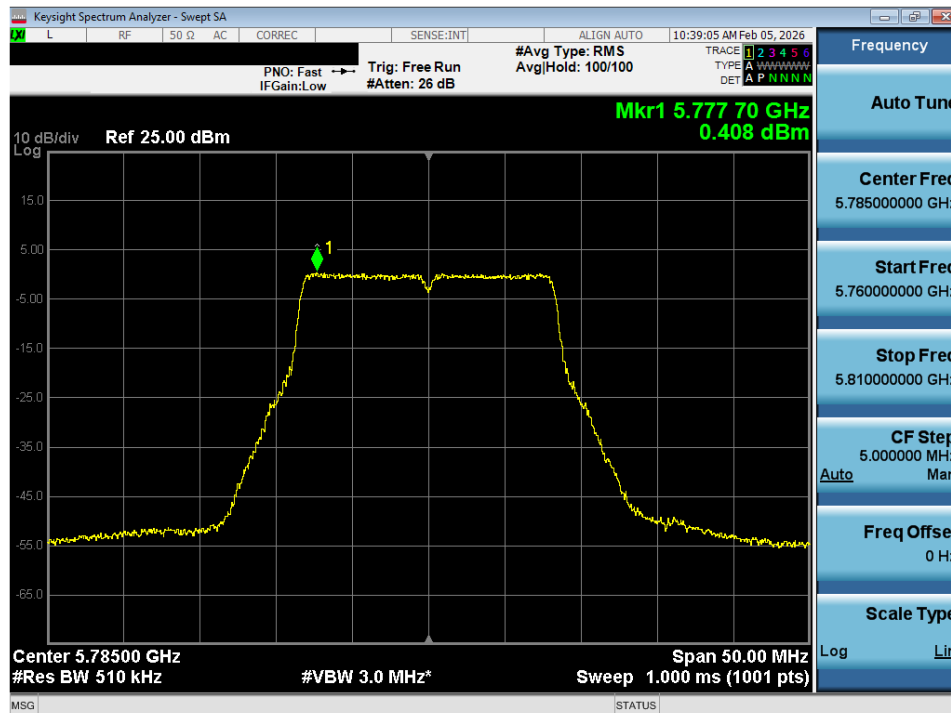
Plot 7-51. Power Spectral Density Plot SISO ANT1 (802.11a (UNII Band 3) – Ch. 157)
