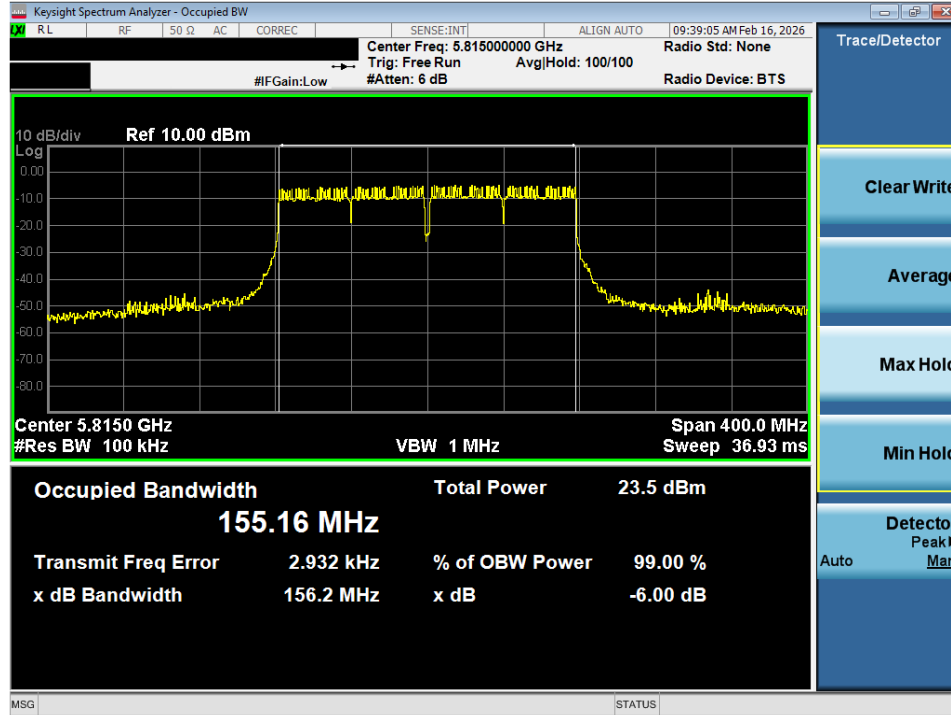
Plot 7-24. 6dB Bandwidth Plot SISO ANT1 (160MHz BW 802.11ac (UNII Band 3/4) – Ch. 163)
