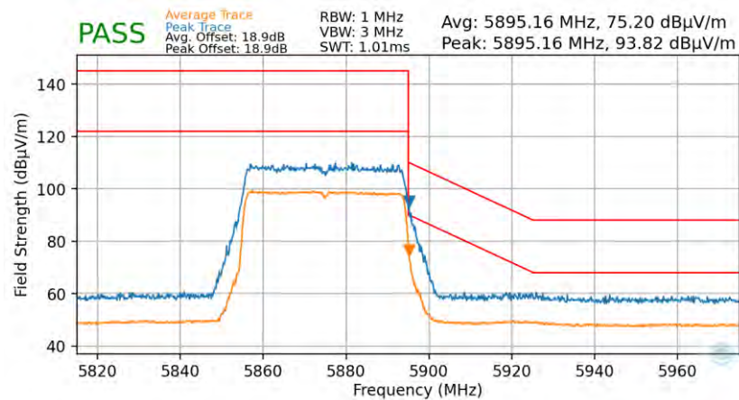
Plot 7-86. Radiated Upper Band Edge Plot (Average & Peak – UNII Band 4)
