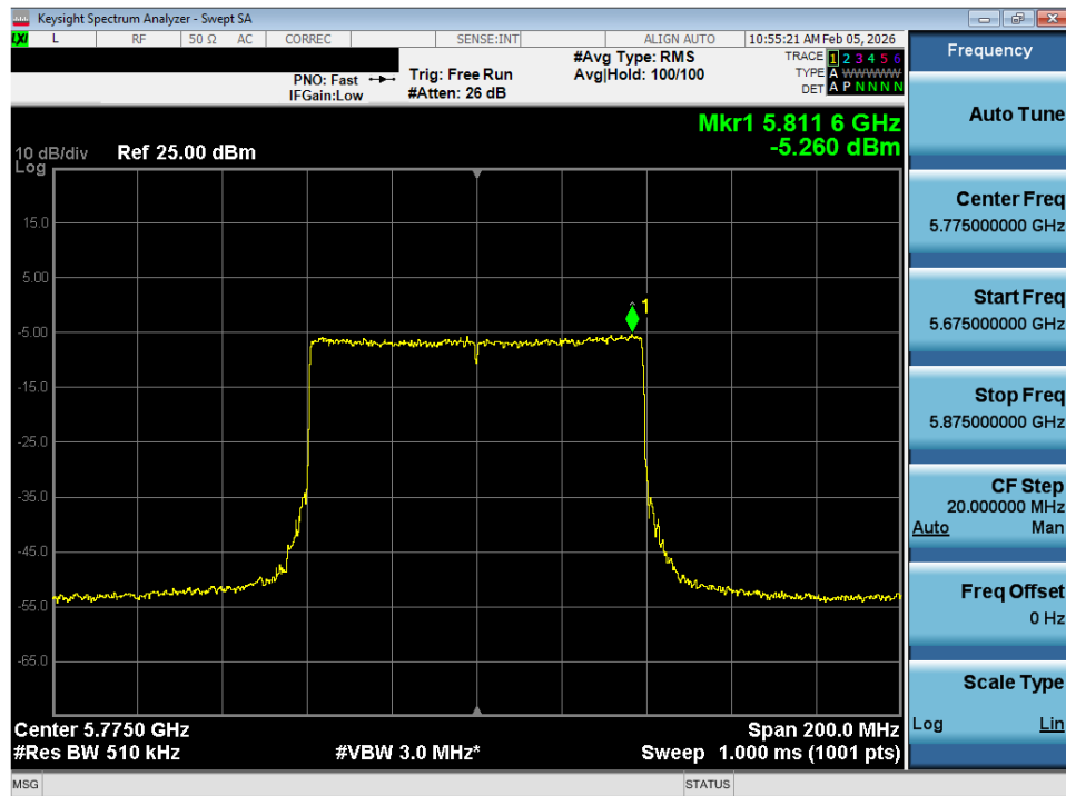
Plot 7-57. Power Spectral Density Plot SISO ANT1 (80MHz BW 802.11ax (UNII Band 3) – Ch. 155)
