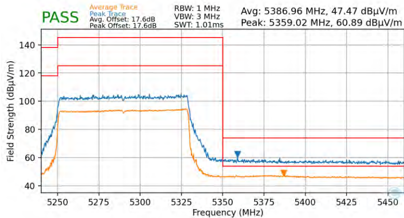
Plot 7-88. Radiated Upper Band Edge Plot (Average & Peak – UNII Band 2A)
