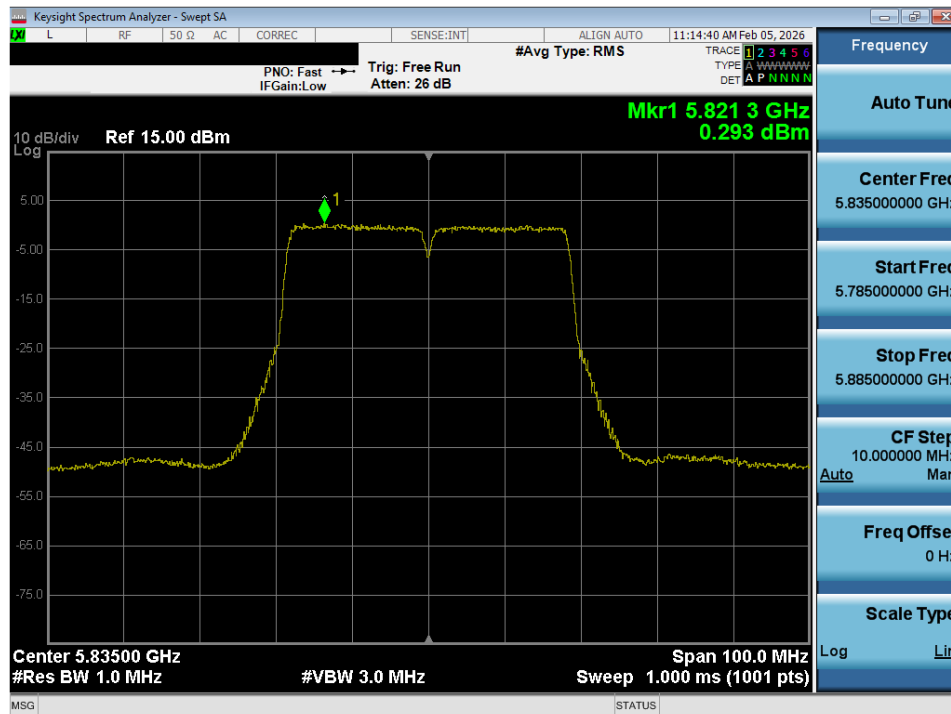
Plot 7-61. Power Spectral Density Plot SISO ANT1 (40MHz BW 802.11n (UNII Band 3/4) – Ch. 167)
