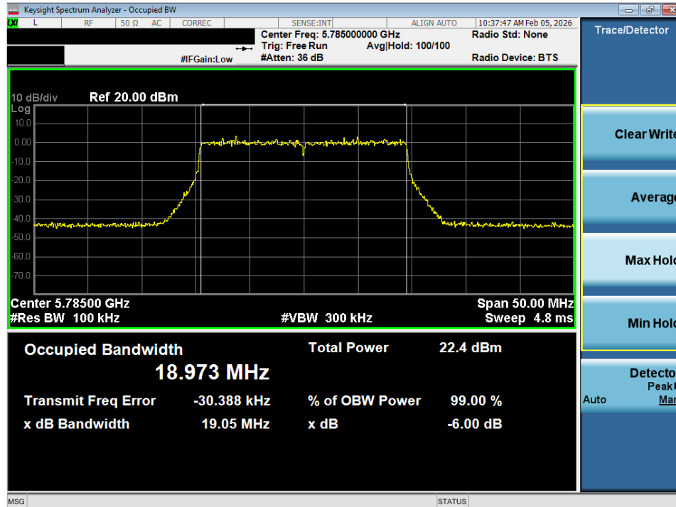
Plot 7-12. 6dB Bandwidth Plot SISO ANT1 (20MHz BW 802.11ax (UNII Band 3) – Ch. 157)
