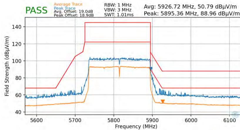
Plot 7-97. Radiated Upper Band Edge Plot (Average & Peak – UNII Band 4)
