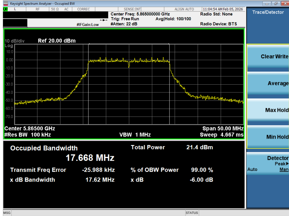
Plot 7-18. 6dB Bandwidth Plot SISO ANT1 (20MHz BW 802.11n (UNII Band 4) – Ch. 173)
