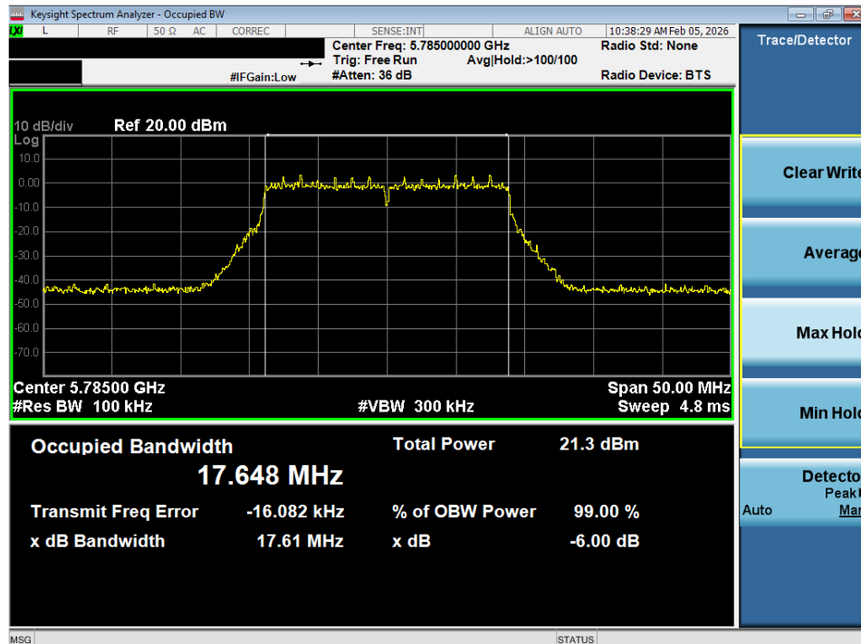
Plot 7-11. 6dB Bandwidth Plot SISO ANT1 (20MHz BW 802.11n (UNII Band 3) – Ch. 157)
