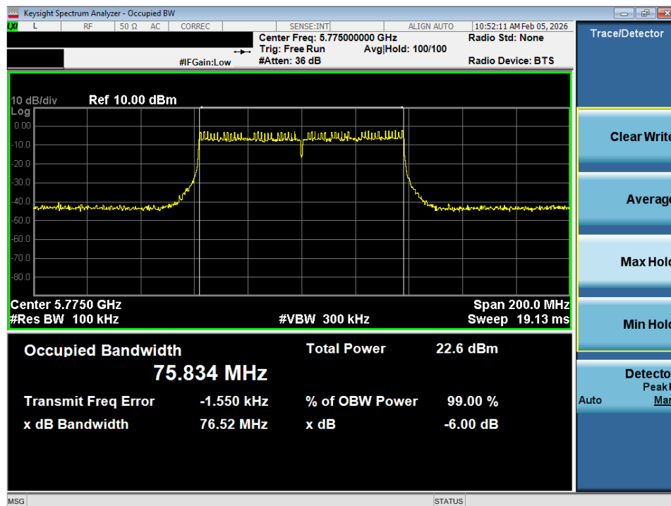
Plot 7-15. 6dB Bandwidth Plot SISO ANT1 (80MHz BW 802.11ac (UNII Band 3) – Ch. 155)
