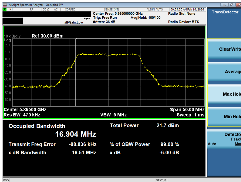
Plot 7-33. OBW Plot SISO ANT1 (802.11a (UNII Band 4) – Ch. 173)
