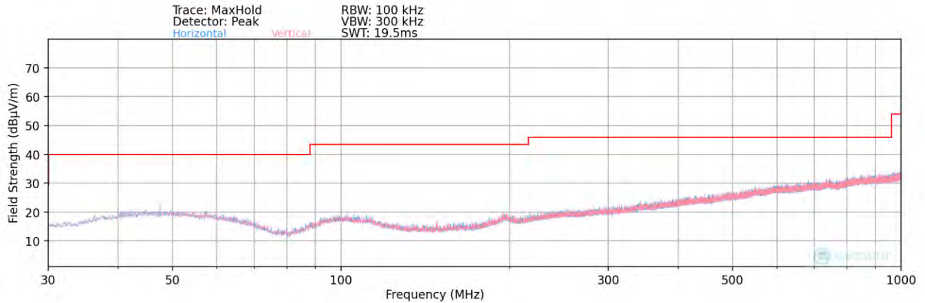
Plot 7-67. Radiated Spurious Plot below 1GHz ANT1 (802.11a)
