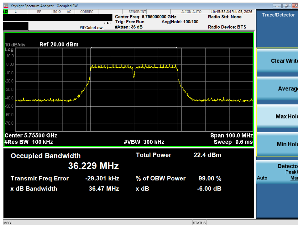
Plot 7-13. 6dB Bandwidth Plot SISO ANT1 (40MHz BW 802.11n (UNII Band 3) – Ch. 151)
