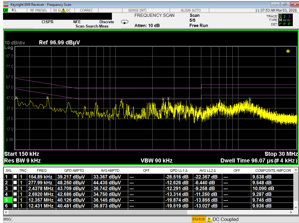
Plot 7-104. Line Conducted Plot with 802.11a UNII Band 3 (L1)
