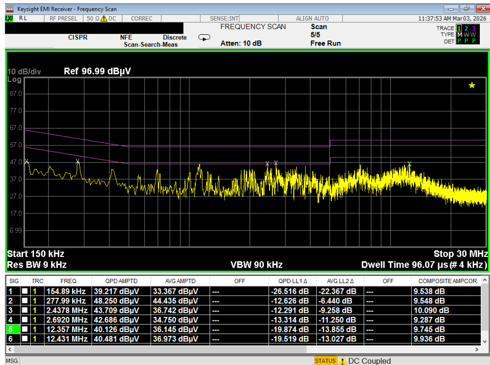
Plot 7-105. Line Conducted Plot with 802.11a UNII Band 3 (N)
