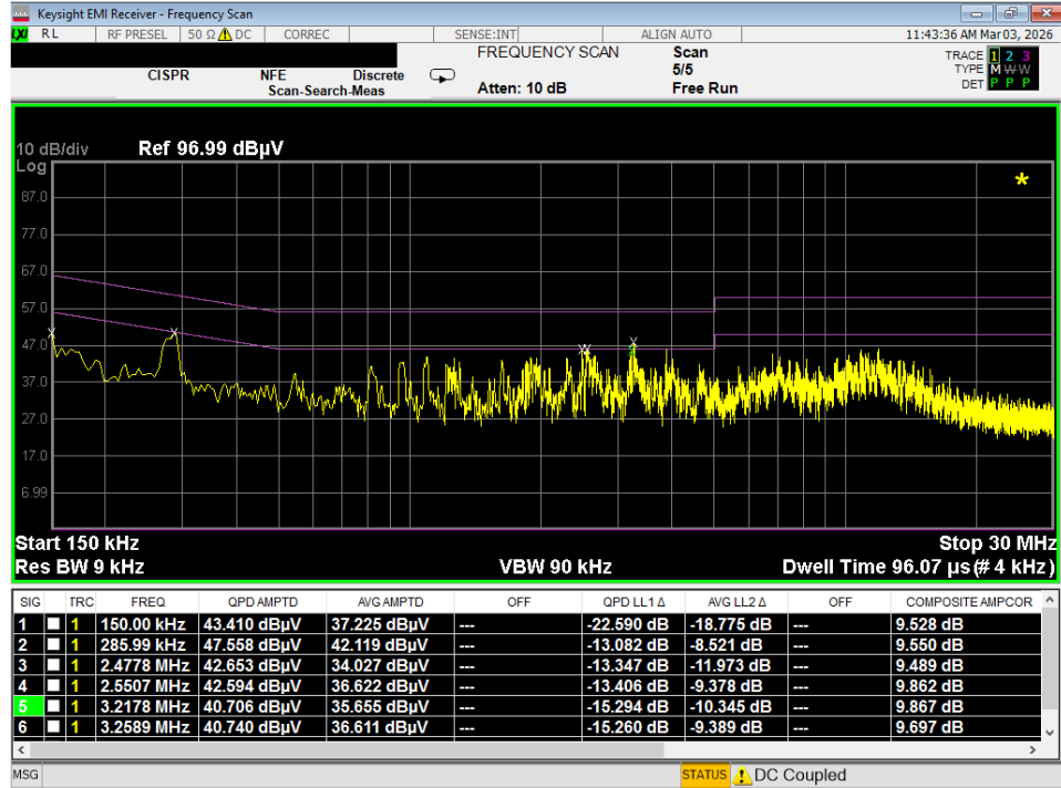
Plot 7-106. Line Conducted Plot with 802.11a UNII Band 4 (L1)
