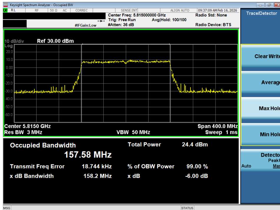
Plot 7-41. OBW Plot SISO ANT1 (160MHz BW 802.11ax (UNII Band 3/4) – Ch. 163)
