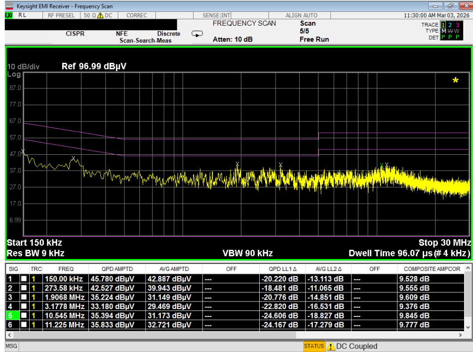
Plot 7-102. Line Conducted Plot with 802.11a UNII Band 2C (L1)
