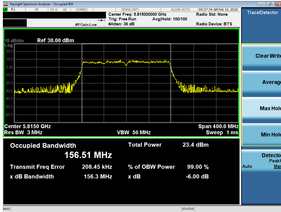
Plot 7-40. OBW Plot SISO ANT1 (160MHz BW 802.11ac (UNII Band 3/4) – Ch. 163)
