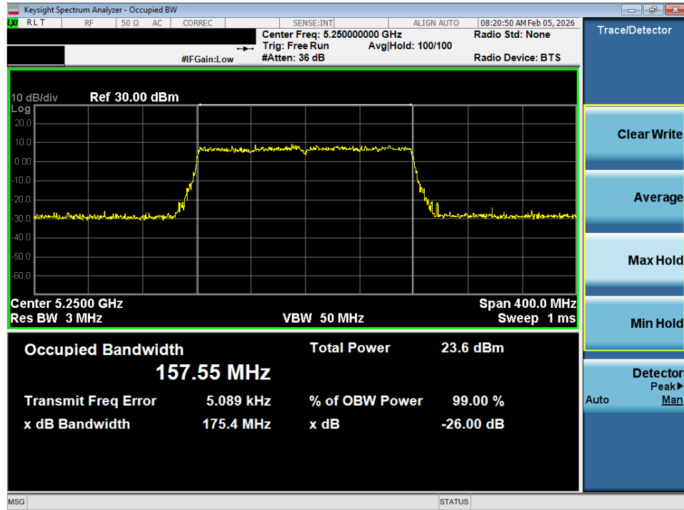
Plot 7-9. 26dB Bandwidth Plot SISO ANT1 (160MHz BW 802.11ax (UNII Band 1/2A) – Ch. 50)
