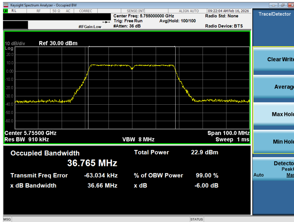
Plot 7-29. OBW Plot SISO ANT1 (40MHz BW 802.11n (UNII Band 3) – Ch. 151)
