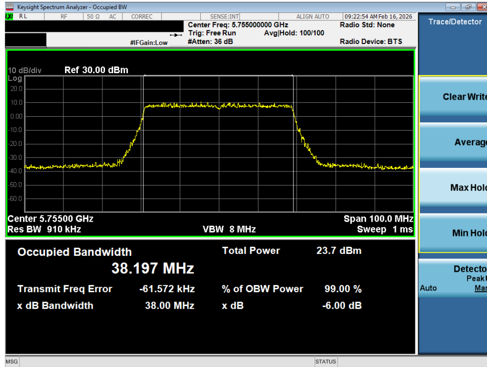
Plot 7-30. OBW Plot SISO ANT1 (40MHz BW 802.11ax (UNII Band 3) – Ch. 151)
