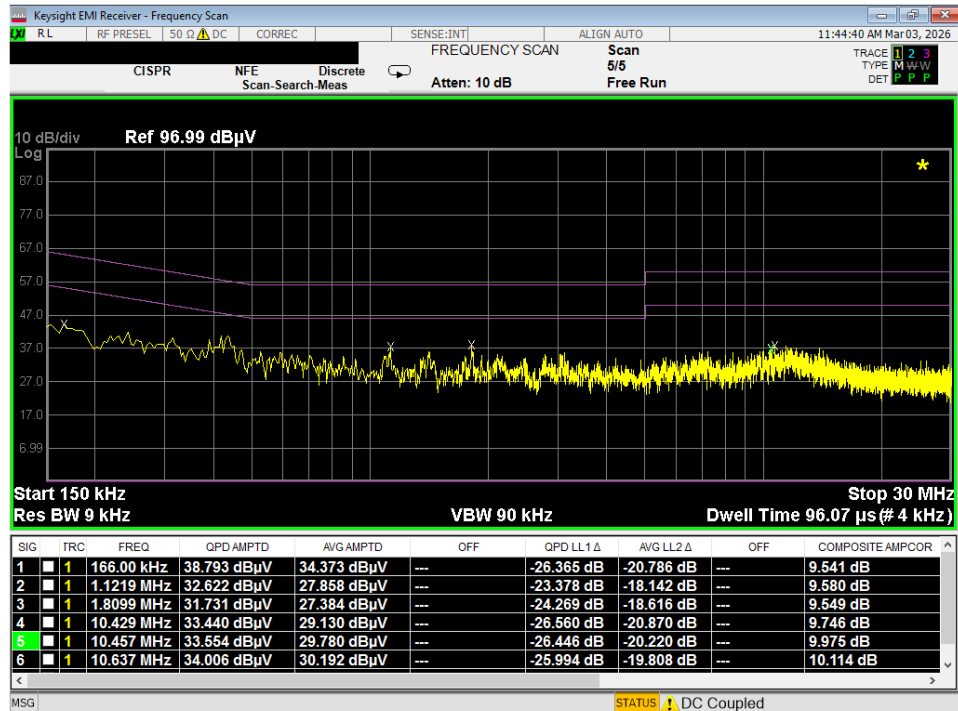
Plot 7-107. Line Conducted Plot with 802.11a UNII Band 4 (N)
