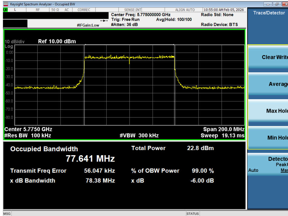
Plot 7-16. 6dB Bandwidth Plot SISO ANT1 (80MHz BW 802.11ax (UNII Band 3) – Ch. 155)
