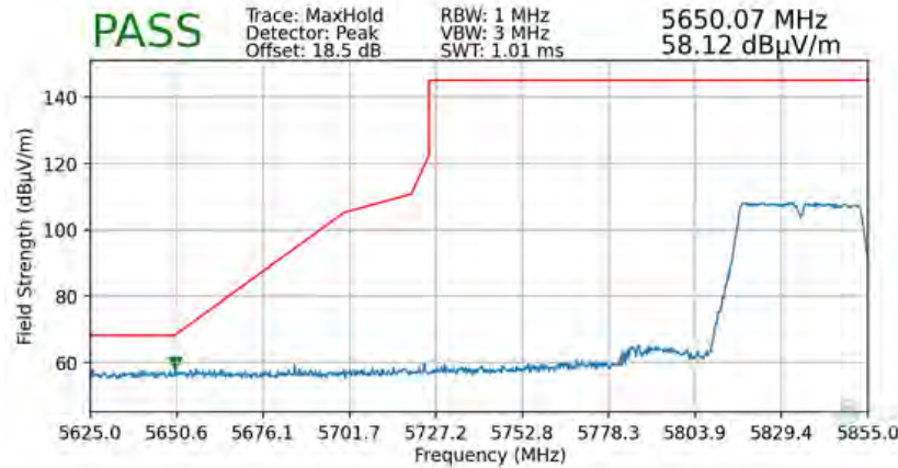
Plot 7-85. Radiated Lower Band Edge Plot (Peak – UNII Band 4)
