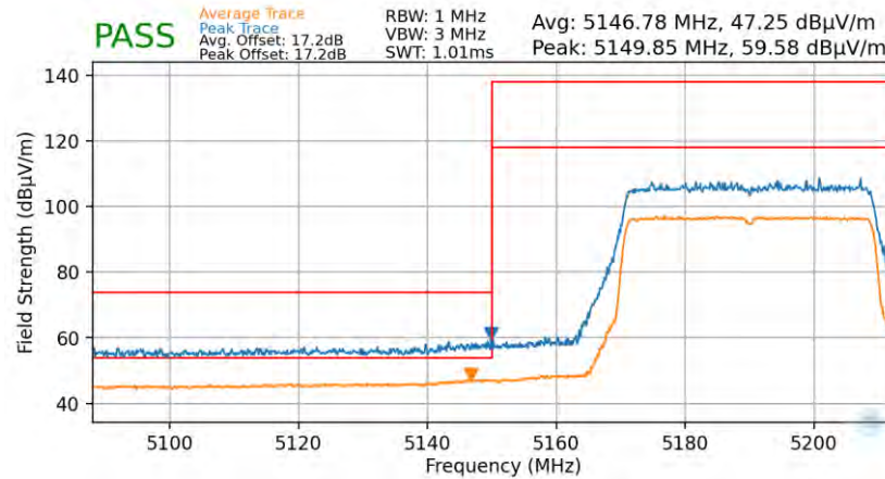
Plot 7-81. Radiated Lower Band Edge Plot (Average & Peak – UNII Band 1)
