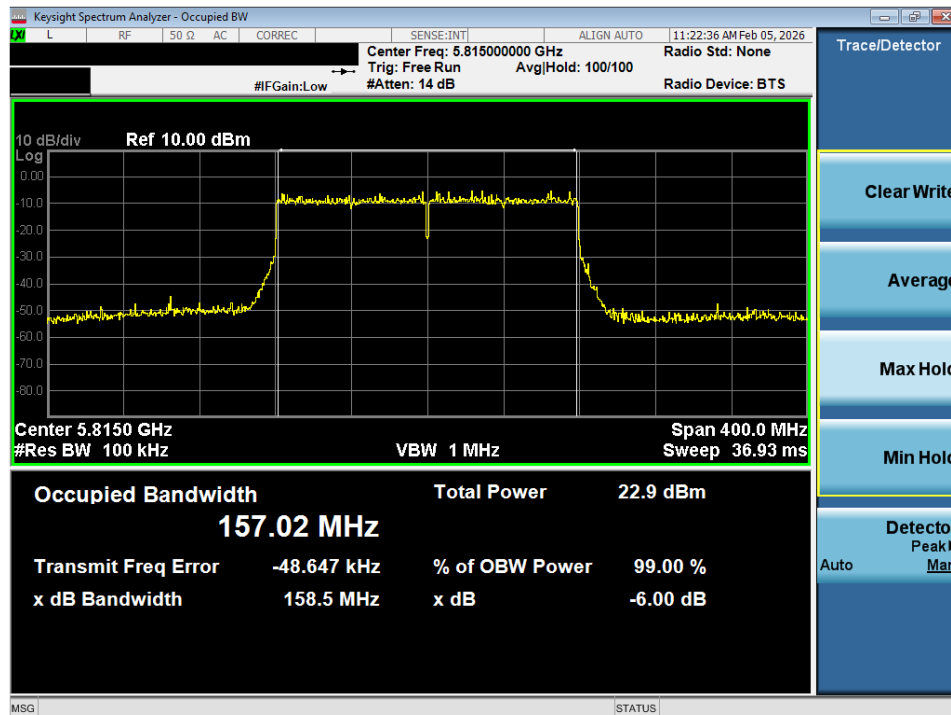
Plot 7-25. 6dB Bandwidth Plot SISO ANT1 (160MHz BW 802.11ax (UNII Band 3/4) – Ch. 163)
