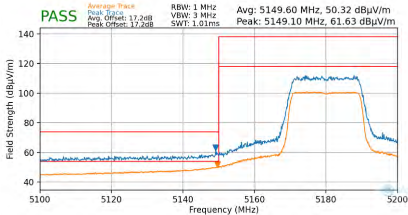
Plot 7-75. Radiated Lower Band Edge Plot (Average & Peak – UNII Band 1)
