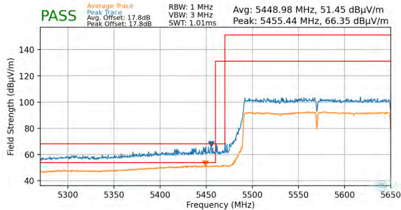
Plot 7-95. Radiated Lower Band Edge Plot (Average & Peak – UNII Band 2C)
