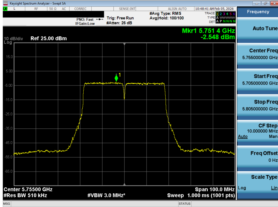
Plot 7-54. Power Spectral Density Plot SISO ANT1 (40MHz BW 802.11n (UNII Band 3) – Ch. 151)
