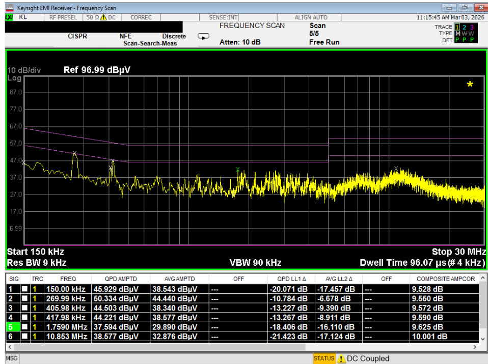
Plot 7-99. Line Conducted Plot with 802.11a UNII Band 1 (N)
