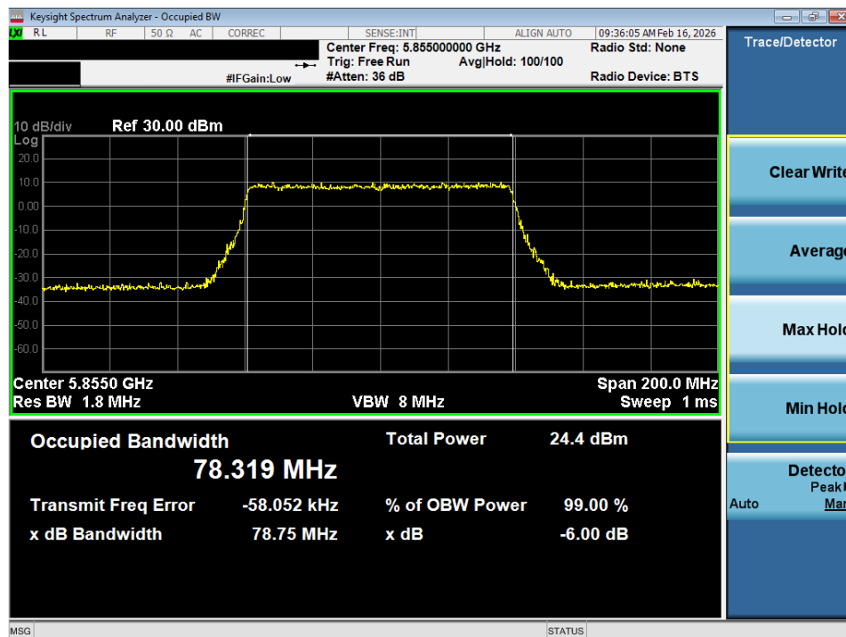
Plot 7-39. OBW Plot SISO ANT1 (80MHz BW 802.11ax (UNII Band 3/4) – Ch. 171)
