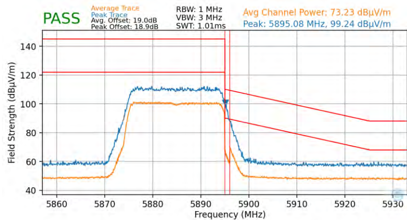
Plot 7-80. Radiated Upper Band Edge Plot (Average & Peak – UNII Band 4)
