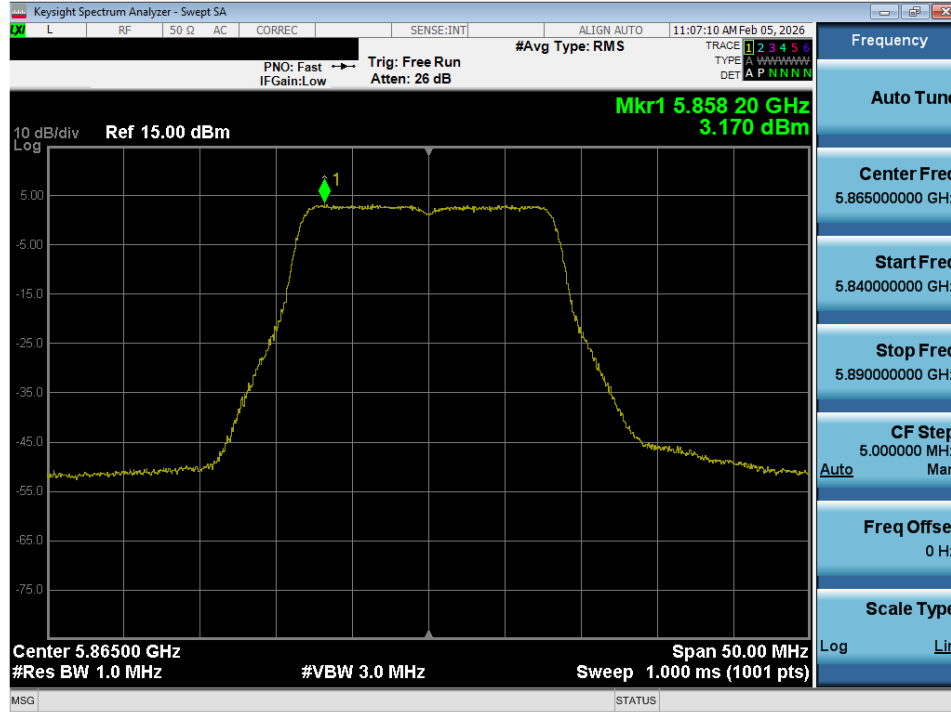
Plot 7-58. Power Spectral Density Plot SISO ANT1 (802.11a (UNII Band 4) – Ch. 173)
