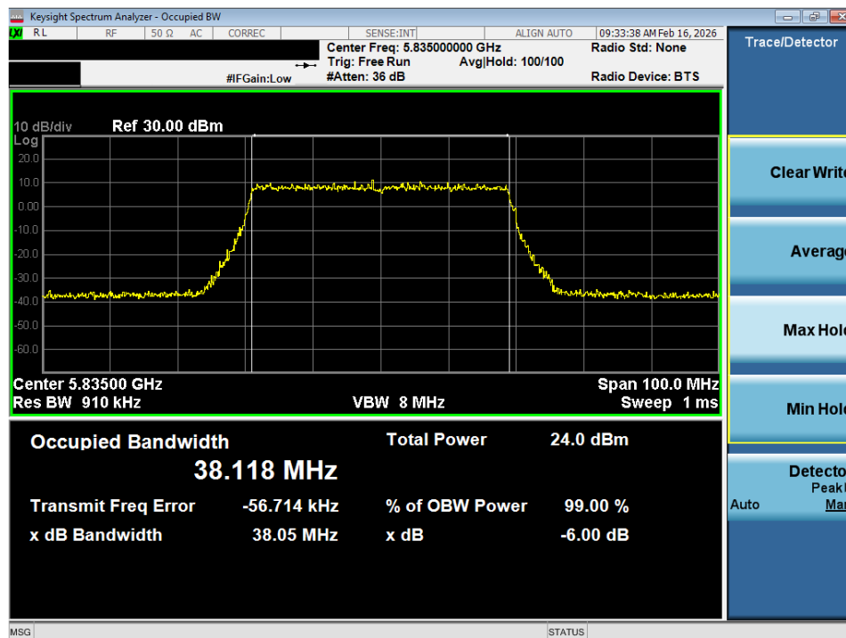
Plot 7-37. OBW Plot SISO ANT1 (40MHz BW 802.11ax (UNII Band 3/4) – Ch. 167)
