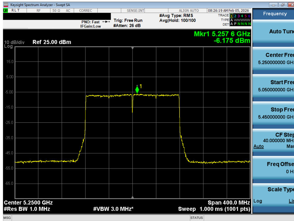
Plot 7-50. Power Spectral Density Plot SISO ANT1 (160MHz BW 802.11ax (UNII Band 1/2A) – Ch. 50)
