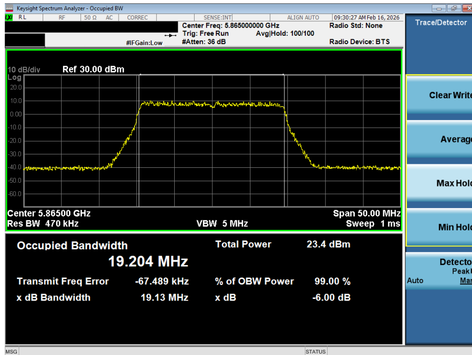
Plot 7-35. OBW Plot SISO ANT1 (20MHz BW 802.11ax (UNII Band 4) – Ch. 173)
