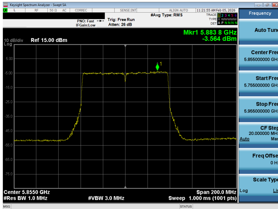
Plot 7-63. Power Spectral Density Plot SISO ANT1 (80MHz BW 802.11ac (UNII Band 3/4) – Ch. 171)
