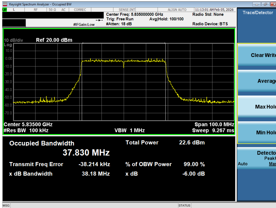
Plot 7-21. 6dB Bandwidth Plot SISO ANT1 (40MHz BW 802.11ax (UNII Band 3/4) – Ch. 167)
