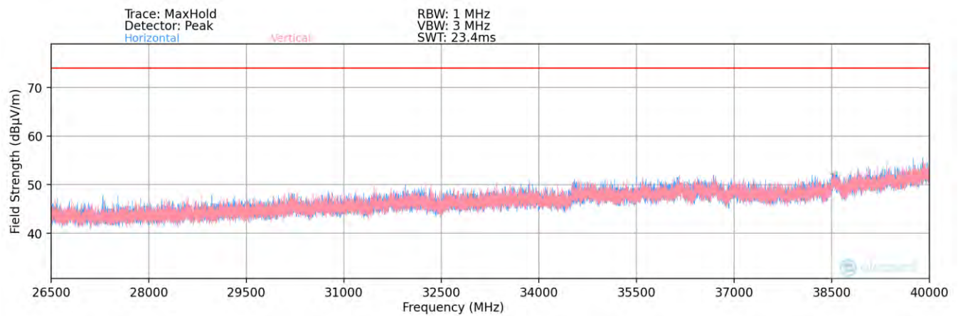
Plot 7-74. Radiated Spurious Plot 26.5GHz – 40GHz ANT1 (802.11a)
