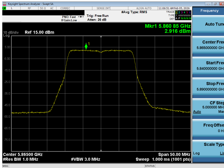
Plot 7-59. Power Spectral Density Plot SISO ANT1 (20MHz BW 802.11n (UNII Band 4) – Ch. 173)
