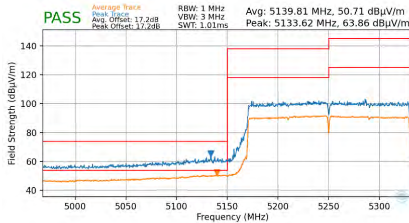
Plot 7-93. Radiated Lower Band Edge Plot (Average & Peak – UNII Band 1)
