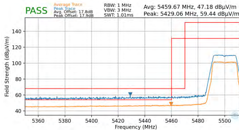
Plot 7-77. Radiated Lower Band Edge Plot (Average & Peak – UNII Band 2C)
