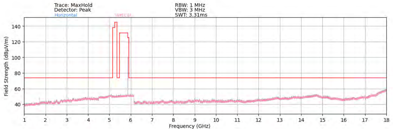
Plot 7-72. Radiated Spurious Plot above 1GHz ANT1 (802.11a – UNII Band 4 Ch. 173)
