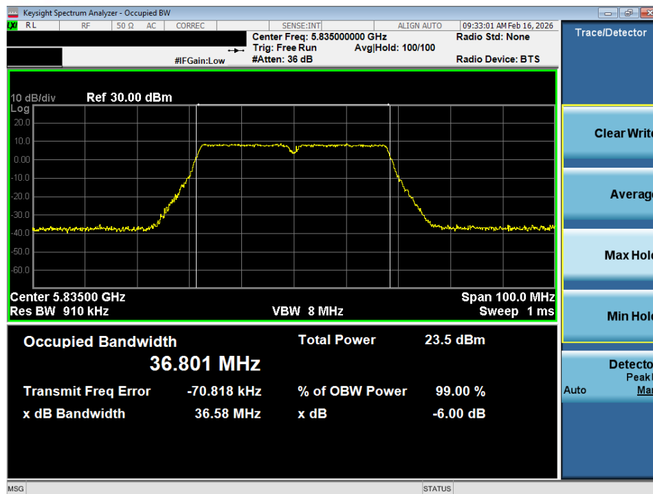
Plot 7-36. OBW Plot SISO ANT1 (40MHz BW 802.11n (UNII Band 3/4) – Ch. 167)
