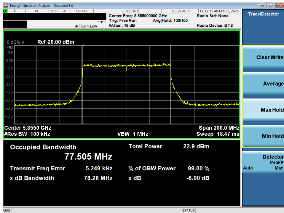
Plot 7-23. 6dB Bandwidth Plot SISO ANT1 (80MHz BW 802.11ax (UNII Band 3/4) – Ch. 171)
