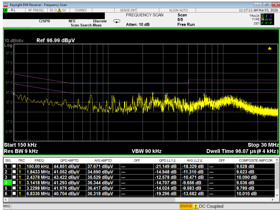
Plot 7-98. Line Conducted Plot with 802.11a UNII Band 1 (L1)
