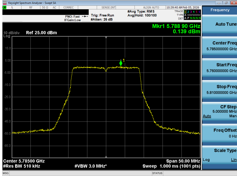
Plot 7-52. Power Spectral Density Plot SISO ANT1 (20MHz BW 802.11n (UNII Band 3) – Ch. 157)
