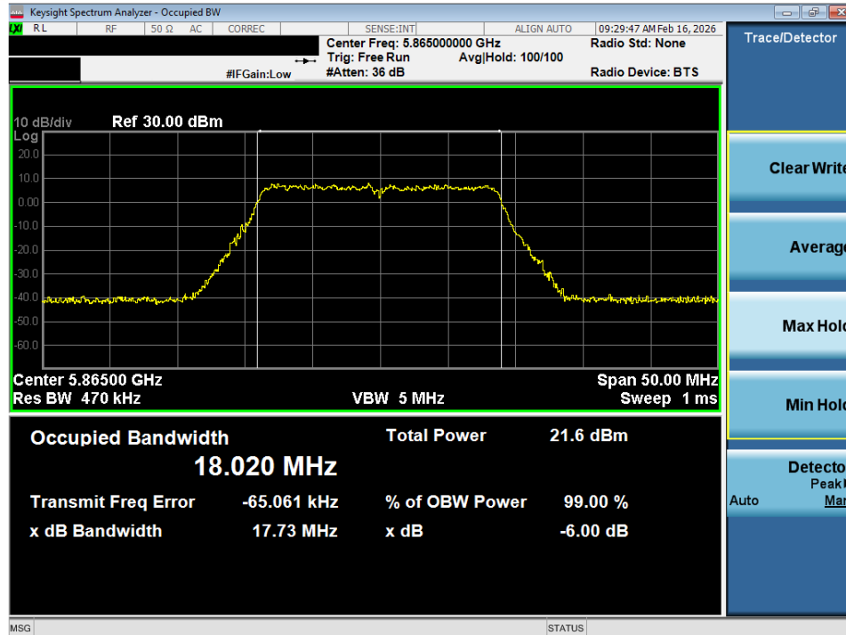
Plot 7-34. OBW Plot SISO ANT1 (20MHz BW 802.11n (UNII Band 4) – Ch. 173)
