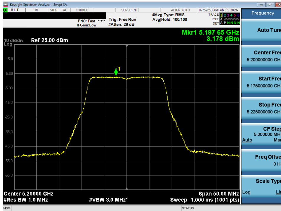
Plot 7-42. Power Spectral Density Plot SISO ANT1 (802.11a (UNII Band 1) – Ch. 40)
