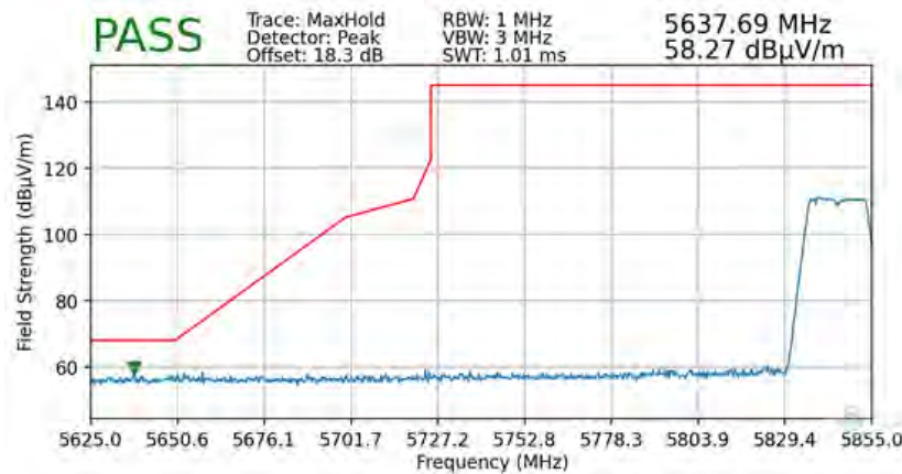
Plot 7-79. Radiated Lower Band Edge Plot (Peak – UNII Band 4)
