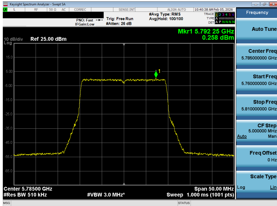
Plot 7-53. Power Spectral Density Plot SISO ANT1 (20MHz BW 802.11ax (UNII Band 3) – Ch. 157)
