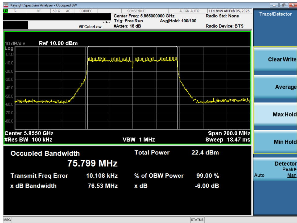
Plot 7-22. 6dB Bandwidth Plot SISO ANT1 (80MHz BW 802.11ac (UNII Band 3/4) – Ch. 171)
