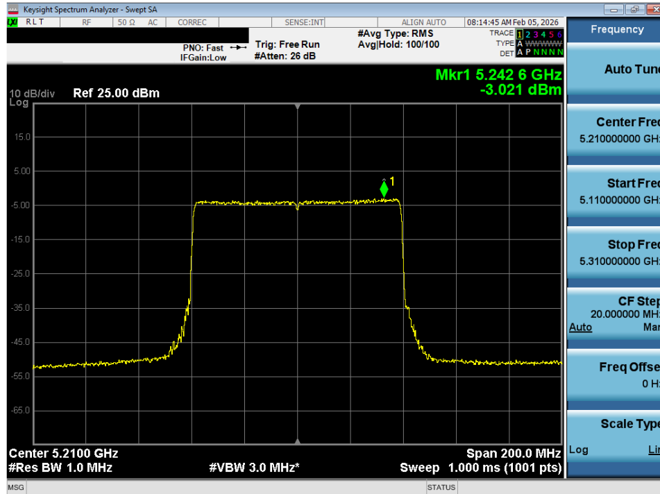
Plot 7-48. Power Spectral Density Plot SISO ANT1 (80MHz BW 802.11ax (UNII Band 1) – Ch. 42)
