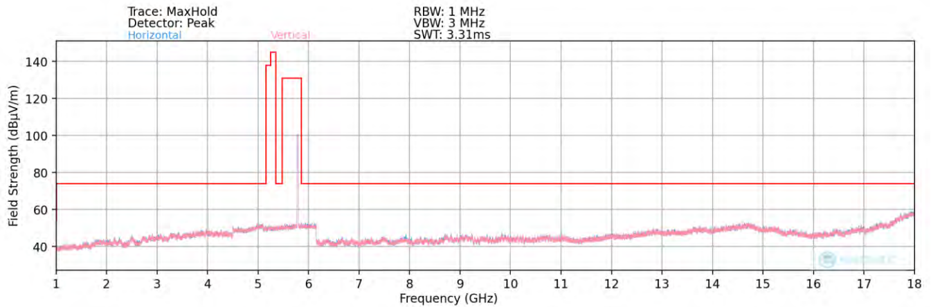
Plot 7-71. Radiated Spurious Plot above 1GHz ANT1 (802.11a – UNII Band 3 Ch. 157)
