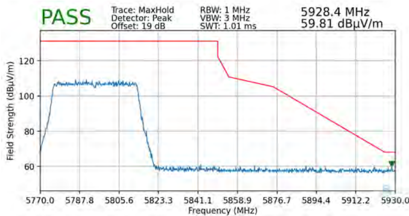
Plot 7-84. Radiated Upper Band Edge Plot (Peak – UNII Band 3)
