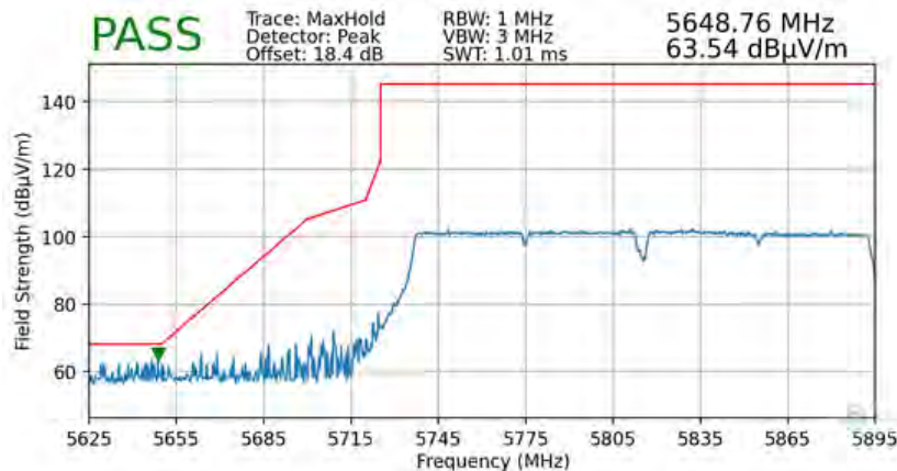
Plot 7-96. Radiated Lower Band Edge Plot (Peak – UNII Band 4)
