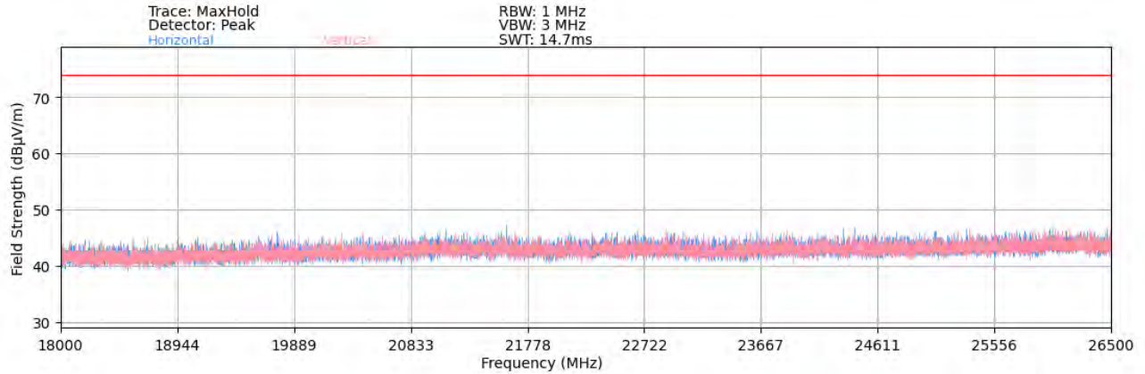
Plot 7-73. Radiated Spurious Plot 18GHz – 26.5GHz ANT1 (802.11a)
