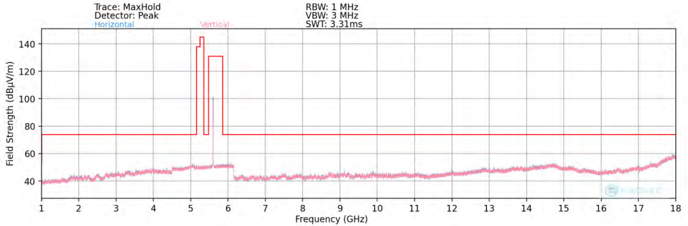
Plot 7-70. Radiated Spurious Plot above 1GHz ANT1 (802.11a – UNII Band 2C Ch. 120)
