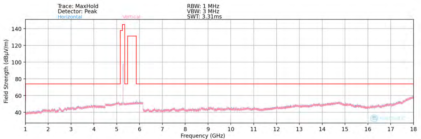
Plot 7-69. Radiated Spurious Plot above 1GHz ANT1 (802.11a – UNII Band 2A Ch. 56)
