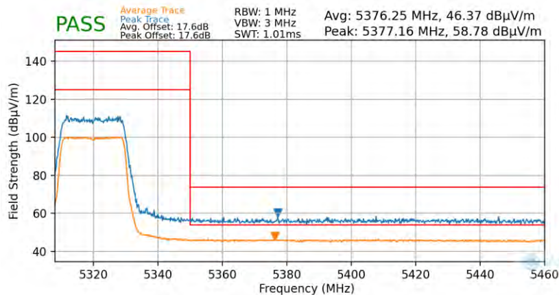
Plot 7-76. Radiated Upper Band Edge Plot (Average & Peak – UNII Band 2A)
