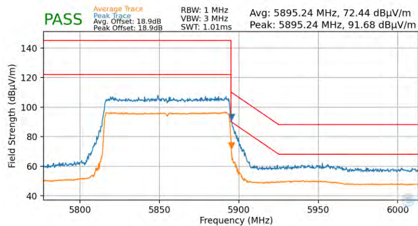
Plot 7-92. Radiated Upper Band Edge Plot (Average & Peak – UNII Band 4)
