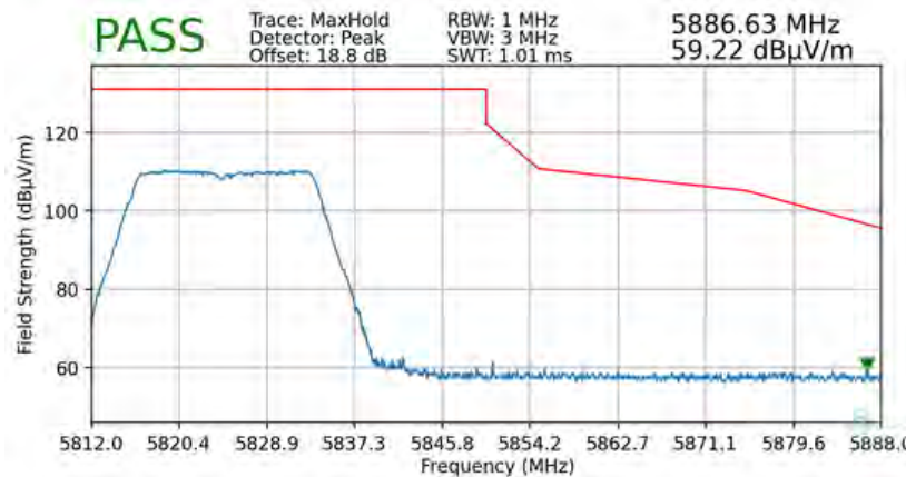
Plot 7-78. Radiated Upper Band Edge Plot (Peak – UNII Band 3)
