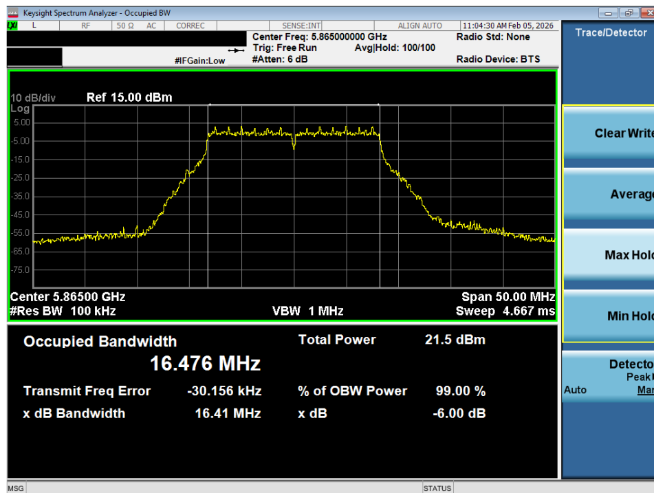
Plot 7-17. 6dB Bandwidth Plot SISO ANT1 (802.11a (UNII Band 4) – Ch. 173)
