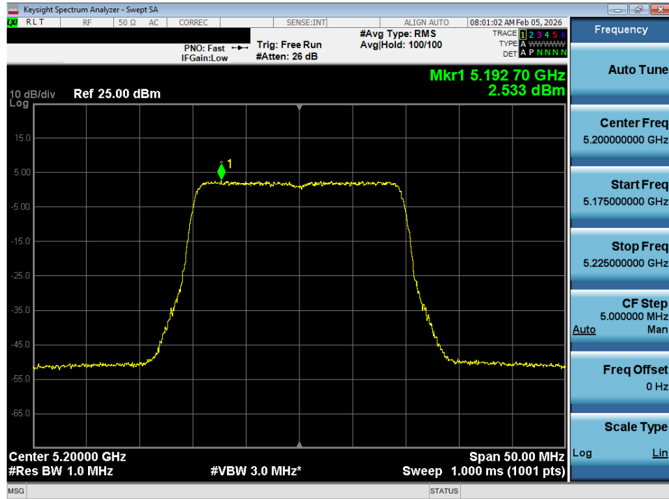
Plot 7-44. Power Spectral Density Plot SISO ANT1 (20MHz BW 802.11ax (UNII Band 1) – Ch. 40)
