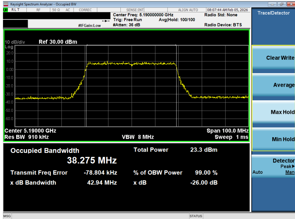
Plot 7-5. 26dB Bandwidth Plot SISO ANT1 (40MHz BW 802.11ax (UNII Band 1) – Ch. 38)
