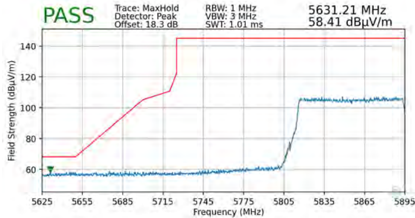
Plot 7-91. Radiated Lower Band Edge Plot (Peak – UNII Band 4)
