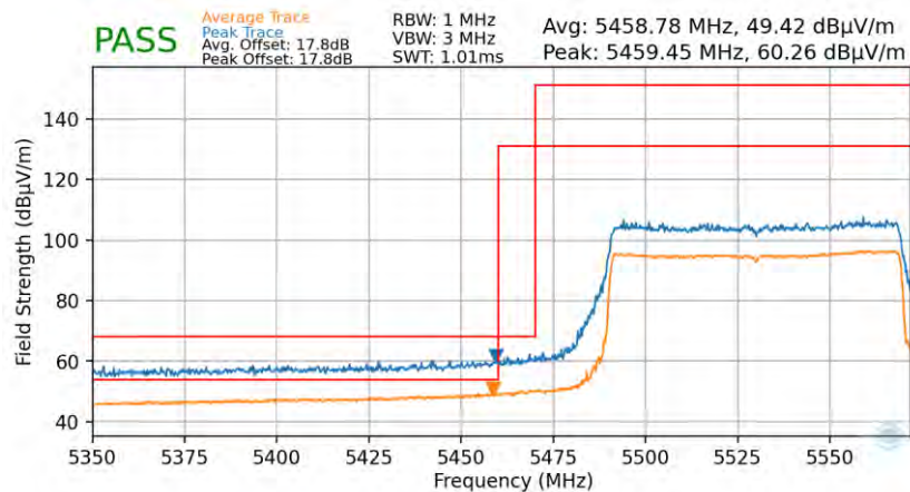
Plot 7-89. Radiated Lower Band Edge Plot (Average & Peak – UNII Band 2C)
