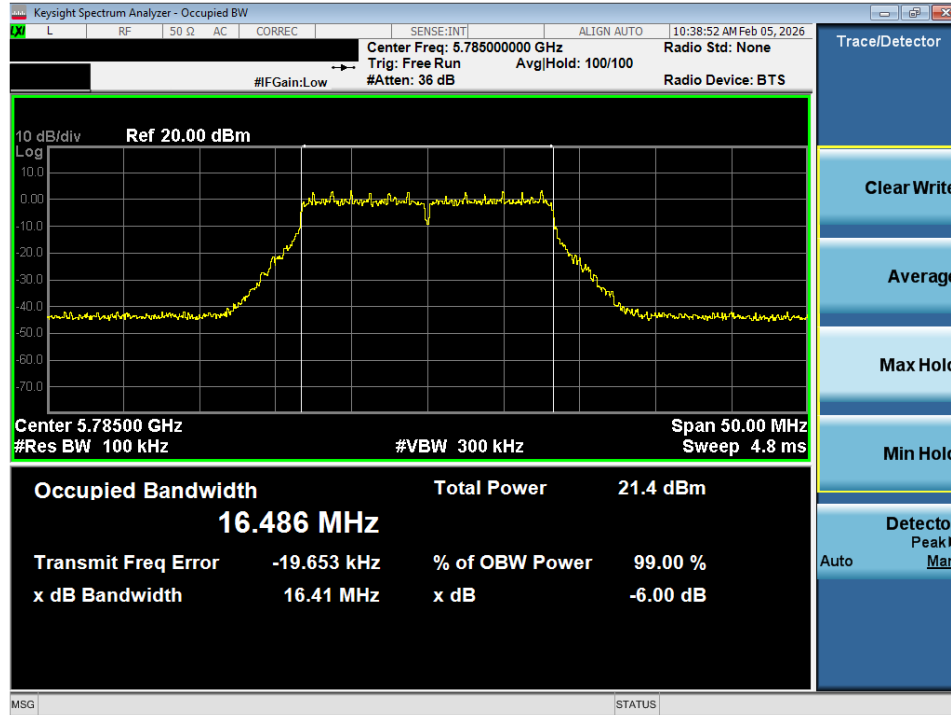
Plot 7-10. 6dB Bandwidth Plot SISO ANT1 (802.11a (UNII Band 3) – Ch. 157)
