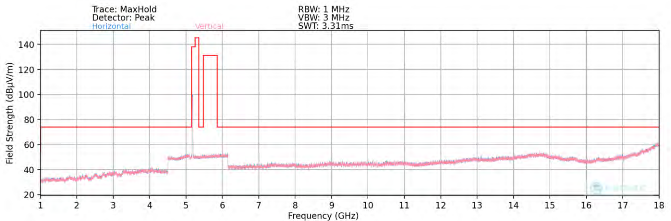
Plot 7-68. Radiated Spurious Plot above 1GHz ANT1 (802.11a – UNII Band 1 Ch. 40)
