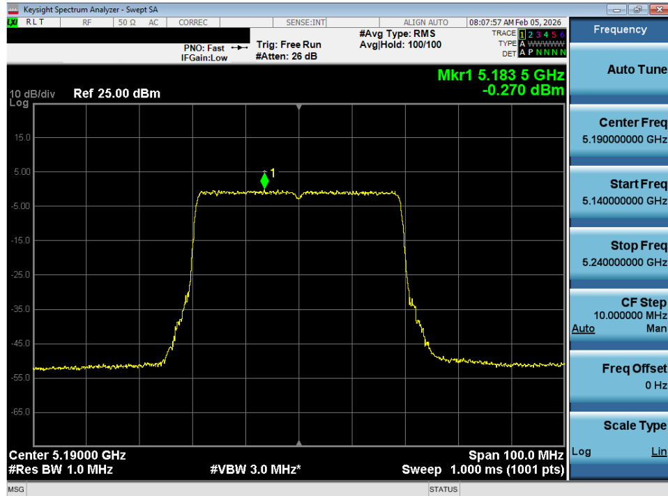
Plot 7-46. Power Spectral Density Plot SISO ANT1 (40MHz BW 802.11ax (UNII Band 1) – Ch. 38)
