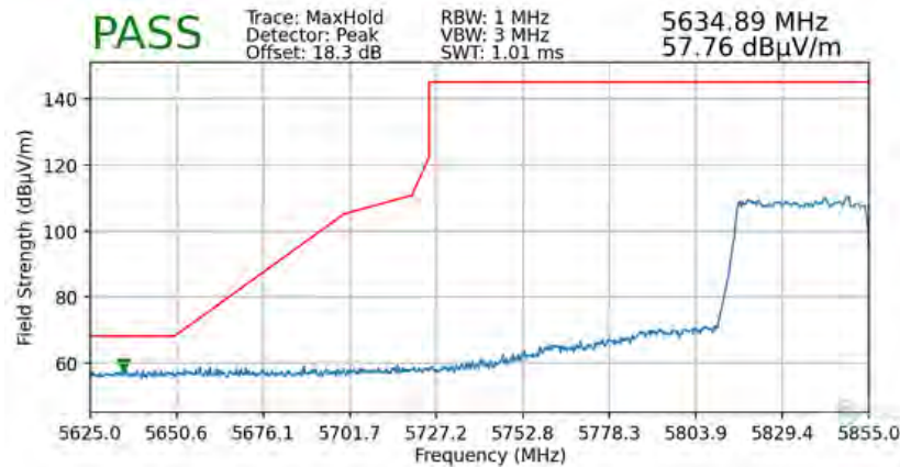
Plot 7-91. Radiated Lower Band Edge Plot (Peak - UNII Band 4 - 484 Tones)
