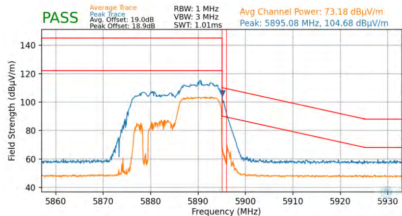
Plot 7-78. Radiated Upper Band Edge Plot (Average & Peak – UNII Band 4 – 106 Tones)
