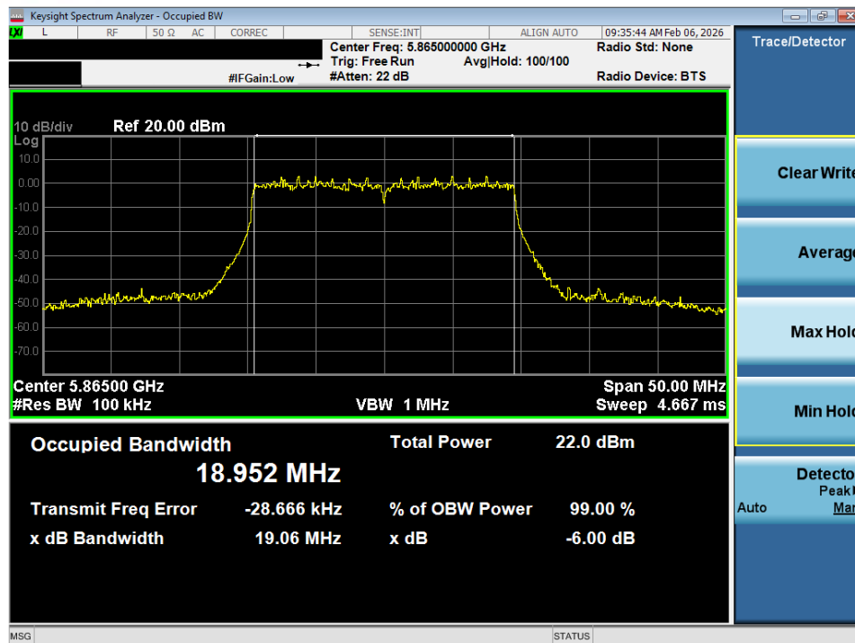
Plot 7-19. 6dB Bandwidth Plot SISO ANT1 (20MHz BW 802.11ax – 242 Tones (UNII Band 4) – Ch. 173)
