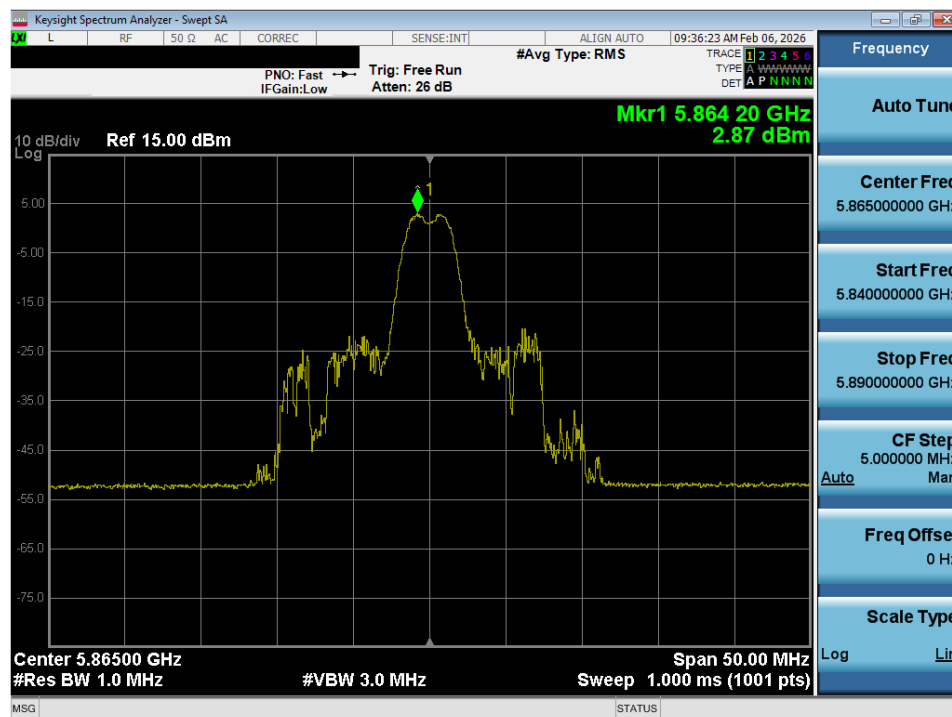
Plot 7-44. Power Spectral Density Plot SISO ANT1 (20MHz BW 802.11ax – 26 Tones (UNII Band 4) – Ch. 173)
