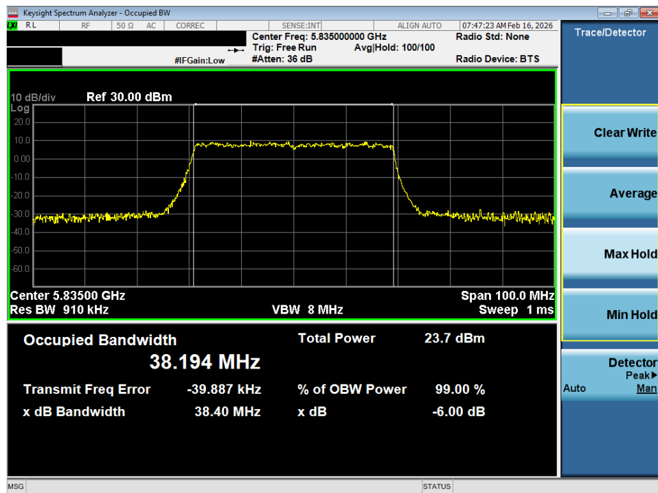
Plot 7-34. OBW Plot SISO ANT1 (40MHz BW 802.11ax – 484 Tones (UNII Band 3/4) – Ch. 167)
