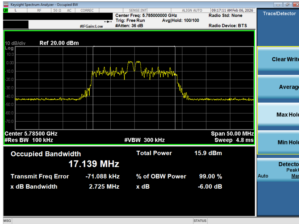
Plot 7-9. 6dB Bandwidth Plot SISO ANT1 (20MHz BW 802.11ax – 26 Tones (UNII Band 3) – Ch. 157)
