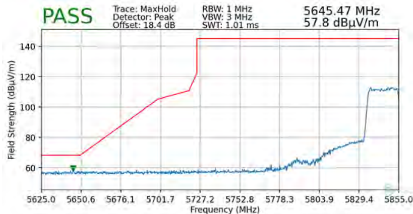
Plot 7-84. Radiated Lower Band Edge Plot (Peak - UNII Band 4 - 242 Tones)
