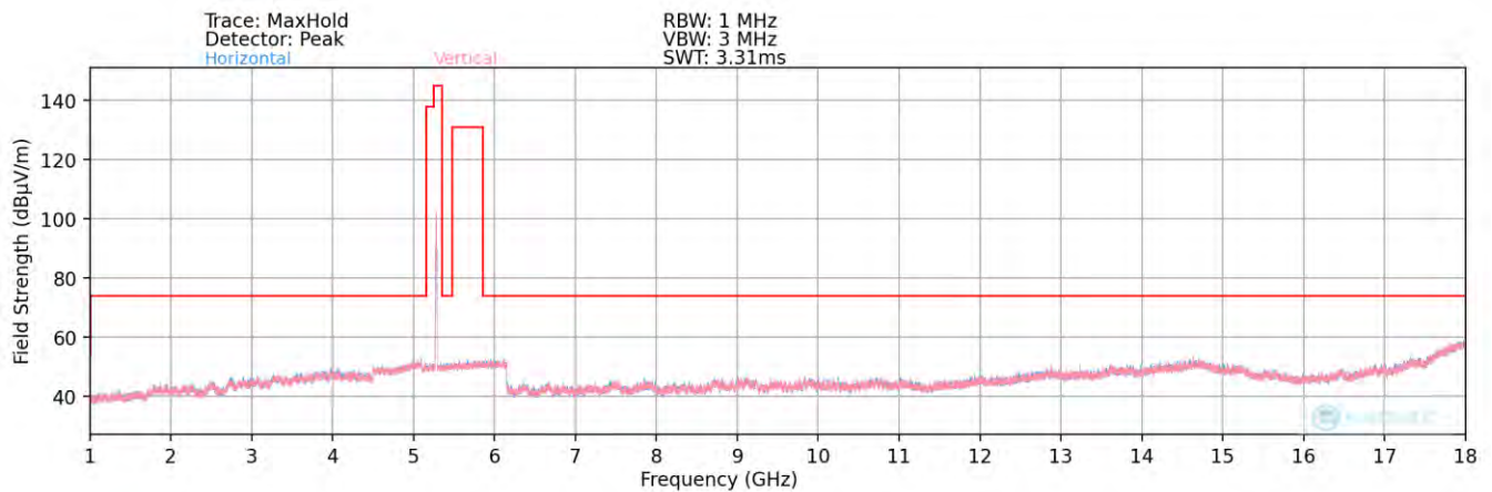
Plot 7-60. Radiated Spurious Plot above 1GHz (802.11ax – UNII 2A Ch. 56)
