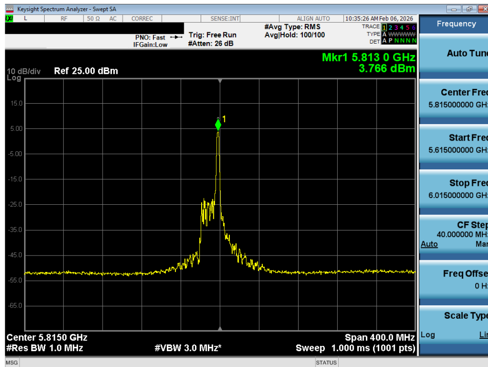
Plot 7-47. Power Spectral Density Plot SISO ANT1 (160MHz BW 802.11ax – 26 Tones (UNII Band 3/4) – Ch. 163)
