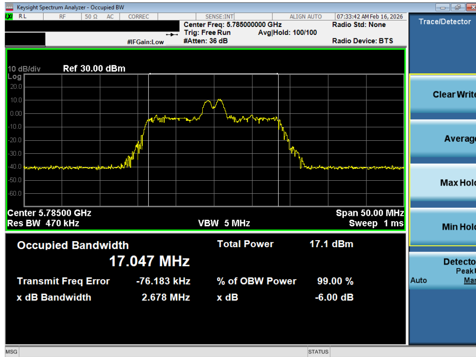
Plot 7-23. OBW Plot SISO ANT1 (20MHz BW 802.11ax – 26 Tones (UNII Band 3) – Ch. 157)
