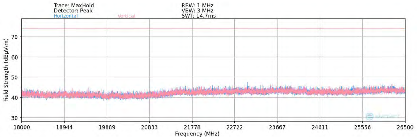
Plot 7-64. Radiated Spurious Plot 18GHz - 26.5GHz (802.11ax)
