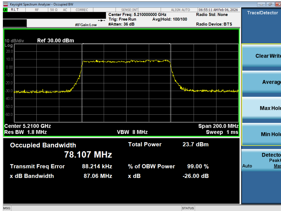
Plot 7-7. 26dB Bandwidth Plot SISO ANT1 (80MHz BW 802.11ax – 996 Tones (UNII Band 1) – Ch. 42)
