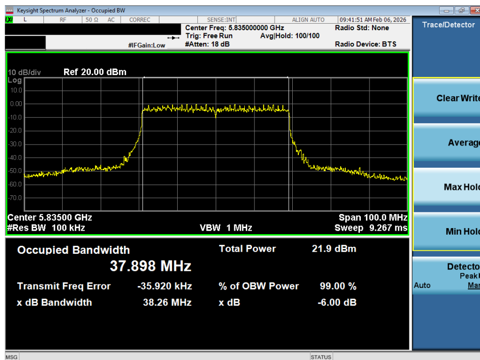
Plot 7-20. 6dB Bandwidth Plot SISO ANT1 (40MHz BW 802.11ax – 484 Tones (UNII Band 3/4) – Ch. 167)
