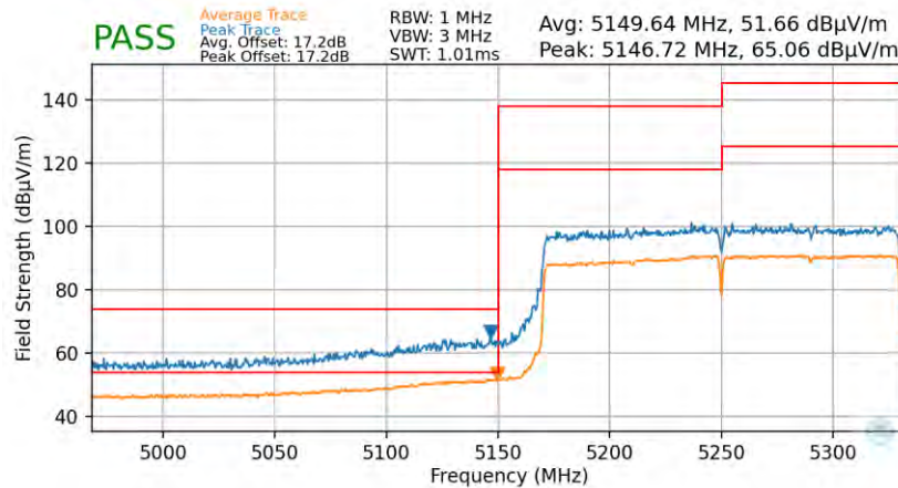
Plot 7-99. Radiated Lower Band Edge Plot (Average & Peak – UNII Band 1 – 2x996T)
