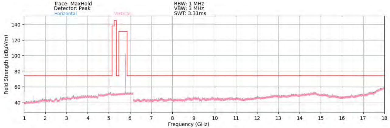
Plot 7-62. Radiated Spurious Plot above 1GHz (802.11ax – UNII 3 Ch. 157)
