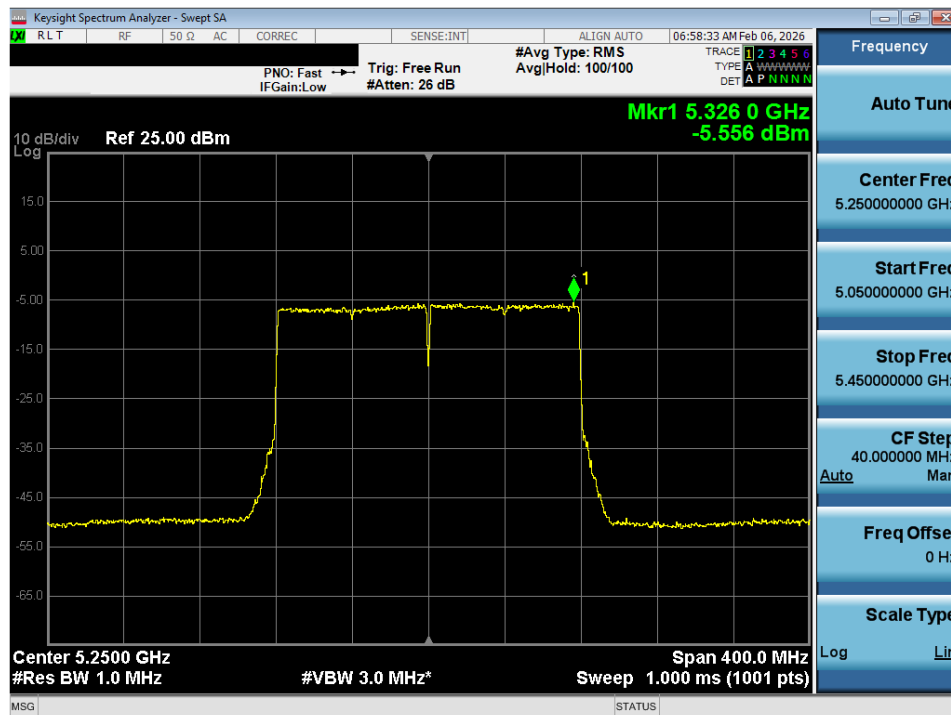
Plot 7-51. Power Spectral Density Plot SISO ANT1 (160MHz BW 802.11ax – 2x996 Tones (UNII Band 1/2A) – Ch. 50)
