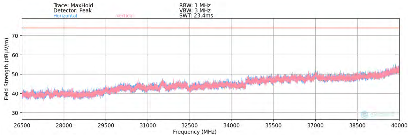
Plot 7-72. Radiated Spurious Plot 26.5GHz - 40GHz (802.11ax)
