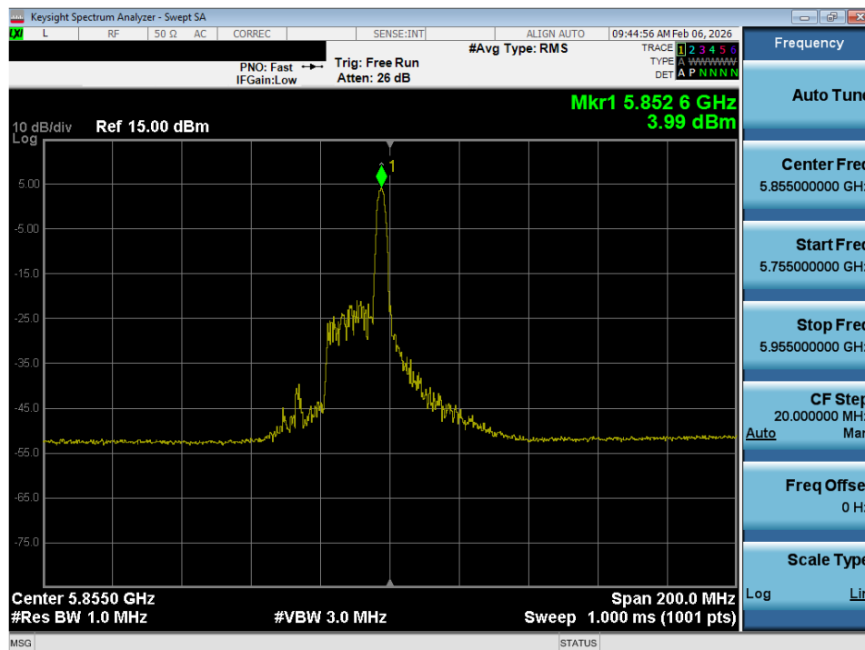
Plot 7-46. Power Spectral Density Plot SISO ANT1 (80MHz BW 802.11ax – 26 Tones (UNII Band 3/4) – Ch. 171)
