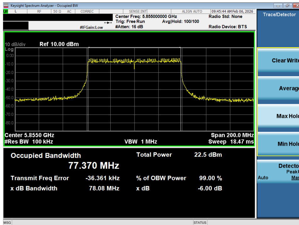
Plot 7-21. 6dB Bandwidth Plot SISO ANT1 (80MHz BW 802.11ax – 996 Tones (UNII Band 3/4) – Ch. 171)
