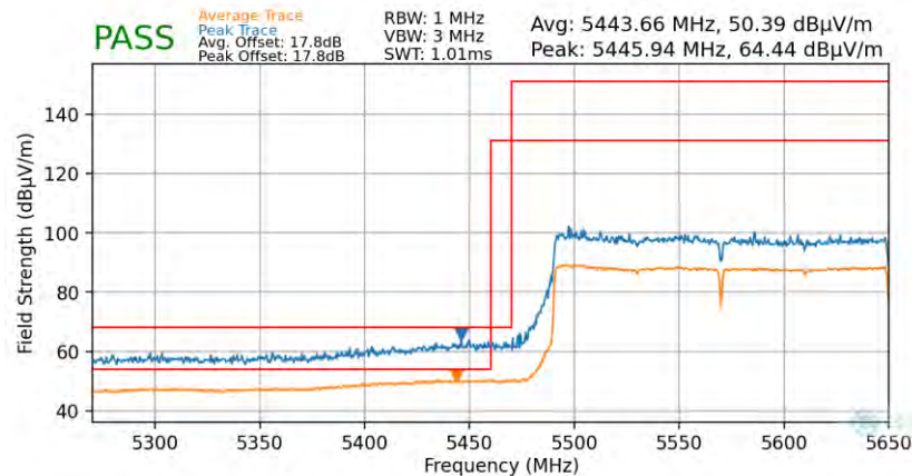
Plot 7-101. Radiated Lower Band Edge Plot (Average & Peak – UNII Band 2C – 2x996T)
