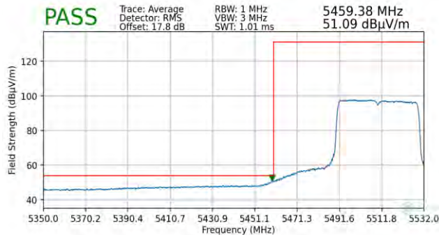
Plot 7-88. Radiated Lower Band Edge Plot (Average – UNII Band 2C – 484 Tones)
