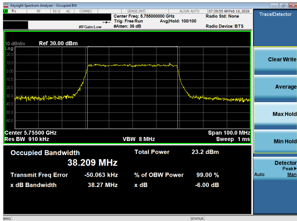
Plot 7-31. OBW Plot SISO ANT1 (40MHz BW 802.11ax – 484 Tones (UNII Band 3) – Ch. 151)
