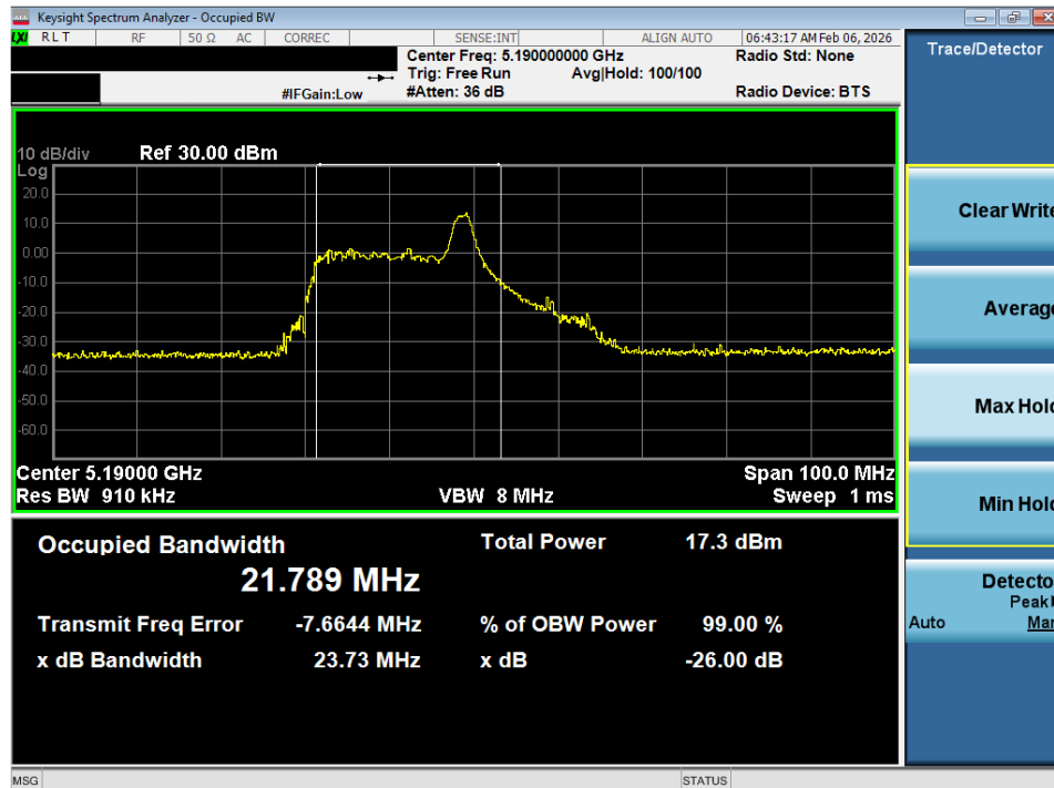
Plot 7-2. 26dB Bandwidth Plot SISO ANT1 (40MHz BW 802.11ax – 26 Tones (UNII Band 1) – Ch. 38)
