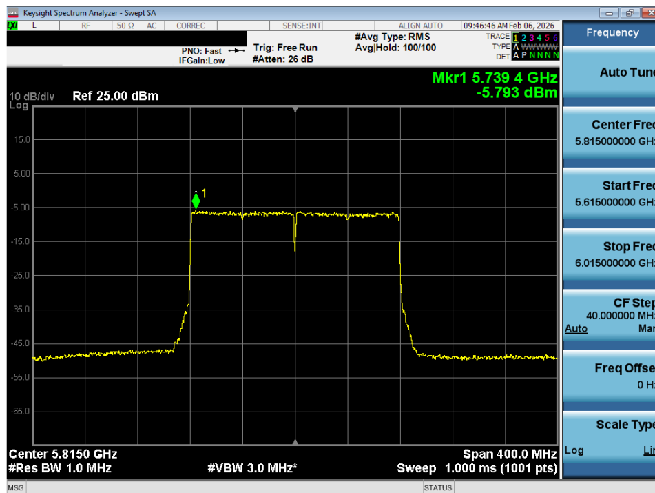
Plot 7-58. Power Spectral Density Plot SISO ANT1 (160MHz BW 802.11ax – 996*2 Tones (UNII Band 3/4) – Ch. 163)
