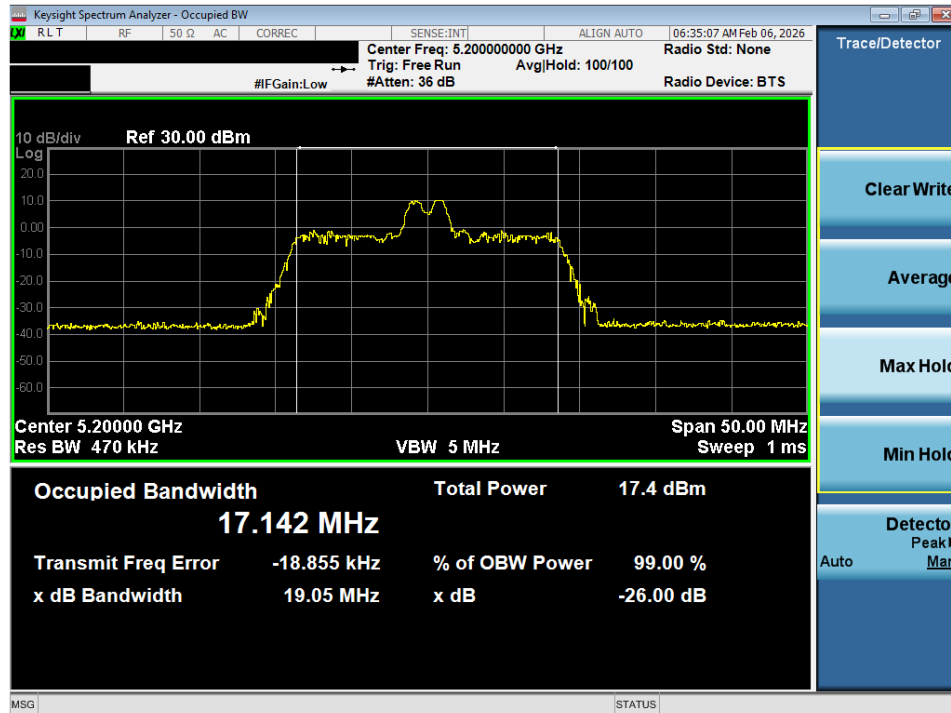
Plot 7-1. 26dB Bandwidth Plot SISO ANT1 (20MHz BW 802.11ax – 26 Tones (UNII Band 1) – Ch. 40)
