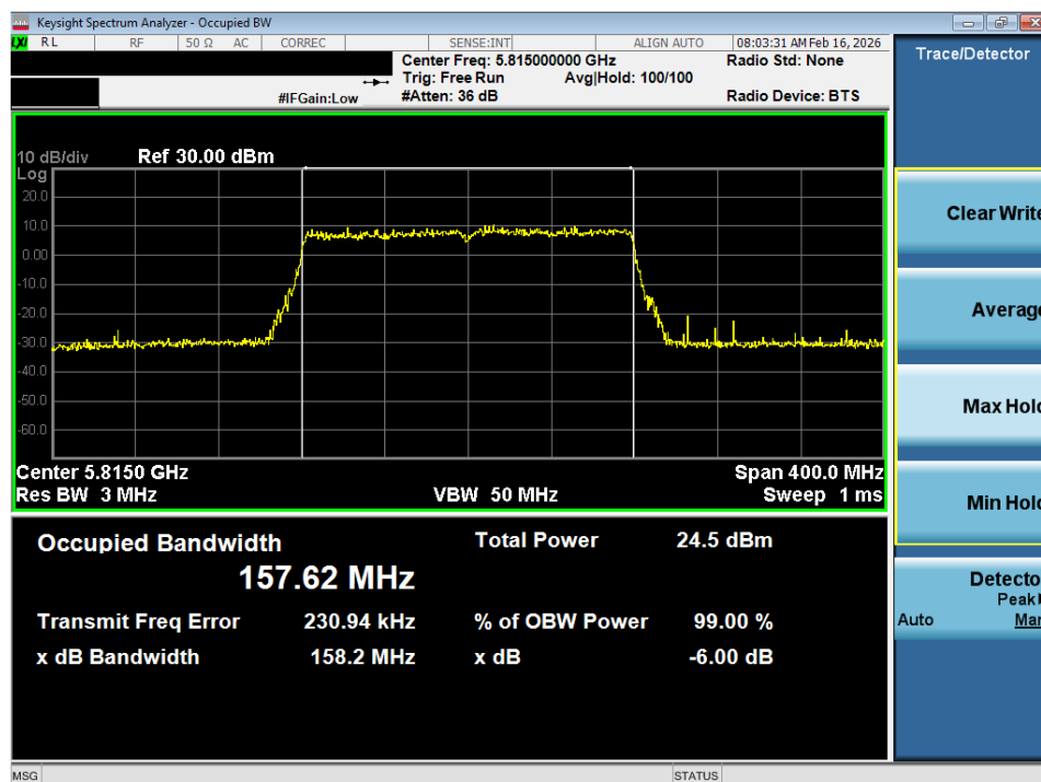
Plot 7-36. OBW Plot SISO ANT1 (160MHz BW 802.11ax – 996*2 Tones (UNII Band 3/4) – Ch. 163)
