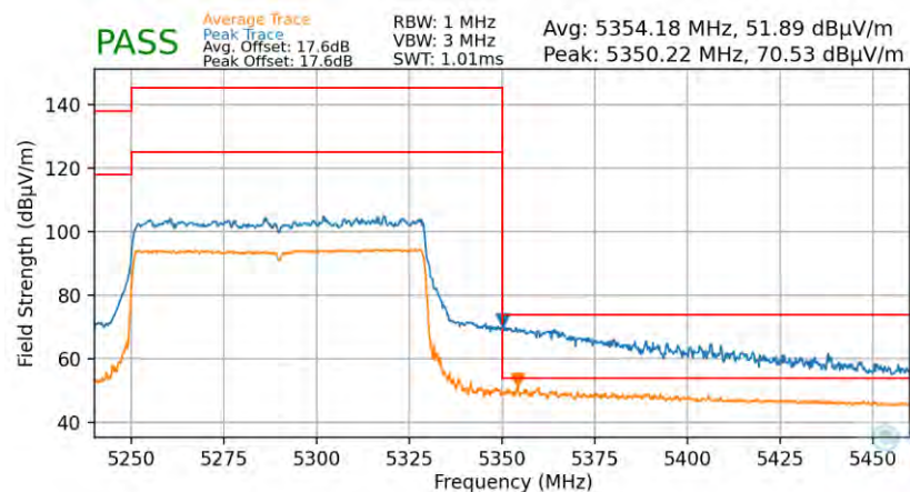
Plot 7-94. Radiated Upper Band Edge Plot (Average & Peak – UNII Band 2A – 996 Tones)
