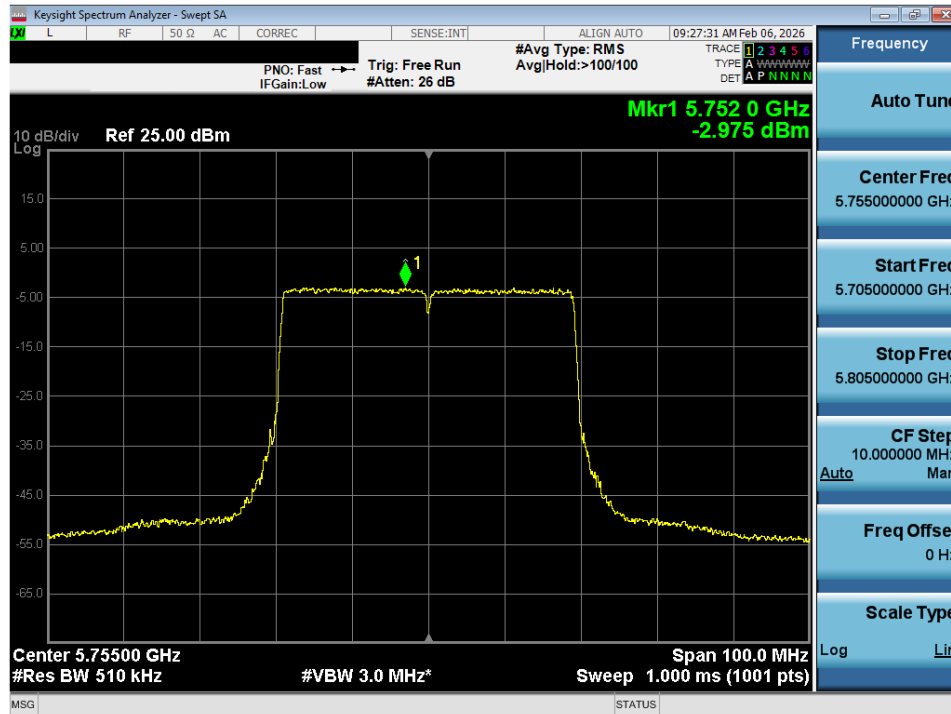
Plot 7-53. Power Spectral Density Plot SISO ANT1 (40MHz BW 802.11ax – 484 Tones (UNII Band 3) – Ch. 151)
