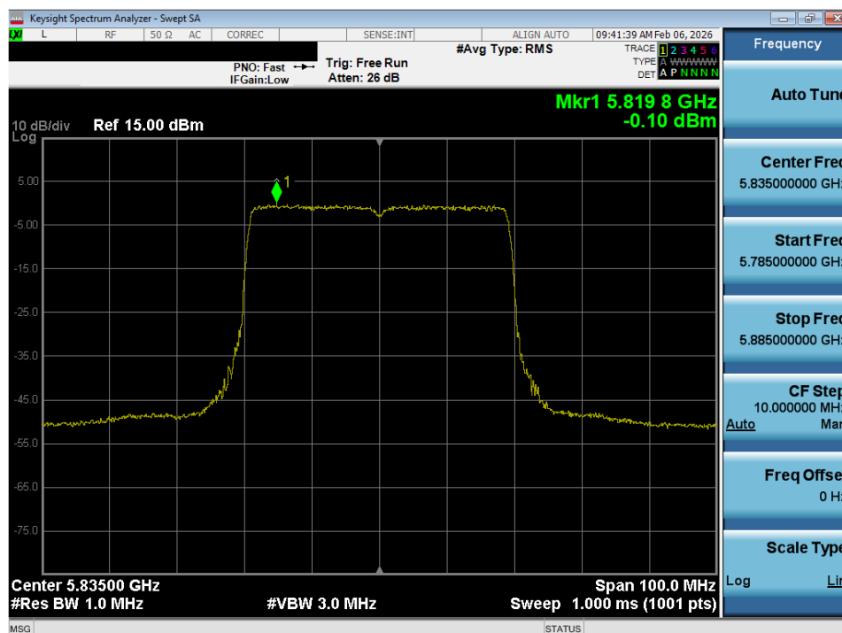
Plot 7-56. Power Spectral Density Plot SISO ANT1 (40MHz BW 802.11ax – 484 Tones (UNII Band 3/4) – Ch. 167)
