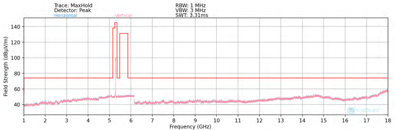
Plot 7-67. Radiated Spurious Plot above 1GHz (802.11ax – UNII 2A Ch. 56)
