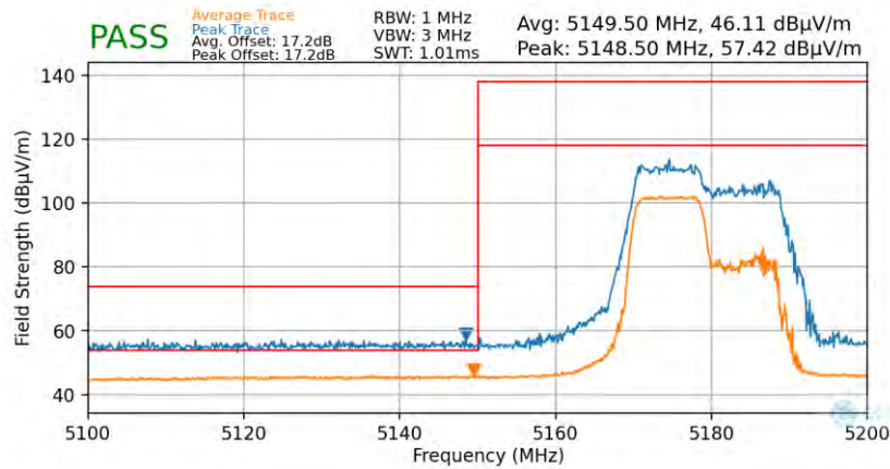
Plot 7-73. Radiated Lower Band Edge Plot (Average & Peak – UNII Band 1 – 106 Tones)
