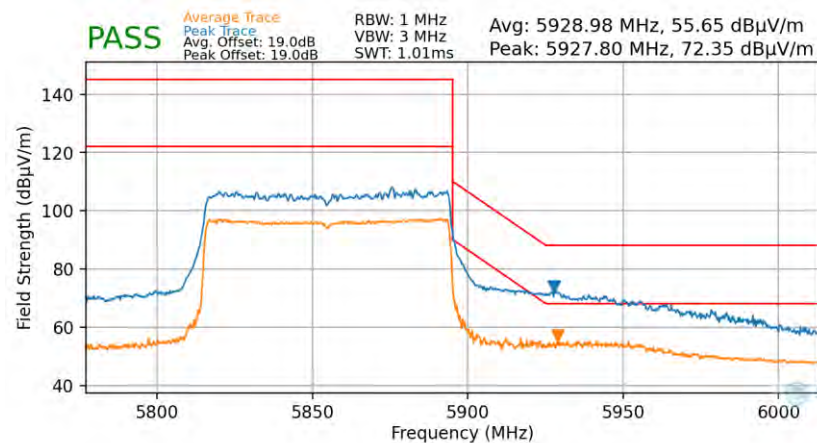
Plot 7-98. Radiated Upper Band Edge Plot (Average & Peak – UNII Band 4 – 996 Tones)
