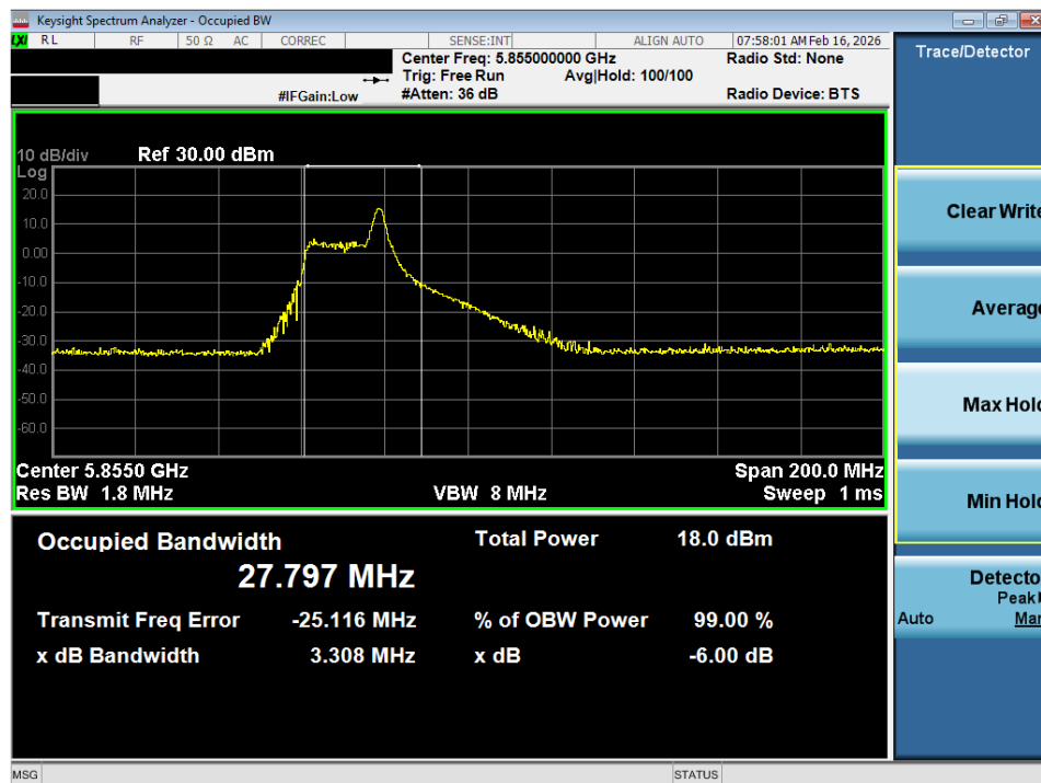
Plot 7-28. OBW Plot SISO ANT1 (80MHz BW 802.11ax – 26 Tones (UNII Band 3/4) – Ch. 171)
