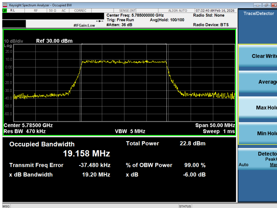
Plot 7-30. OBW Plot SISO ANT1 (20MHz BW 802.11ax – 242 Tones (UNII Band 3) – Ch. 157)
