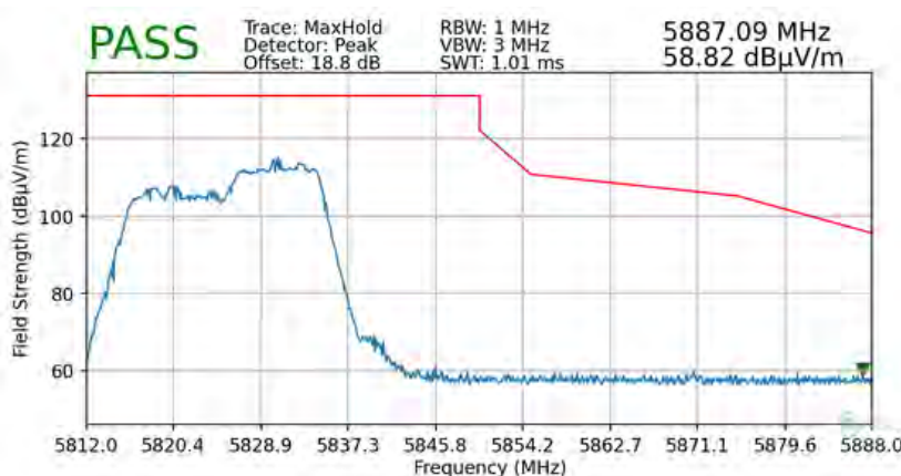
Plot 7-76. Radiated Upper Band Edge Plot (Peak – UNII Band 3 – 106 Tones)
