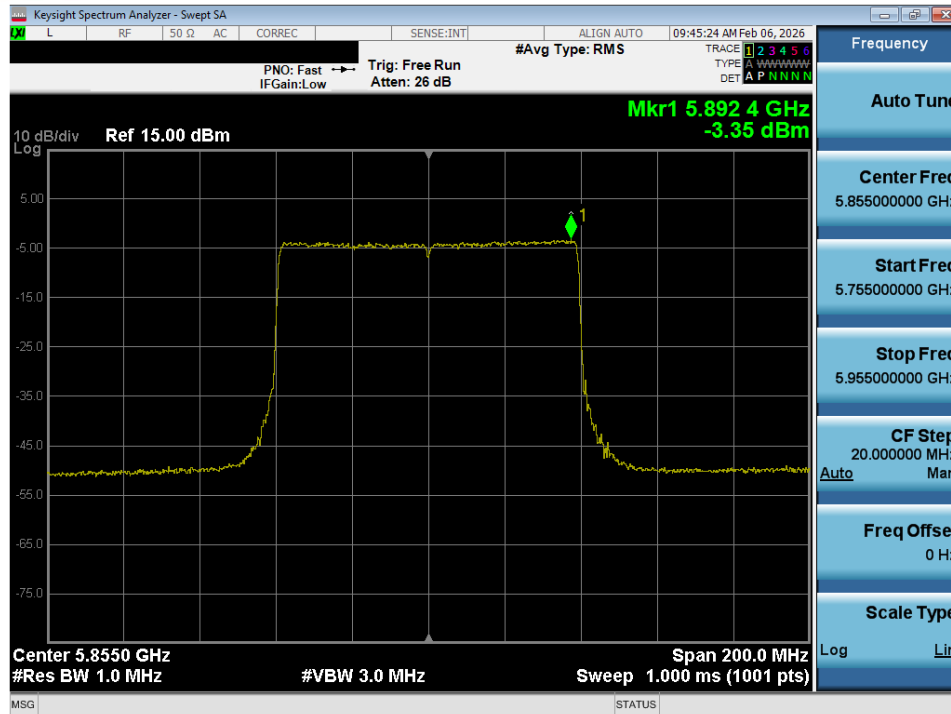
Plot 7-57. Power Spectral Density Plot SISO ANT1 (80MHz BW 802.11ax – 996 Tones (UNII Band 3/4) – Ch. 171)
