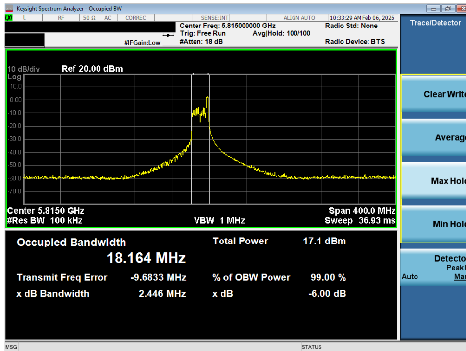
Plot 7-15. 6dB Bandwidth Plot SISO ANT1 (160MHz BW 802.11ax – 26 Tones (UNII Band 3/4) – Ch. 163)
