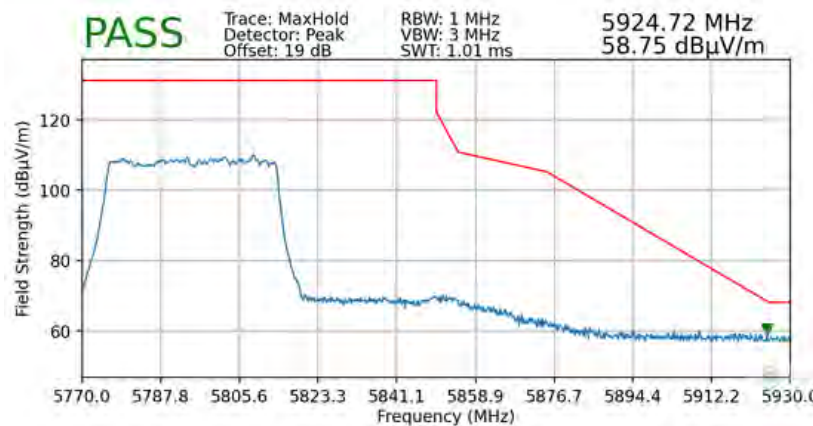
Plot 7-90. Radiated Upper Band Edge Plot (Peak – UNII Band 3 – 484 Tones)
