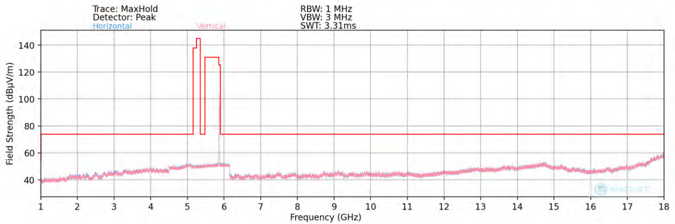
Plot 7-63. Radiated Spurious Plot above 1GHz (802.11ax – UNII 4 Ch. 173)
