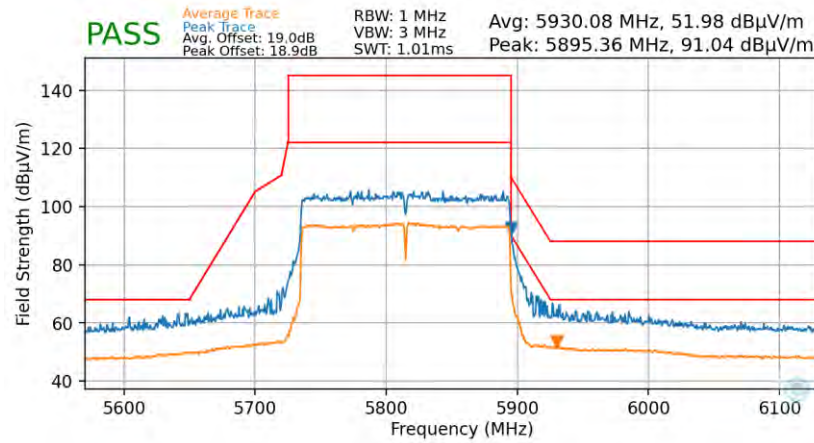
Plot 7-103. Radiated Upper Band Edge Plot (Average & Peak – UNII Band 4 – 2x996T)
