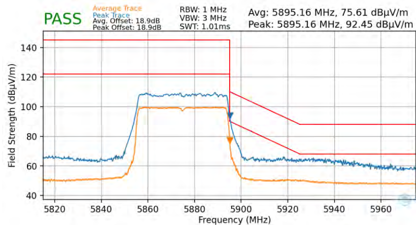
Plot 7-92. Radiated Upper Band Edge Plot (Average & Peak - UNII Band 4 - 484 Tones)
