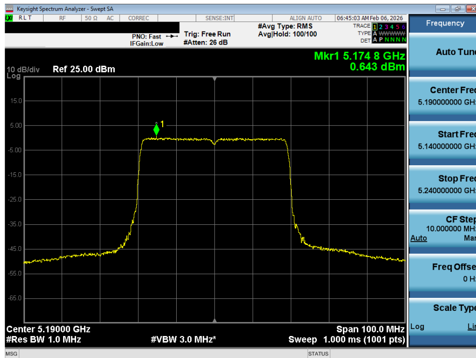
Plot 7-49. Power Spectral Density Plot SISO ANT1 (40MHz BW 802.11ax – 484 Tones (UNII Band 1) – Ch. 38)
