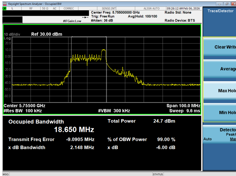
Plot 7-10. 6dB Bandwidth Plot SISO ANT1 (40MHz BW 802.11ax – 26 Tones (UNII Band 3) – Ch. 151)
