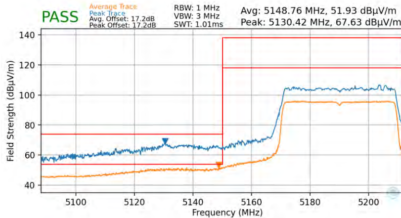
Plot 7-86. Radiated Lower Band Edge Plot (Average & Peak – UNII Band 1 – 484 Tones)
