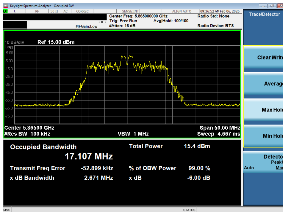
Plot 7-12. 6dB Bandwidth Plot SISO ANT1 (20MHz BW 802.11ax – 26 Tones (UNII Band 4) – Ch. 173)
