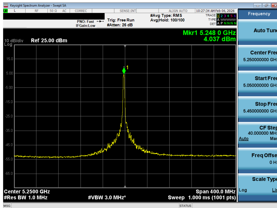
Plot 7-40. Power Spectral Density Plot SISO ANT1 (160MHz BW 802.11ax – 26 Tones (UNII Band 1/2A) – Ch. 50)
