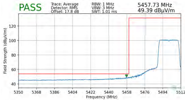
Plot 7-81. Radiated Lower Band Edge Plot (Average – UNII Band 2C – 242 Tones)
