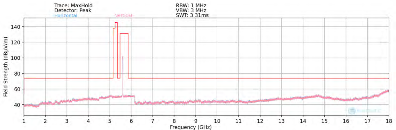
Plot 7-68. Radiated Spurious Plot above 1GHz (802.11ax – UNII 2C Ch. 120)
