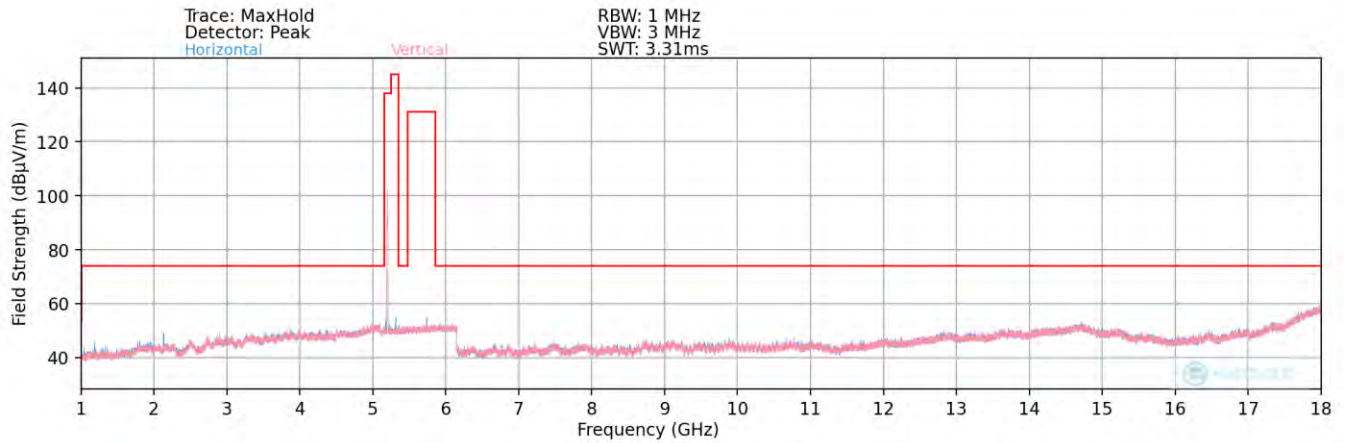
Plot 7-59. Radiated Spurious Plot above 1GHz (802.11ax – UNII 1 Ch. 40)
