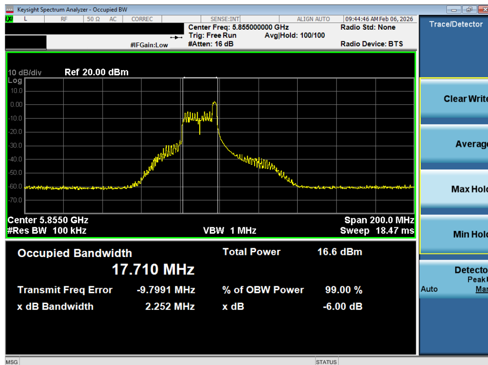
Plot 7-14. 6dB Bandwidth Plot SISO ANT1 (80MHz BW 802.11ax – 26 Tones (UNII Band 3/4) – Ch. 171)
