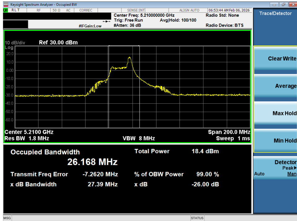
Plot 7-3. 26dB Bandwidth Plot SISO ANT1 (80MHz BW 802.11ax – 26 Tones (UNII Band 1) – Ch. 42)
