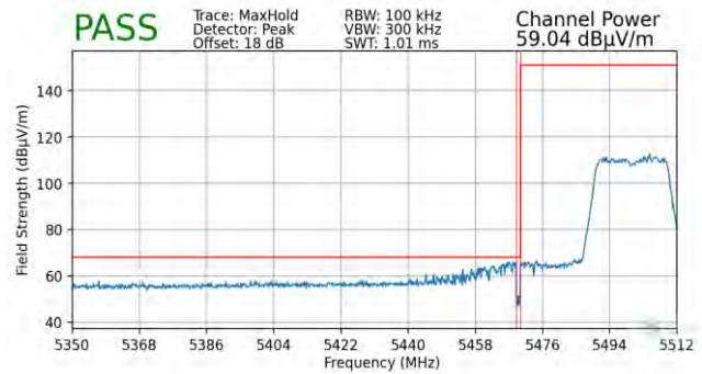
Plot 7-82. Radiated Lower Band Edge Plot (Peak – UNII Band 2C – 242 Tones)
