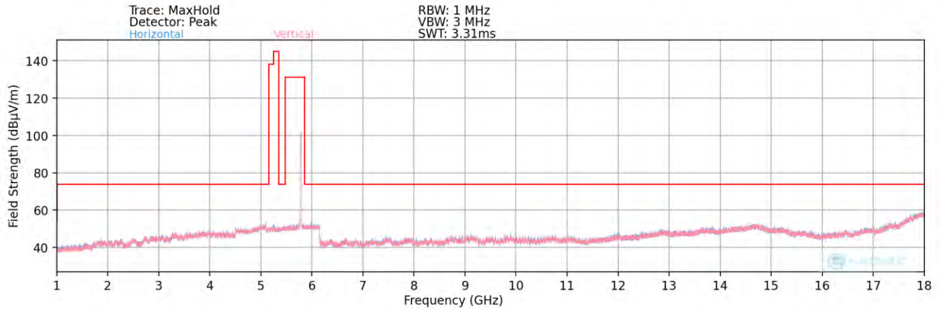
Plot 7-69. Radiated Spurious Plot above 1GHz (802.11ax – UNII 3 Ch. 157)
