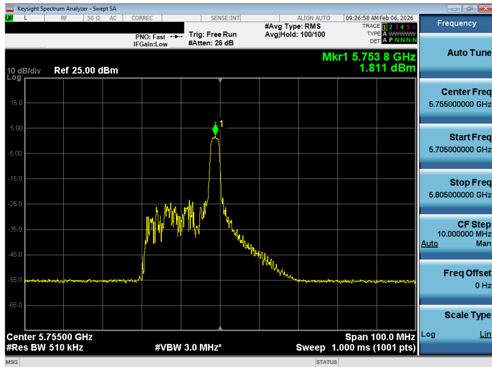
Plot 7-42. Power Spectral Density Plot SISO ANT1 (40MHz BW 802.11ax – 26 Tones (UNII Band 3) – Ch. 151)
