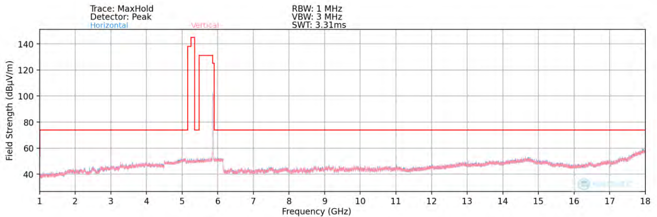
Plot 7-70. Radiated Spurious Plot above 1GHz (802.11ax – UNII 4 Ch. 173)
