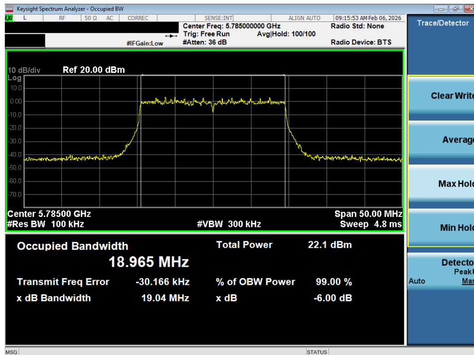
Plot 7-16. 6dB Bandwidth Plot SISO ANT1 (20MHz BW 802.11ax – 242 Tones (UNII Band 3) – Ch. 157)
