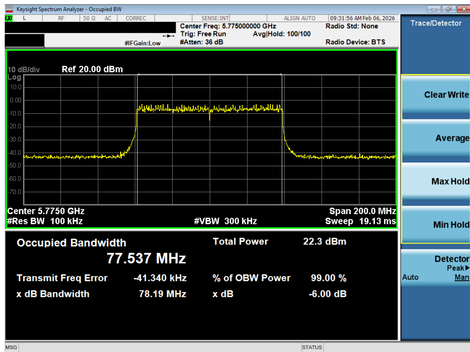
Plot 7-18. 6dB Bandwidth Plot SISO ANT1 (80MHz BW 802.11ax – 996 Tones (UNII Band 3) – Ch. 155)
