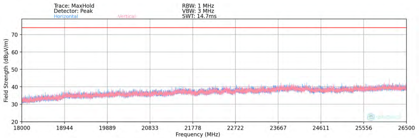
Plot 7-71. Radiated Spurious Plot 18GHz - 26.5GHz (802.11ax)
