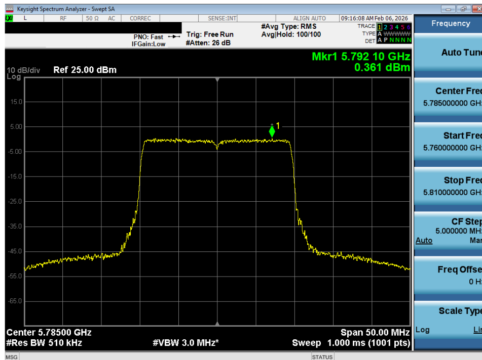
Plot 7-52. Power Spectral Density Plot SISO ANT1 (20MHz BW 802.11ax – 242 Tones (UNII Band 3) – Ch. 157)
