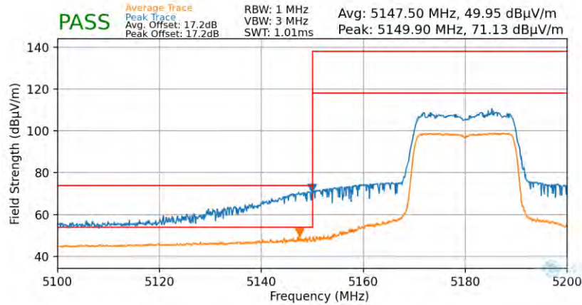
Plot 7-79. Radiated Lower Band Edge Plot (Average & Peak – UNII Band 1 – 242 Tones)
