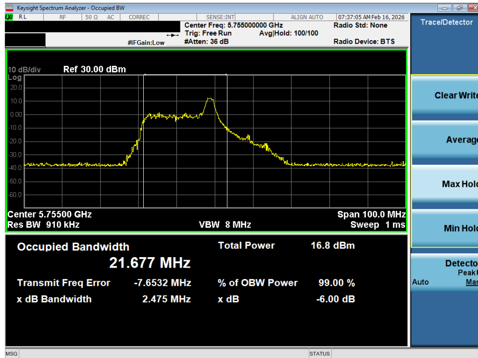
Plot 7-24. OBW Plot SISO ANT1 (40MHz BW 802.11ax – 26 Tones (UNII Band 3) – Ch. 151)
