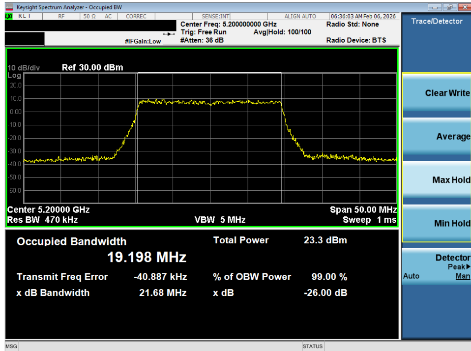
Plot 7-5. 26dB Bandwidth Plot SISO ANT1 (20MHz BW 802.11ax – 242 Tones (UNII Band 1) – Ch. 40)
