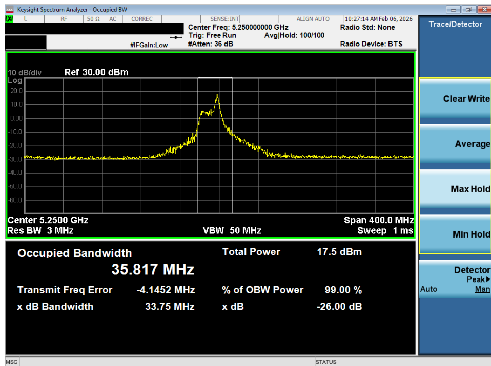
Plot 7-4. 26dB Bandwidth Plot SISO ANT1 (160MHz BW 802.11ax – 26 Tones (UNII Band 1/2A) – Ch. 50)
