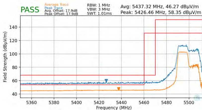
Plot 7-75. Radiated Lower Band Edge Plot (Average & Peak – UNII Band 2C – 106 Tones)
