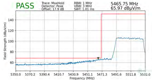
Plot 7-89. Radiated Lower Band Edge Plot (Peak – UNII Band 2C – 484 Tones)
