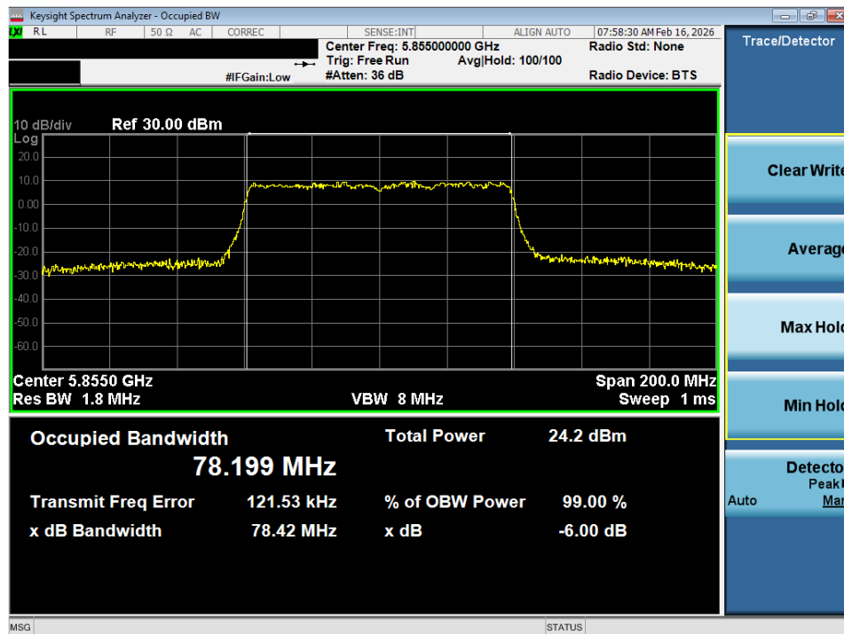
Plot 7-35. OBW Plot SISO ANT1 (80MHz BW 802.11ax – 996 Tones (UNII Band 3/4) – Ch. 171)
