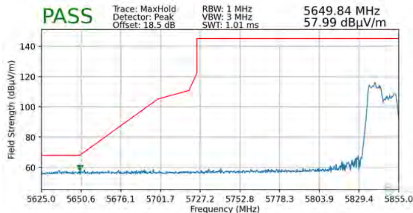
Plot 7-77. Radiated Lower Band Edge Plot (Peak – UNII Band 4 – 106 Tones)
