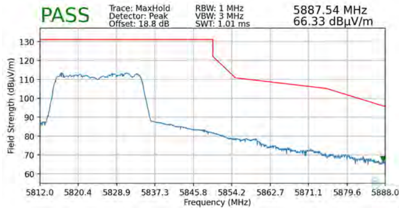
Plot 7-83. Radiated Upper Band Edge Plot (Peak – UNII Band 3 – 242 Tones)
