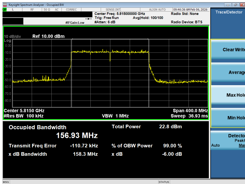
Plot 7-22. 6dB Bandwidth Plot SISO ANT1 (160MHz BW 802.11ax – 996*2 Tones (UNII Band 3/4) – Ch. 163)
