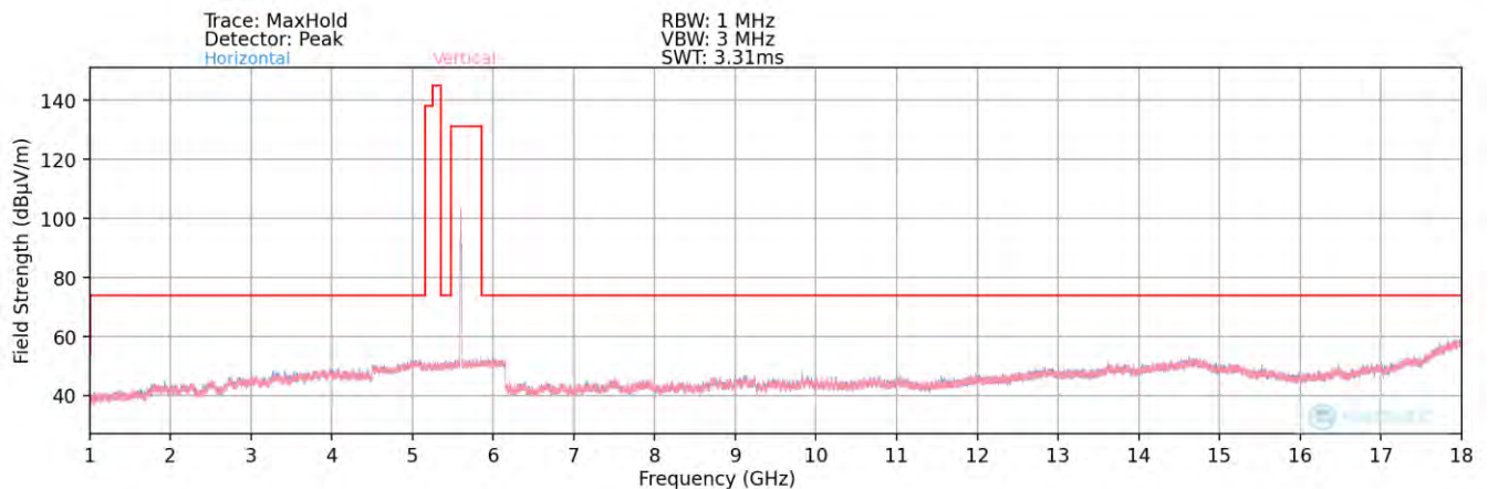
Plot 7-61. Radiated Spurious Plot above 1GHz (802.11ax – UNII 2C Ch. 120)
