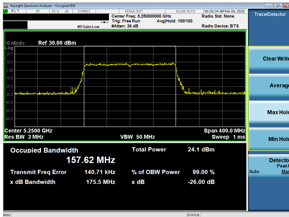
Plot 7-8. 26dB Bandwidth Plot SISO ANT1 (160MHz BW 802.11ax – 2x996 Tones (UNII Band 1/2A) – Ch. 50)
