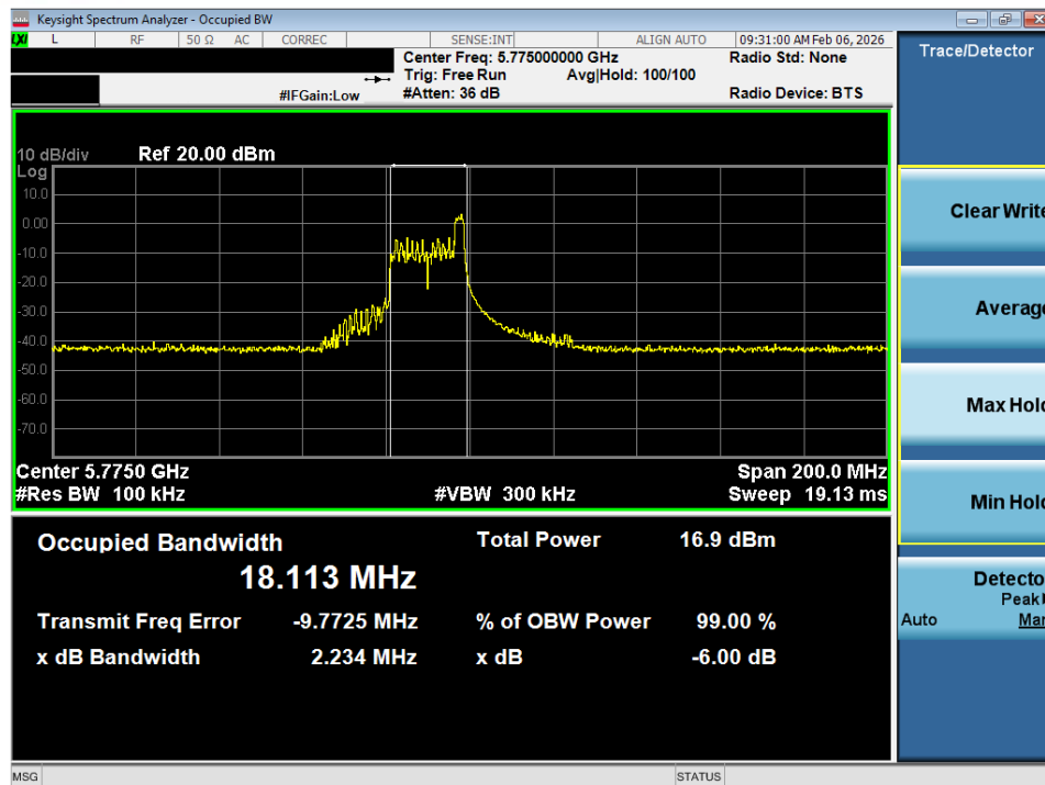
Plot 7-11. 6dB Bandwidth Plot SISO ANT1 (80MHz BW 802.11ax – 26 Tones (UNII Band 3) – Ch. 155)
