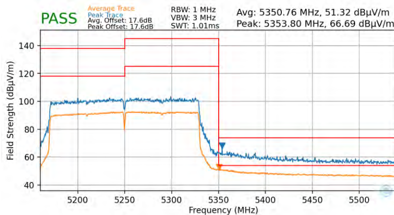
Plot 7-100. Radiated Upper Band Edge Plot (Average & Peak – UNII Band 2A – 2x996T)
