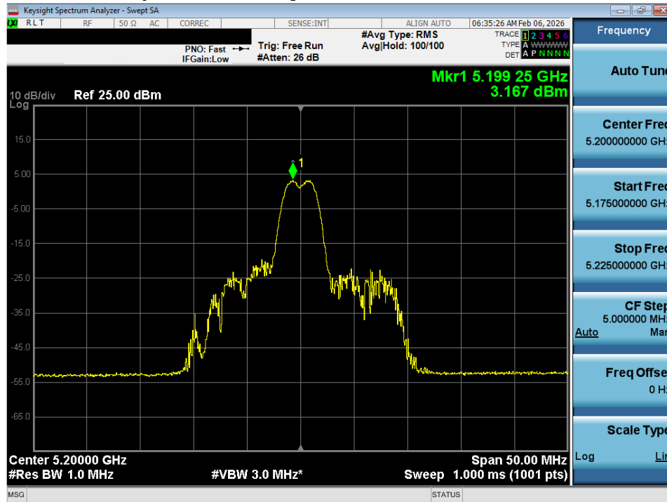
Plot 7-37. Power Spectral Density Plot SISO ANT1 (20MHz BW 802.11ax – 26 Tones (UNII Band 1) – Ch. 40)
