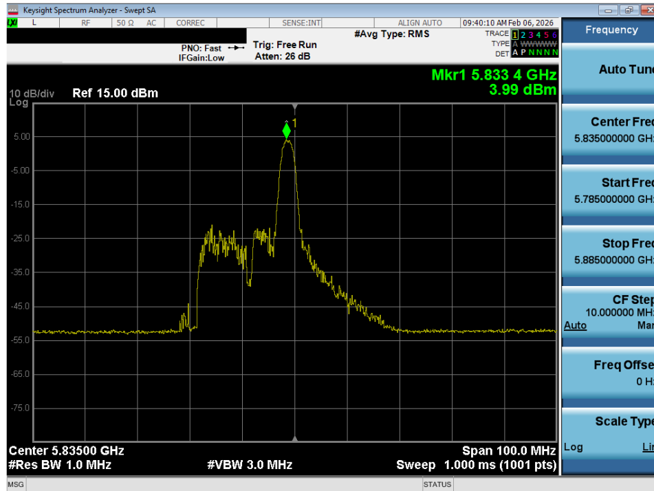
Plot 7-45. Power Spectral Density Plot SISO ANT1 (40MHz BW 802.11ax – 26 Tones (UNII Band 3/4) – Ch. 167)
