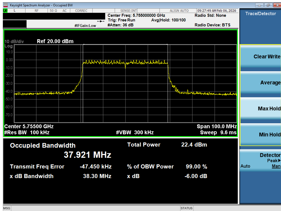
Plot 7-17. 6dB Bandwidth Plot SISO ANT1 (40MHz BW 802.11ax – 484 Tones (UNII Band 3) – Ch. 151)
