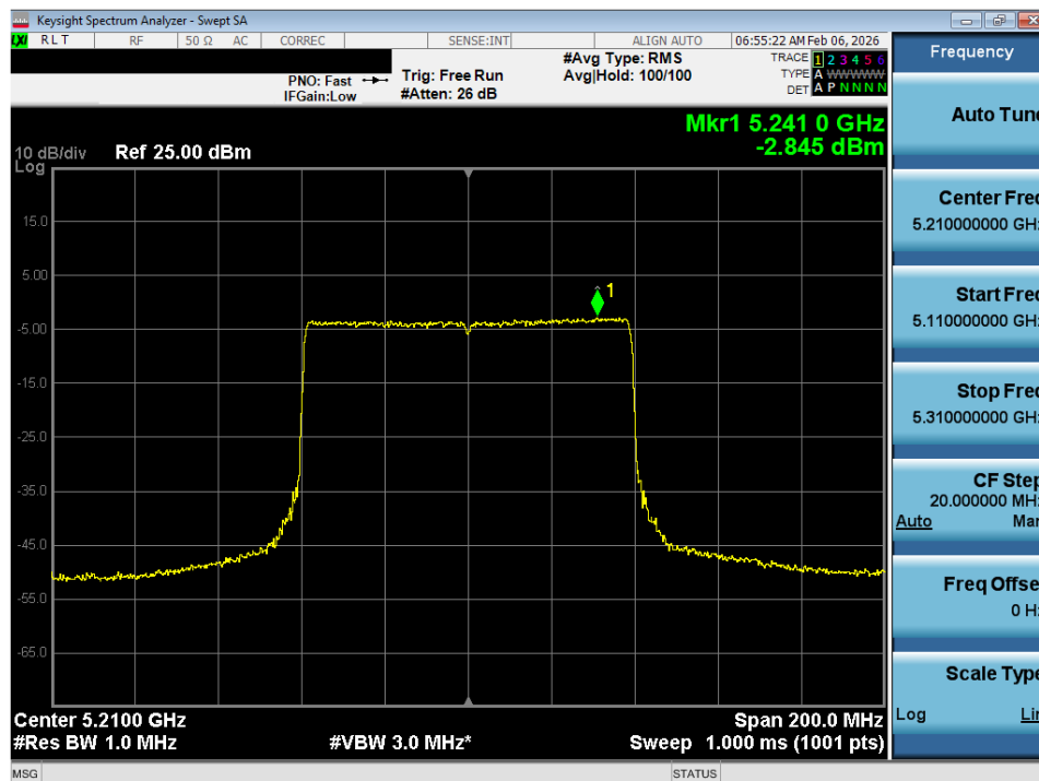
Plot 7-50. Power Spectral Density Plot SISO ANT1 (80MHz BW 802.11ax – 996 Tones (UNII Band 1) – Ch. 42)
