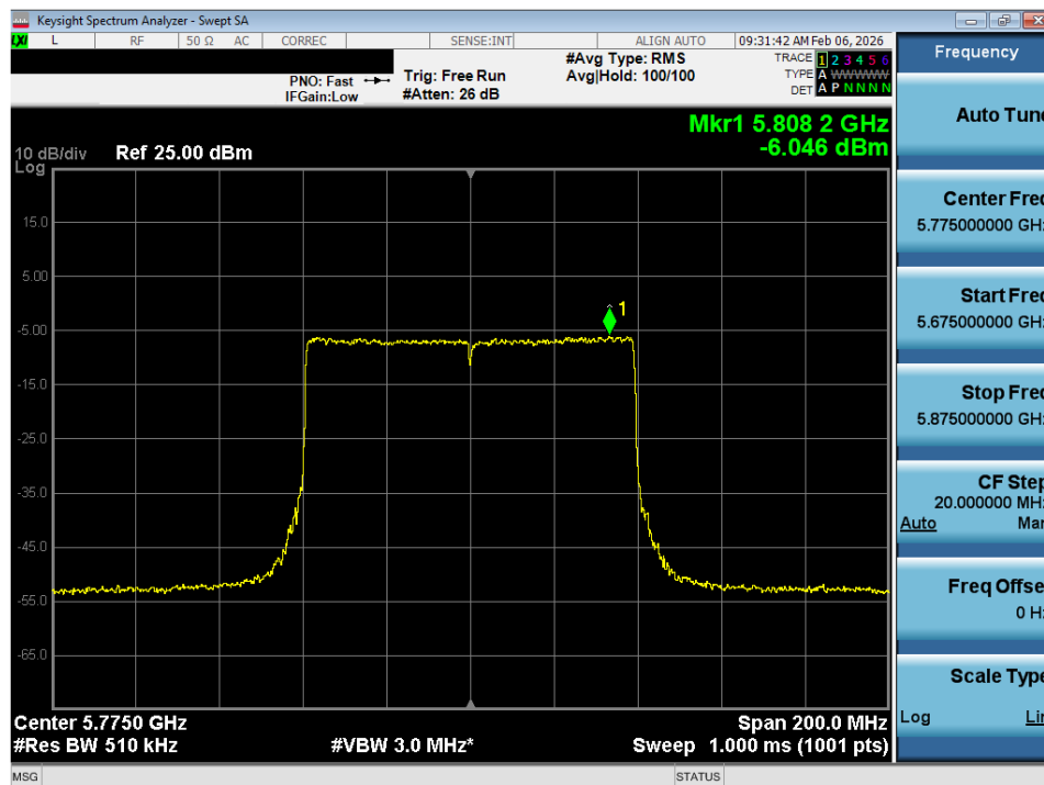
Plot 7-54. Power Spectral Density Plot SISO ANT1 (80MHz BW 802.11ax – 996 Tones (UNII Band 3) – Ch. 155)
