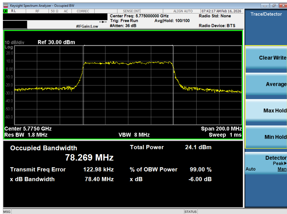
Plot 7-32. OBW Plot SISO ANT1 (80MHz BW 802.11ax – 996 Tones (UNII Band 3) – Ch. 155)
