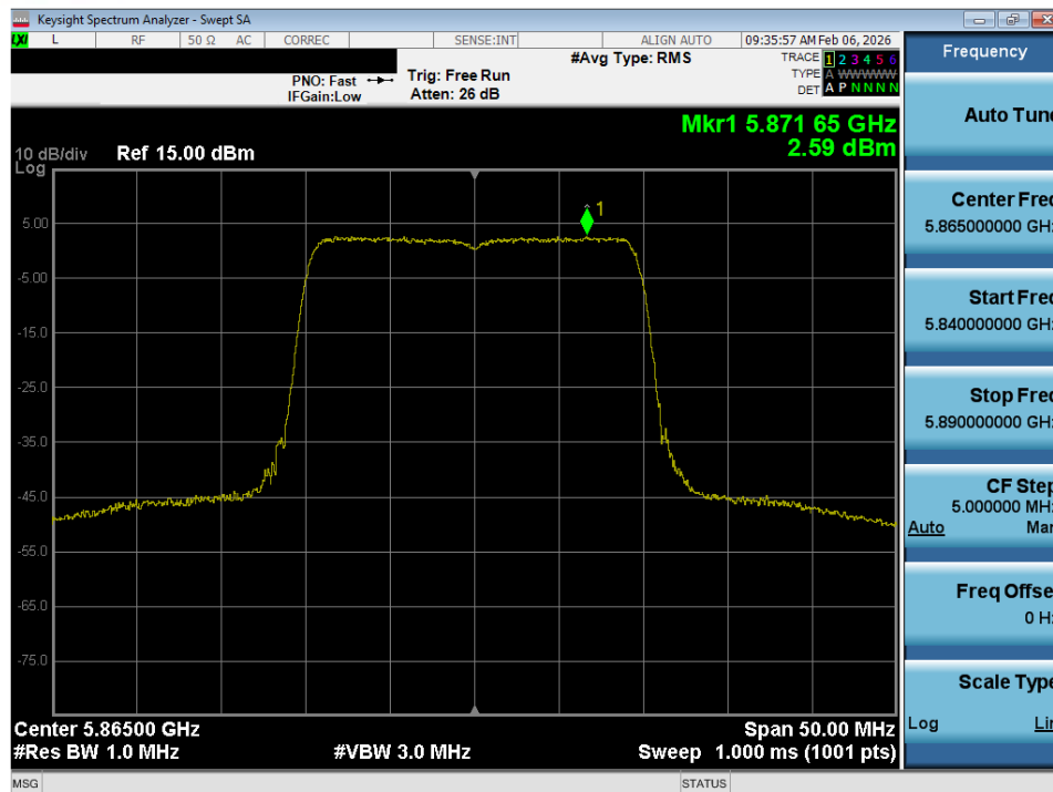
Plot 7-55. Power Spectral Density Plot SISO ANT1 (20MHz BW 802.11ax – 242 Tones (UNII Band 4) – Ch. 173)
