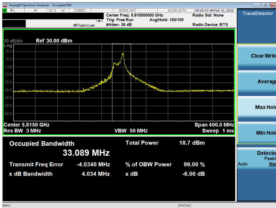
Plot 7-29. OBW Plot SISO ANT1 (160MHz BW 802.11ax – 26 Tones (UNII Band 3/4) – Ch. 163)
