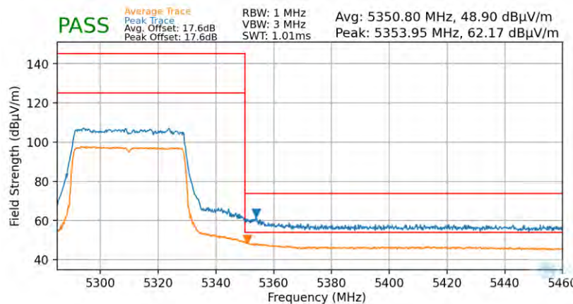
Plot 7-87. Radiated Upper Band Edge Plot (Average & Peak – UNII Band 2A – 484 Tones)
