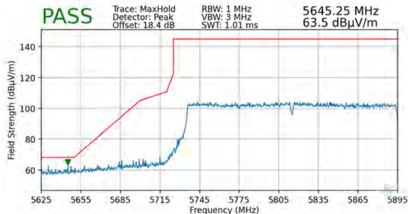
Plot 7-102. Radiated Lower Band Edge Plot (Peak – UNII Band 4 – 2x996T)
