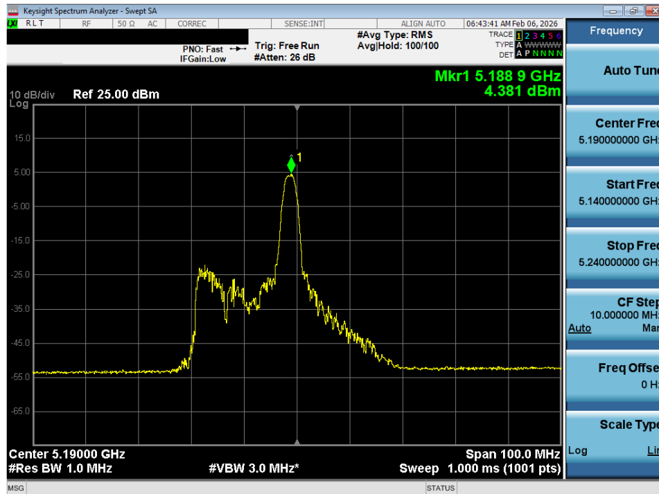
Plot 7-38. Power Spectral Density Plot SISO ANT1 (40MHz BW 802.11ax – 26 Tones (UNII Band 1) – Ch. 38)
