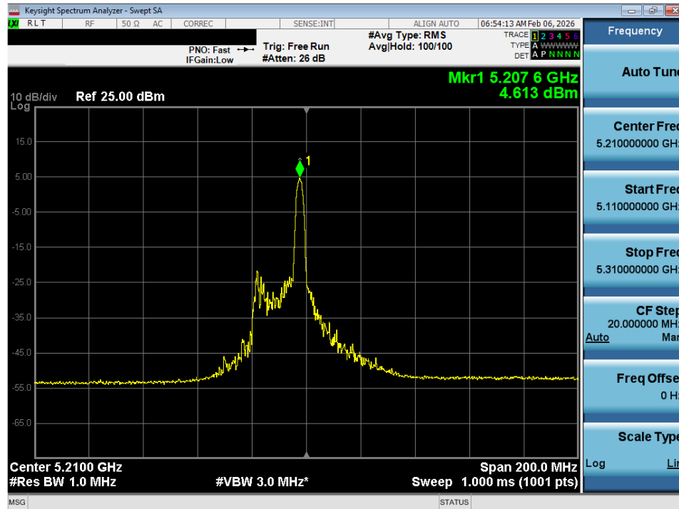
Plot 7-39. Power Spectral Density Plot SISO ANT1 (80MHz BW 802.11ax – 26 Tones (UNII Band 1) – Ch. 42)
