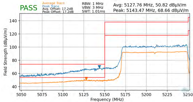
Plot 7-93. Radiated Lower Band Edge Plot (Average & Peak – UNII Band 1 – 996 Tones)
