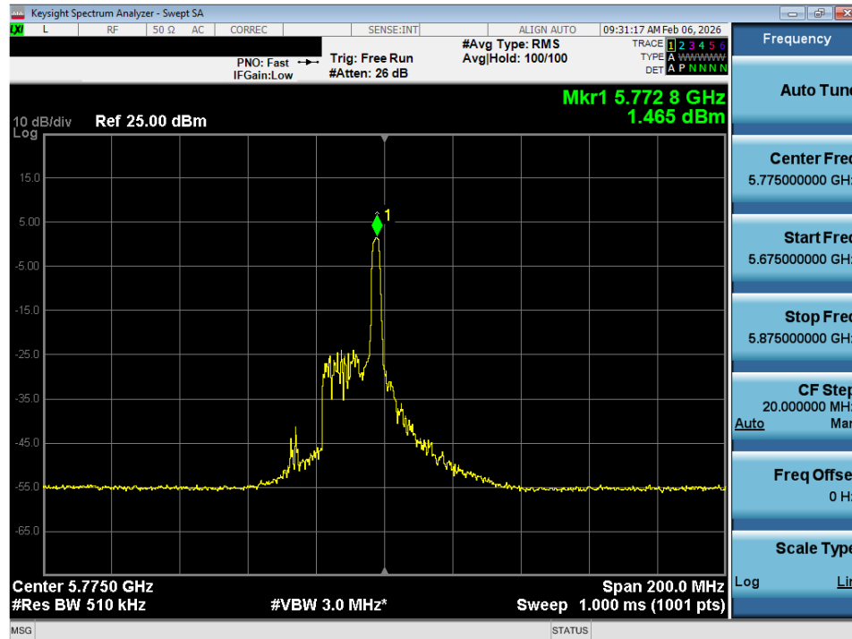
Plot 7-43. Power Spectral Density Plot SISO ANT1 (80MHz BW 802.11ax – 26 Tones (UNII Band 3) – Ch. 155)
