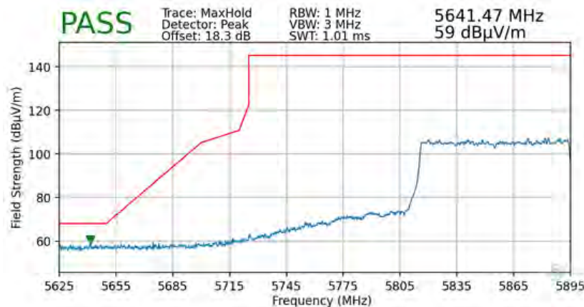
Plot 7-97. Radiated Lower Band Edge Plot (Peak – UNII Band 4 – 996 Tones)
