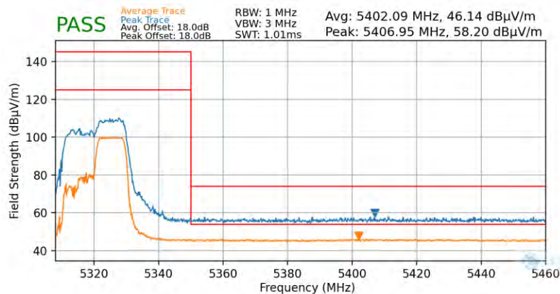
Plot 7-74. Radiated Upper Band Edge Plot (Average & Peak – UNII Band 2A – 106 Tones)
