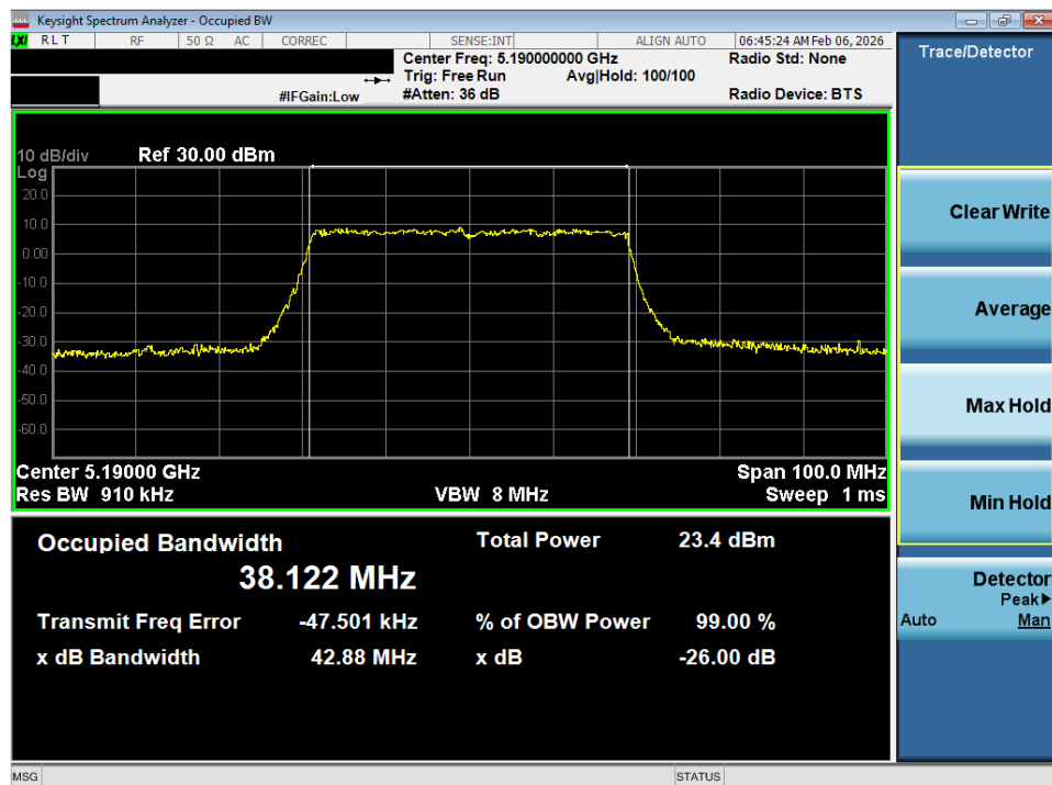
Plot 7-6. 26dB Bandwidth Plot SISO ANT1 (40MHz BW 802.11ax – 484 Tones (UNII Band 1) – Ch. 38)
