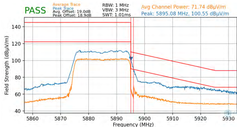
Plot 7-85. Radiated Upper Band Edge Plot (Average & Peak - UNII Band 4 - 242 Tones)
