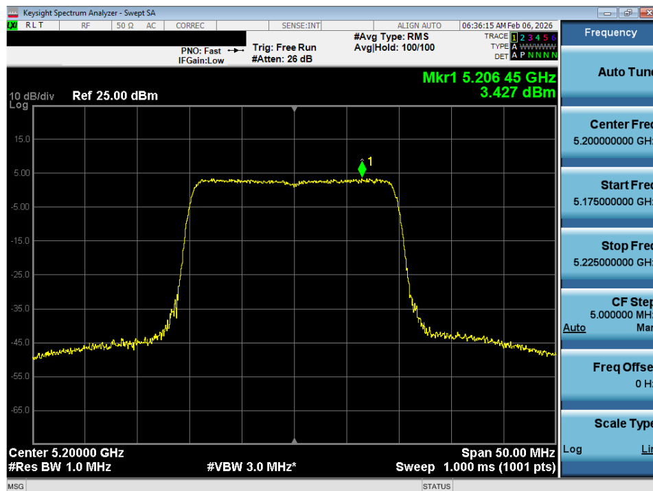
Plot 7-48. Power Spectral Density Plot SISO ANT1 (20MHz BW 802.11ax – 242 Tones (UNII Band 1) – Ch. 40)
