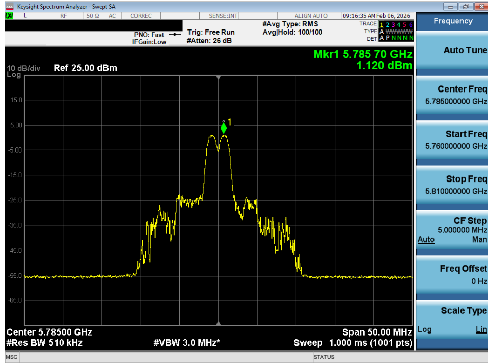
Plot 7-41. Power Spectral Density Plot SISO ANT1 (20MHz BW 802.11ax – 26 Tones (UNII Band 3) – Ch. 157)
