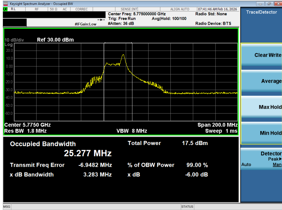
Plot 7-25. OBW Plot SISO ANT1 (80MHz BW 802.11ax – 26 Tones (UNII Band 3) – Ch. 155)
