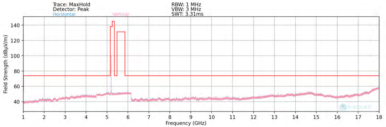
Plot 7-66. Radiated Spurious Plot above 1GHz (802.11ax – UNII 1 Ch. 40)
