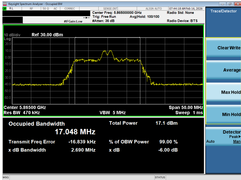
Plot 7-26. OBW Plot SISO ANT1 (20MHz BW 802.11ax – 26 Tones (UNII Band 4) – Ch. 173)
