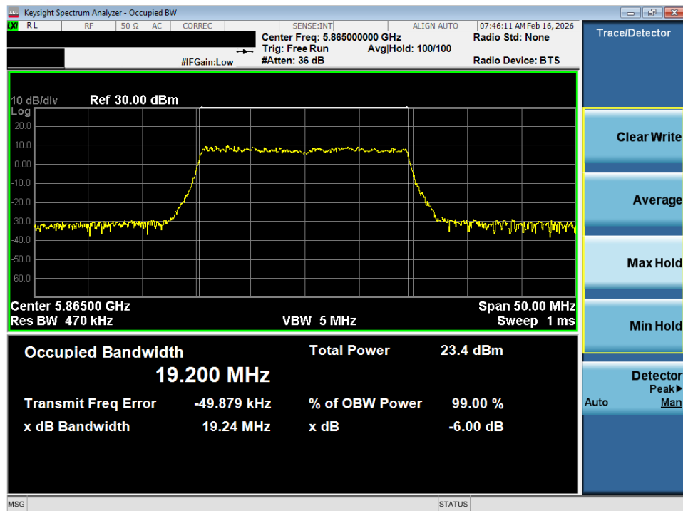
Plot 7-33. OBW Plot SISO ANT1 (20MHz BW 802.11ax – 242 Tones (UNII Band 4) – Ch. 173)
