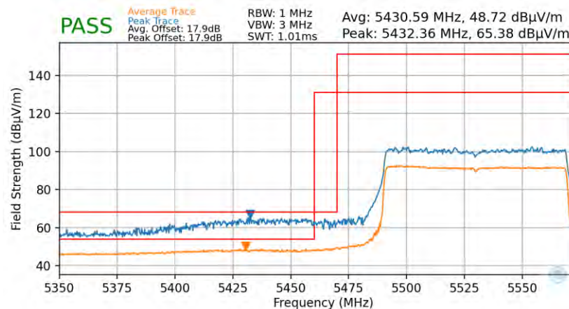
Plot 7-95. Radiated Lower Band Edge Plot (Average & Peak – UNII Band 2C – 996 Tones)
