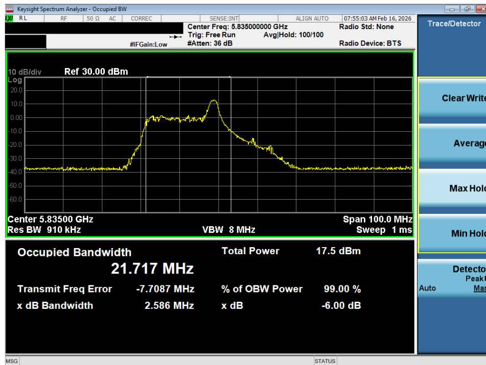
Plot 7-27. OBW Plot SISO ANT1 (40MHz BW 802.11ax – 26 Tones (UNII Band 3/4) – Ch. 167)
