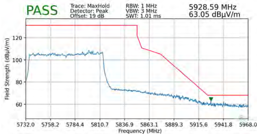
Plot 7-96. Radiated Upper Band Edge Plot (Peak – UNII Band 3 – 996 Tones)
