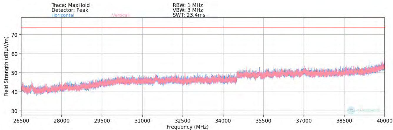
Plot 7-65. Radiated Spurious Plot 26.5GHz - 40GHz (802.11ax)
