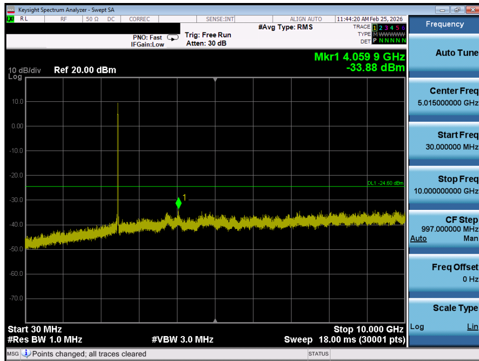
Plot 7-57. Conducted Spurious Plot SISO ANT1 (802.11b – Ch. 11)
