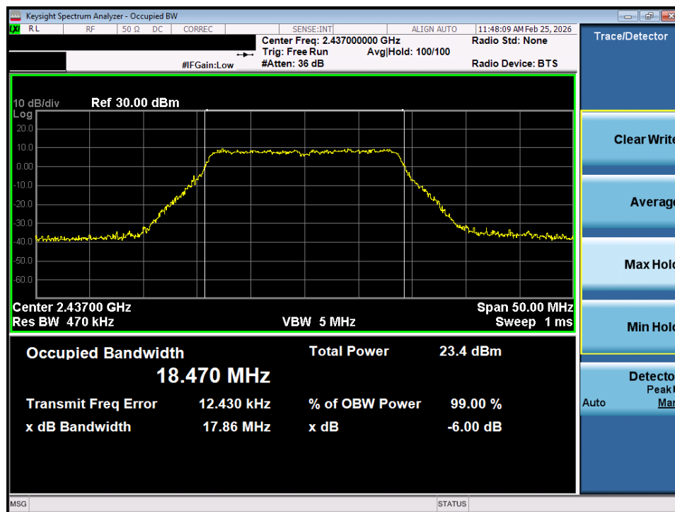
Plot 7-20. OBW Plot SISO ANT1 (802.11n/ac (2.4GHz) – Ch. 6)
