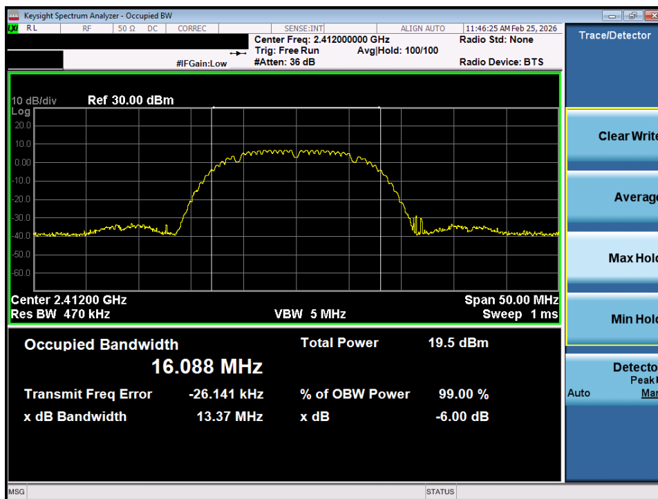
Plot 7-13. OBW Plot SISO ANT1 (802.11b – Ch. 1)
