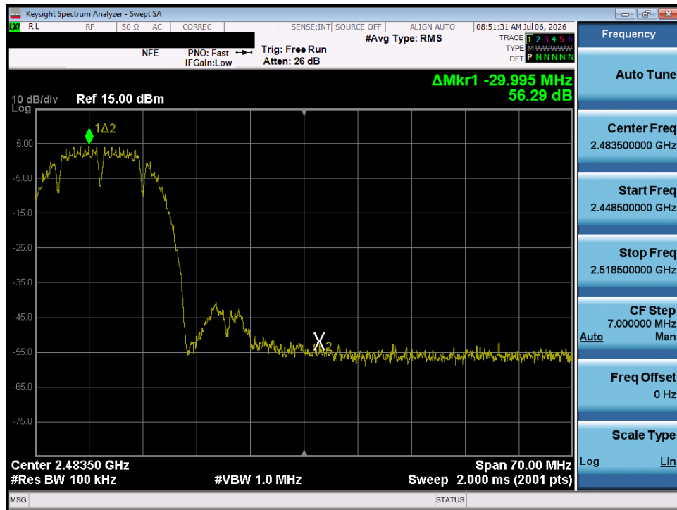
Plot 7-39. Band Edge Plot SISO ANT1 (802.11b – Ch. 10)
