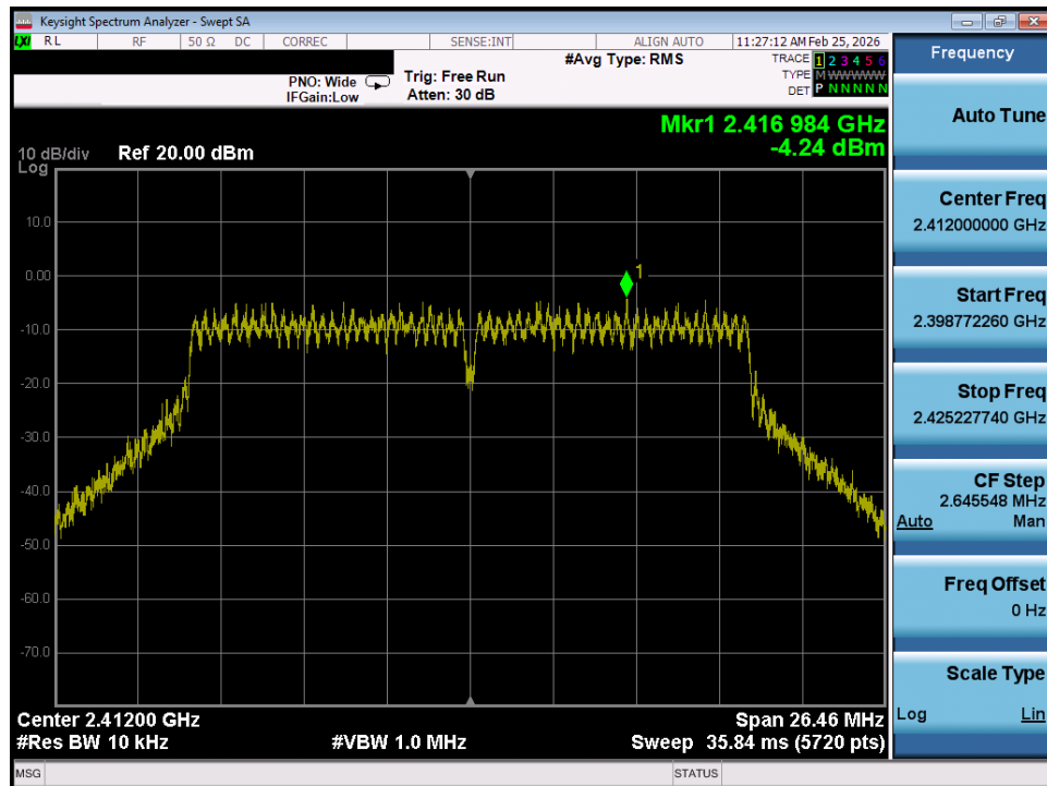
Plot 7-31. Power Spectral Density Plot SISO ANT1 (802.11n/ac (2.4GHz) – Ch. 1)
