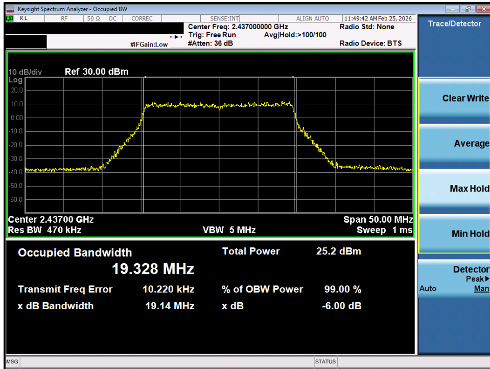
Plot 7-23. OBW Plot SISO ANT1 (802.11ax (2.4GHz) – Ch. 6)
