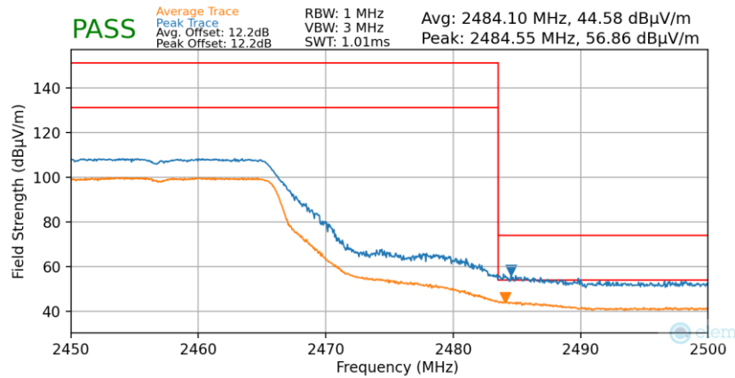
Plot 7-66. Radiated Restricted Upper Band Edge Measurement (Average & Peak)
