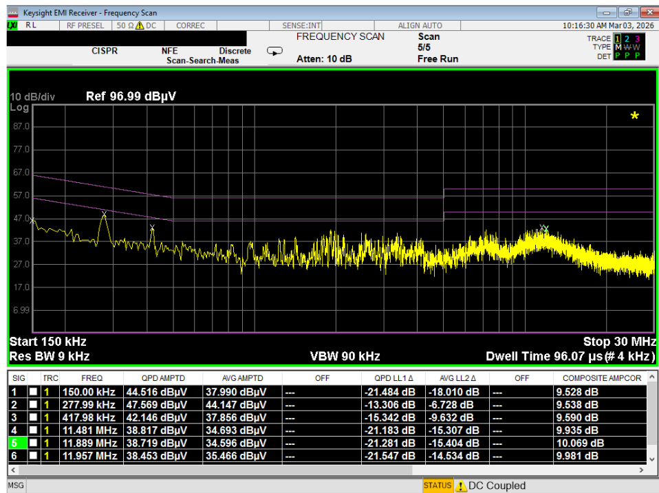
Plot 7-69. Line Conducted Plot with 802.11b (N)
