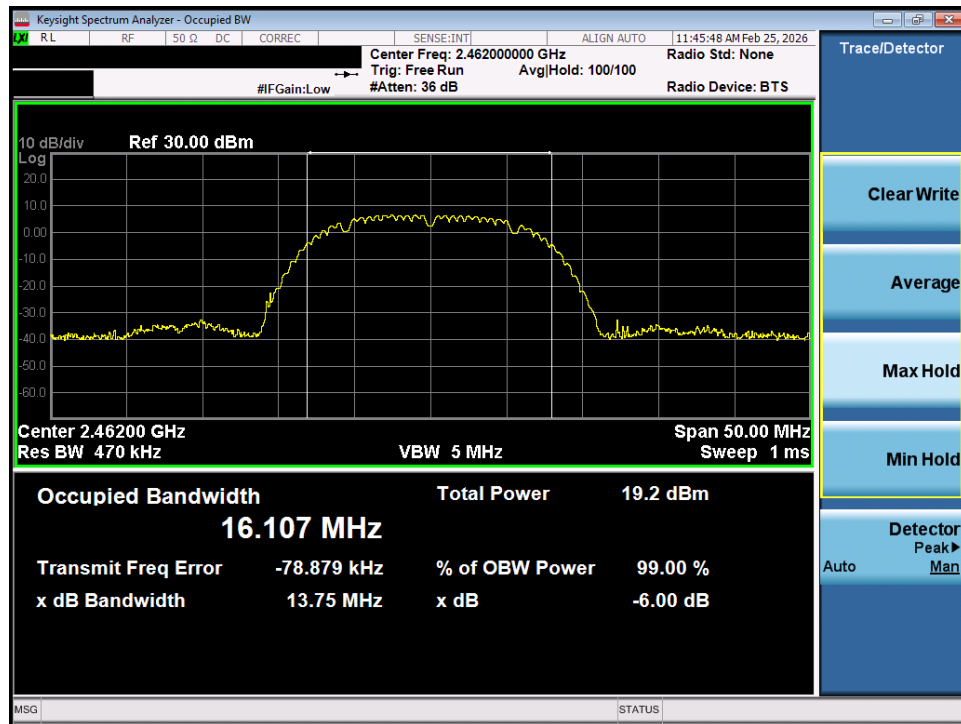
Plot 7-15. OBW Plot SISO ANT1 (802.11b – Ch. 11)
