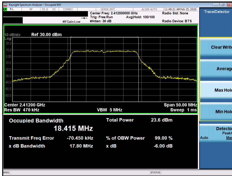
Plot 7-19. OBW Plot SISO ANT1 (802.11n/ac (2.4GHz) – Ch. 1)
