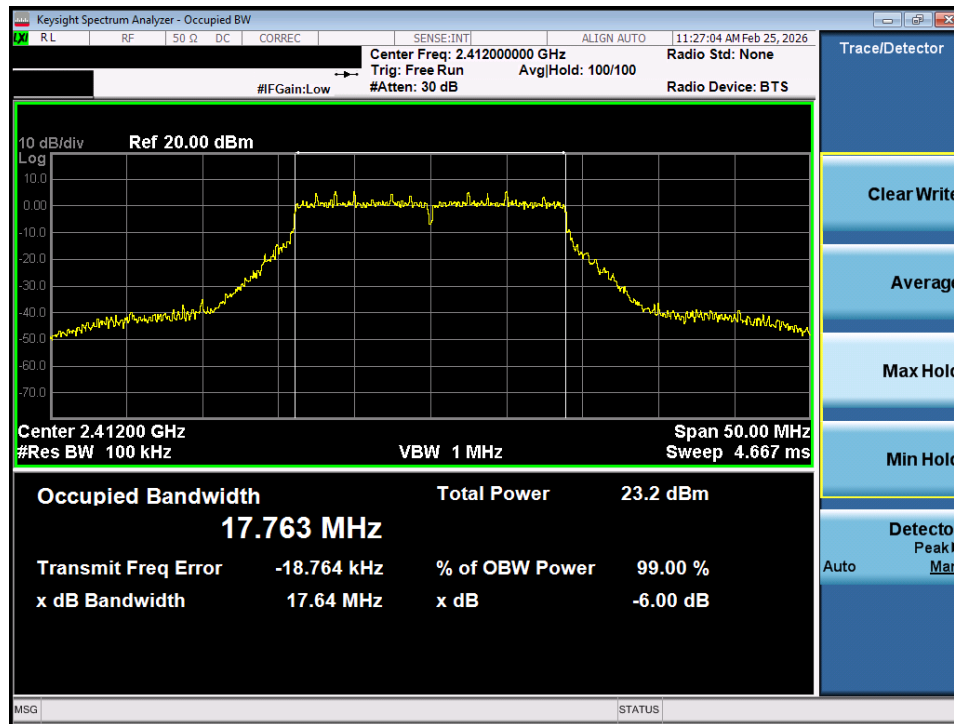
Plot 7-7. 6dB Bandwidth Plot SISO ANT1 (802.11n/ac (2.4GHz) – Ch. 1)
