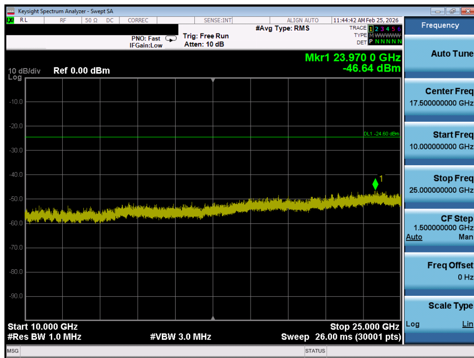
Plot 7-58. Conducted Spurious Plot SISO ANT1 (802.11b – Ch. 11)
