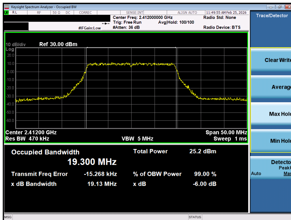
Plot 7-22. OBW Plot SISO ANT1 (802.11ax (2.4GHz) – Ch. 1)
