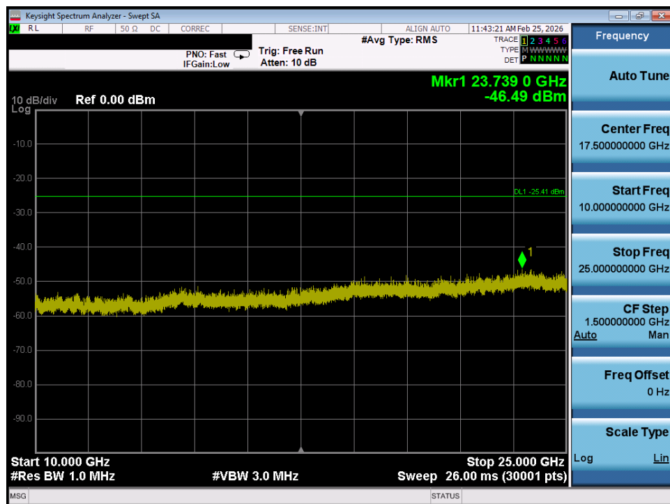
Plot 7-56. Conducted Spurious Plot SISO ANT1 (802.11b – Ch. 6)
