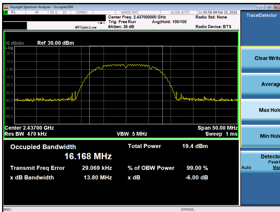
Plot 7-14. OBW Plot SISO ANT1 (802.11b – Ch. 6)
