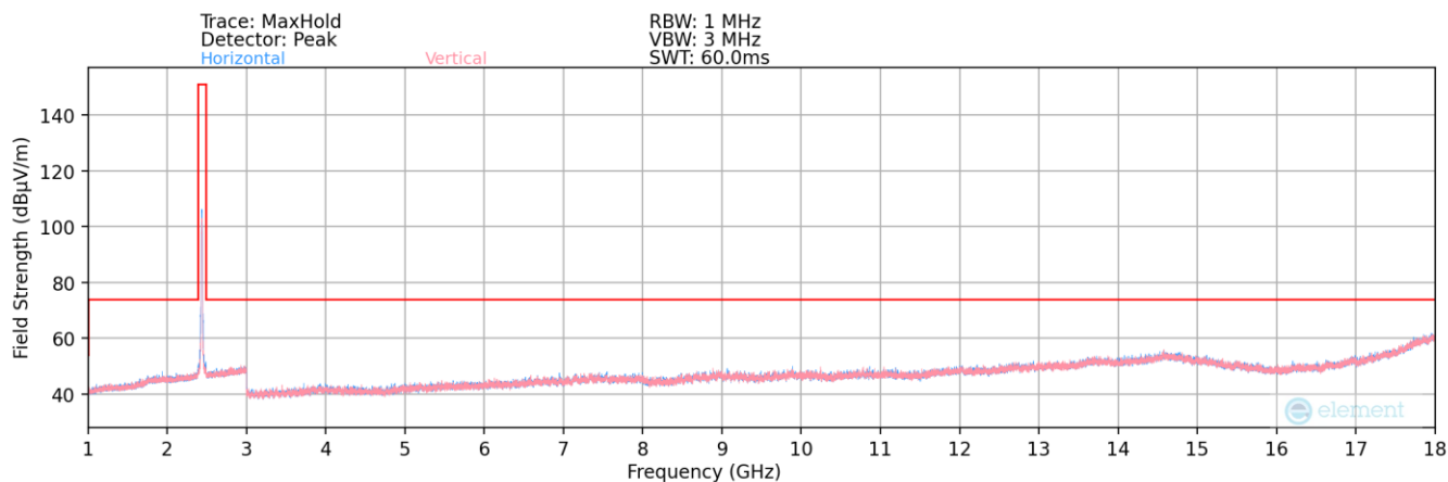
Plot 7-61. Radiated Spurious Plot above 1GHz (802.11b – Ch. 6)
