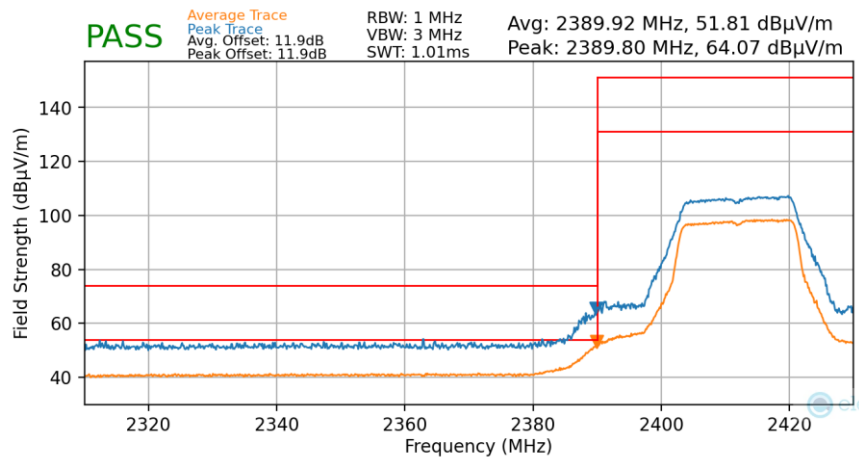
Plot 7-64. Radiated Restricted Lower Band Edge Measurement (Average & Peak)
