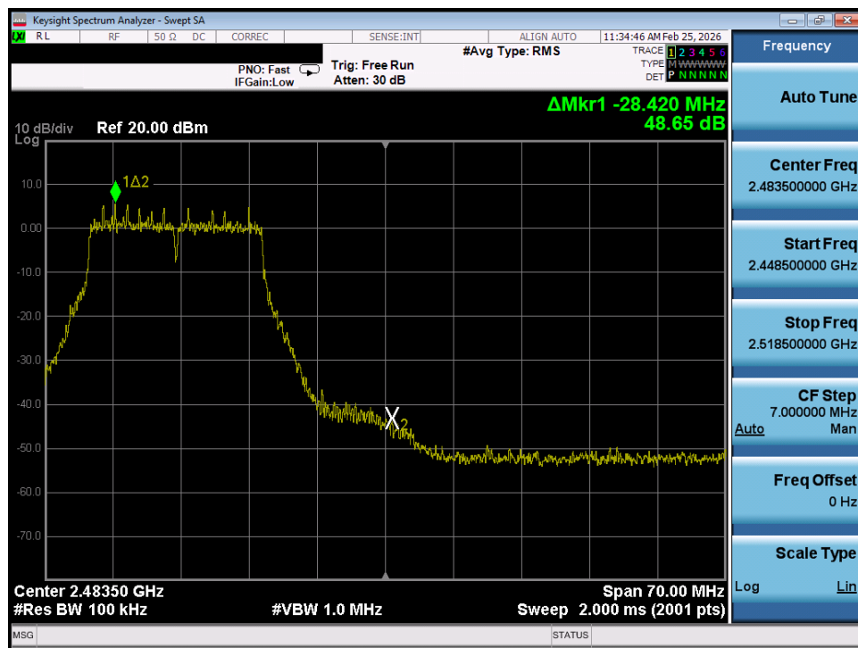
Plot 7-48. Band Edge Plot SISO ANT1 (802.11n/ac – Ch. 11)
