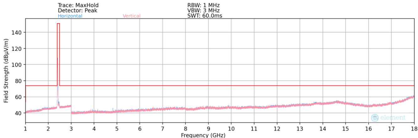
Plot 7-60. Radiated Spurious Plot above 1GHz (802.11b – Ch. 1)
