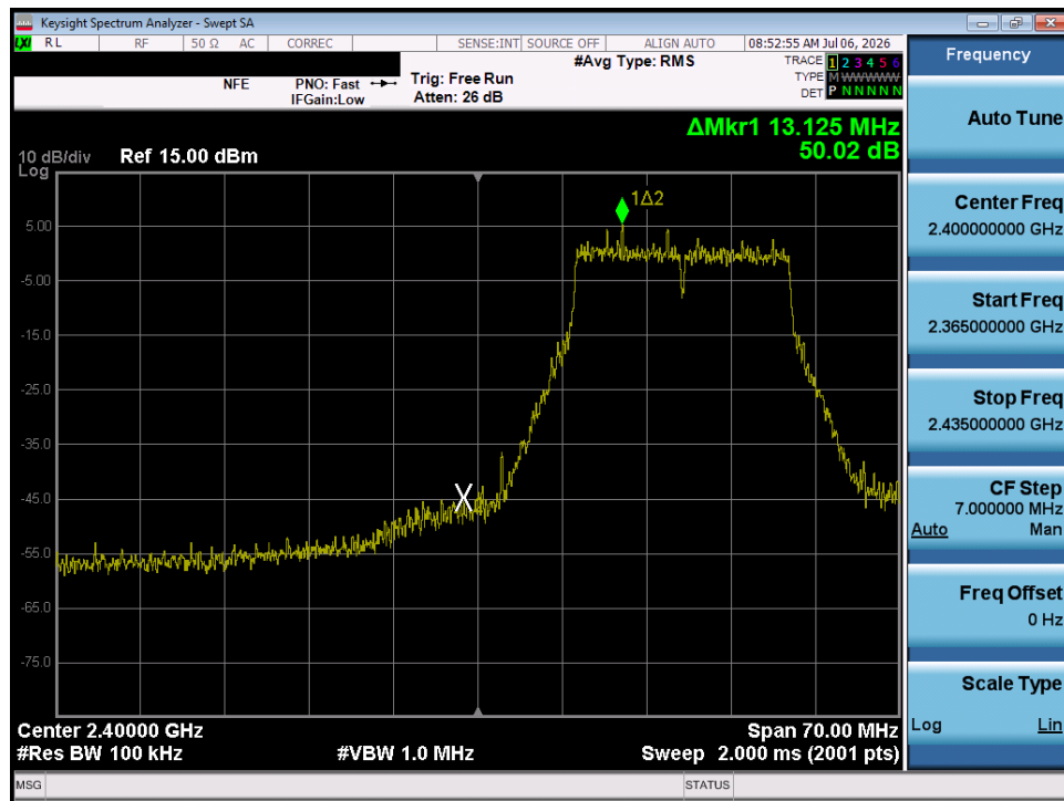
Plot 7-46. Band Edge Plot SISO ANT1 (802.11n/ac – Ch. 2)
