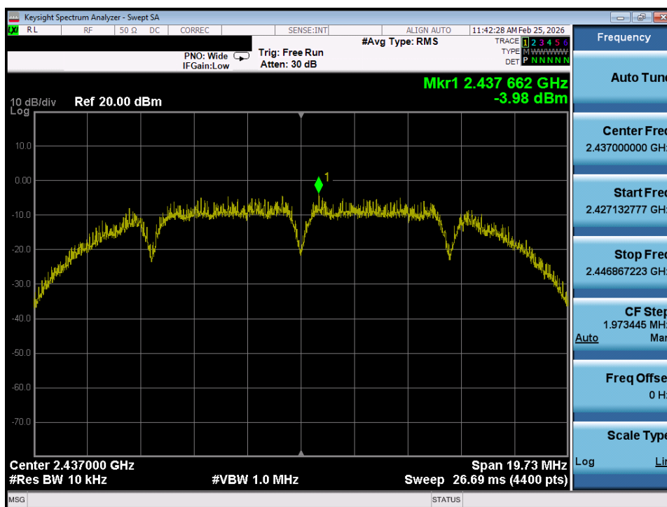
Plot 7-26. Power Spectral Density Plot SISO ANT1 (802.11b – Ch. 6)
