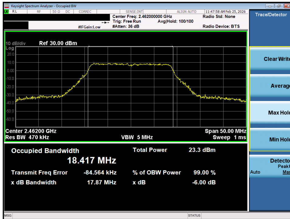
Plot 7-21. OBW Plot SISO ANT1 (802.11n/ac (2.4GHz) – Ch. 11)
