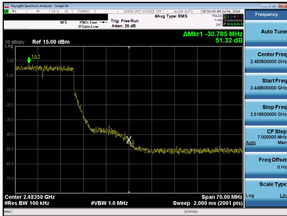
Plot 7-51. Band Edge Plot SISO ANT1 (802.11ax - Ch. 10)
