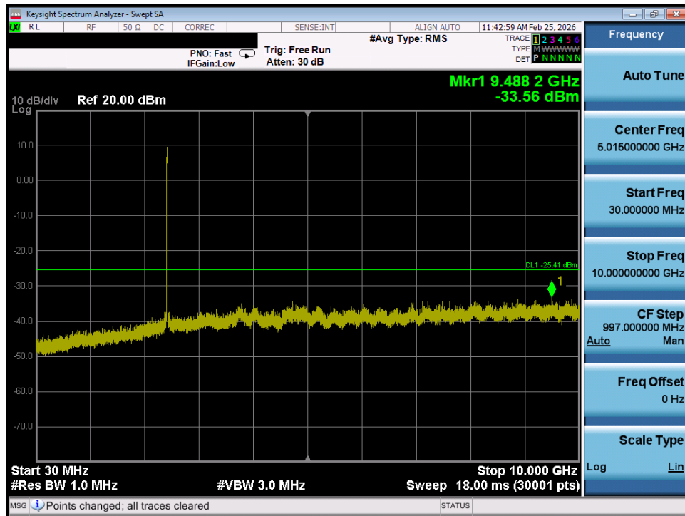
Plot 7-55. Conducted Spurious Plot SISO ANT1 (802.11b – Ch. 6)
