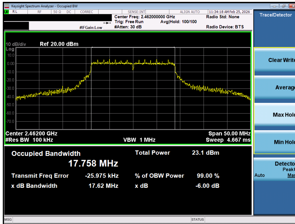
Plot 7-9. 6dB Bandwidth Plot SISO ANT1 (802.11n/ac (2.4GHz) – Ch. 11)
