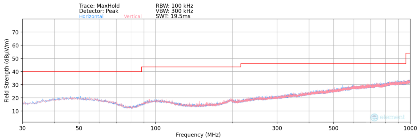
Plot 7-59. Radiated Spurious Plot below 1GHz
