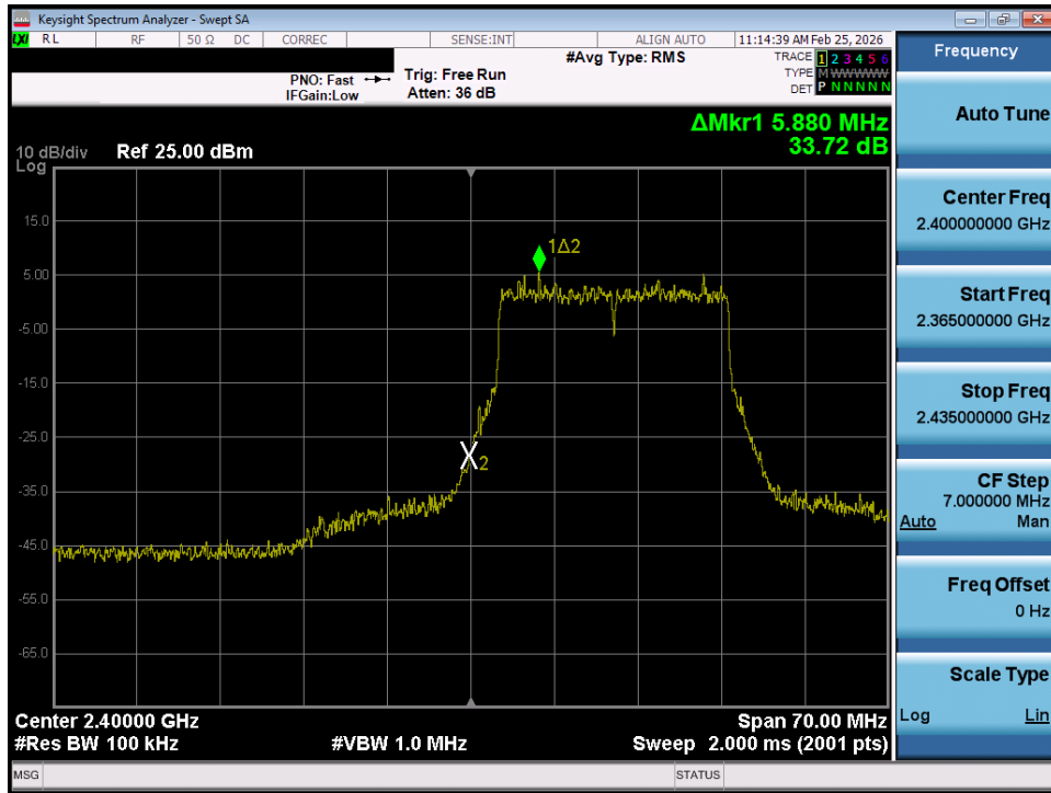
Plot 7-49. Band Edge Plot SISO ANT1 (802.11ax – Ch. 1)
