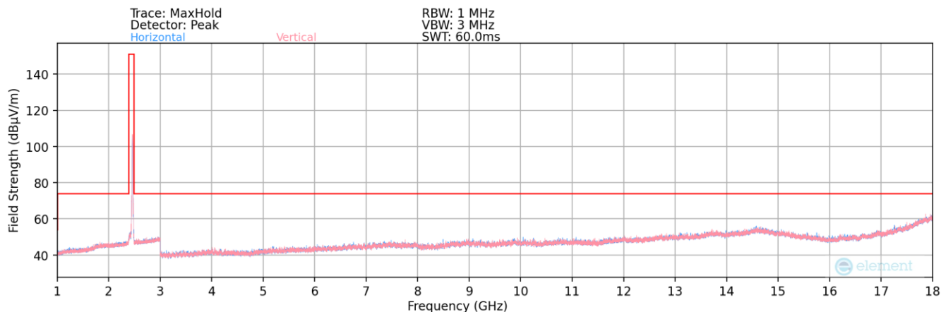
Plot 7-62. Radiated Spurious Plot above 1GHz (802.11b – Ch. 11)
