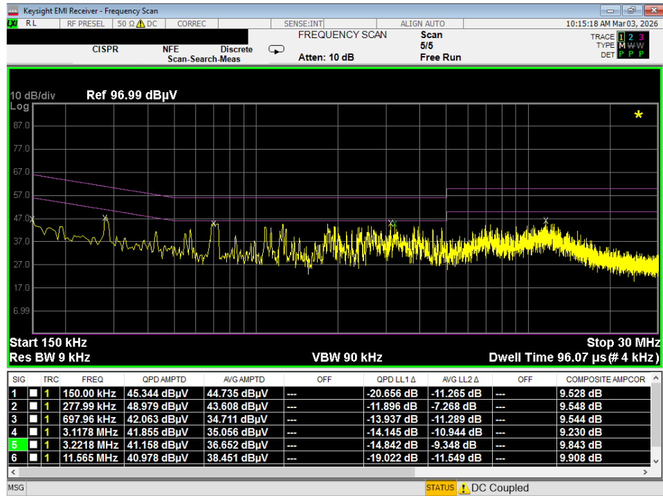
Plot 7-68. Line Conducted Plot with 802.11b (L1)
