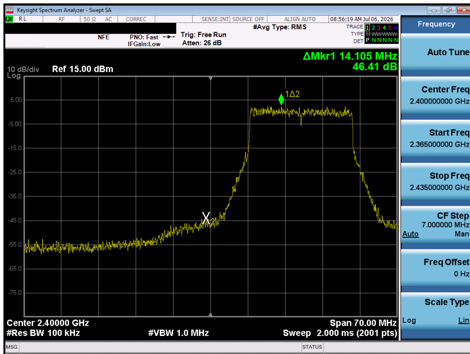
Plot 7-50. Band Edge Plot SISO ANT1 (802.11ax – Ch. 2)
