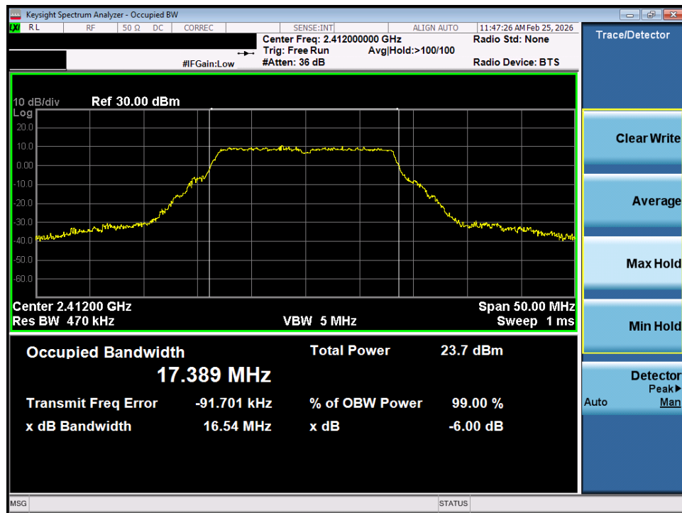
Plot 7-16. OBW Plot SISO ANT1 (802.11g – Ch. 1)
