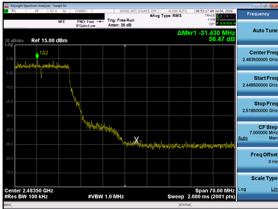
Plot 7-47. Band Edge Plot SISO ANT1 (802.11n/ac – Ch. 10)
