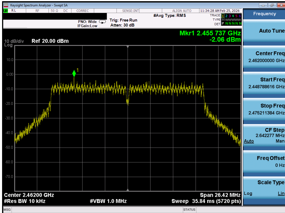
Plot 7-33. Power Spectral Density Plot SISO ANT1 (802.11n/ac (2.4GHz) – Ch. 11)
