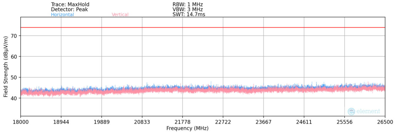
Plot 7-63. Radiated Spurious Plot above 18GHz
