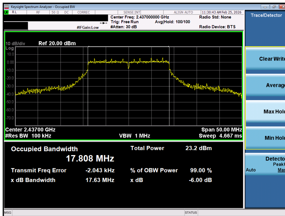
Plot 7-8. 6dB Bandwidth Plot SISO ANT1 (802.11n/ac (2.4GHz) – Ch. 6)
