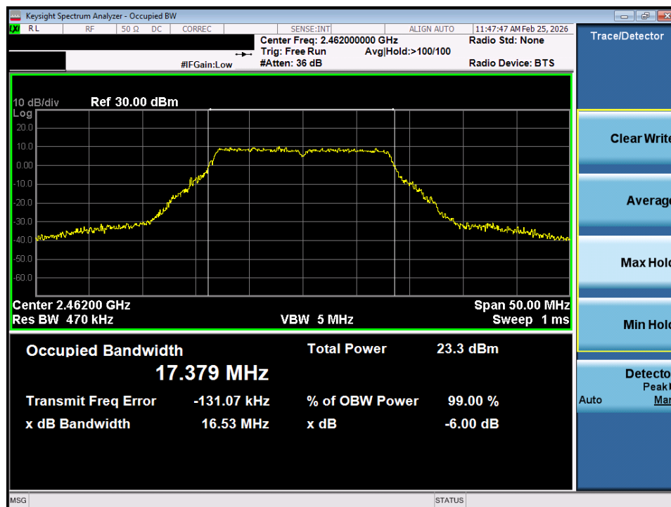
Plot 7-18. OBW Plot SISO ANT1 (802.11g – Ch. 11)
