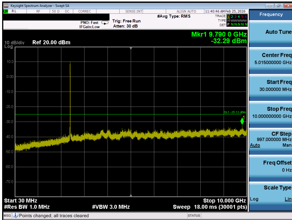
Plot 7-53. Conducted Spurious Plot SISO ANT1 (802.11b – Ch. 1)
