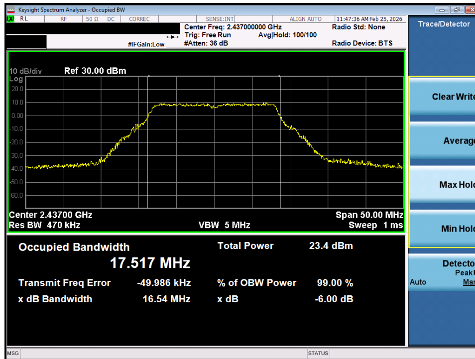
Plot 7-17. OBW Plot SISO ANT1 (802.11g – Ch. 6)
