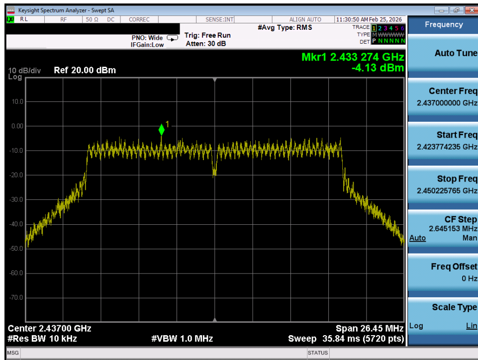
Plot 7-32. Power Spectral Density Plot SISO ANT1 (802.11n/ac (2.4GHz) – Ch. 6)
