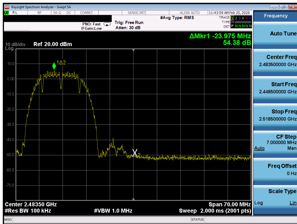
Plot 7-40. Band Edge Plot SISO ANT1 (802.11b – Ch. 11)
