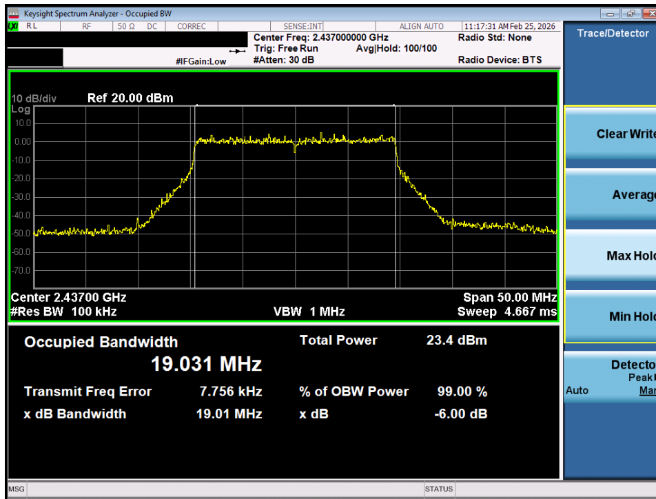
Plot 7-11. 6dB Bandwidth Plot SISO ANT1 (802.11ax (2.4GHz) – Ch. 6)
