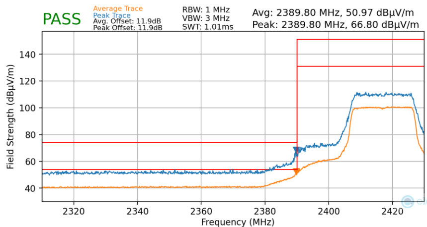
Plot 7-65. Radiated Restricted Lower Band Edge Measurement (Average & Peak)
