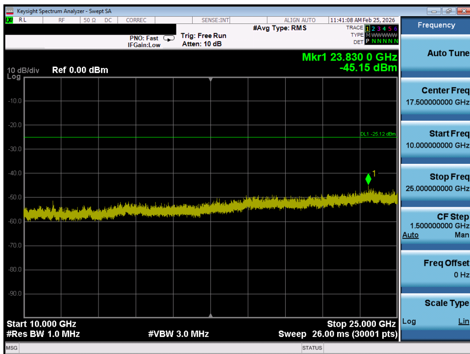
Plot 7-54. Conducted Spurious Plot SISO ANT1 (802.11b – Ch. 1)
