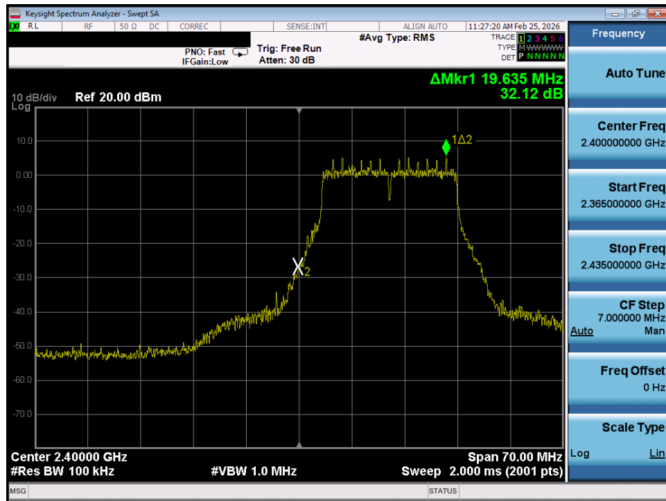
Plot 7-45. Band Edge Plot SISO ANT1 (802.11n/ac – Ch. 1)
