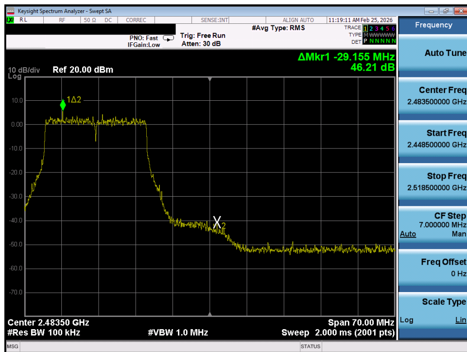
Plot 7-52. Band Edge Plot SISO ANT1 (802.11ax - Ch. 11)
