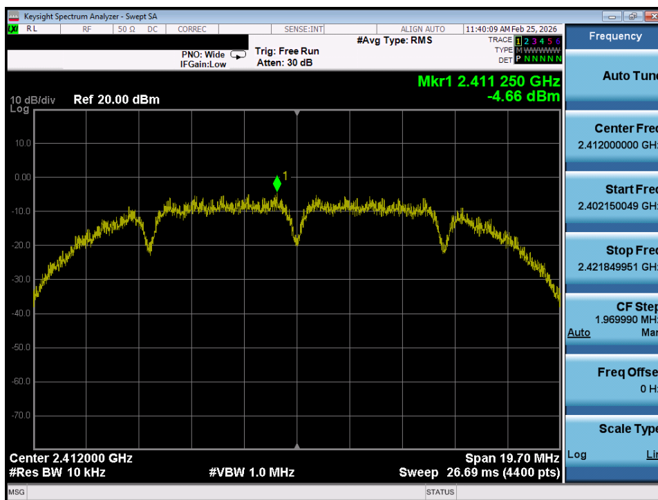
Plot 7-25. Power Spectral Density Plot SISO ANT1 (802.11b – Ch. 1)
