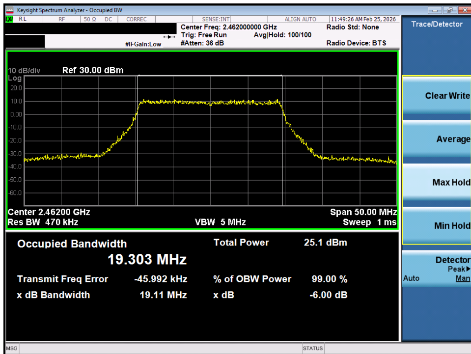
Plot 7-24. OBW Plot SISO ANT1 (802.11ax (2.4GHz) – Ch. 11)
