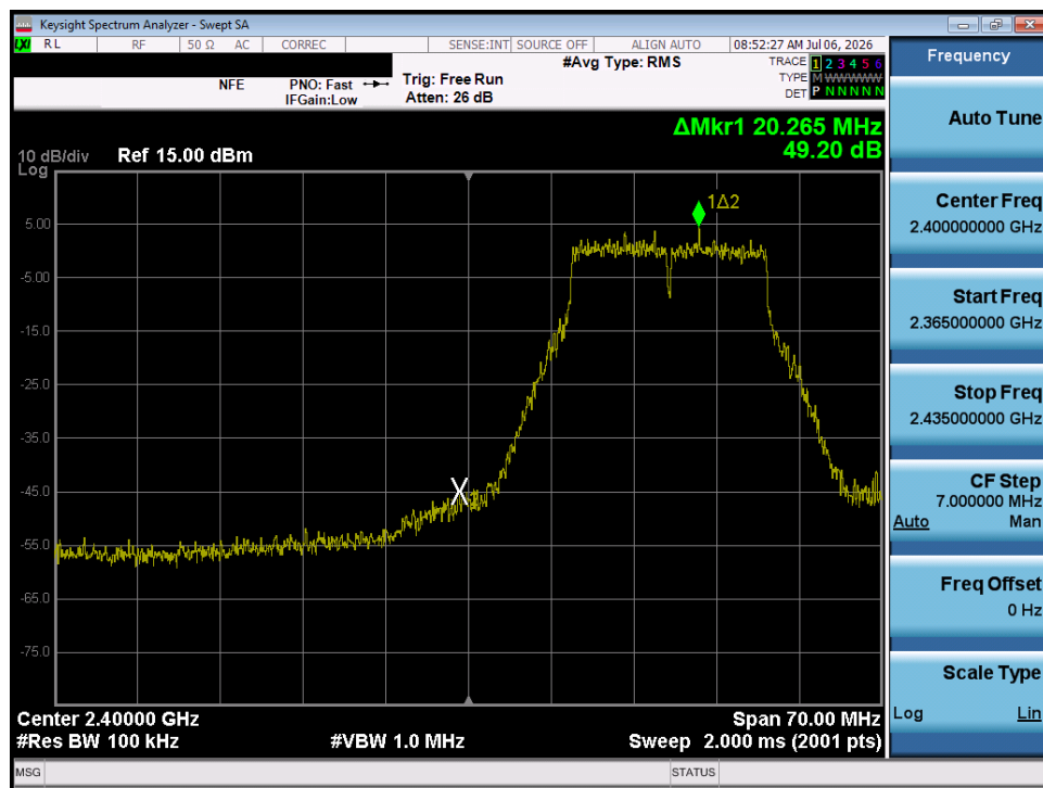
Plot 7-42. Band Edge Plot SISO ANT1 (802.11g - Ch. 2)
