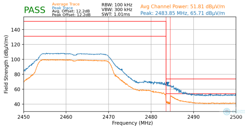
Plot 7-67. Radiated Restricted Upper Band Edge Measurement (Average & Peak)
