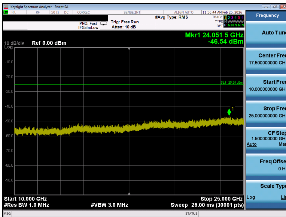
Plot 7-28. Conducted Spurious Plot SISO ANT1 (802.11ax OFDMA – 26 Tones – Ch. 6)
