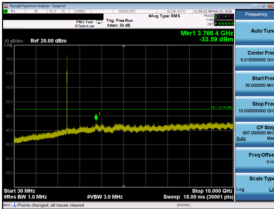
Plot 7-27. Conducted Spurious Plot SISO ANT1 (802.11ax OFDMA – 26 Tones – Ch. 6)
