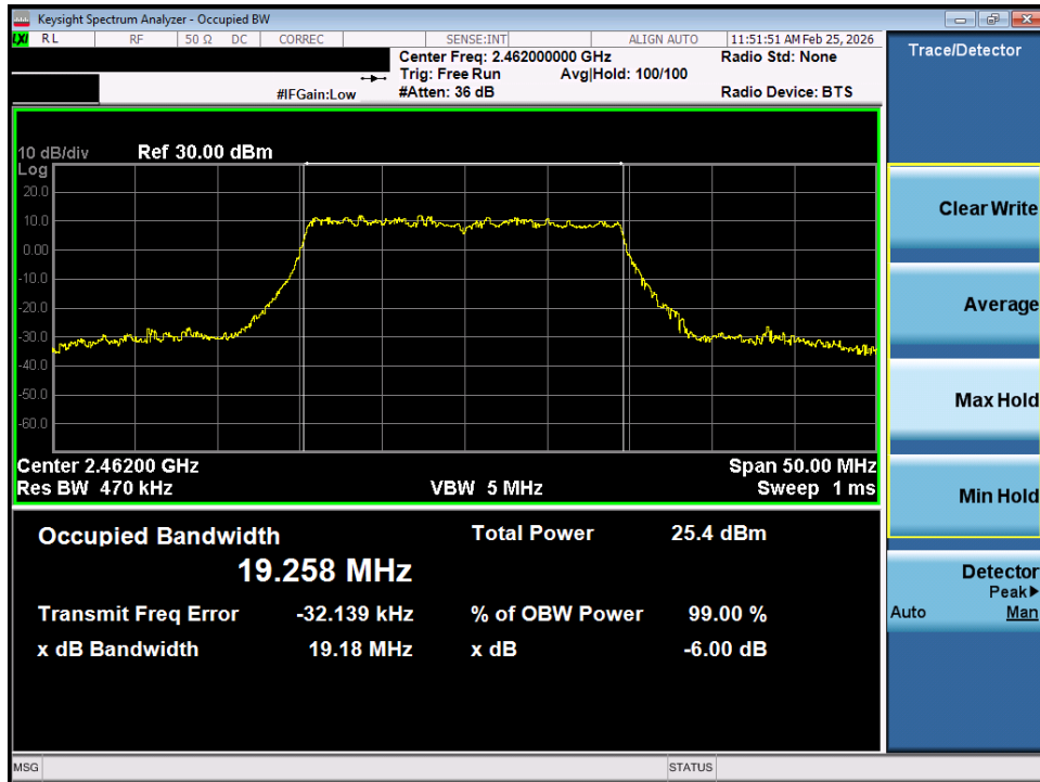
Plot 7-12. OBW Plot SISO ANT1 (802.11ax OFDMA – 242 Tones – Ch. 11)
