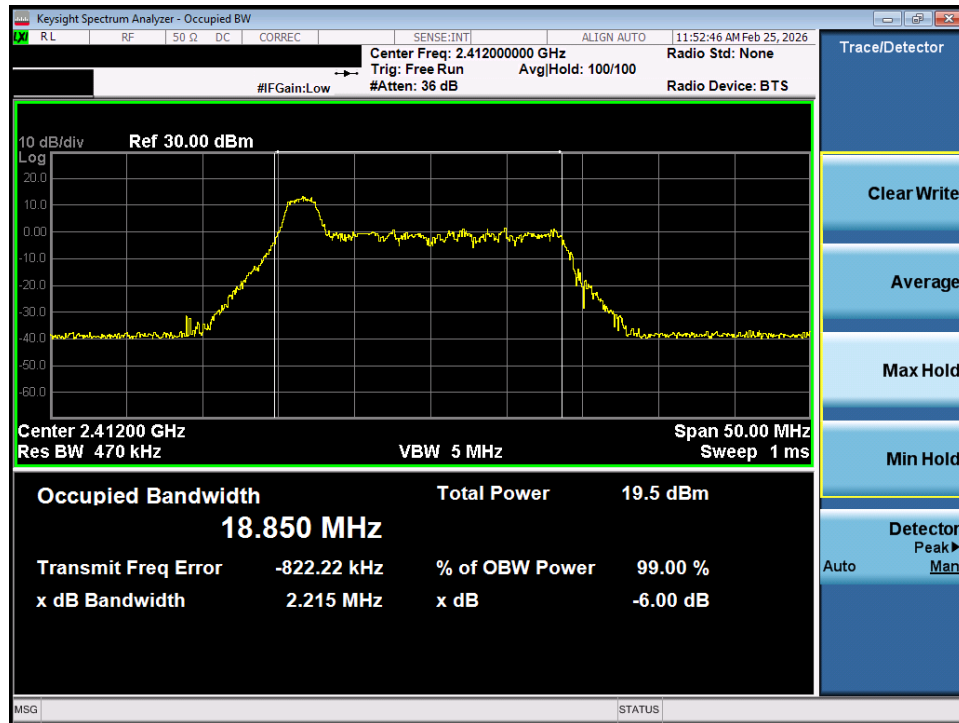
Plot 7-7. OBW Plot SISO ANT1 (802.11ax OFDMA – 26 Tones – Ch. 1)
