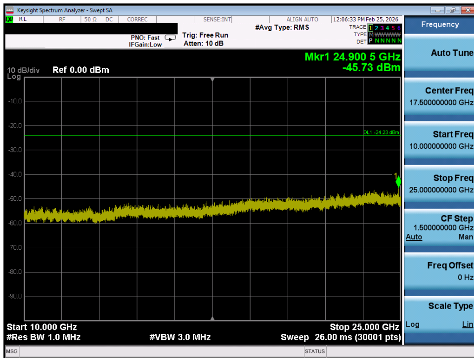
Plot 7-34. Conducted Spurious Plot SISO ANT1 (802.11ax OFDMA – 242 Tones – Ch. 6)
