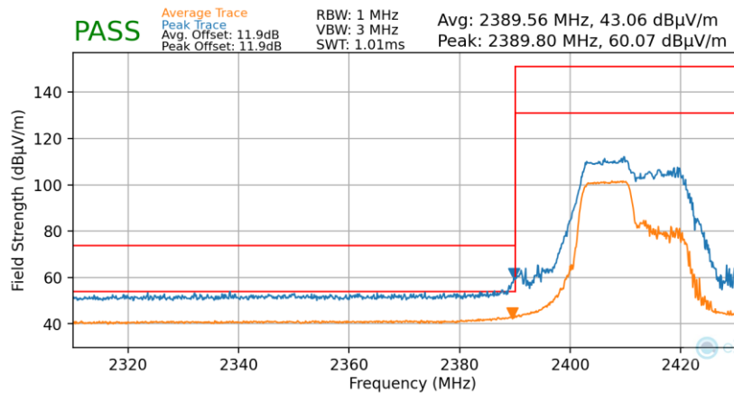
Plot 7-46. Radiated Restricted Lower Band Edge Measurement (Average & Peak – 106 Tones)
