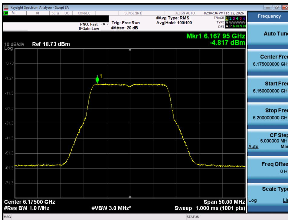
Plot 7-6. Power Spectral Density Plot SISO ANT1 (20MHz 802.11a (UNII Band 5) – Ch. 45) - LPI
