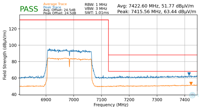
Plot 7-50. Radiated Upper Band Edge Plot SISO (Average & Peak – UNII Band 8)
