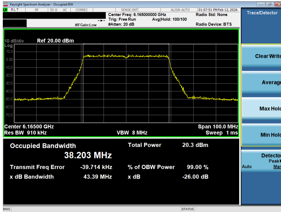
Plot 7-3. 26dB Bandwidth Plot SISO ANT1 (40MHz 802.11ax (UNII Band 5) – Ch. 43) - LPI
