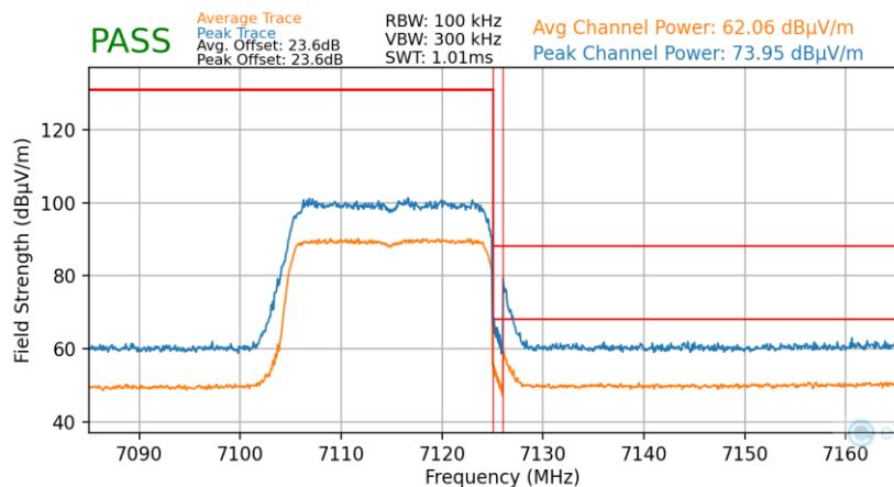
Plot 7-44. Radiated Upper Band Edge Plot SISO (Average & Peak – UNII Band 8)
