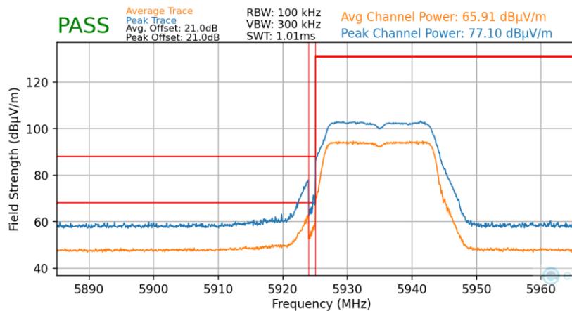
Plot 7-43. Radiated Lower Band Edge Plot SISO (Average & Peak – UNII Band 5)
