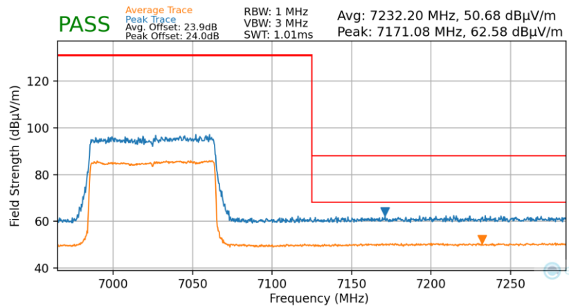
Plot 7-48. Radiated Upper Band Edge Plot SISO (Average & Peak – UNII Band 8)
