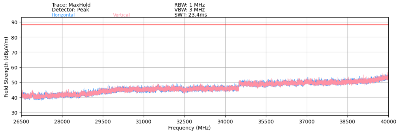
Plot 7-30. Radiated Spurious Plot 26.5GHz - 40GHz (802.11ax)
