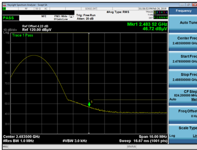
Plot 7-29. Radiated Restricted Upper Band Edge Measurement (Average)
