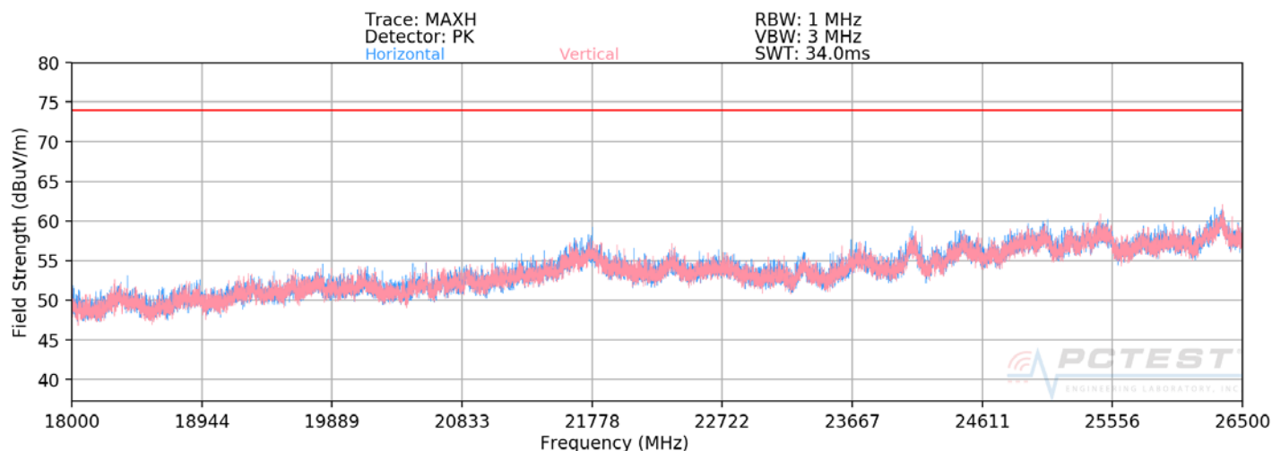
Plot 7-45. Radiated Spurious Plot above 18GHz
