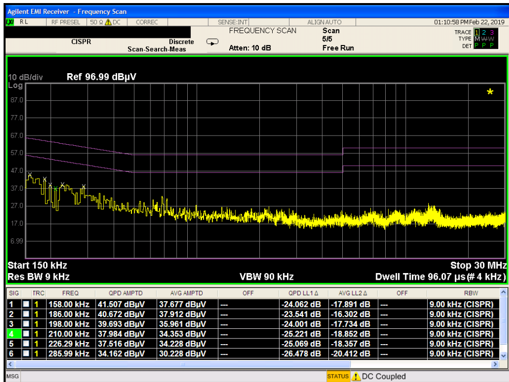
Plot 7-10. Line-Conducted Test Plot with Inductive Coupling Mode #2 (N)
