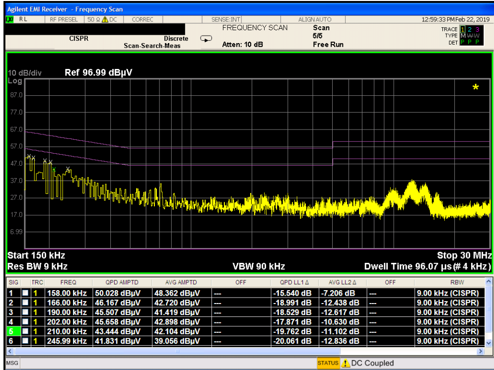
Plot 7-7. Line-Conducted Test Plot with Inductive Coupling Mode #1 (L1)
