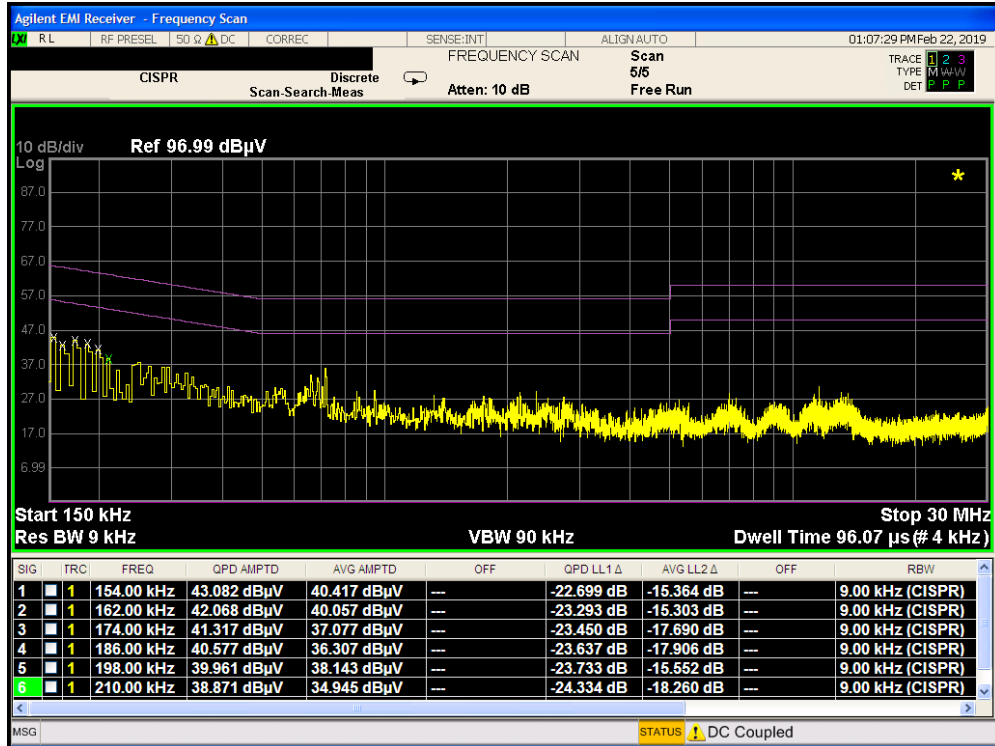
Plot 7-9. Line-Conducted Test Plot with Inductive Coupling Mode #2 (L1)
