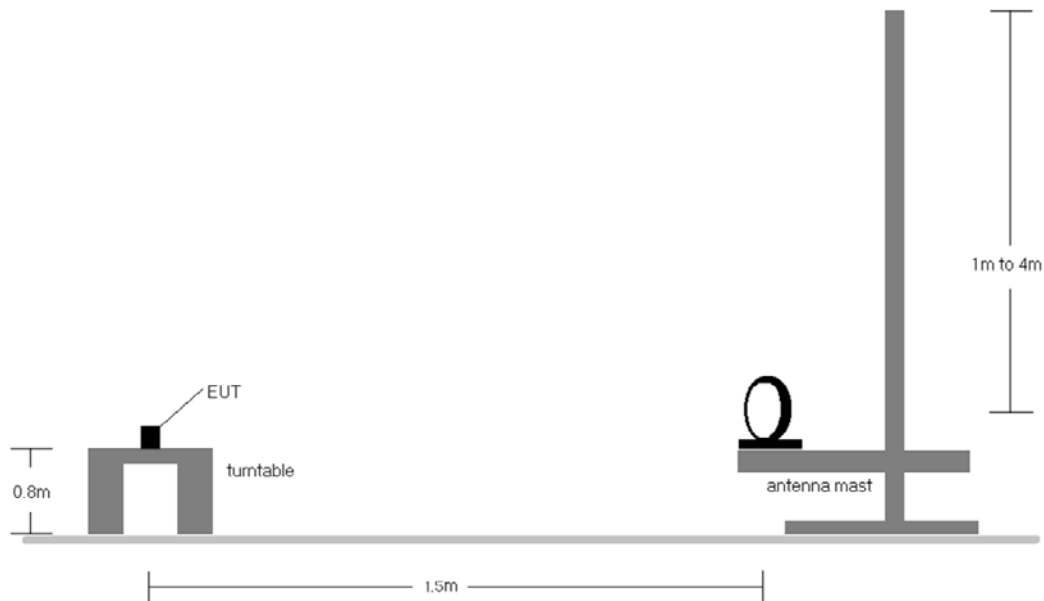
Figure 7-1. Radiated Test Setup
