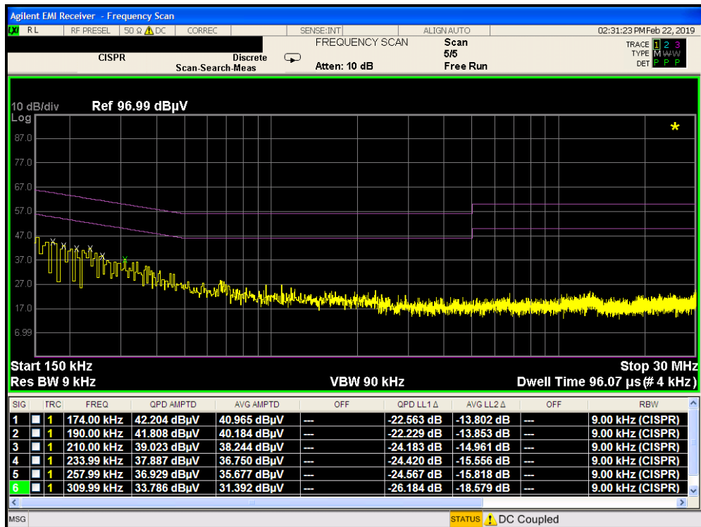
Plot 7-8. Line-Conducted Test Plot with Inductive Coupling Mode #1 (N)
