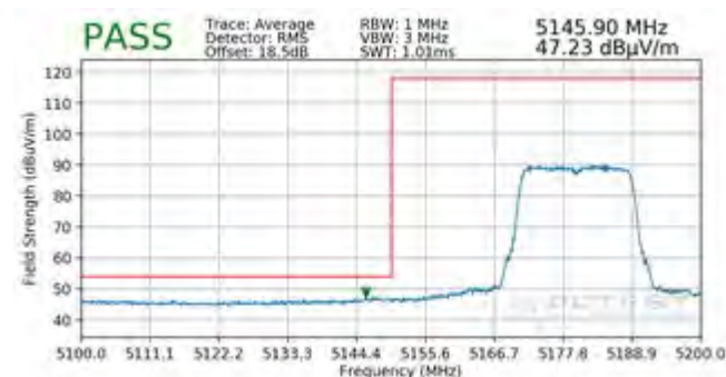
Plot 7-85. Radiated Lower Band Edge Plot SISO ANT1 (Average – UNII Band 1)
