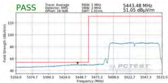
Plot 7-103. Radiated Lower Band Edge Plot – SISO (Average – UNII Band 2C)
