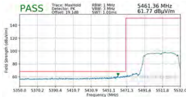
Plot 7-97. Radiated Lower Band Edge Plot SISO ANT1 (Peak – UNII Band 2C)
