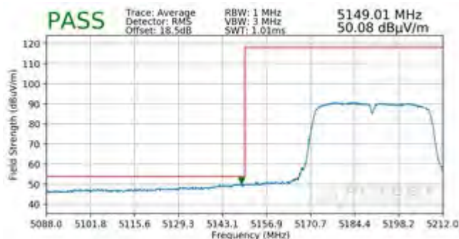
Plot 7-92. Radiated Lower Band Edge Plot SISO ANT1 (Average – UNII Band 1)
