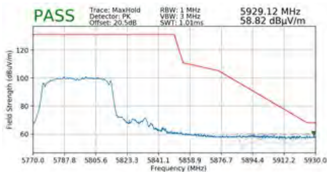
Plot 7-98. Radiated Upper Band Edge Plot SISO ANT1 (Peak – UNII Band 3)
