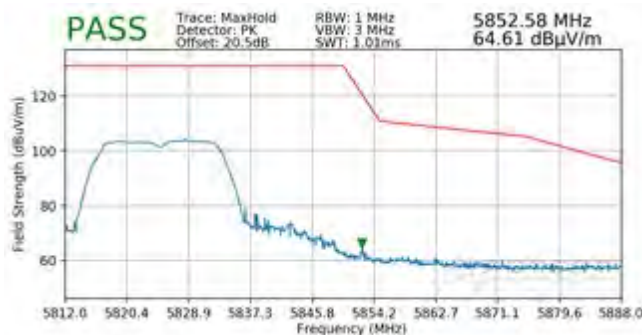
Plot 7-91. Radiated Upper Band Edge Plot SISO ANT1 (Peak – UNII Band 3)
