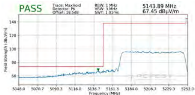
Plot 7-100. Radiated Lower Band Edge Plot – SISO (Peak – UNII Band 1)
