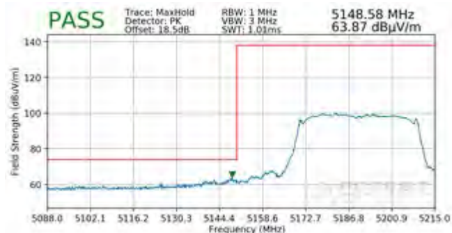
Plot 7-93. Radiated Lower Band Edge Plot SISO ANT1 (Peak – UNII Band 1)
