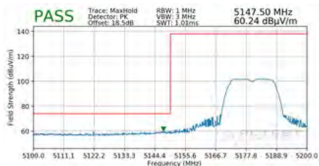
Plot 7-86. Radiated Lower Band Edge Plot SISO ANT1 (Peak – UNII Band 1)
