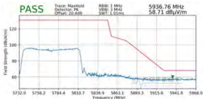
Plot 7-105. Radiated Upper Band Edge Plot MIMO (Peak – UNII Band 3)
