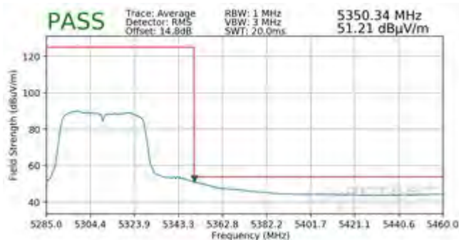
Plot 7-94. Radiated Upper Band Edge Plot SISO ANT1 (Average – UNII Band 2A)
