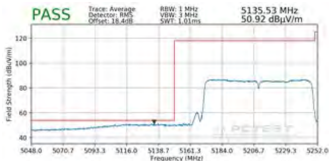
Plot 7-99. Radiated Lower Band Edge Plot – SISO (Average – UNII Band 1)
