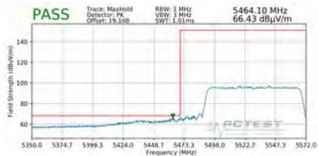
Plot 7-104. Radiated Lower Band Edge Plot - SISO (Peak – UNII Band 2C)
