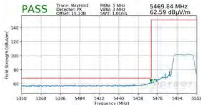
Plot 7-90. Radiated Lower Band Edge Plot SISO ANT1 (Peak – UNII Band 2C)
