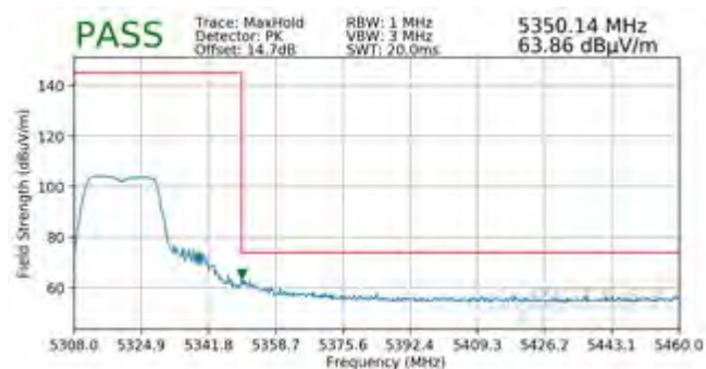
Plot 7-88. Radiated Upper Band Edge Plot SISO ANT1 (Peak – UNII Band 2A)
