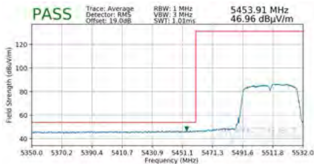
Plot 7-96. Radiated Lower Band Edge Plot SISO ANT1 (Average – UNII Band 2C)
