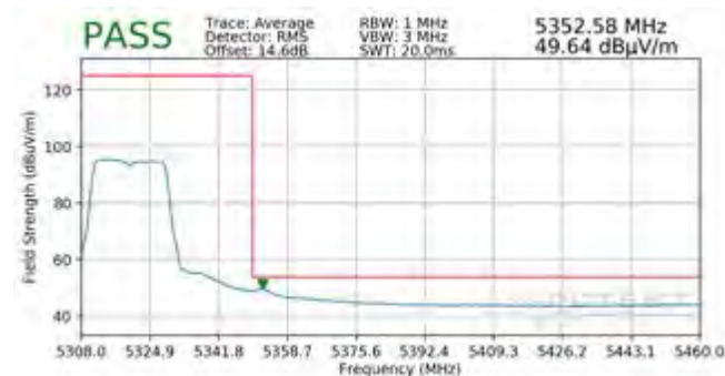
Plot 7-87. Radiated Upper Band Edge Plot SISO ANT1 (Average – UNII Band 2A)
