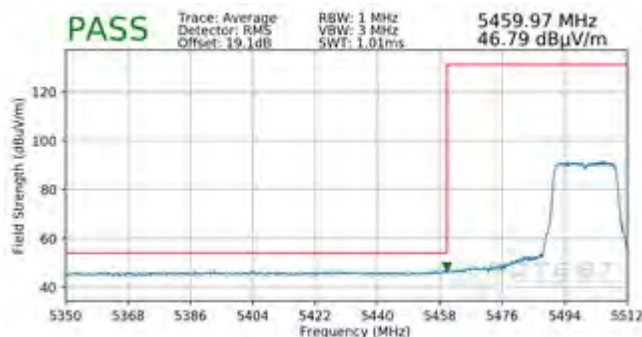
Plot 7-89. Radiated Lower Band Edge Plot SISO ANT1 (Average – UNII Band 2C)
