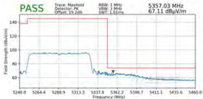
Plot 7-102. Radiated Upper Band Edge Plot – SISO (Peak – UNII Band 2A)
