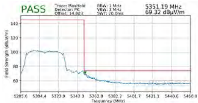
Plot 7-95. Radiated Upper Band Edge Plot SISO ANT1 (Peak – UNII Band 2A)
