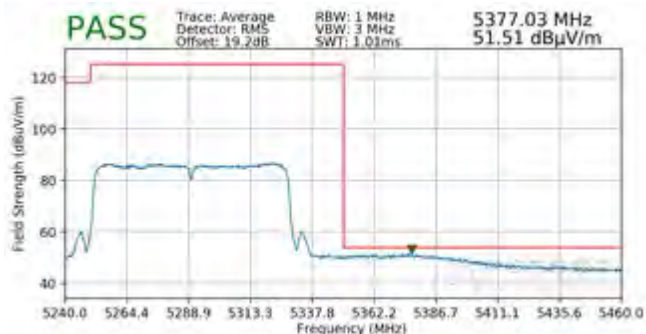
Plot 7-101. Radiated Upper Band Edge Plot - SISO (Average – UNII Band 2A)
