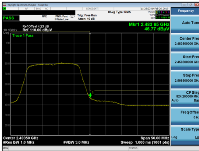
Plot 7-49. Radiated Restricted Upper Band Edge Measurement (Average)
