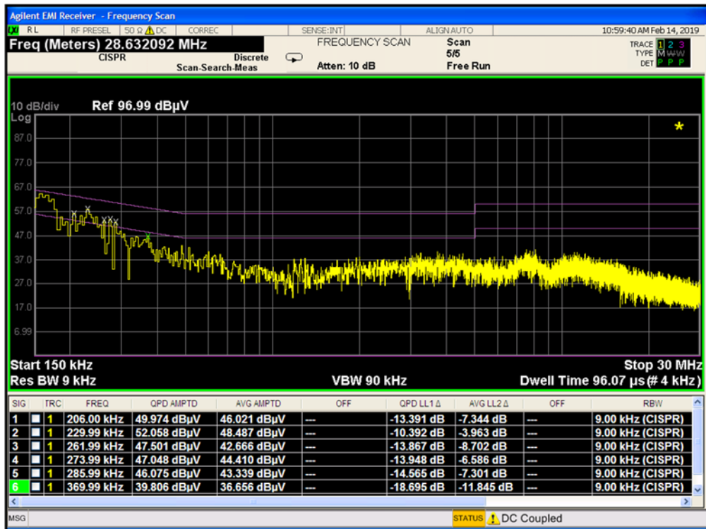
Plot 7-52. Line Conducted Plot with 802.11b (L1)
