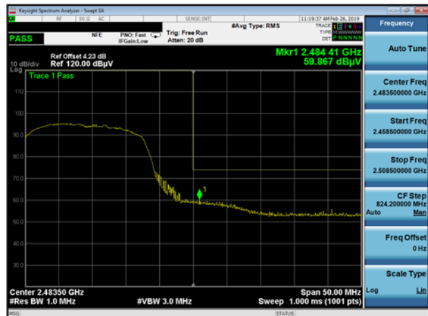
Plot 7-48. Radiated Restricted Upper Band Edge Measurement (Peak)
