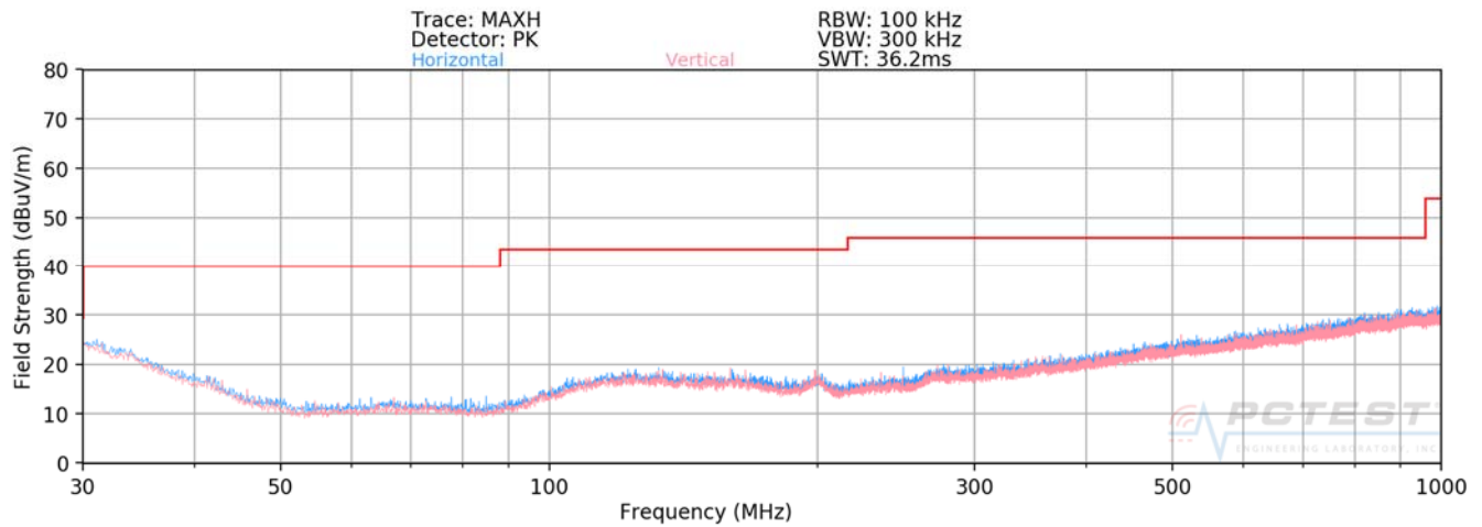
Plot 7-51. Radiated Spurious Plot below 1GHz
