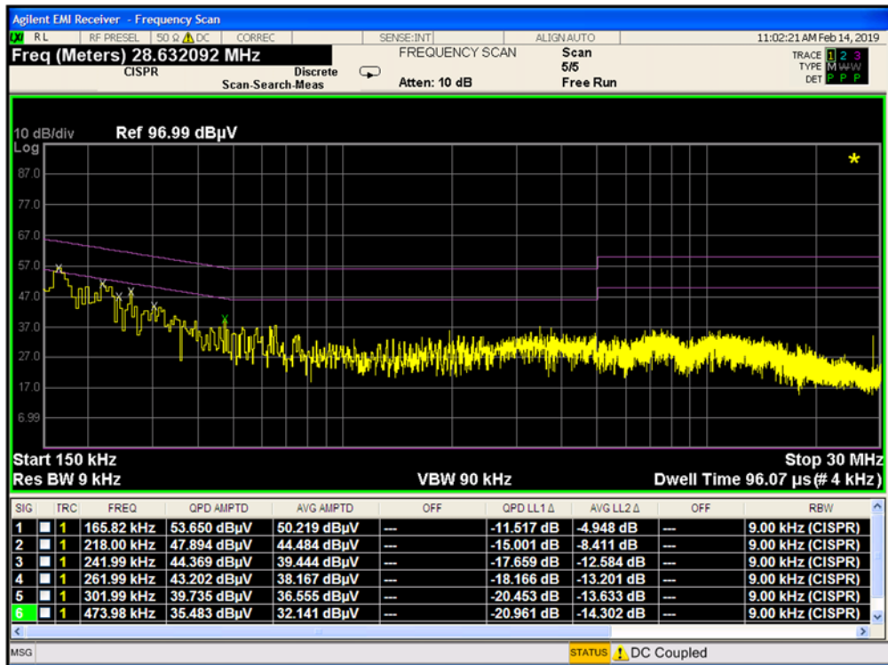
Plot 7-53. Line Conducted Plot with 802.11b (N)
