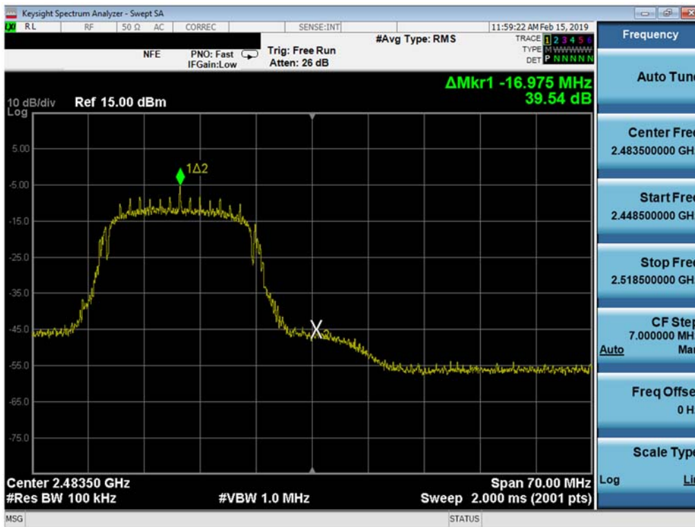
Plot 7-29. Band Edge Plot (802.11n– Ch. 12)
