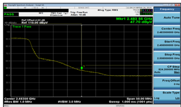
Plot 7-43. Radiated Restricted Upper Band Edge Measurement (Average)
