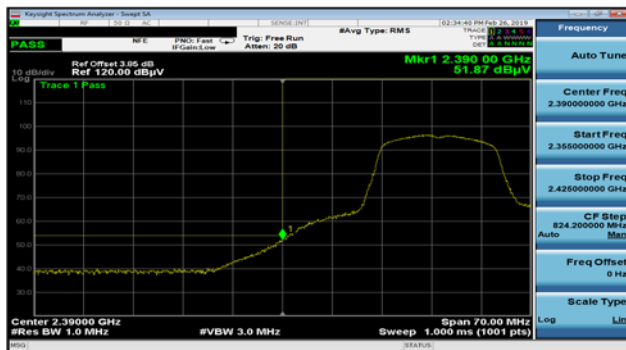
Plot 7-41. Radiated Restricted Lower Band Edge Measurement (Average)
