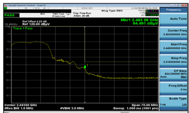
Plot 7-44. Radiated Restricted Upper Band Edge Measurement (Peak)
