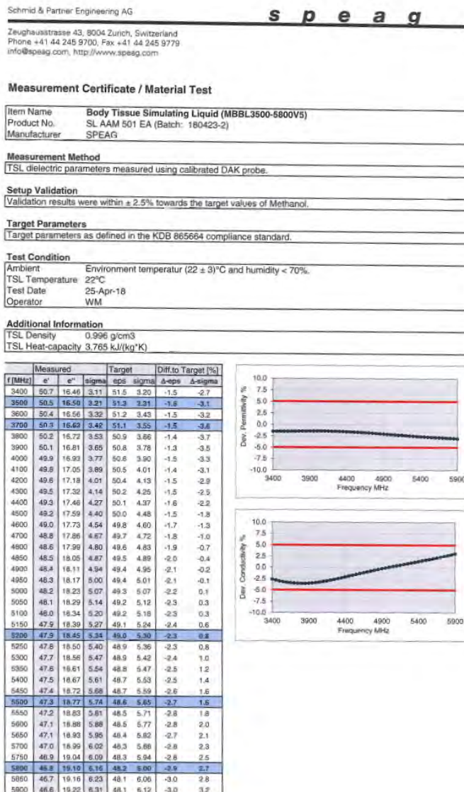
Figure D-7 5 GHz Body Tissue Equivalent Matter
