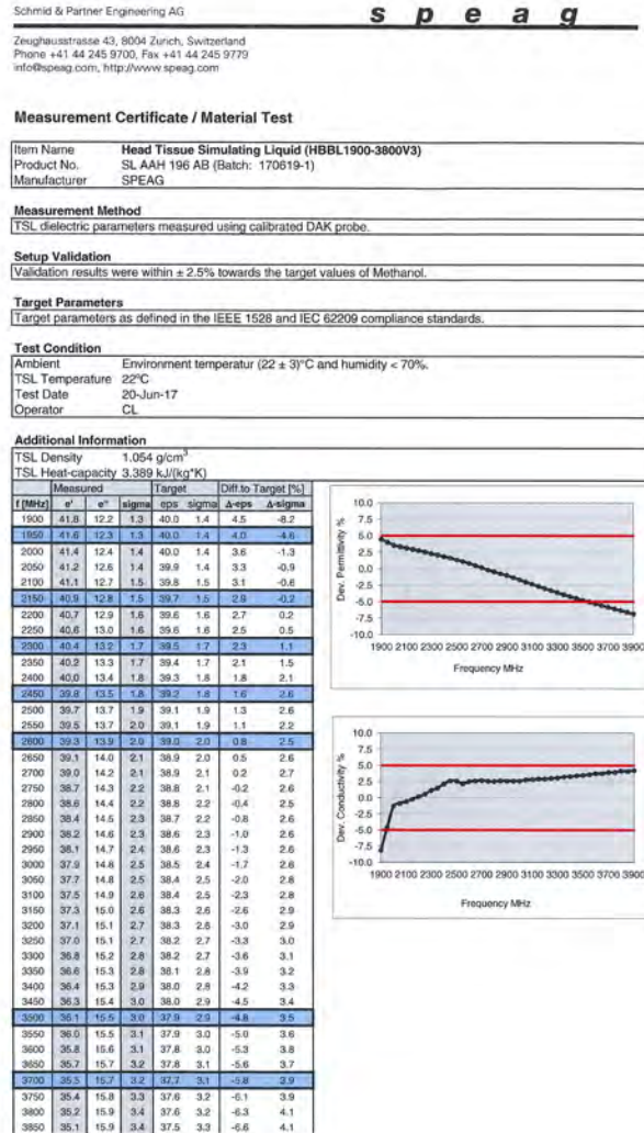
Figure D-4 Composition of 2.4 GHz Head Tissue Equivalent Matter
