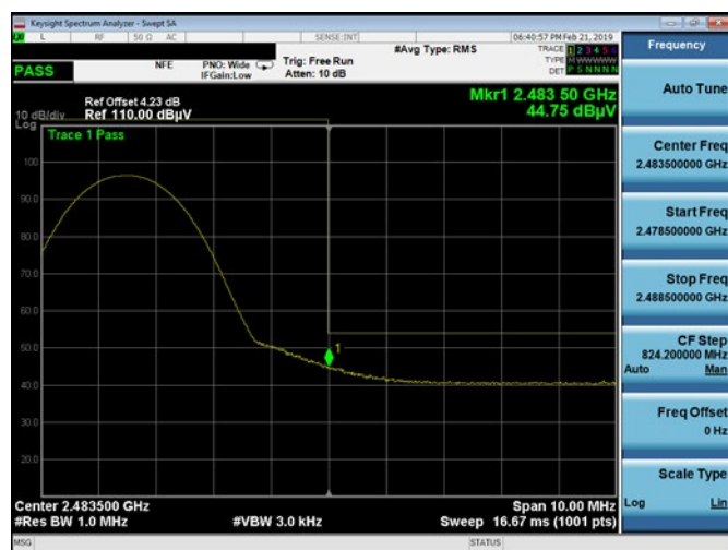
Plot 7-29. Radiated Restricted Upper Band Edge Measurement (Average)
