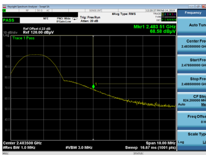
Plot 7-30. Radiated Restricted Upper Band Edge Measurement (Peak)
