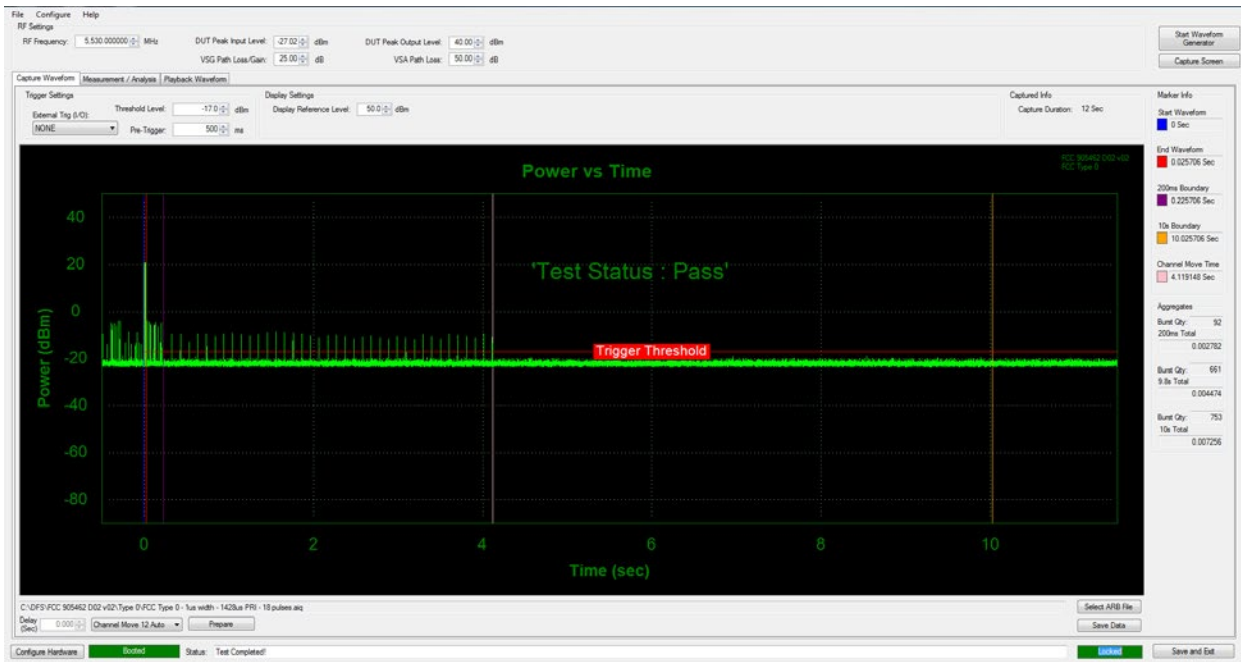
Figure 9-9. 5530MHz - Channel Move/ Closing Transmission Time - (80 MHz)
