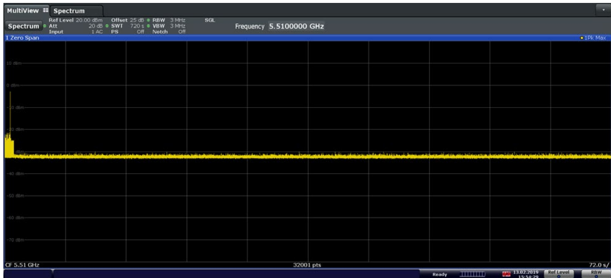
Figure 9-11. 5510MHz - Non-Occupancy Period (10 Minutes) - (40MHz)
