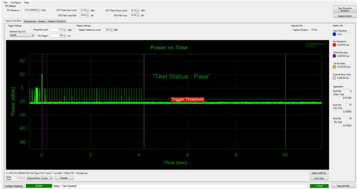
Figure 9-8. 5510MHz - Channel Move/ Closing Transmission Time - (40 MHz)
