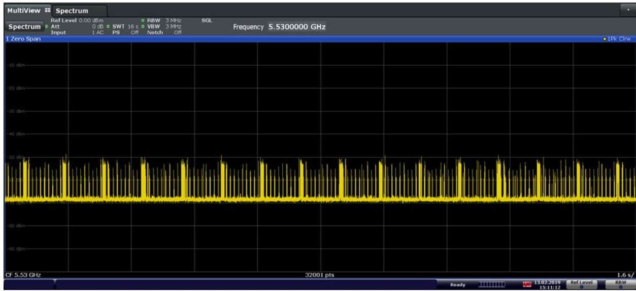
Figure 9-5. 5530MHz - Channel Loading - (80MHz)
