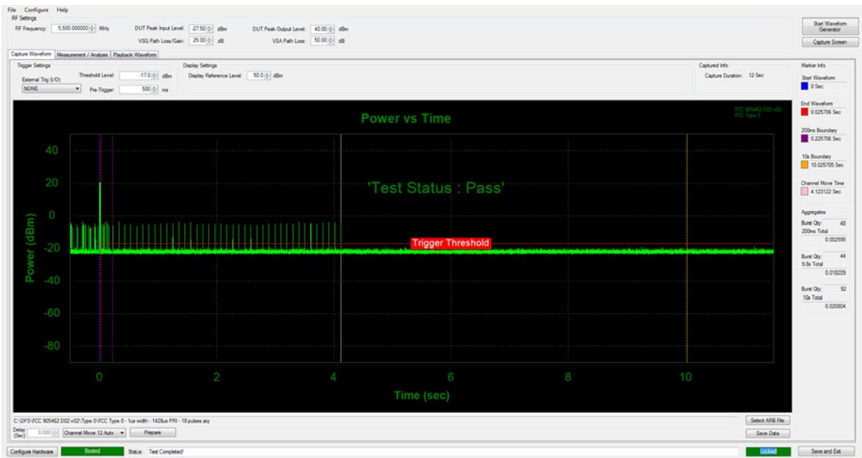
Figure 9-7. 5500MHz - Channel Move/ Closing Transmission Time - (20 MHz)
