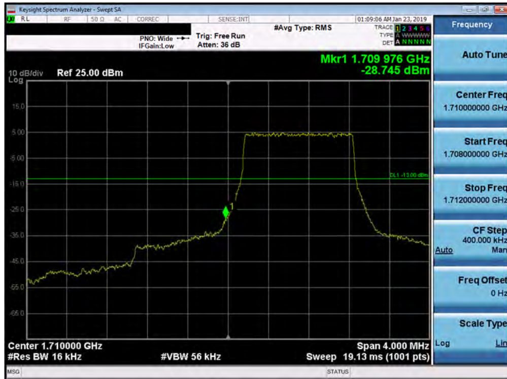
Plot 7-112. Lower Band Edge Plot (Band 66/4 - 1.4MHz QPSK - Full RB Configuration)
