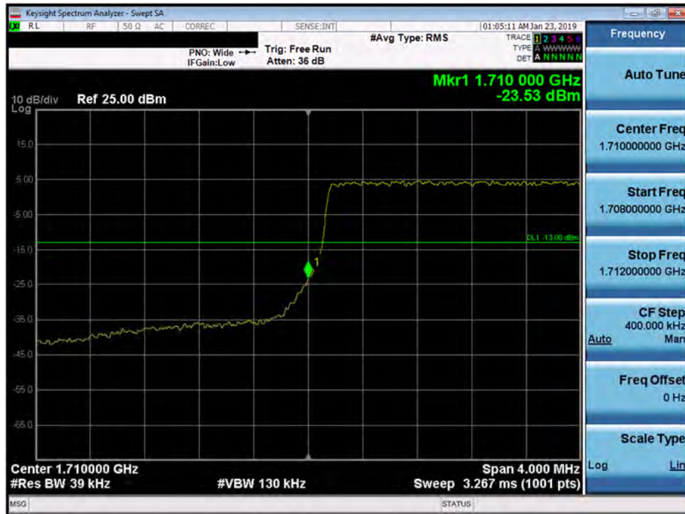
Plot 7-118. Lower Band Edge Plot (Band 66/4 - 3.0MHz QPSK - Full RB Configuration)
