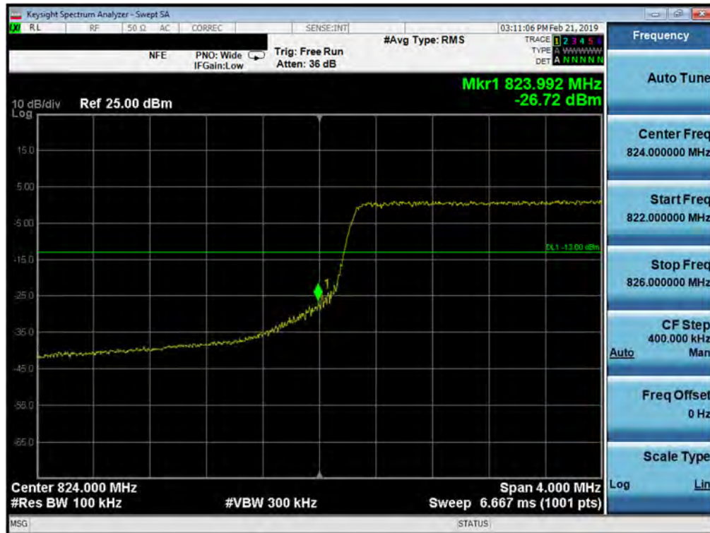
Plot 7-108. Lower Band Edge Plot (Band 5 - 5.0MHz QPSK - Full RB Configuration)
