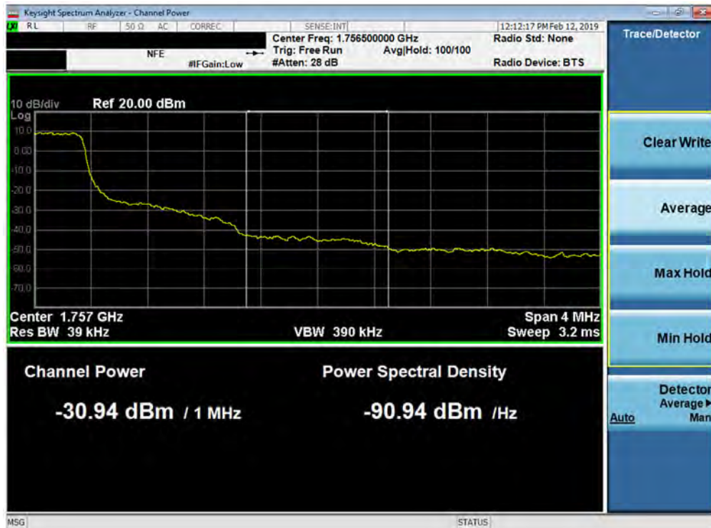
Plot 7-115. Upper Extended Band Edge Plot (Band 4 - 1.4MHz QPSK - Full RB Configuration)
