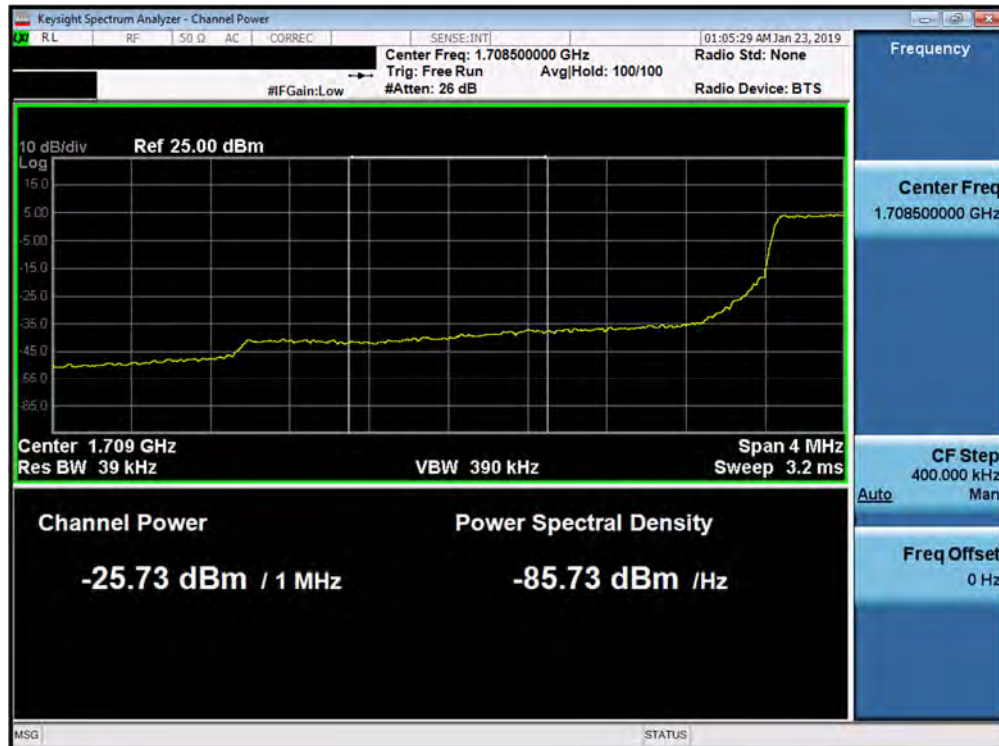
Plot 7-119. Lower Extended Band Edge Plot (Band 66/4 - 3.0MHz QPSK - Full RB Configuration)
