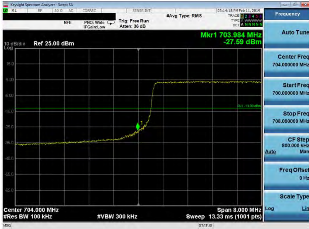
Plot 7-102. Lower Band Edge Plot (Band 17 - 10.0MHz QPSK - Full RB Configuration)
