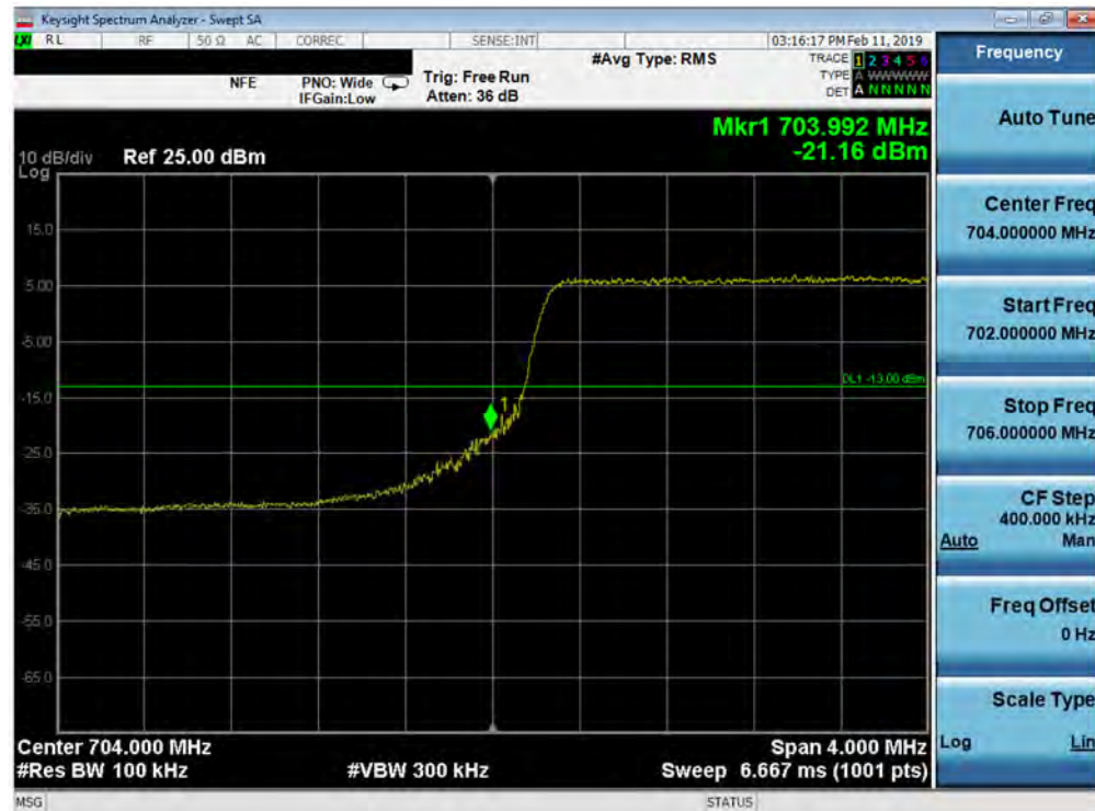
Plot 7-99. Lower Band Edge Plot (Band 17 - 5.0MHz QPSK - Full RB Configuration)
