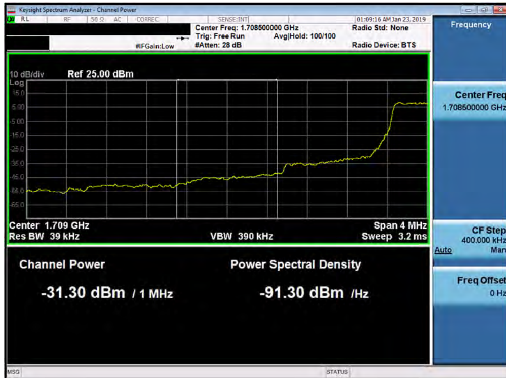
Plot 7-113. Lower Extended Band Edge Plot (Band 66/4 - 1.4MHz QPSK - Full RB Configuration)
