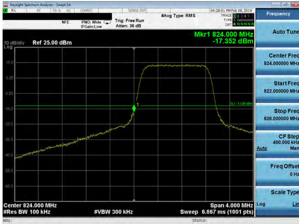
Plot 7-104. Lower Band Edge Plot (Band 5 - 1.4MHz QPSK - Full RB Configuration)
