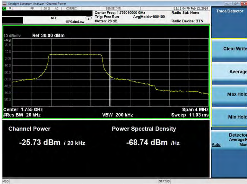
Plot 7-114. Upper Band Edge Plot (Band 4 - 1.4MHz QPSK - Full RB Configuration)
