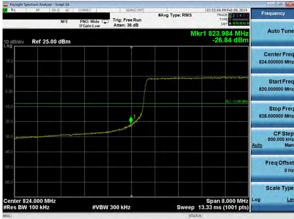
Plot 7-110. Lower Band Edge Plot (Band 5 - 10.0MHz QPSK - Full RB Configuration)
