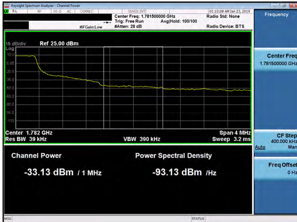
Plot 7-117. Upper Extended Band Edge Plot (Band 66 - 1.4MHz QPSK - Full RB Configuration)
