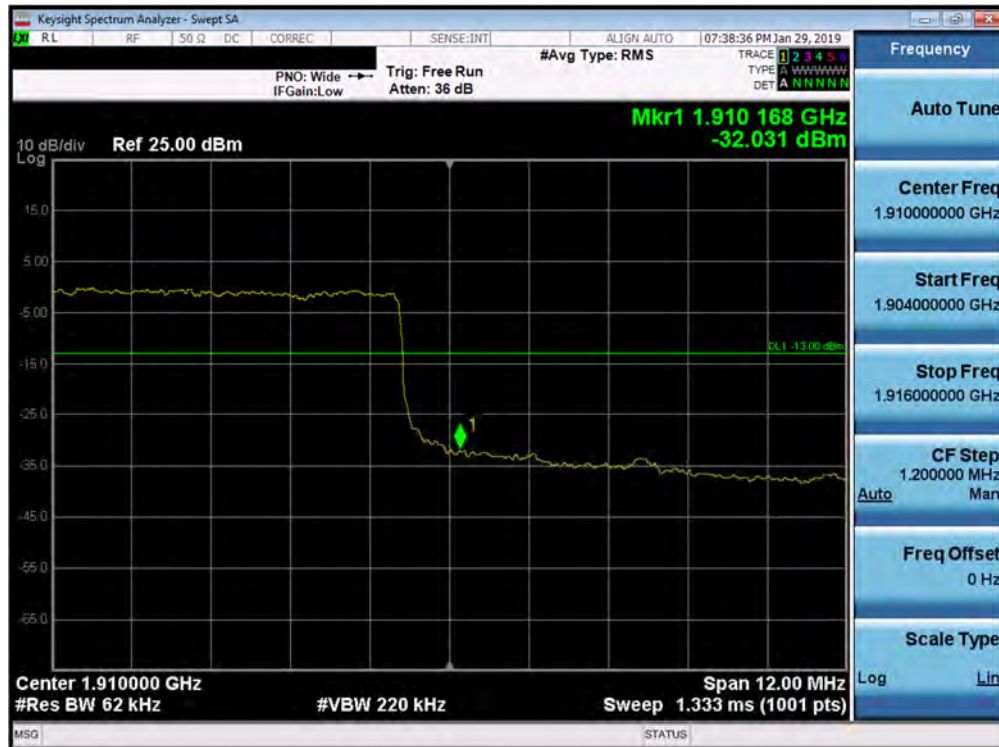
Plot 7-166. Upper Band Edge Plot (Band 2 - 15.0MHz QPSK - Full RB Configuration)
