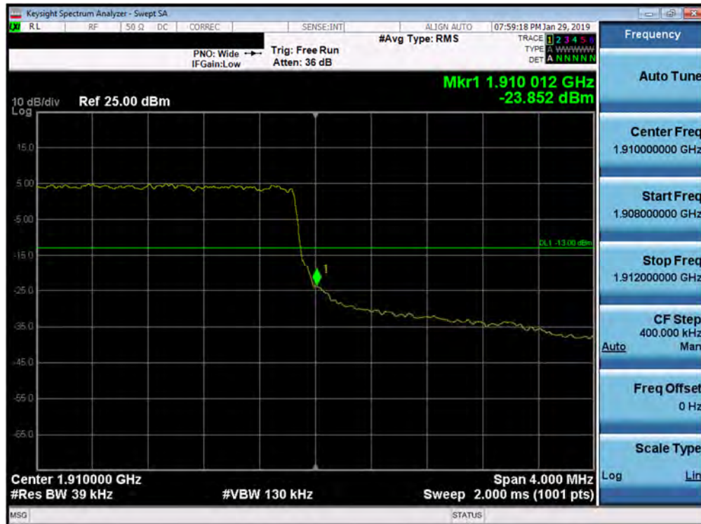
Plot 7-154. Upper Band Edge Plot (Band 2 - 3.0MHz QPSK - Full RB Configuration)
