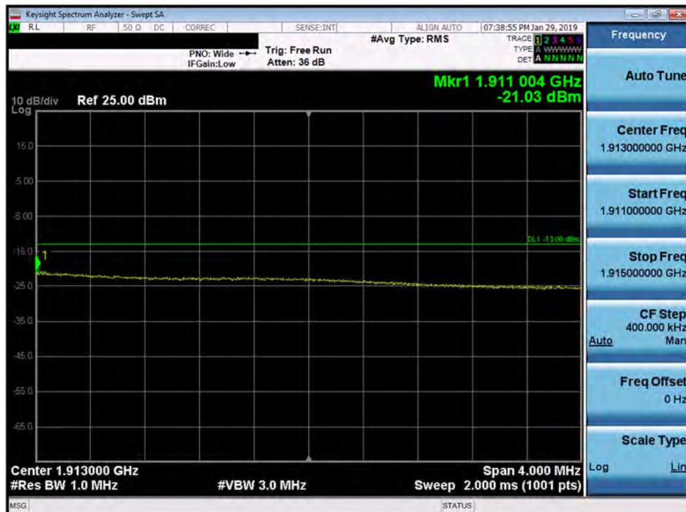
Plot 7-167. Upper Extended Band Edge Plot (Band 2 - 15.0MHz QPSK - Full RB Configuration)
