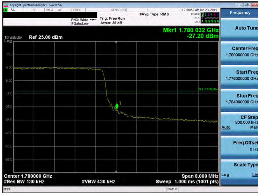
Plot 7-134. Upper Band Edge Plot (Band 66 - 10.0MHz QPSK - Full RB Configuration)
