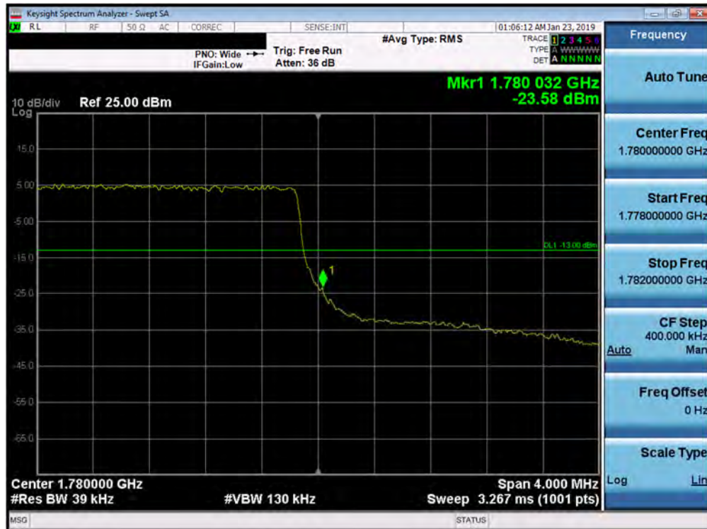
Plot 7-122. Upper Band Edge Plot (Band 66 - 3.0MHz QPSK - Full RB Configuration)
