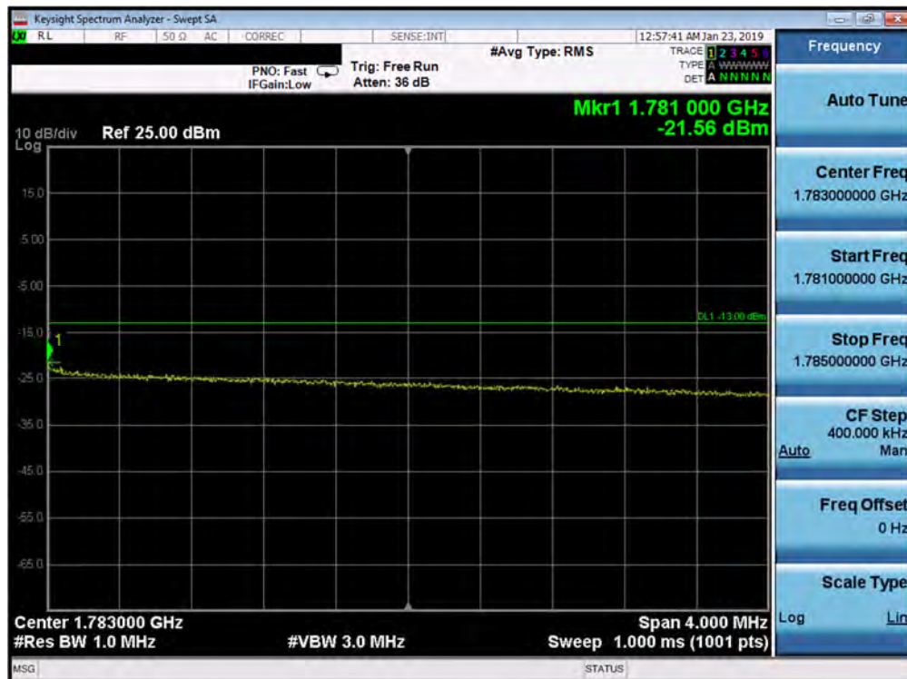
Plot 7-135. Upper Extended Band Edge Plot (Band 66 - 10.0MHz QPSK - Full RB Configuration)
