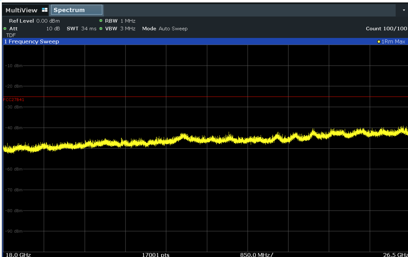
Plot 7-210. Radiated Spurious Plot 18GHz – 26.5GHz (Band 41) - V
