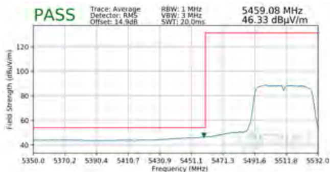
Plot 7-95. Radiated Lower Band Edge Plot SISO ANT1 (Average – UNII Band 2C)
