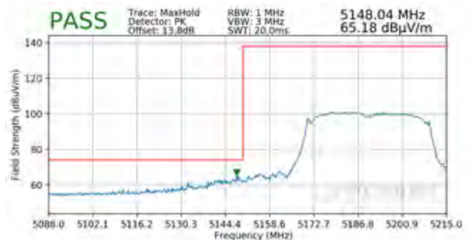
Plot 7-92. Radiated Lower Band Edge Plot SISO ANT1 (Peak – UNII Band 1)
