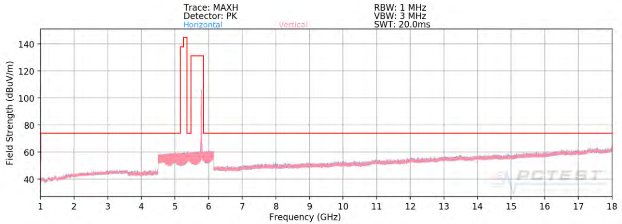
Plot 7-81. Radiated Spurious Plot above 1GHz (802.11a – U3 Ch. 157)
