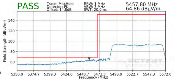
Plot 7-103. Radiated Lower Band Edge Plot - SISO (Peak – UNII Band 2C)
