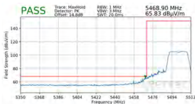
Plot 7-89. Radiated Lower Band Edge Plot SISO ANT1 (Peak – UNII Band 2C)
