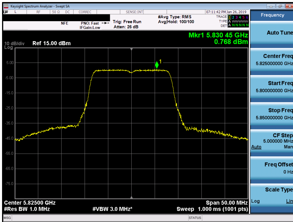
Plot 7-71. Power Spectral Density Plot (802.11a (UNII Band 3) – Ch. 165)
