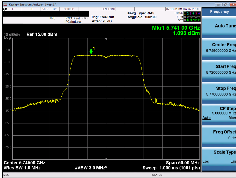
Plot 7-72. Power Spectral Density Plot (20MHz BW 802.11n (UNII Band 3) – Ch. 149)
