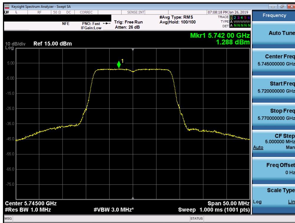
Plot 7-69. Power Spectral Density Plot (802.11a (UNII Band 3) – Ch. 149)
