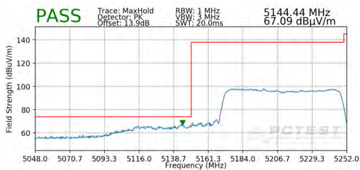
Plot 7-99. Radiated Lower Band Edge Plot – SISO (Peak – UNII Band 1)
