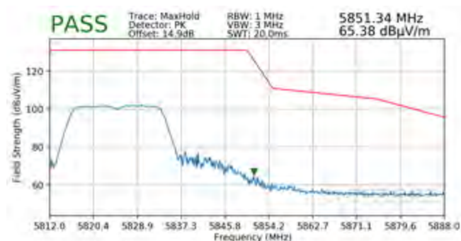
Plot 7-90. Radiated Upper Band Edge Plot SISO ANT1 (Peak – UNII Band 3)
