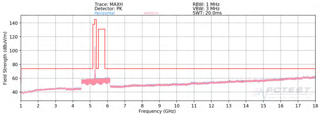
Plot 7-79. Radiated Spurious Plot above 1GHz (802.11a – U2A Ch. 56)
