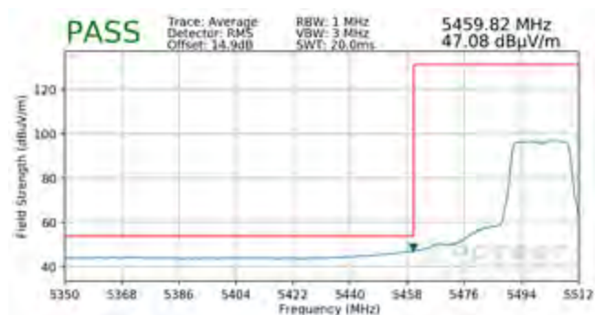
Plot 7-88. Radiated Lower Band Edge Plot SISO ANT1 (Average – UNII Band 2C)
