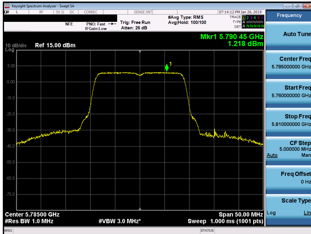
Plot 7-73. Power Spectral Density Plot (20MHz BW 802.11n (UNII Band 3) – Ch. 157)
