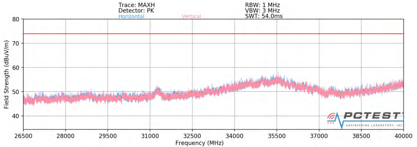
Plot 7-83. Radiated Spurious Plot 26.5GHz - 40GHz (802.11a)
