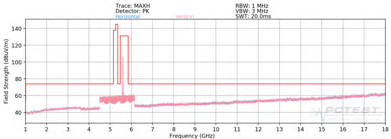
Plot 7-80. Radiated Spurious Plot above 1GHz (802.11a – U2C Ch.120)
