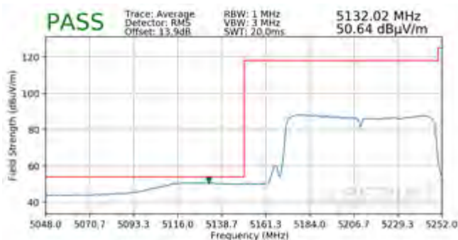
Plot 7-98. Radiated Lower Band Edge Plot – SISO (Average – UNII Band 1)
