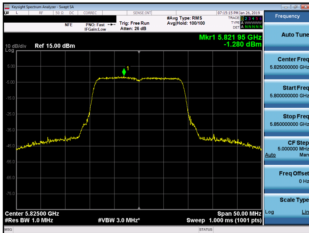
Plot 7-74. Power Spectral Density Plot (20MHz BW 802.11n (UNII Band 3) – Ch. 165)
