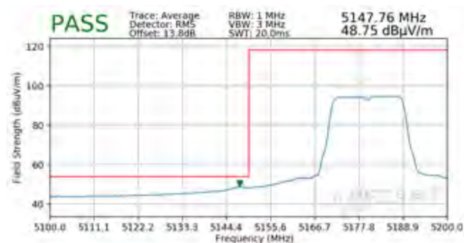
Plot 7-84. Radiated Lower Band Edge Plot SISO ANT1 (Average – UNII Band 1)
