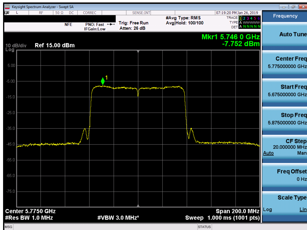
Plot 7-77. Power Spectral Density Plot (80MHz BW 802.11ac (UNII Band 3) – Ch. 155)
