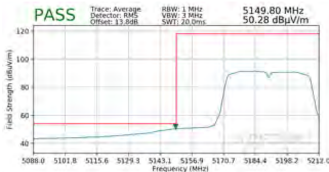
Plot 7-91. Radiated Lower Band Edge Plot SISO ANT1 (Average – UNII Band 1)
