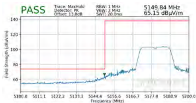
Plot 7-85. Radiated Lower Band Edge Plot SISO ANT1 (Peak – UNII Band 1)
