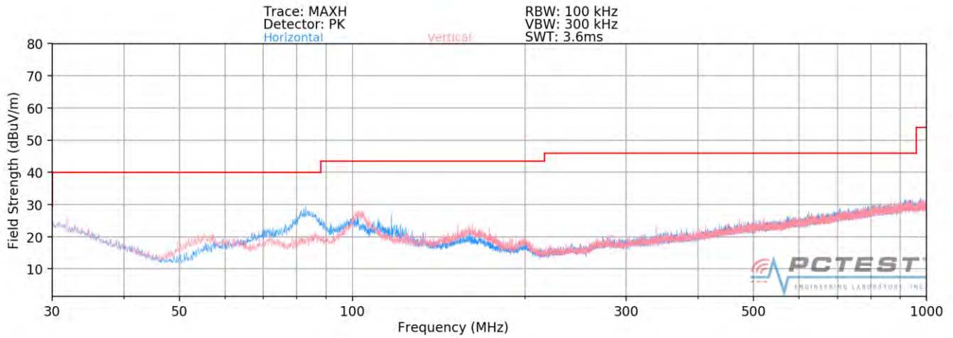
Plot 7-105. Radiated Spurious Plot below 1GHz (802.11a – U3 Ch. 157)
