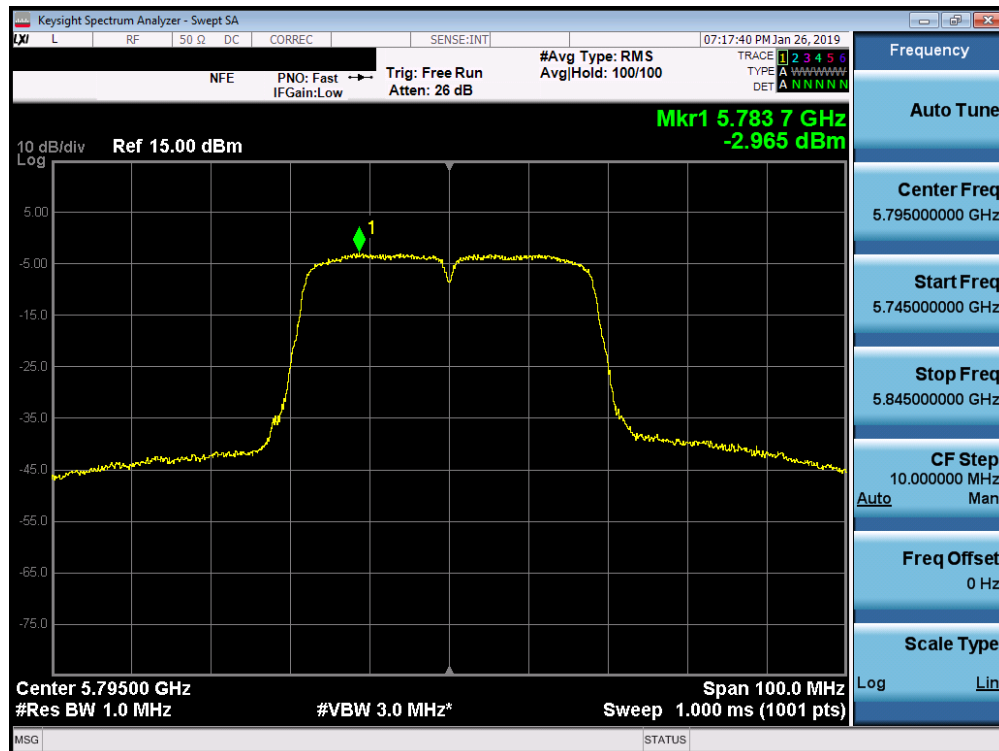
Plot 7-76. Power Spectral Density Plot (40MHz BW 802.11n (UNII Band 3) – Ch. 159)
