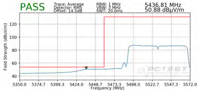
Plot 7-102. Radiated Lower Band Edge Plot – SISO (Average – UNII Band 2C)
