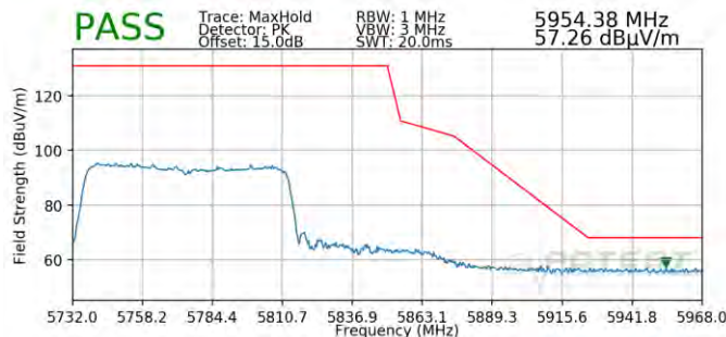
Plot 7-104. Radiated Upper Band Edge Plot MIMO (Peak – UNII Band 3)
