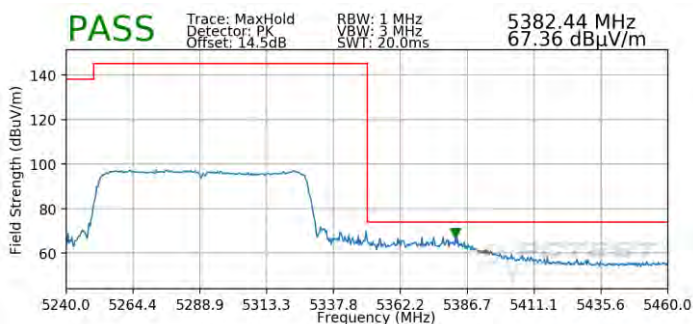
Plot 7-101. Radiated Upper Band Edge Plot – SISO (Peak – UNII Band 2A)
