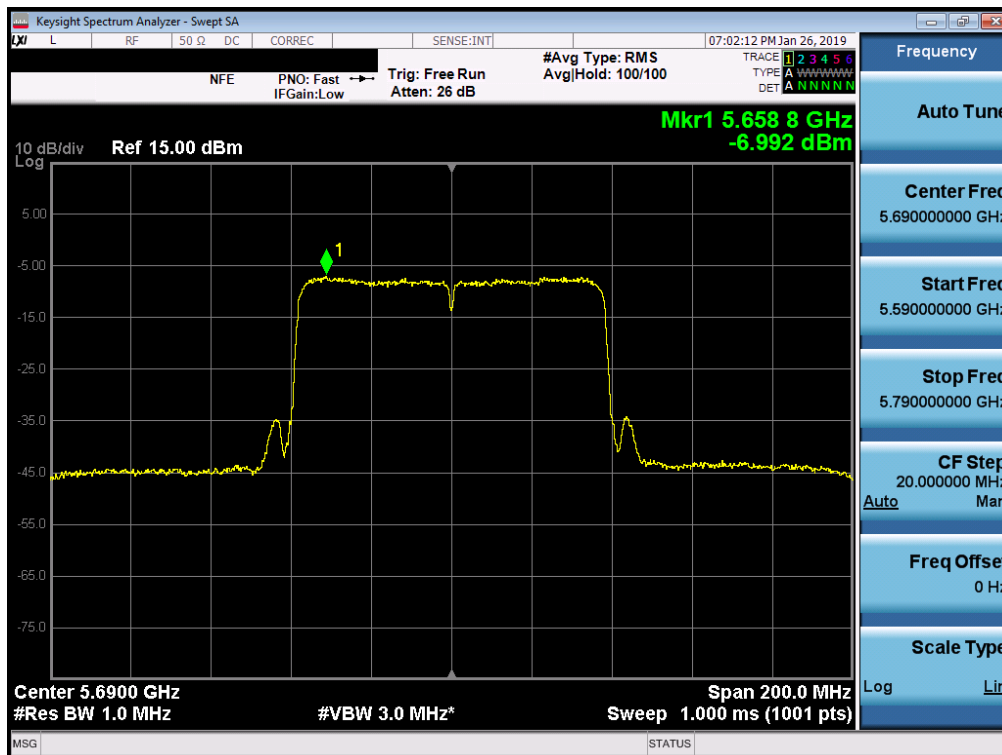
Plot 7-68. Power Spectral Density Plot (80MHz BW 802.11ac (UNII Band 2C) – Ch. 138)
