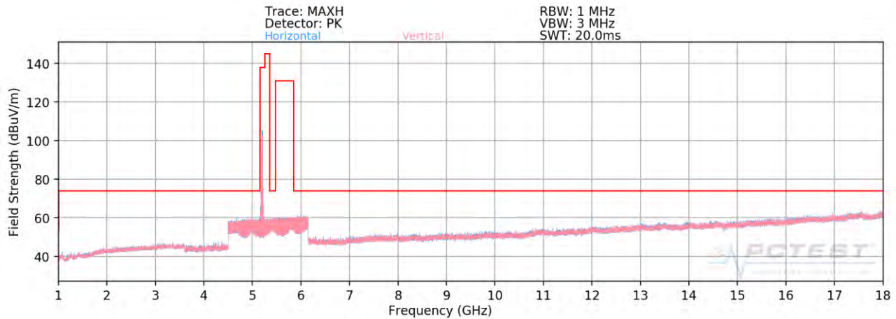
Plot 7-78. Radiated Spurious Plot above 1GHz (802.11a – U1 Ch. 40)
