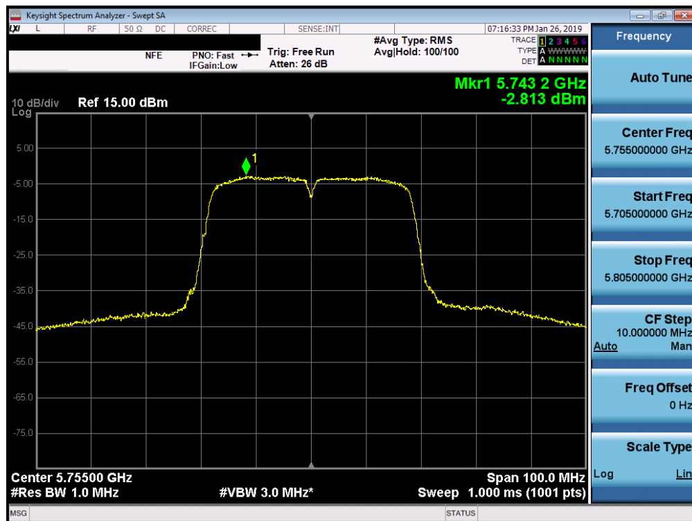
Plot 7-75. Power Spectral Density Plot (40MHz BW 802.11n (UNII Band 3) – Ch. 151)
