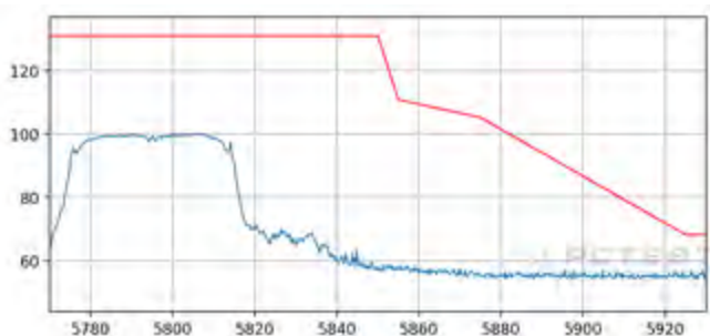
Plot 7-97. Radiated Upper Band Edge Plot SISO ANT1 (Peak – UNII Band 3)
