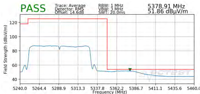
Plot 7-100. Radiated Upper Band Edge Plot - SISO (Average – UNII Band 2A)
