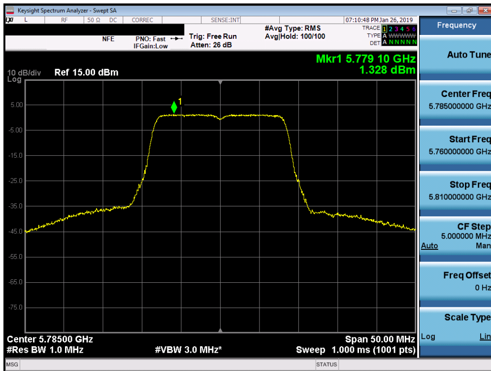
Plot 7-70. Power Spectral Density Plot (802.11a (UNII Band 3) – Ch. 157)
