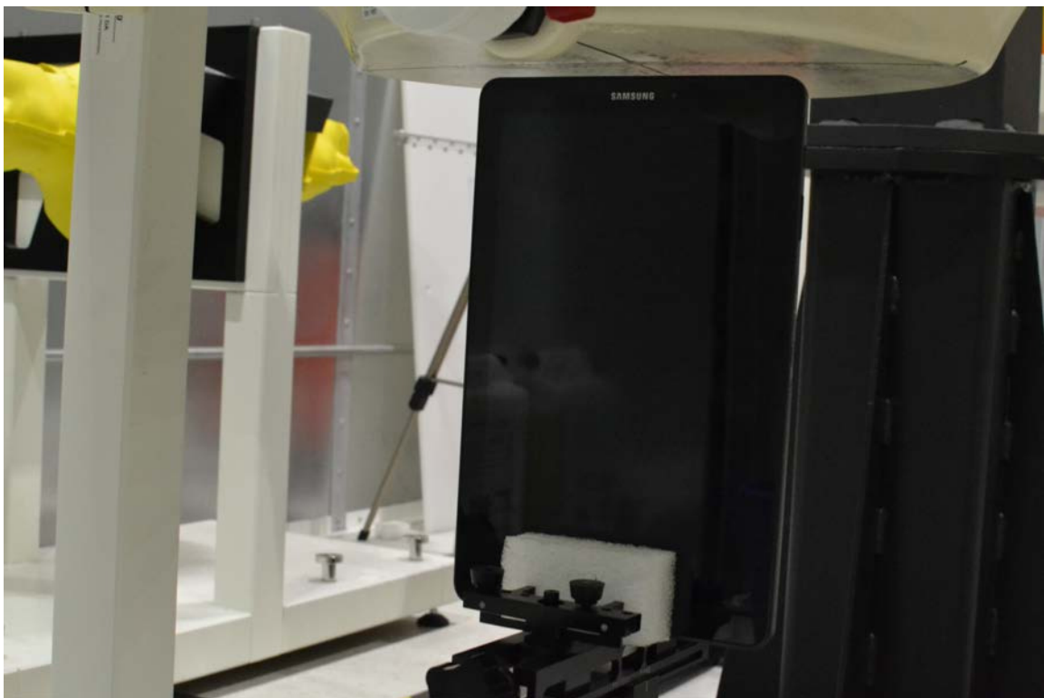
SAR Test Setup Photo 3: Top Edge at 0.4 cm
