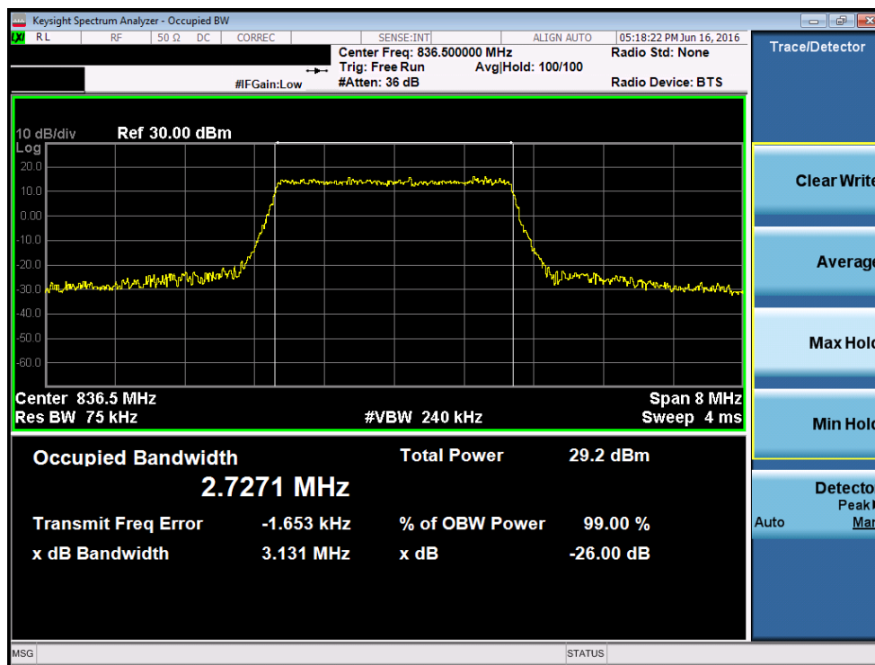
Plot 7-4. Occupied Bandwidth Plot (Band 5 – 3.0MHz 16-QAM – RB Size 15)
