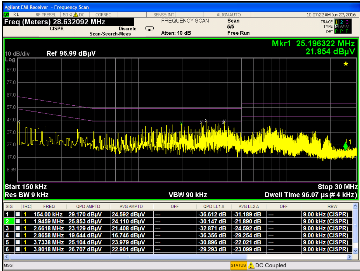
Plot 7-6. Line-Conducted Test Plot (L1)
