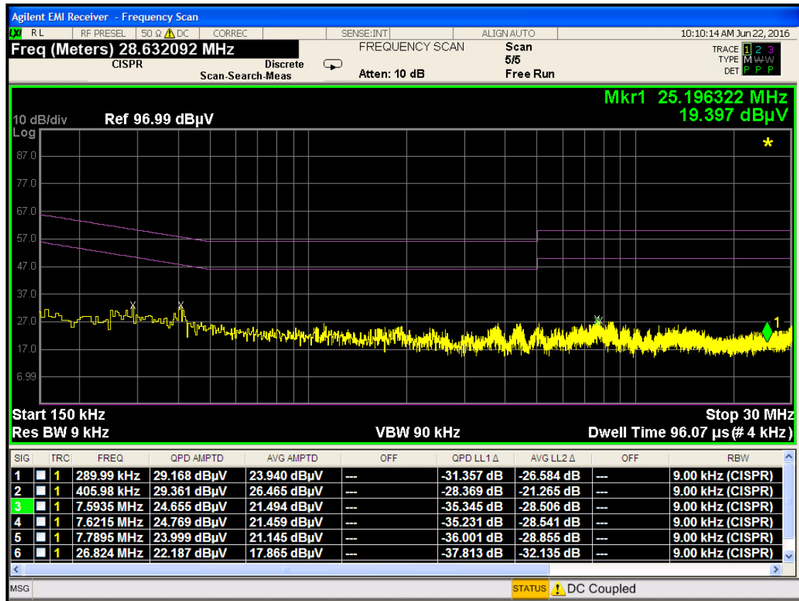
Plot 7-7. Line-Conducted Test Plot (N)
