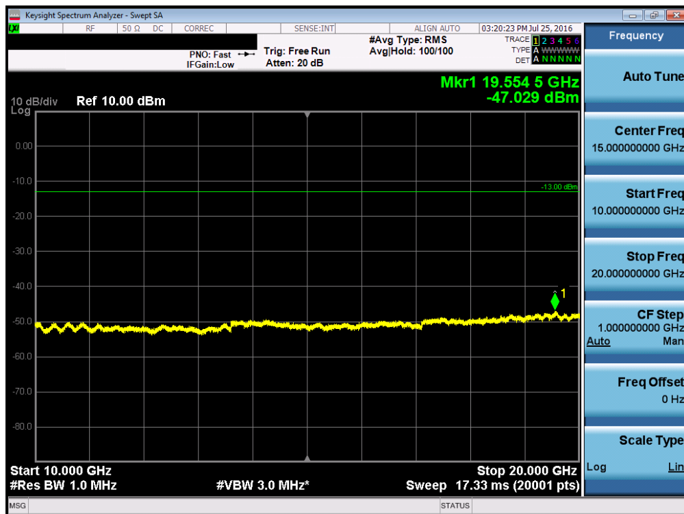
Plot 7-72. Conducted Spurious Plot (Band 2 – 5.0MHz QPSK – RB Size 1, RB Offset 0 – High Channel)
