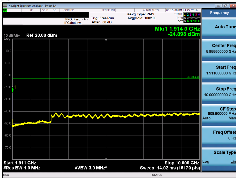
Plot 7-71. Conducted Spurious Plot (Band 2 – 5.0MHz QPSK – RB Size 1, RB Offset 0 – High Channel)
