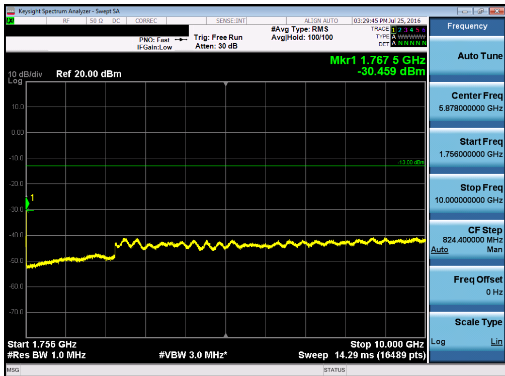
Plot 7-62. Conducted Spurious Plot (Band 4 – 15.0MHz QPSK – RB Size 1, RB Offset 0 – High Channel)
