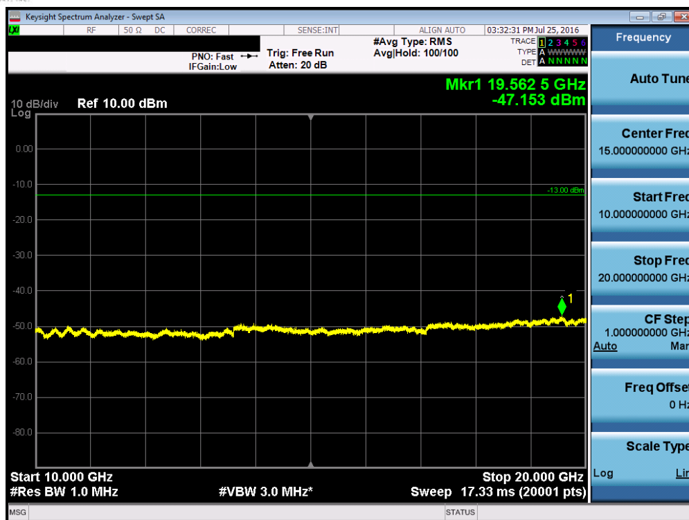
Plot 7-57. Conducted Spurious Plot (Band 4 – 15.0MHz QPSK – RB Size 1, RB Offset 0 – Low Channel)
