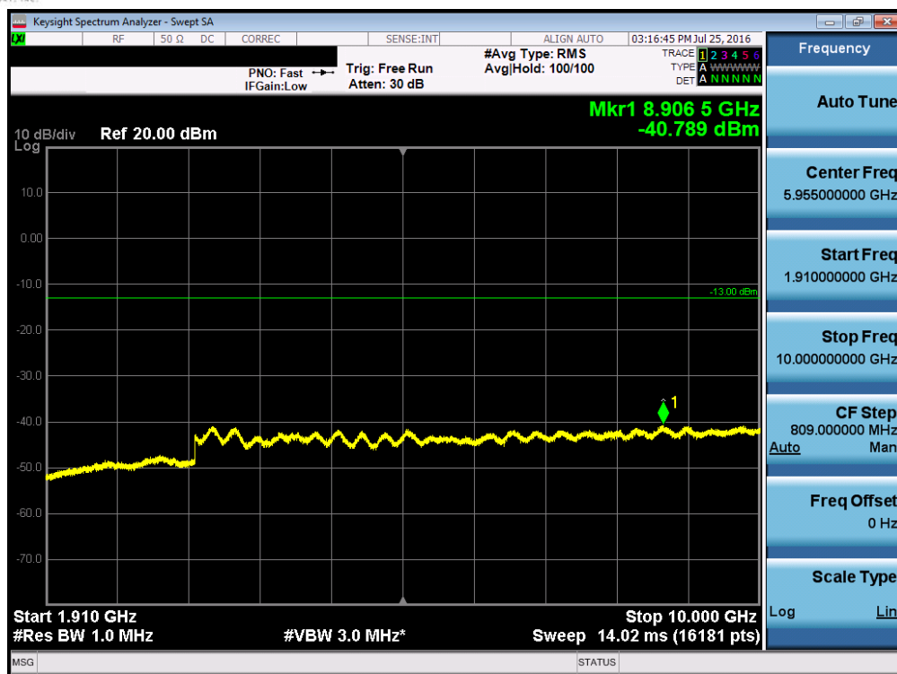
Plot 7-65. Conducted Spurious Plot (Band 2 – 5.0MHz QPSK – RB Size 1, RB Offset 0 – Low Channel)
