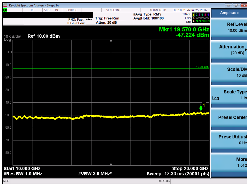
Plot 7-66. Conducted Spurious Plot (Band 2 – 5.0MHz QPSK – RB Size 1, RB Offset 0 – Low Channel)
