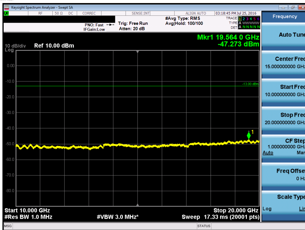
Plot 7-69. Conducted Spurious Plot (Band 2 – 5.0MHz QPSK – RB Size 1, RB Offset 0 – Mid Channel)
