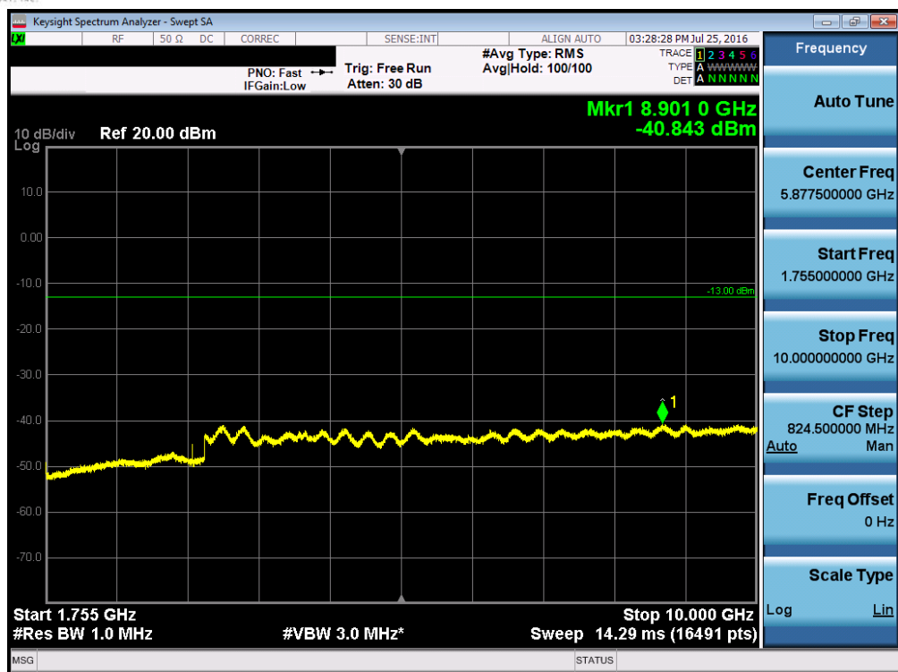
Plot 7-59. Conducted Spurious Plot (Band 4 – 15.0MHz QPSK – RB Size 1, RB Offset 0 – Mid Channel)
