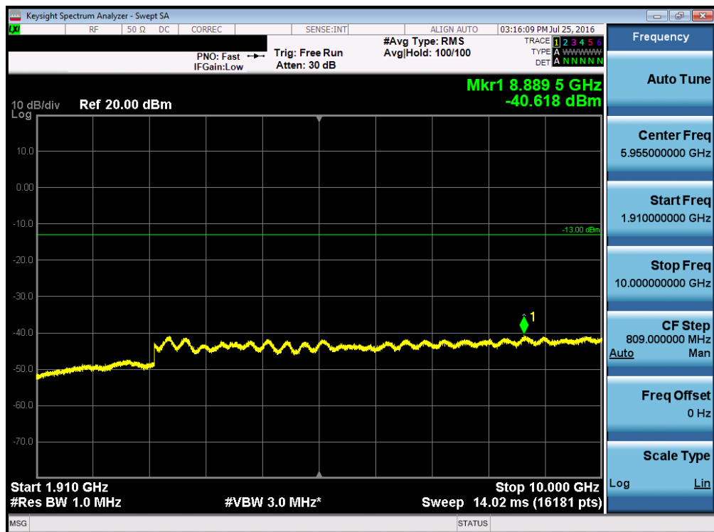
Plot 7-68. Conducted Spurious Plot (Band 2 – 5.0MHz QPSK – RB Size 1, RB Offset 0 – Mid Channel)
