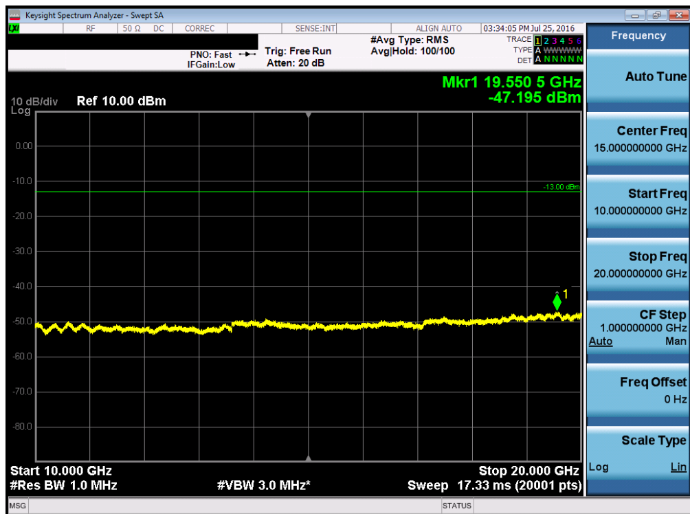
Plot 7-60. Conducted Spurious Plot (Band 4 – 15.0MHz QPSK – RB Size 1, RB Offset 0 – Mid Channel)
