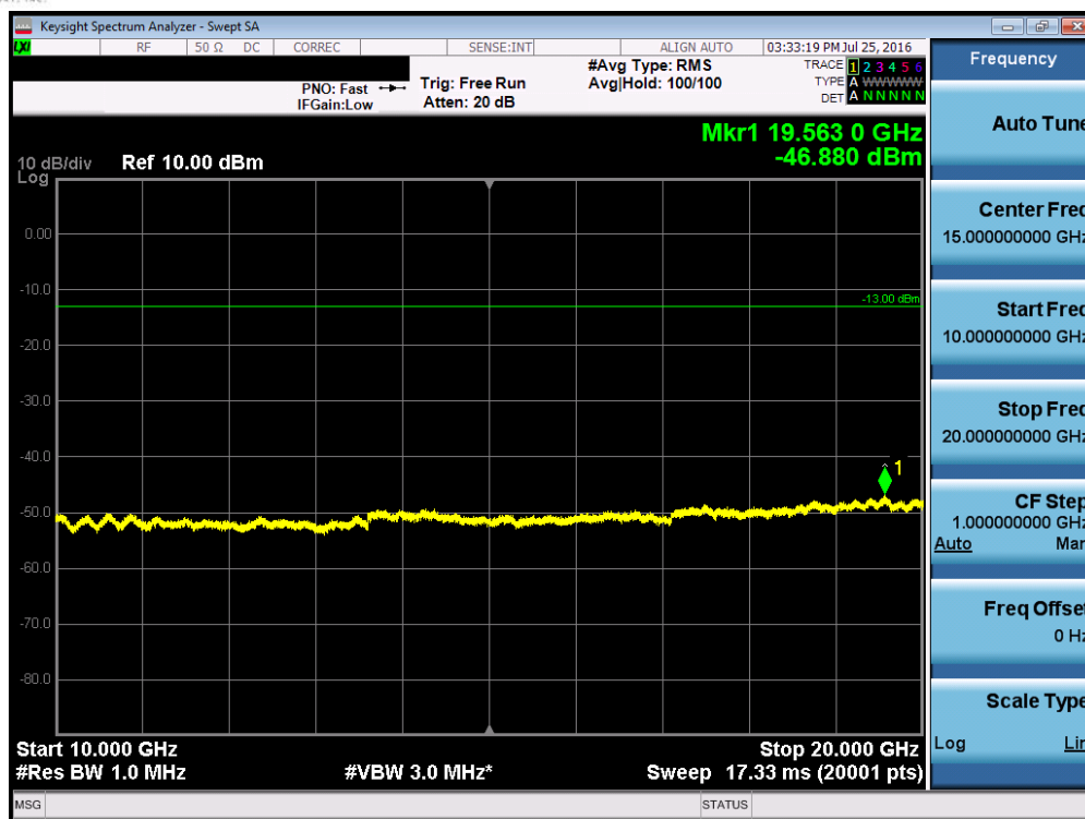
Plot 7-63. Conducted Spurious Plot (Band 4 – 15.0MHz QPSK – RB Size 1, RB Offset 0 – High Channel)
