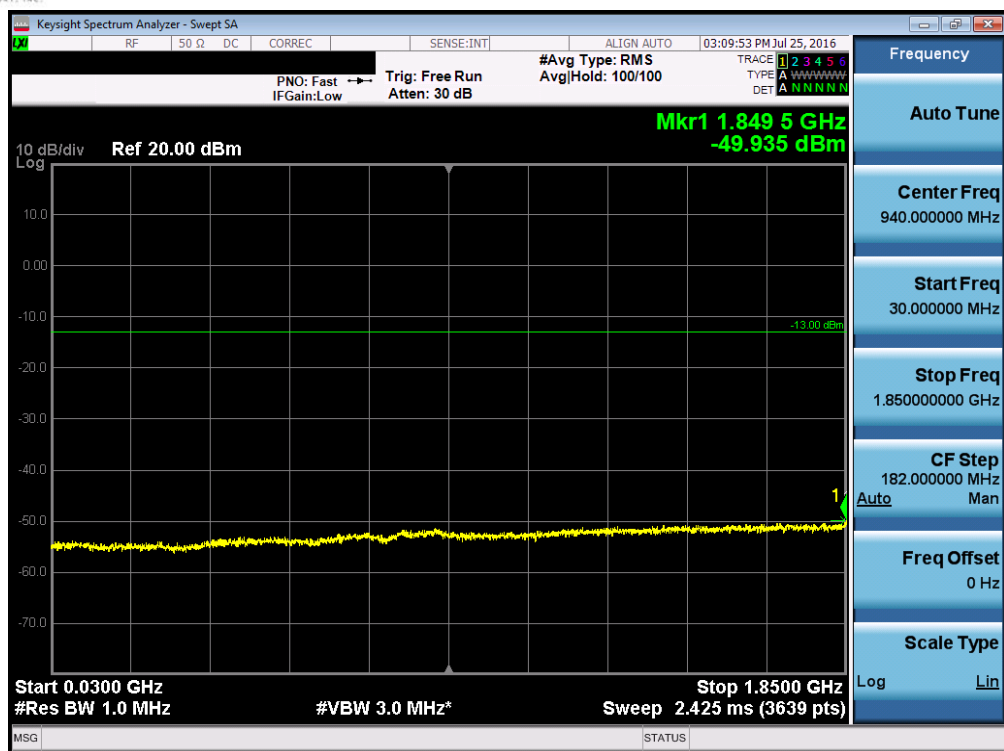
Plot 7-67. Conducted Spurious Plot (Band 2 – 5.0MHz QPSK – RB Size 1, RB Offset 0 – Mid Channel)
