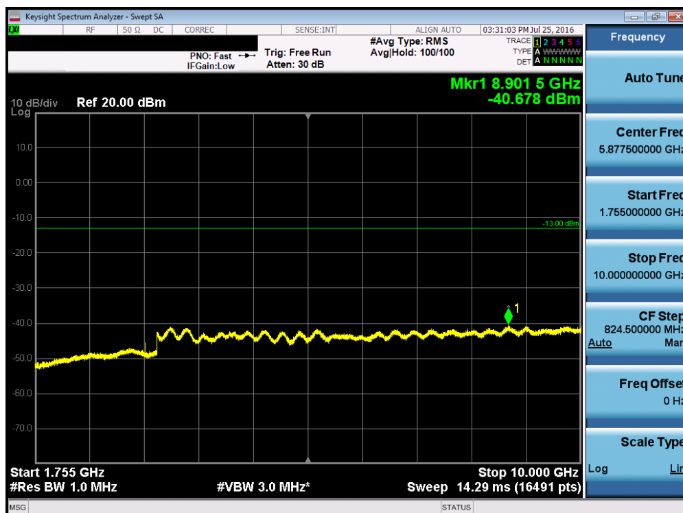
Plot 7-56. Conducted Spurious Plot (Band 4 – 15.0MHz QPSK – RB Size 1, RB Offset 0 – Low Channel)
