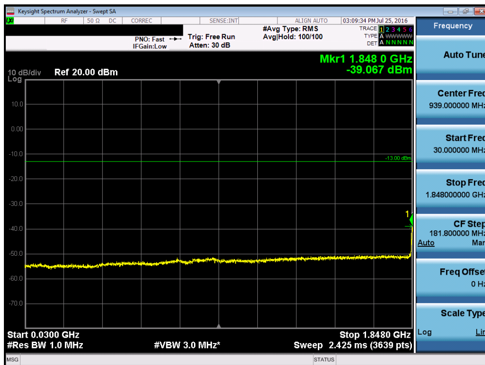
Plot 7-64. Conducted Spurious Plot (Band 2 – 5.0MHz QPSK – RB Size 1, RB Offset 0 – Low Channel)
