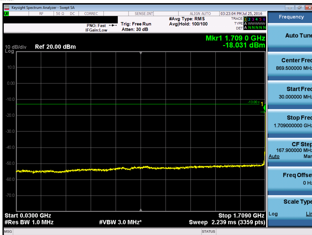
Plot 7-55. Conducted Spurious Plot (Band 4 – 15.0MHz QPSK – RB Size 1, RB Offset 0 – Low Channel)
