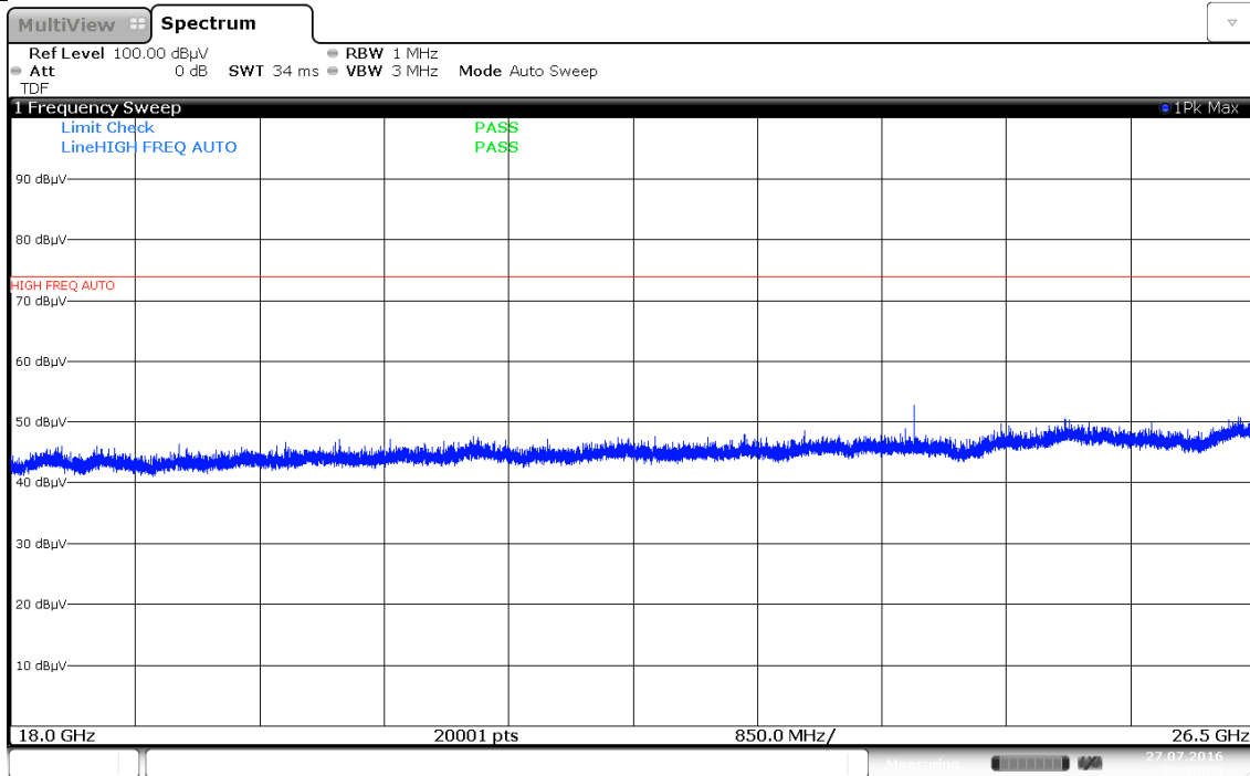
Plot 7-89. Radiated Spurious Plot above 18GHz (802.11a – Ant. Pol. V)
