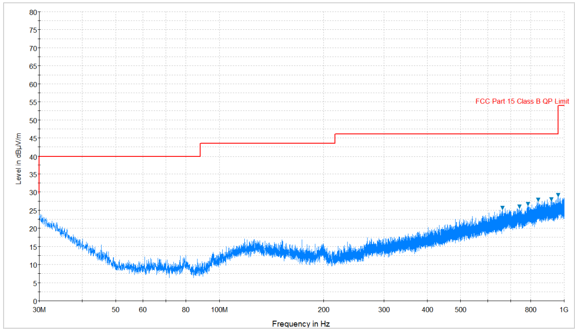
Plot 7-109. Radiated Spurious Plot below 1GHz (802.11a – U3 Ch. 157, Ant. Pol. H)
