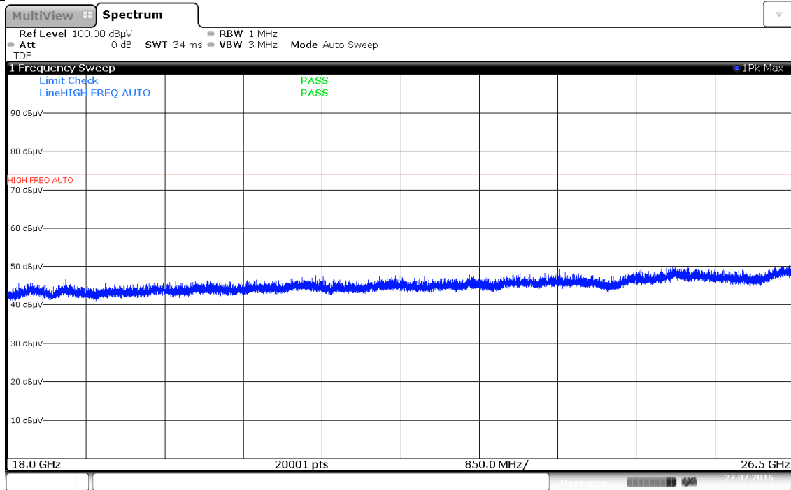
Plot 7-87. Radiated Spurious Plot above 18GHz (802.11a – Ant. Pol. H)
