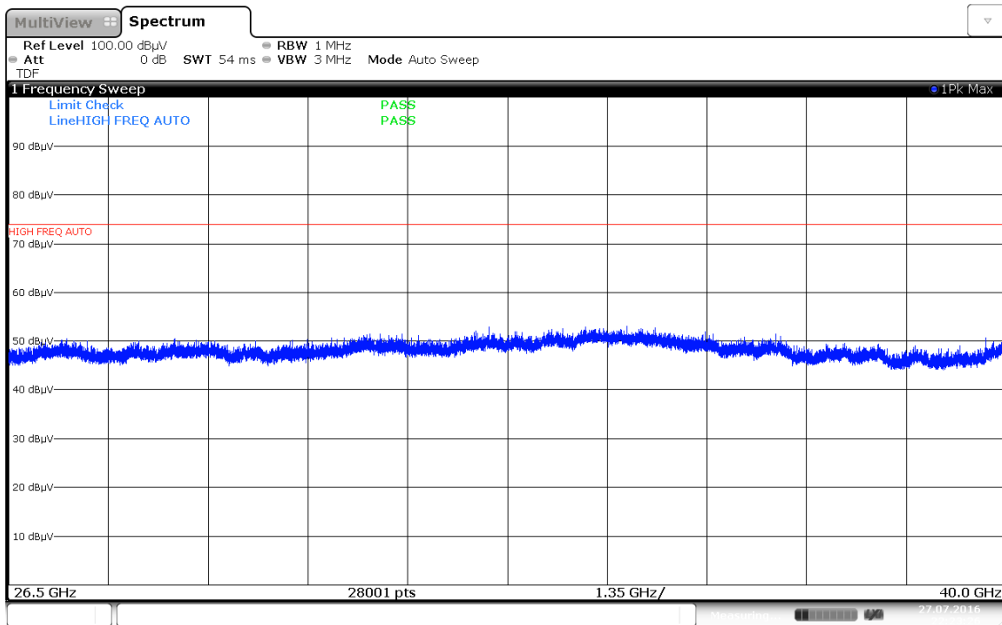
Plot 7-88. Radiated Spurious Plot above 26GHz (802.11a – Ant. Pol. H)
