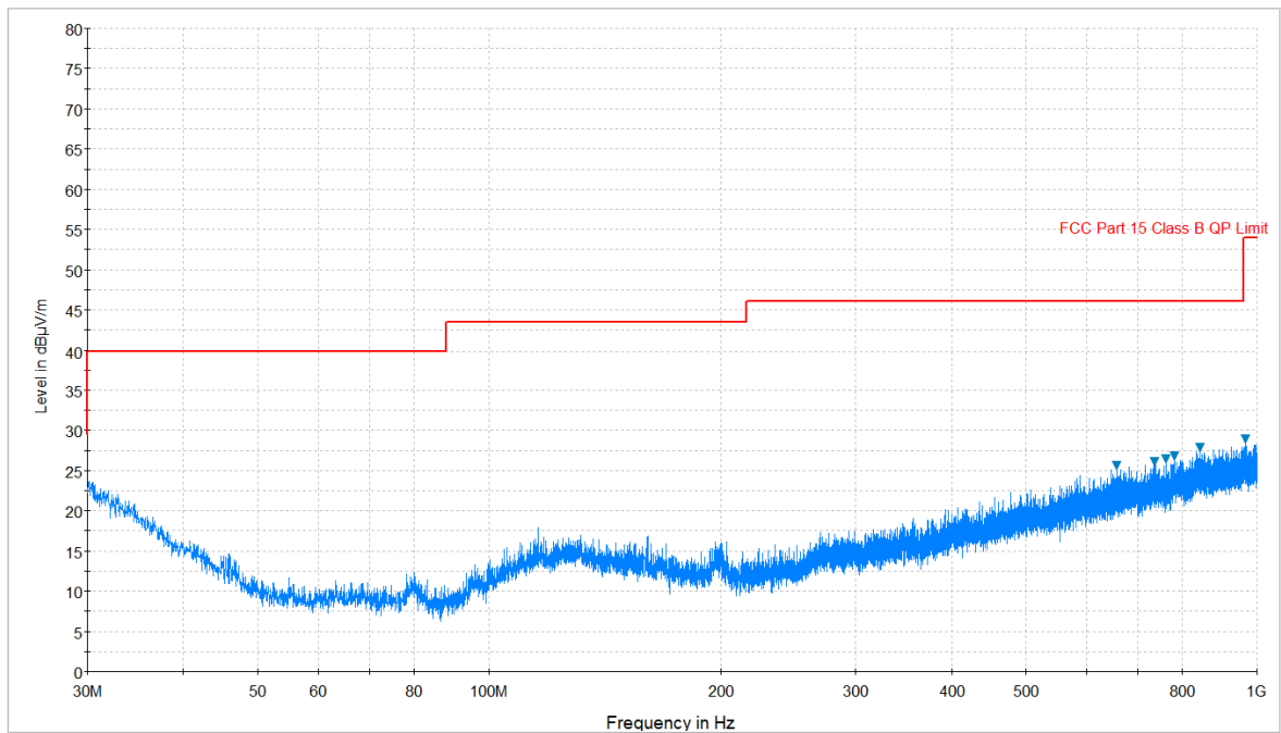
Plot 7-110. Radiated Spurious Plot below 1GHz (802.11a – U3 Ch. 157, Ant. Pol. V)
