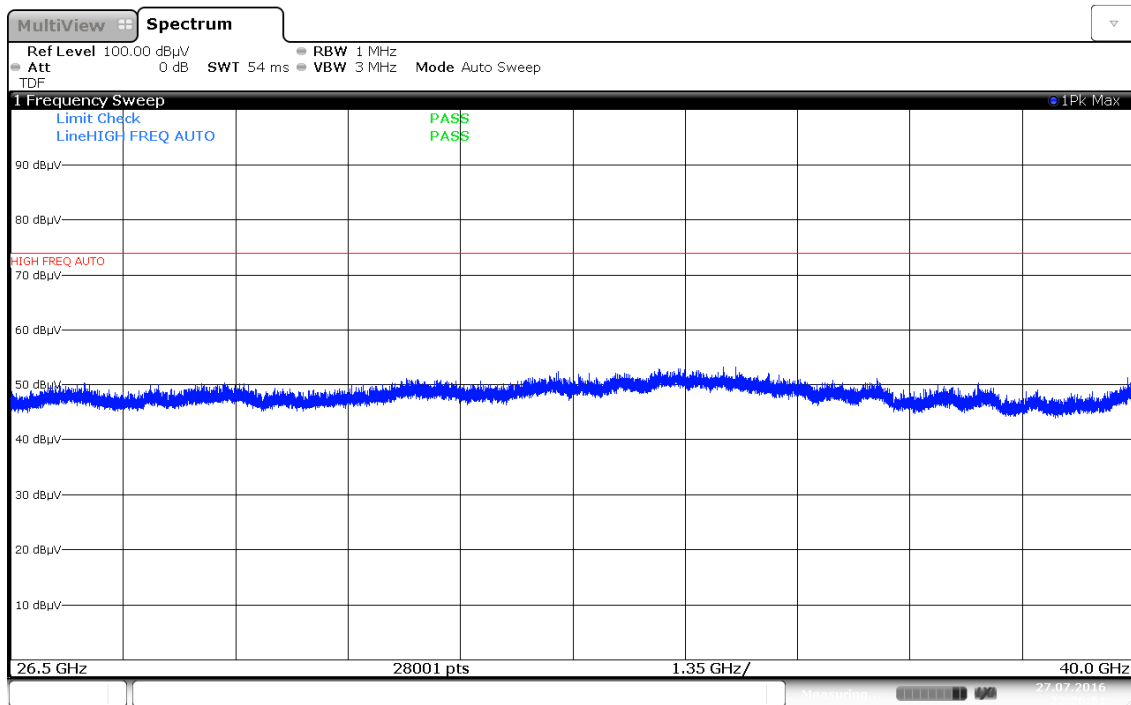
Plot 7-90. Radiated Spurious Plot above 26GHz (802.11a – Ant. Pol. V)
